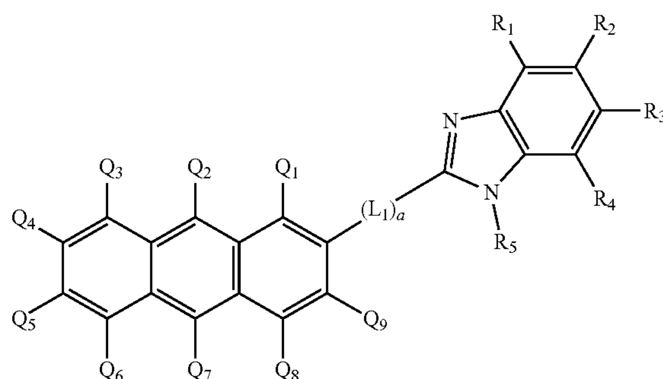
Formula 2
