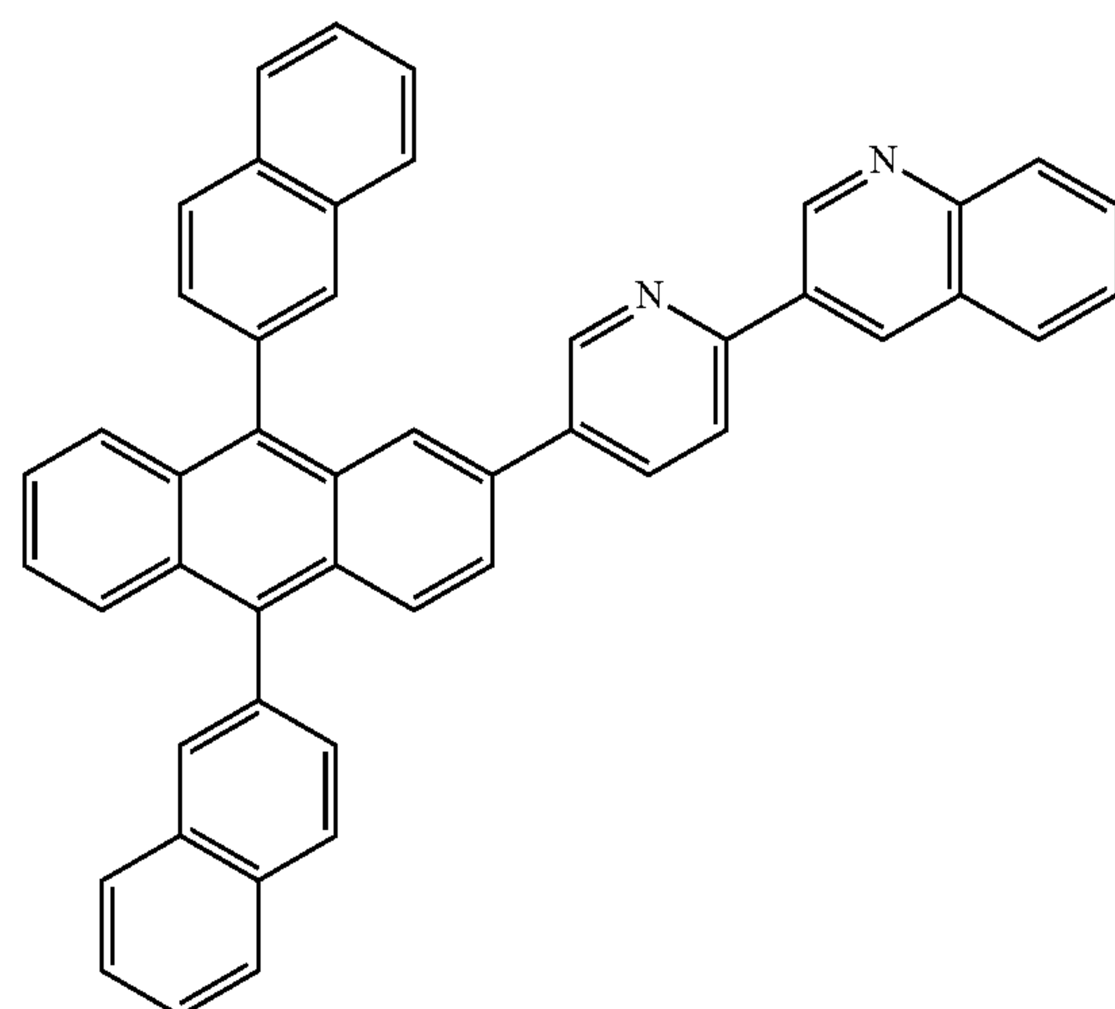
Compound 7
