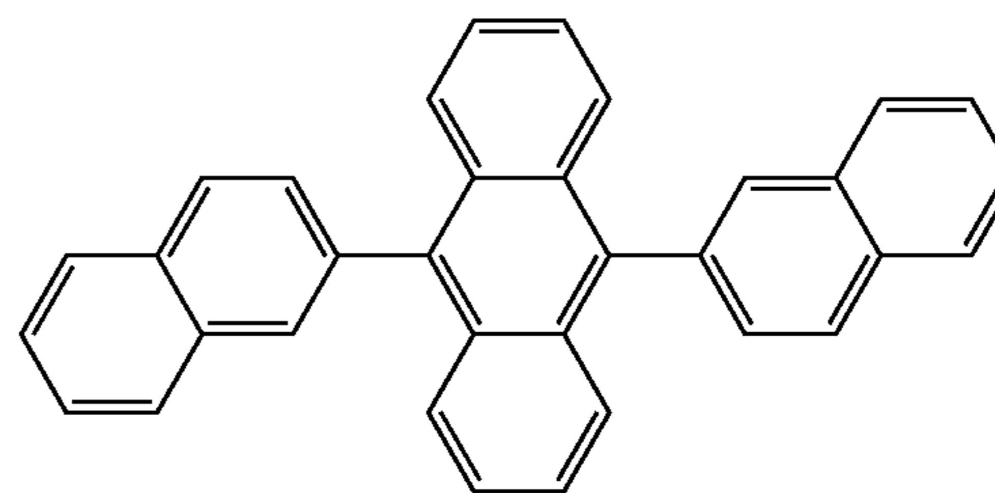
Compound 5
