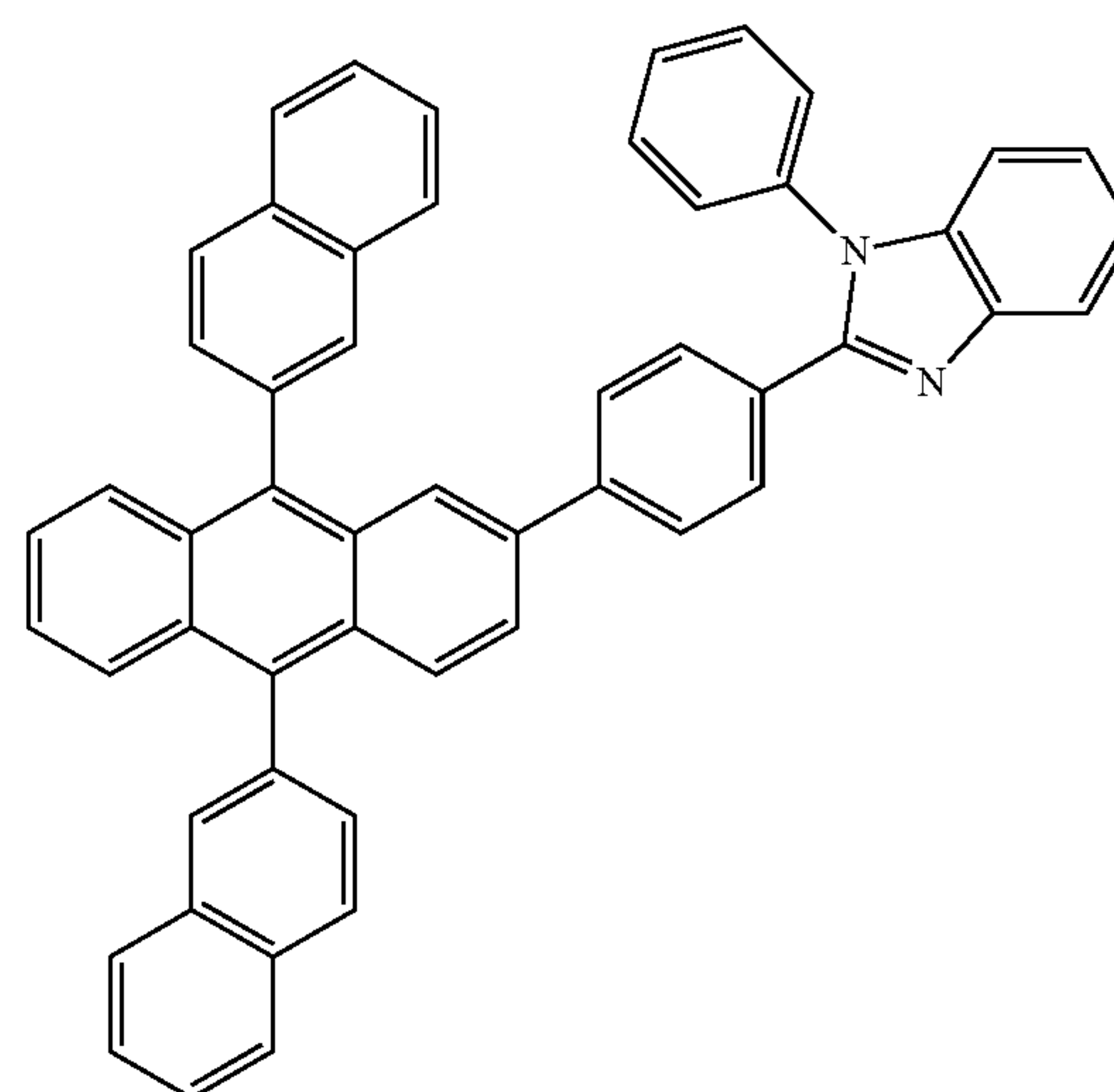
Compound 6
