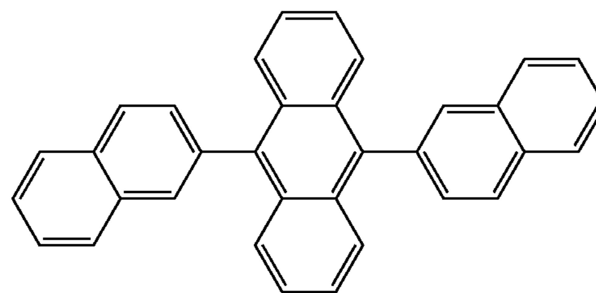
Compound 5
