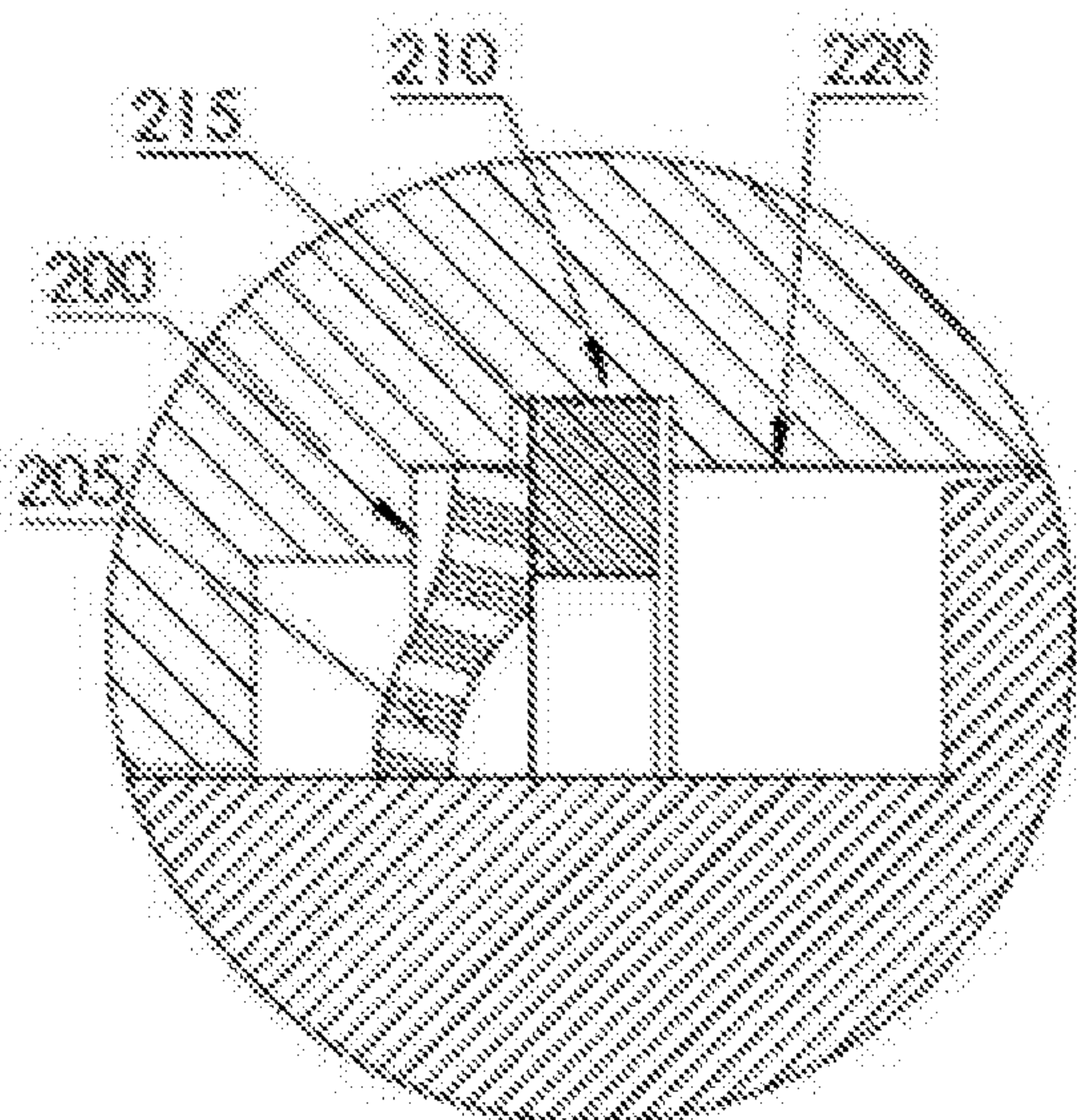
DETAIL C Retention Apparatus 265
