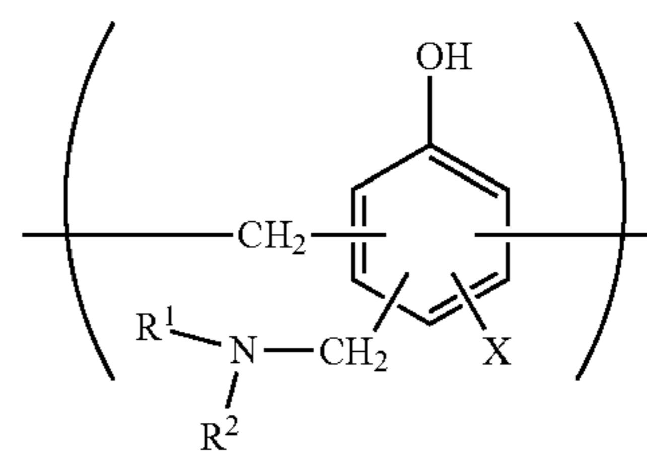
[Chemical Formula 3]
