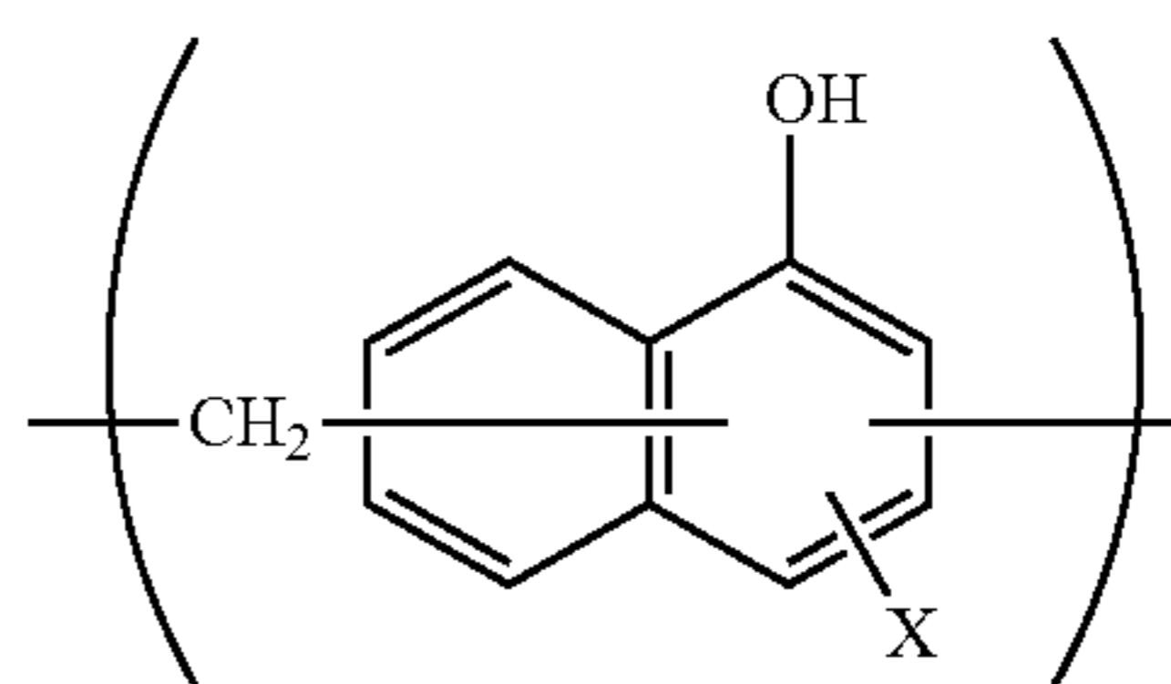
[Chemical Formula 4]
