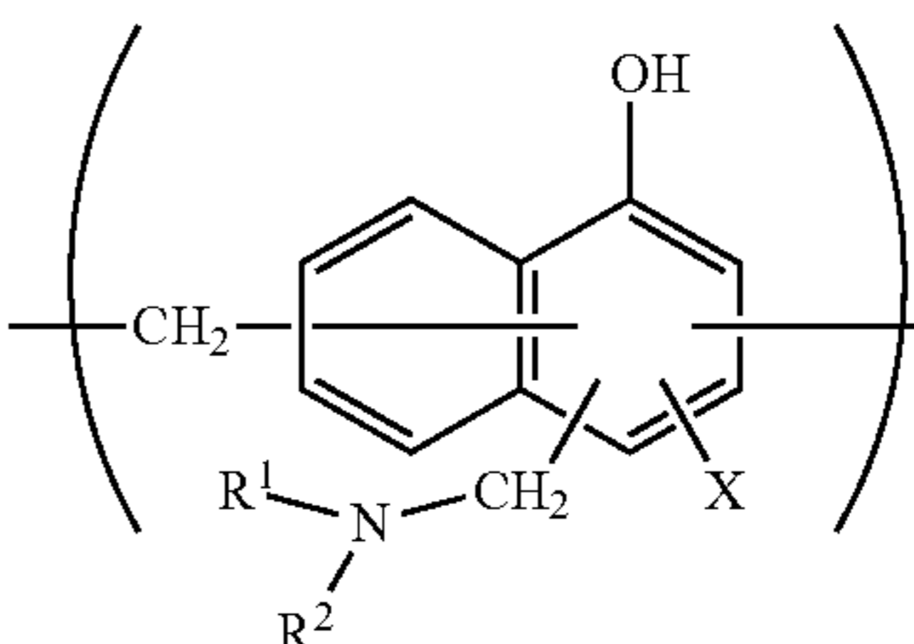
[Chemical Formula 4]
