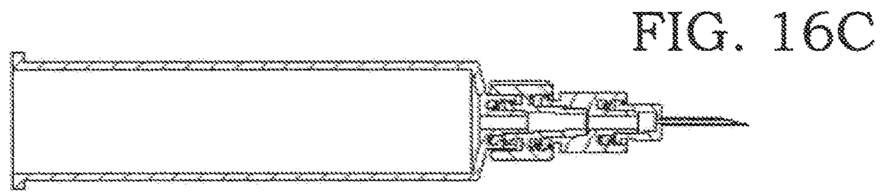
SECTION B-B
