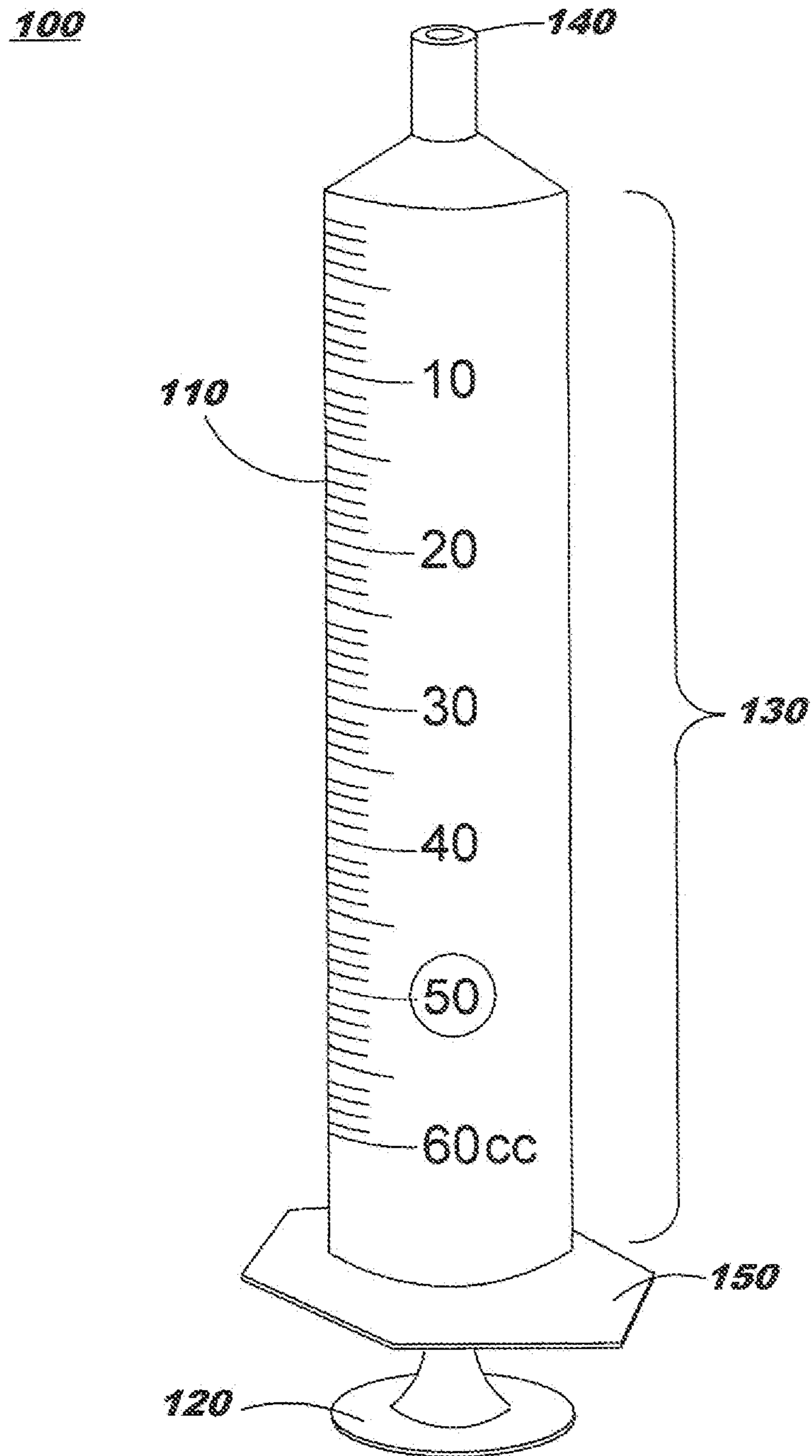
FIG. 1 (Prior Art)
