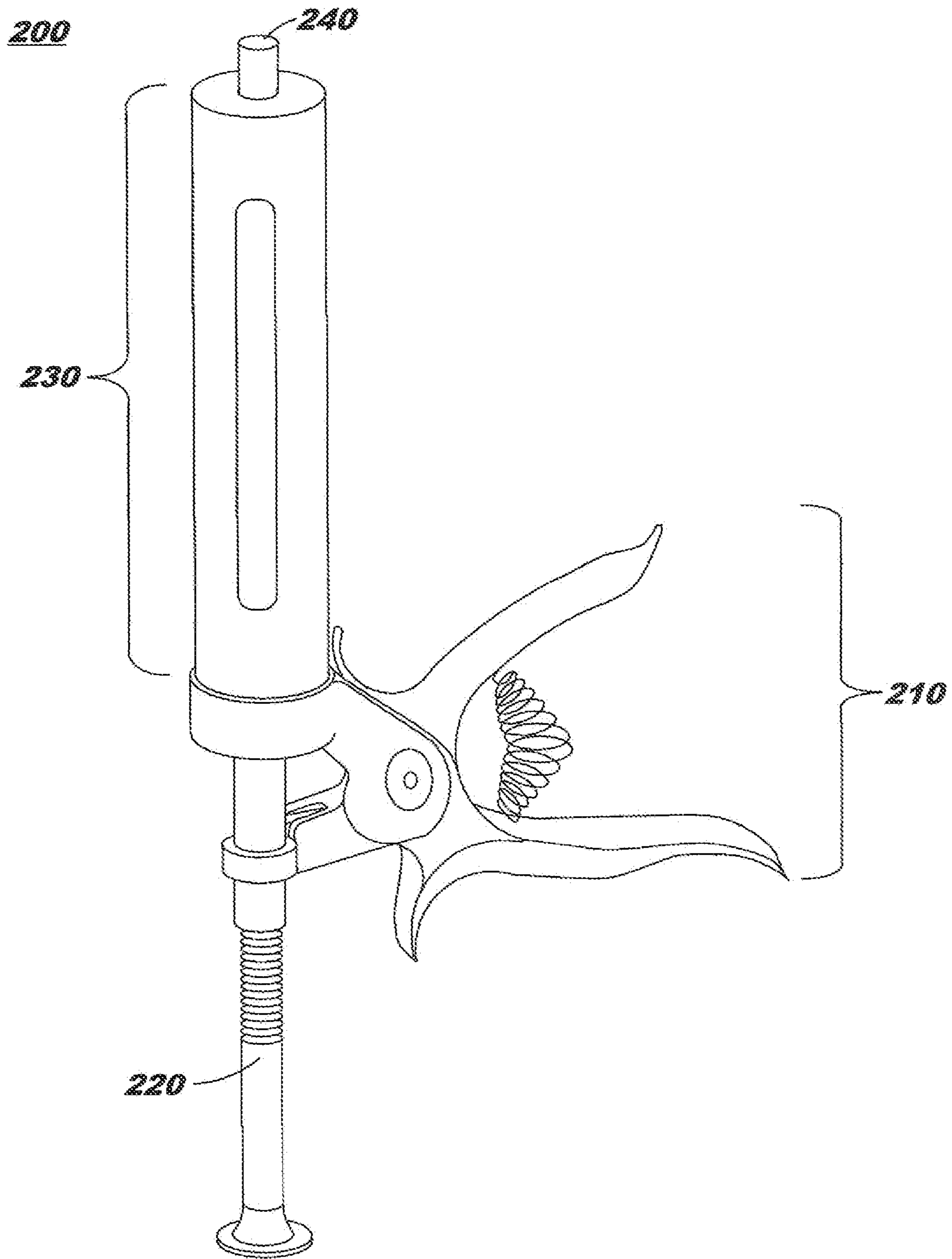
FIG. 2 (Prior Art)
