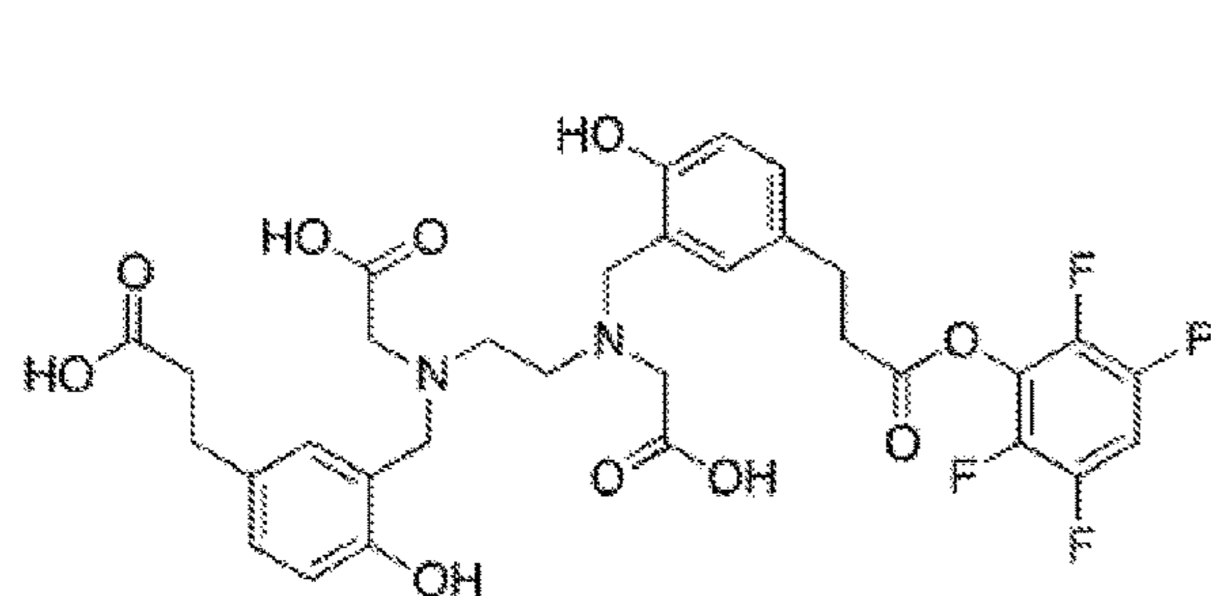
(HBED-CC)TFP
