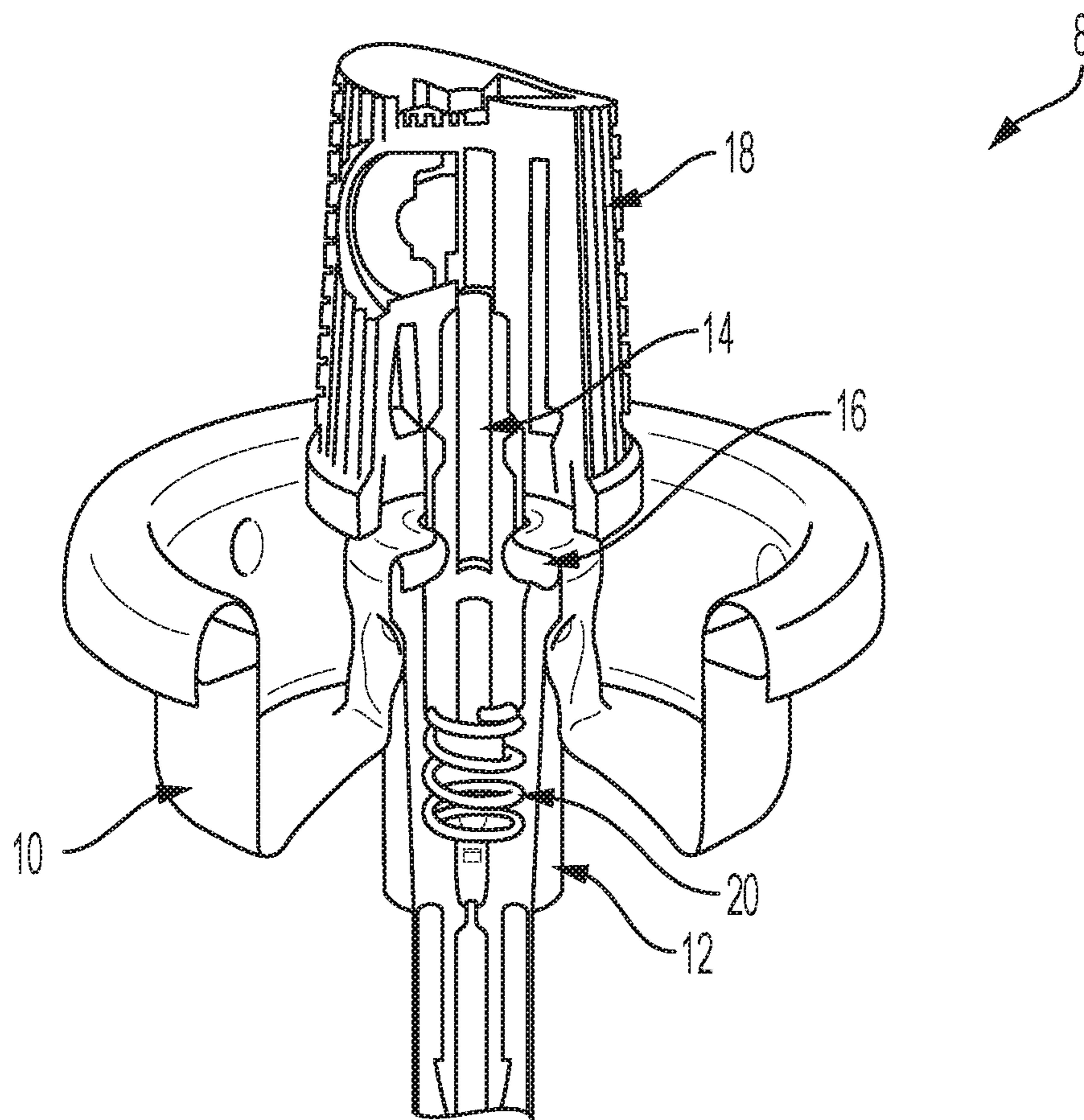
FIG. 1 PRIOR ART
