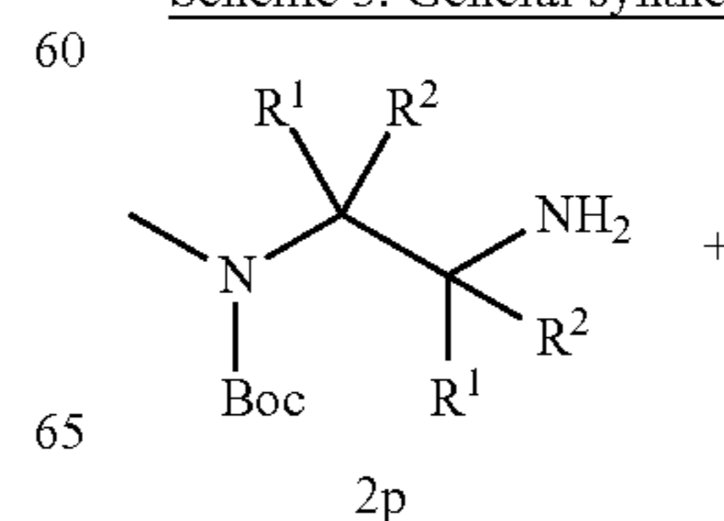
Scheme 3. General synthesis of [6,8] systems of nucleophilic substitution
