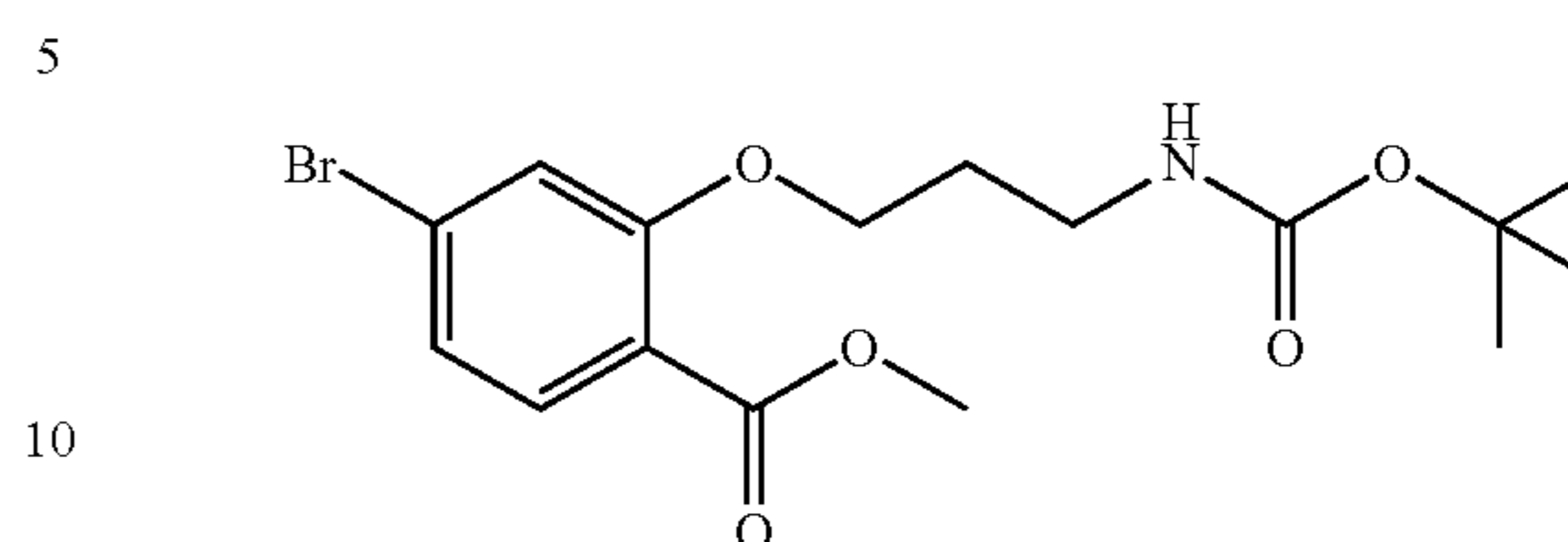
Step-2: Methyl 4-bromo-2-(3-(tert-butoxycarbonylamino)propoxy)benzoate
