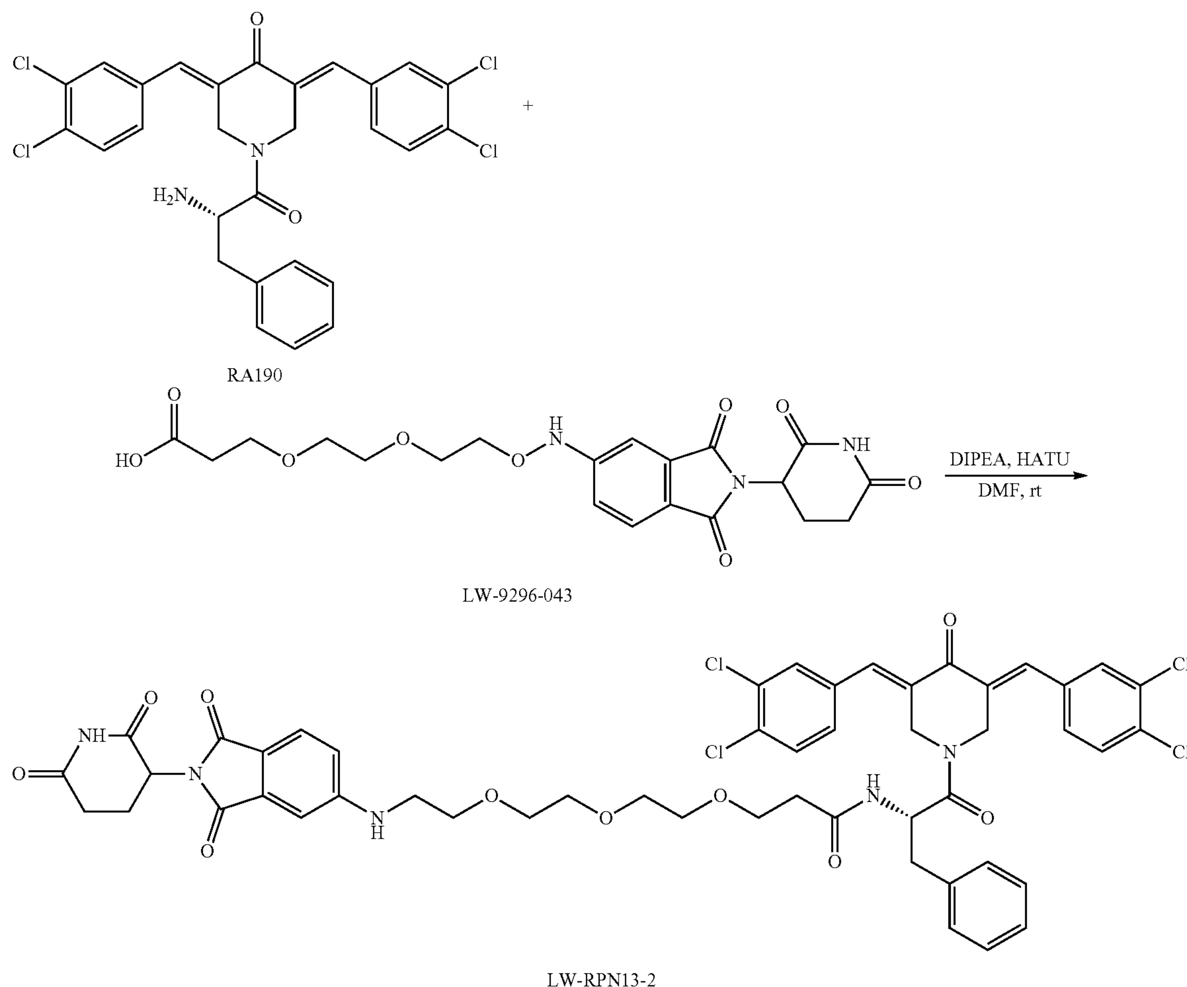
Scheme 3. Exemplary synthesis of LW-RPN13-2
