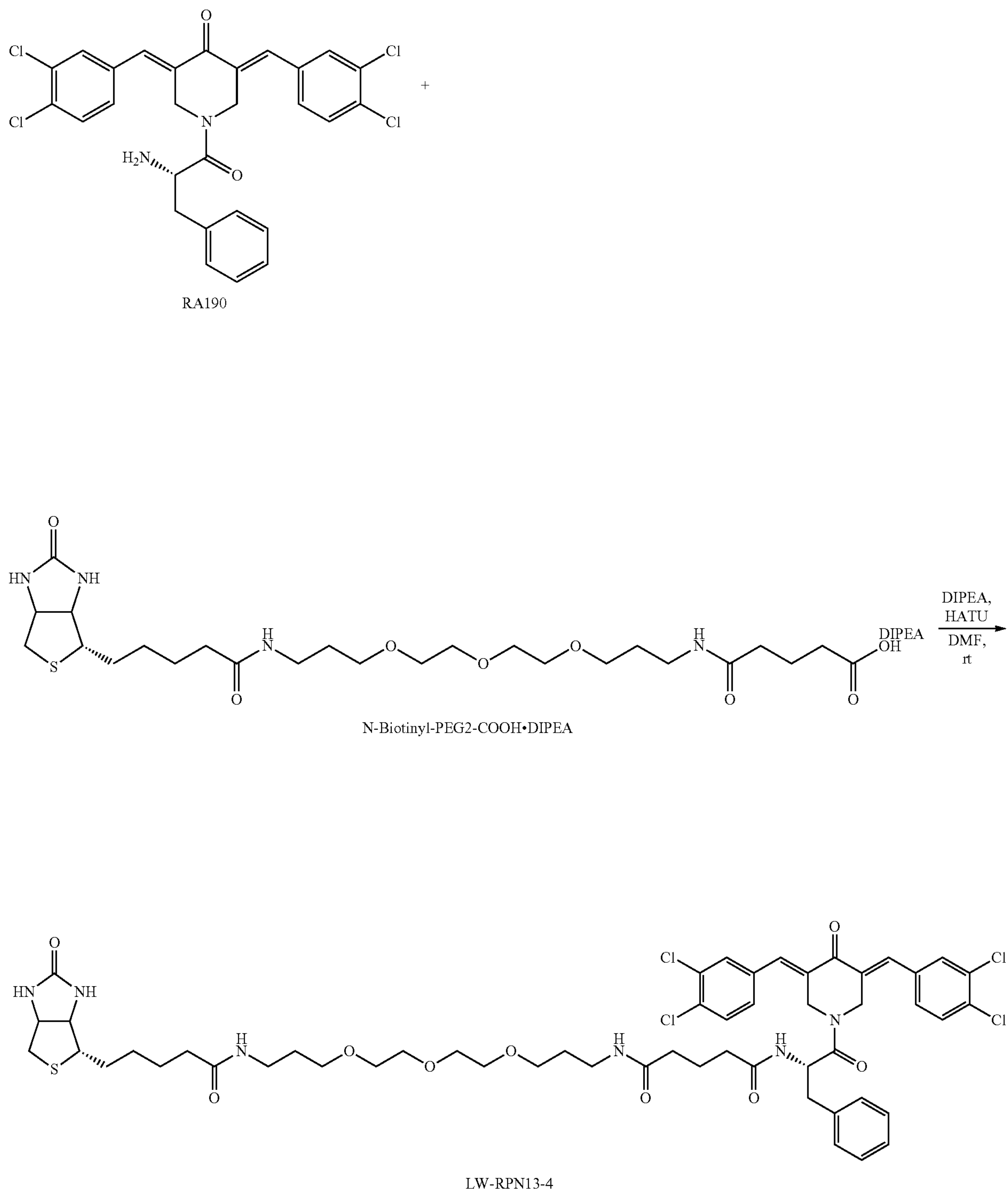
Scheme 1. Exemplary synthesis of LW-RPN13-4
