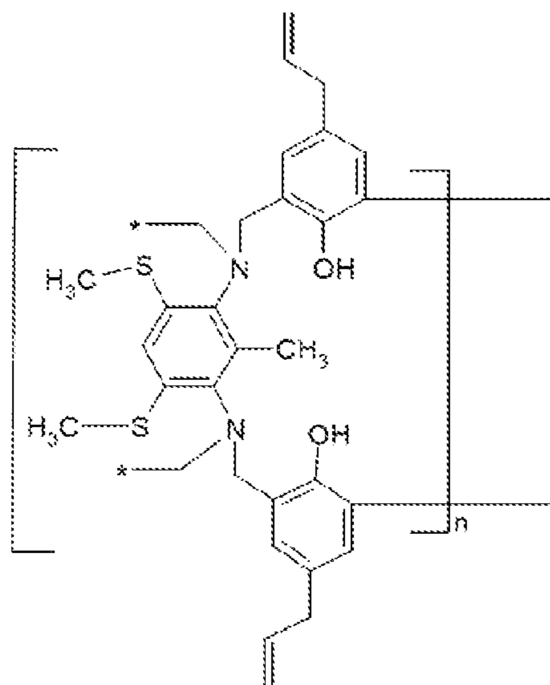
Polymer P-2'
