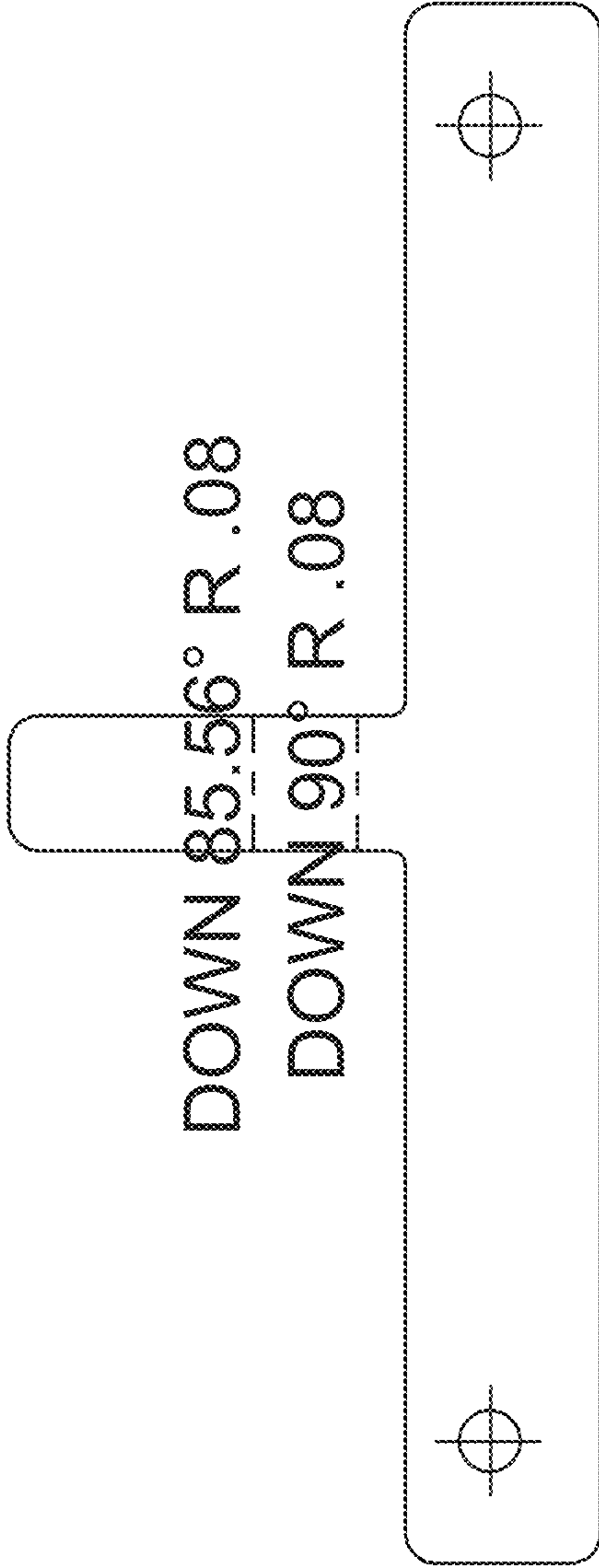
FLAT PATTERN
