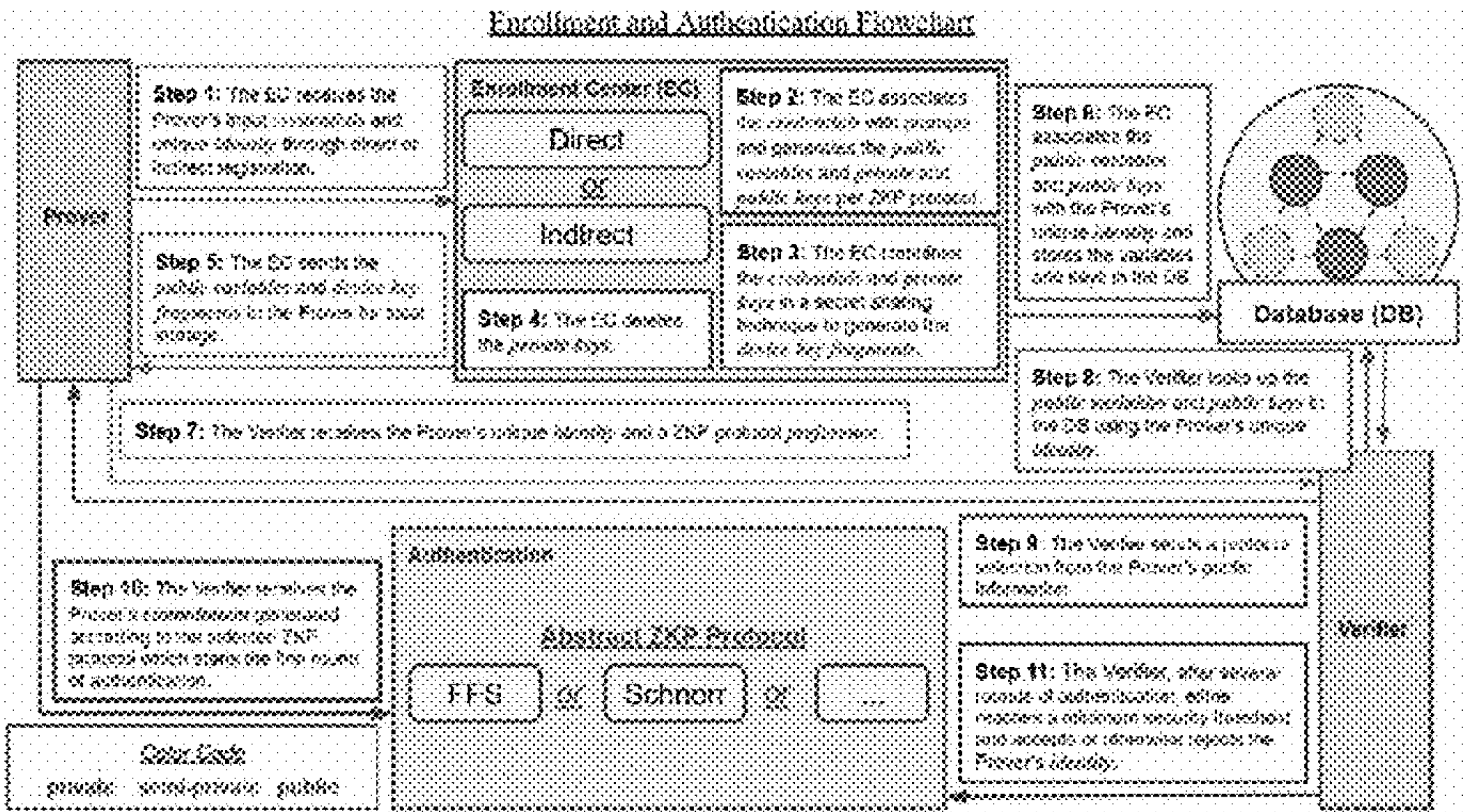
A flowchart of enrollment and authentication process
