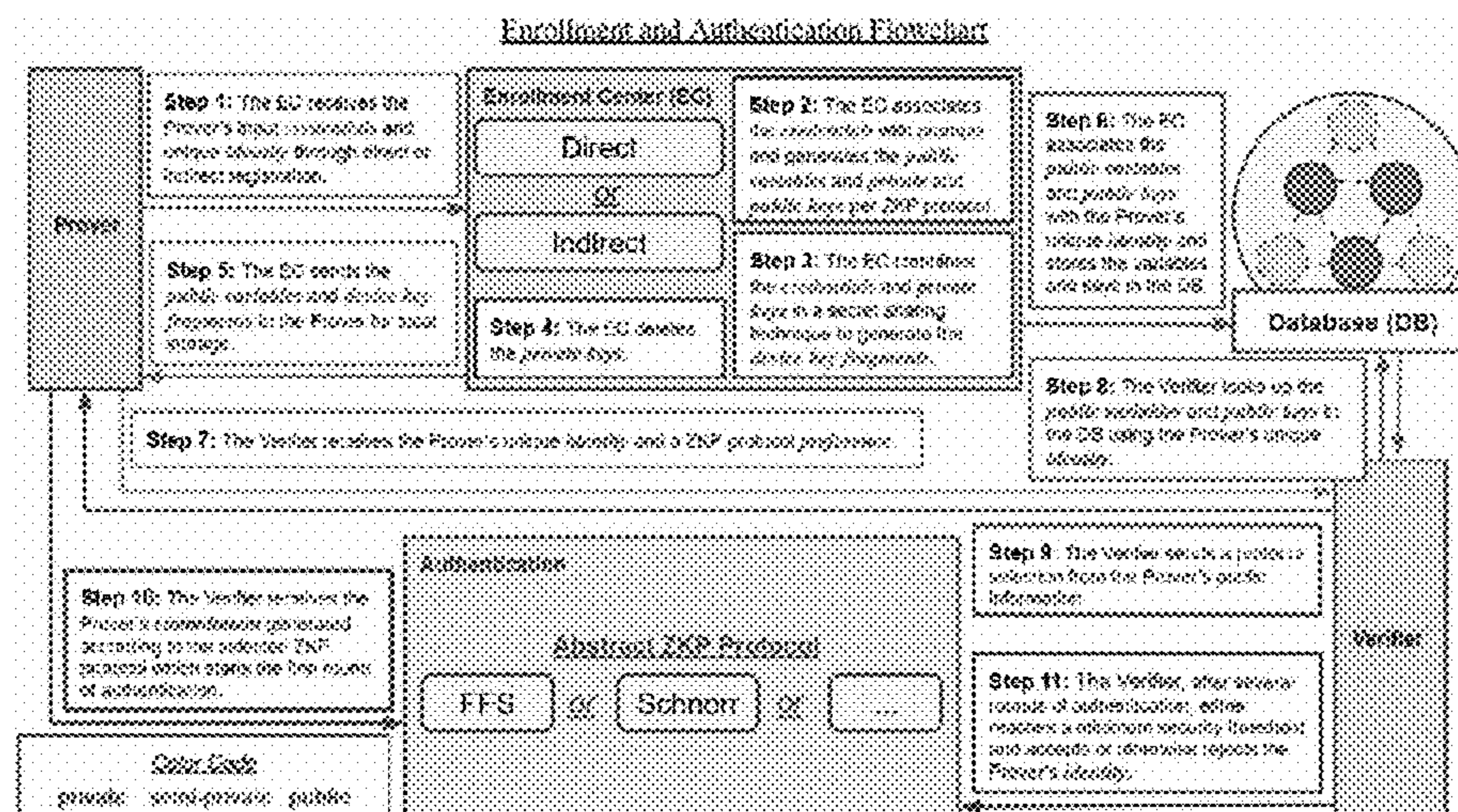
A flowchart of enrollment and authentication process
