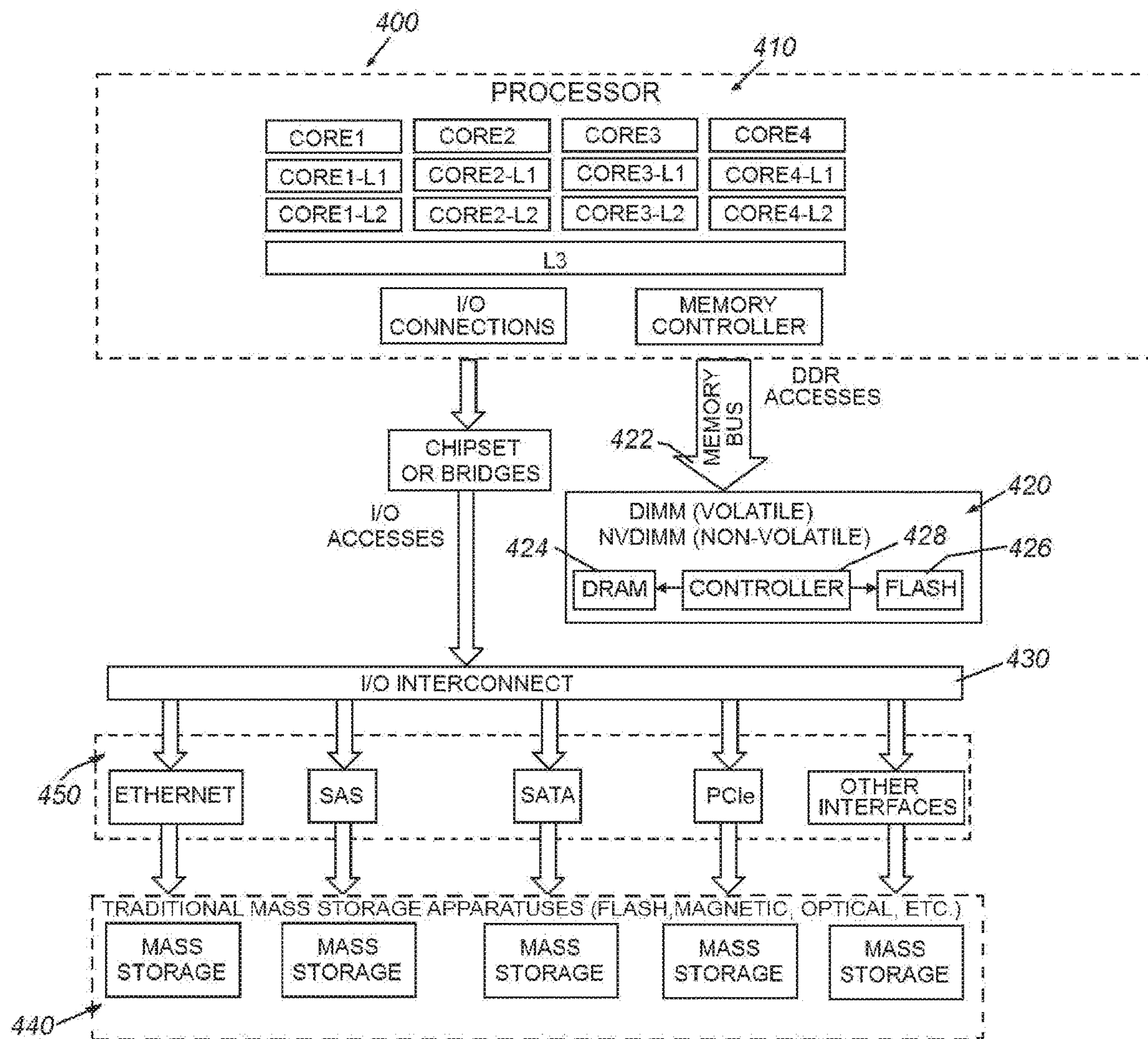
Fig. 4 (Background Art)
