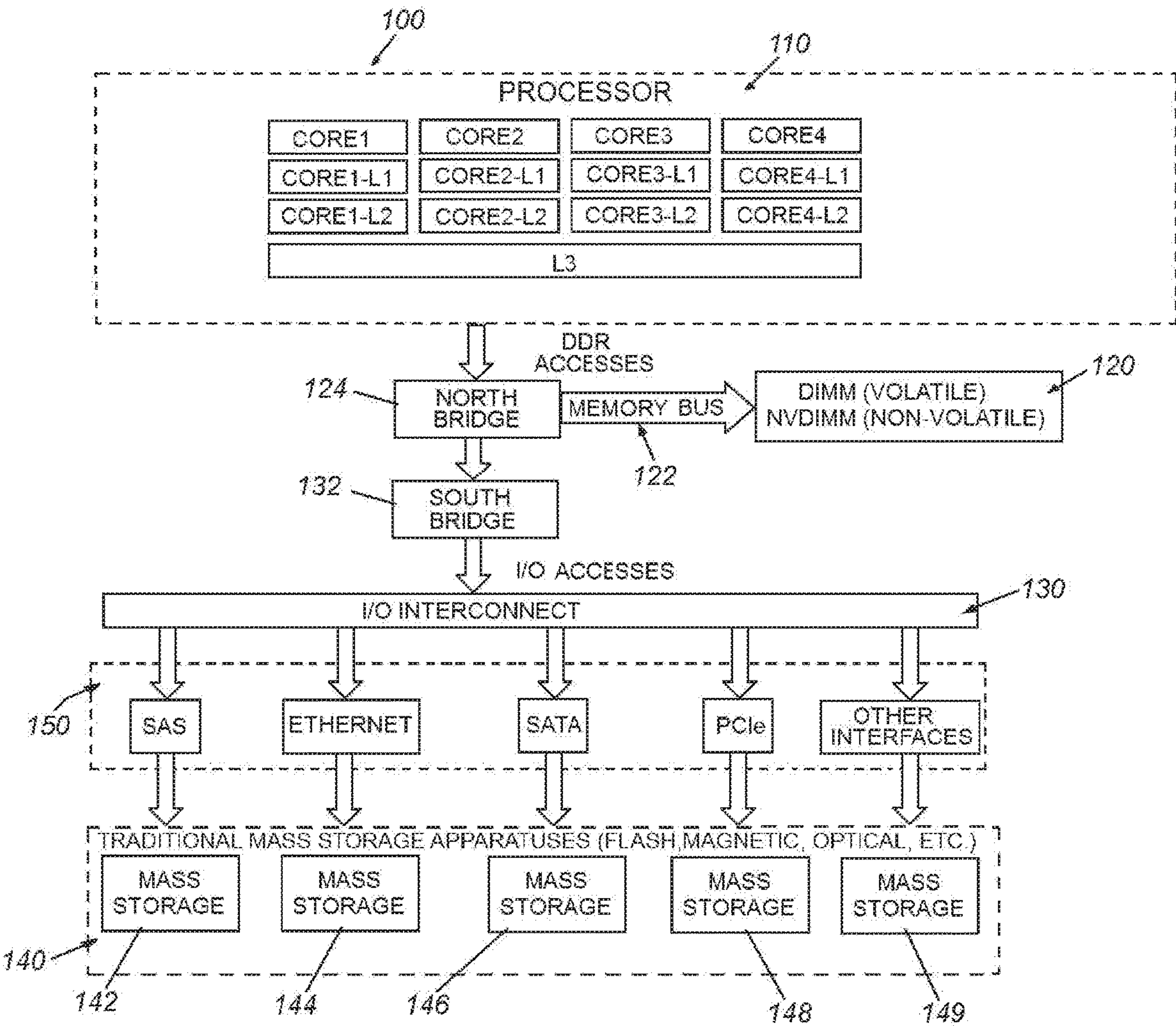
Fig. 1 (Background Art)
