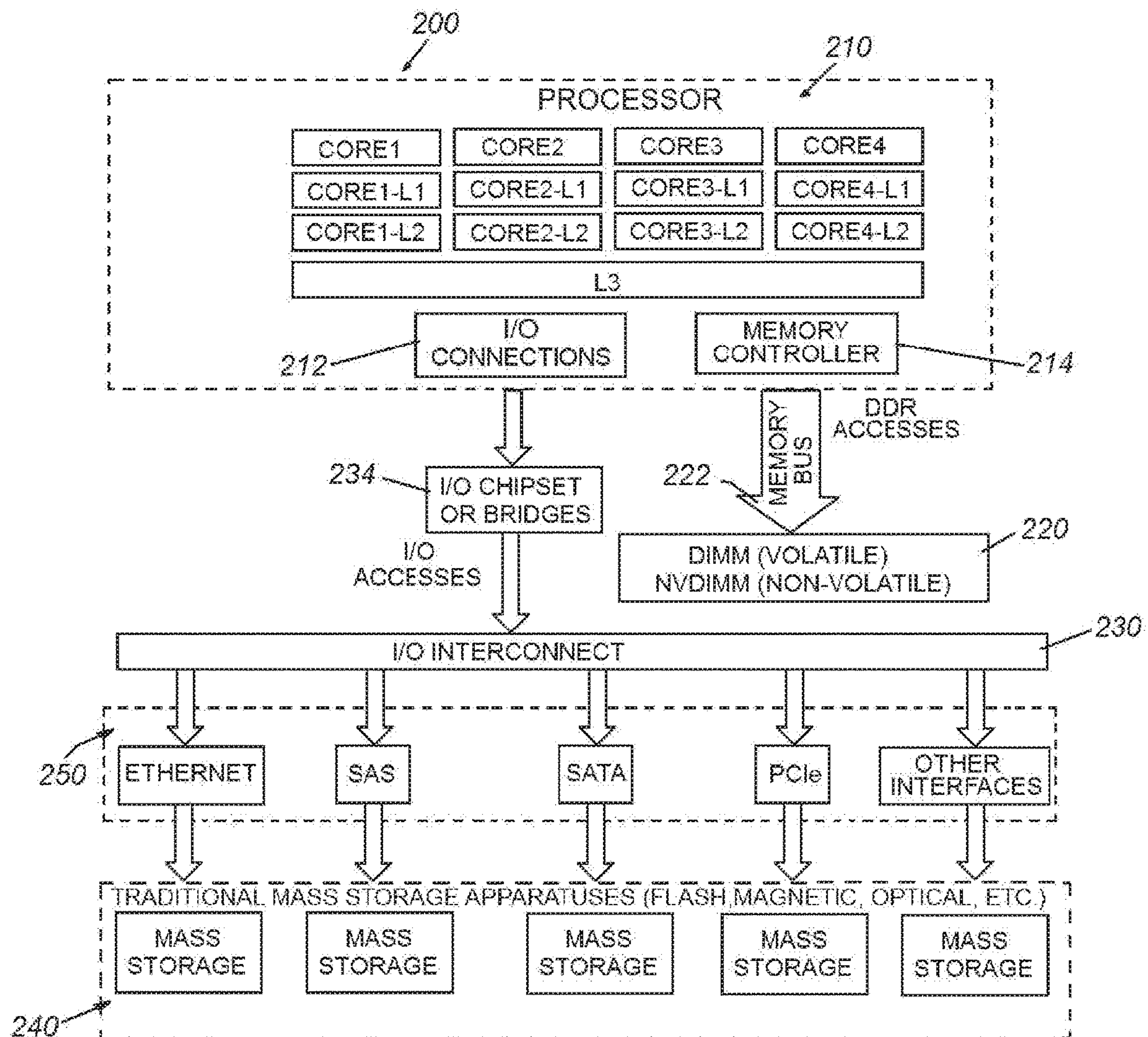
Fig. 2 (Background Art)
