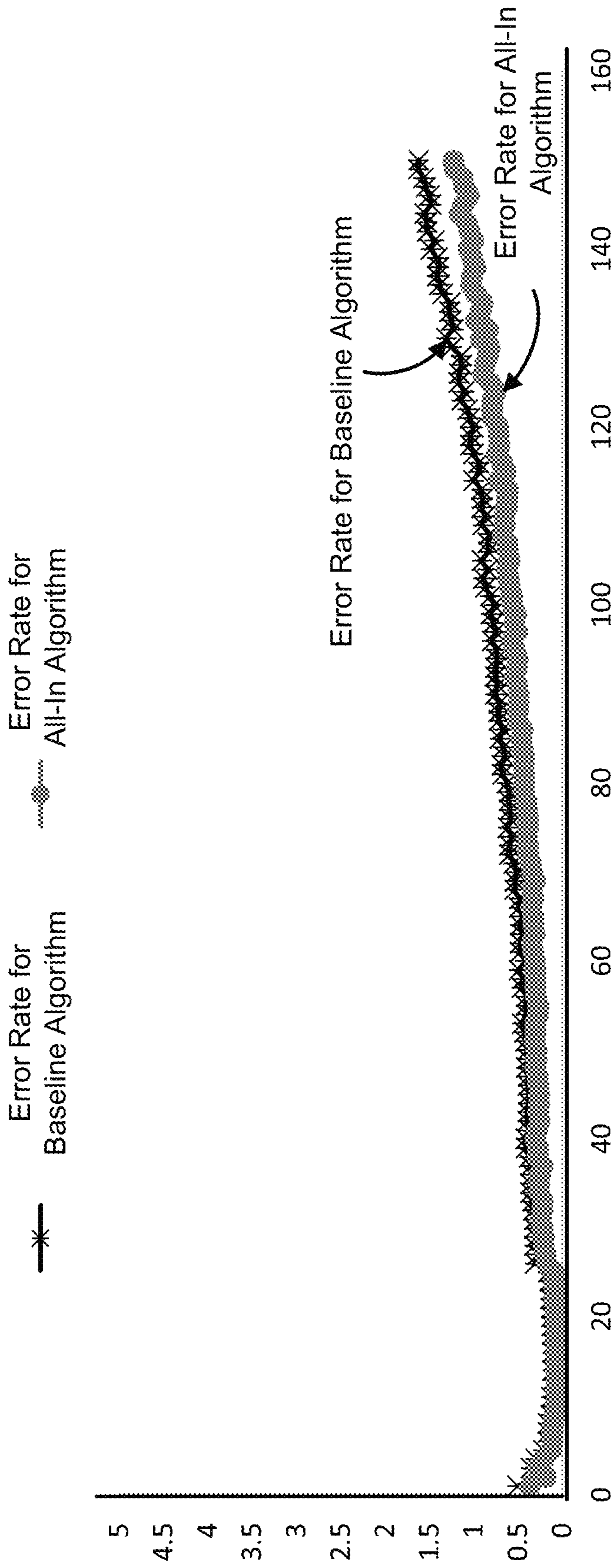
Best Tile Error Rate for Cycles in Sequencing Run A
