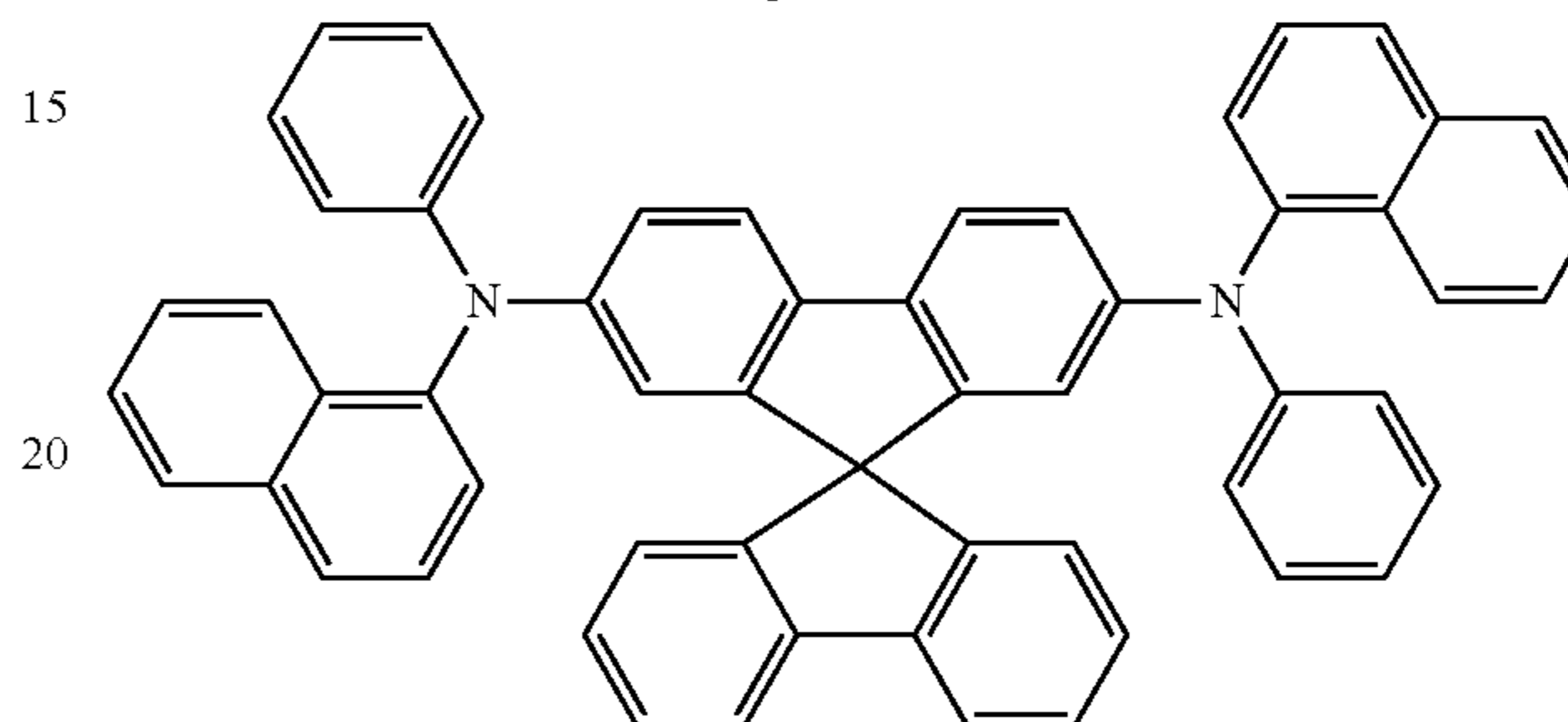
Spiro-NPB
