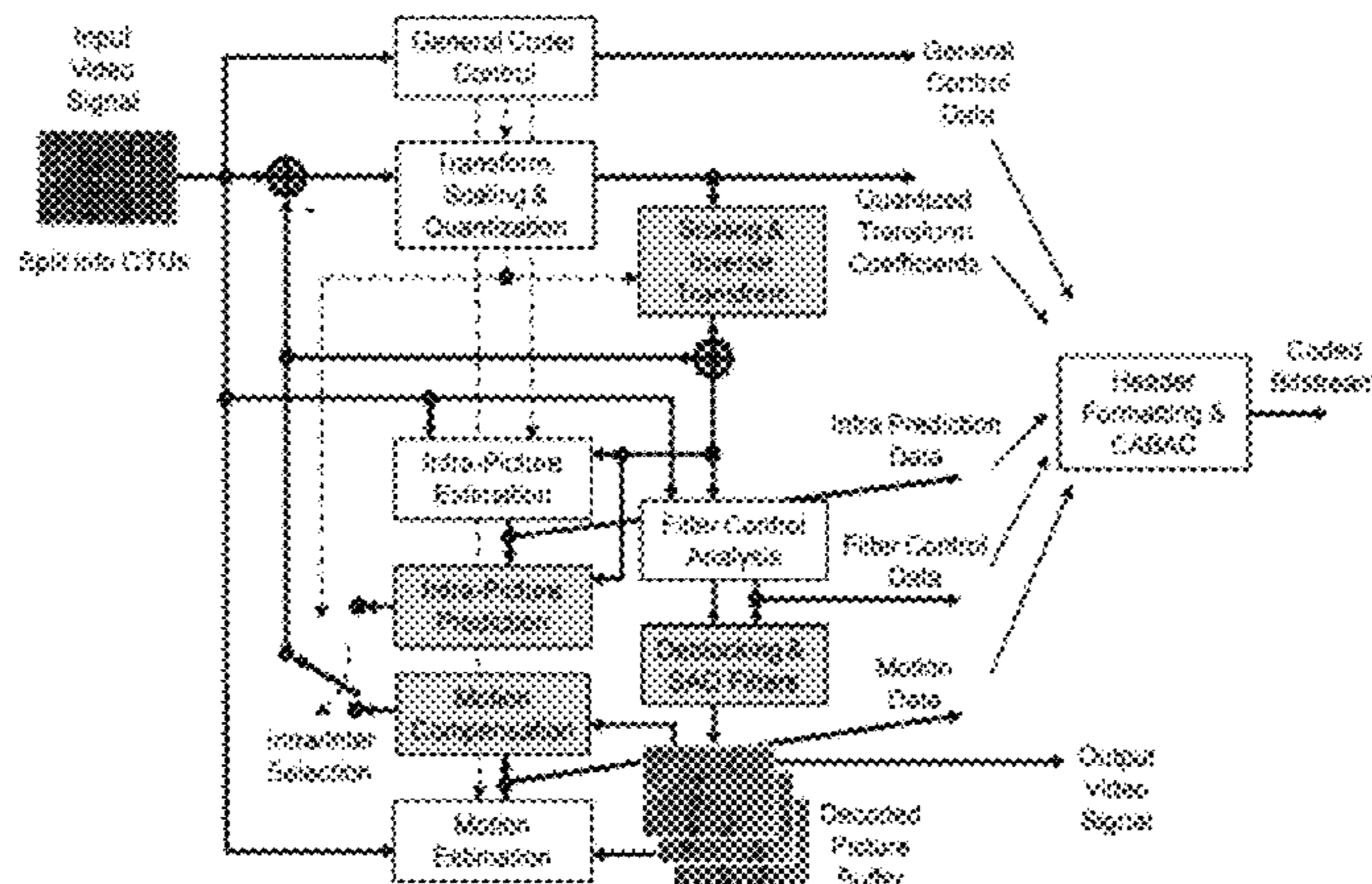
Typical HEVC video encoder (with decoding modeling elements shaded in light gray)
