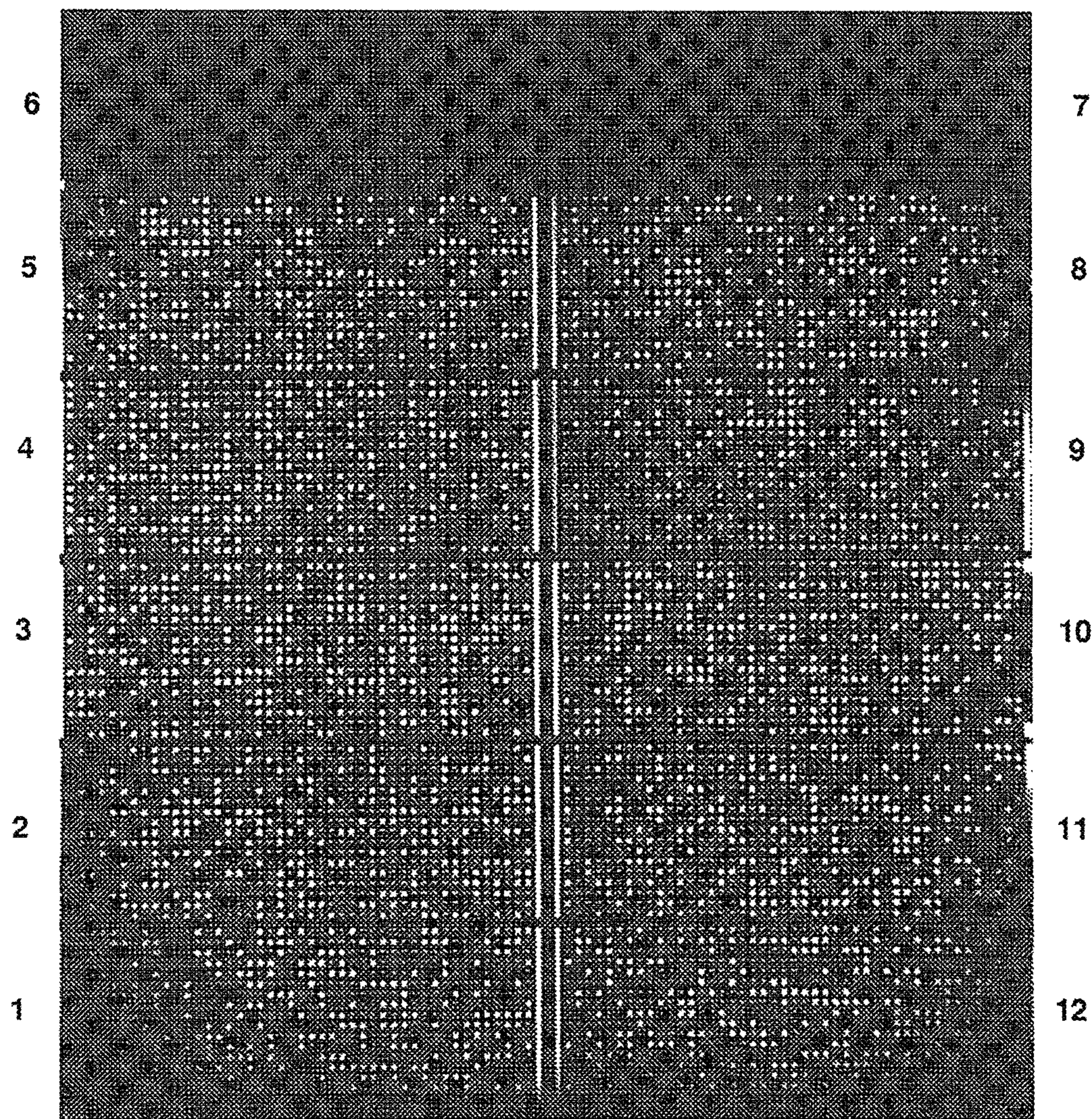
Chr21 FAM
