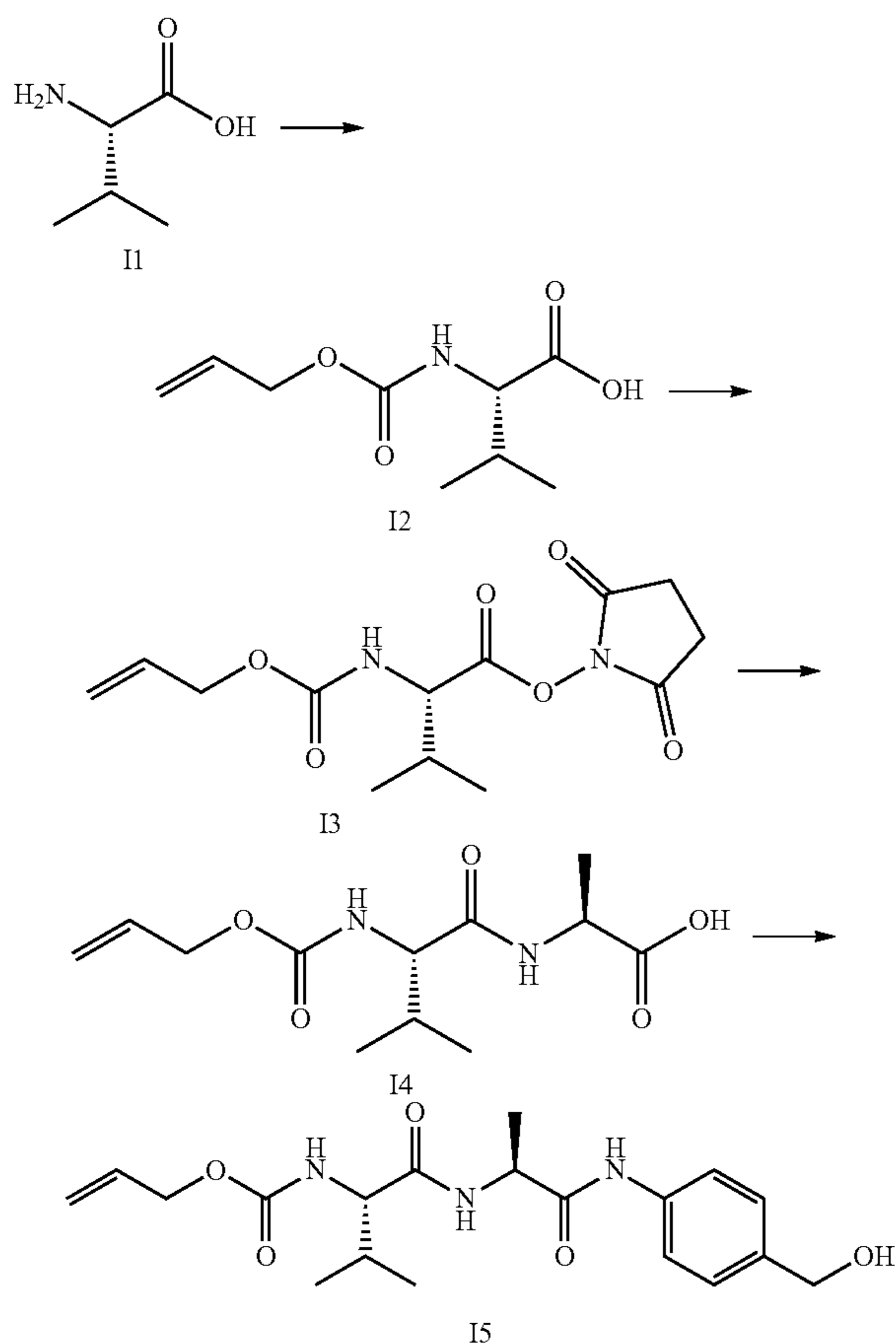
(a-i) (S)-2-(allyloxycarbonylamino)-3-methylbutanoic acid (12)
