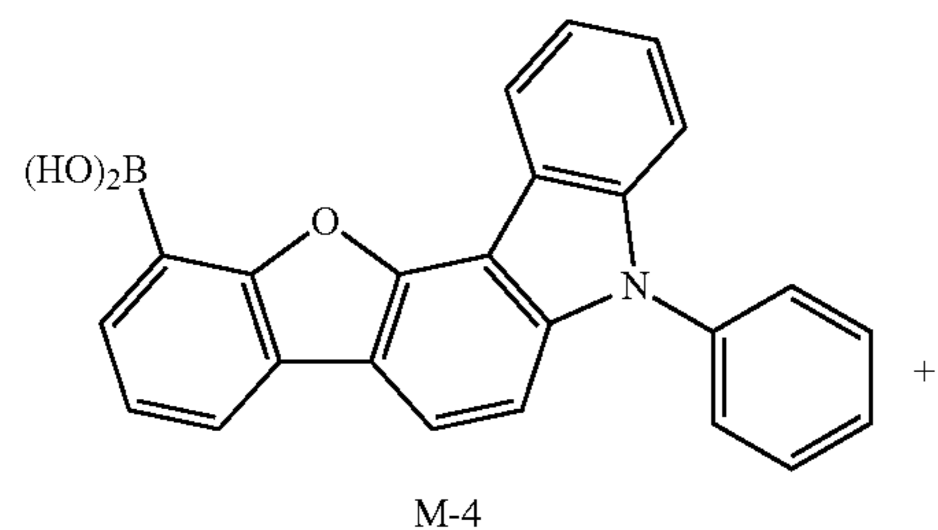
Reaction Scheme 10
