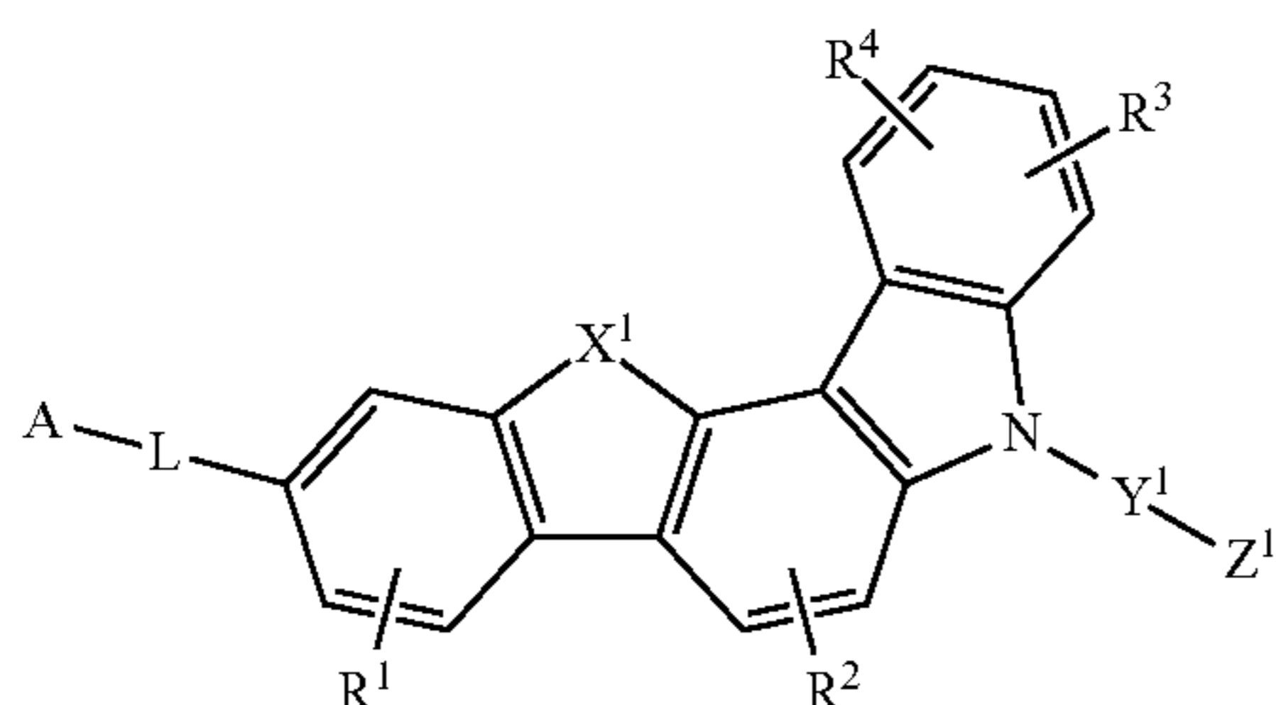
[Chemical Formula 1-3]
