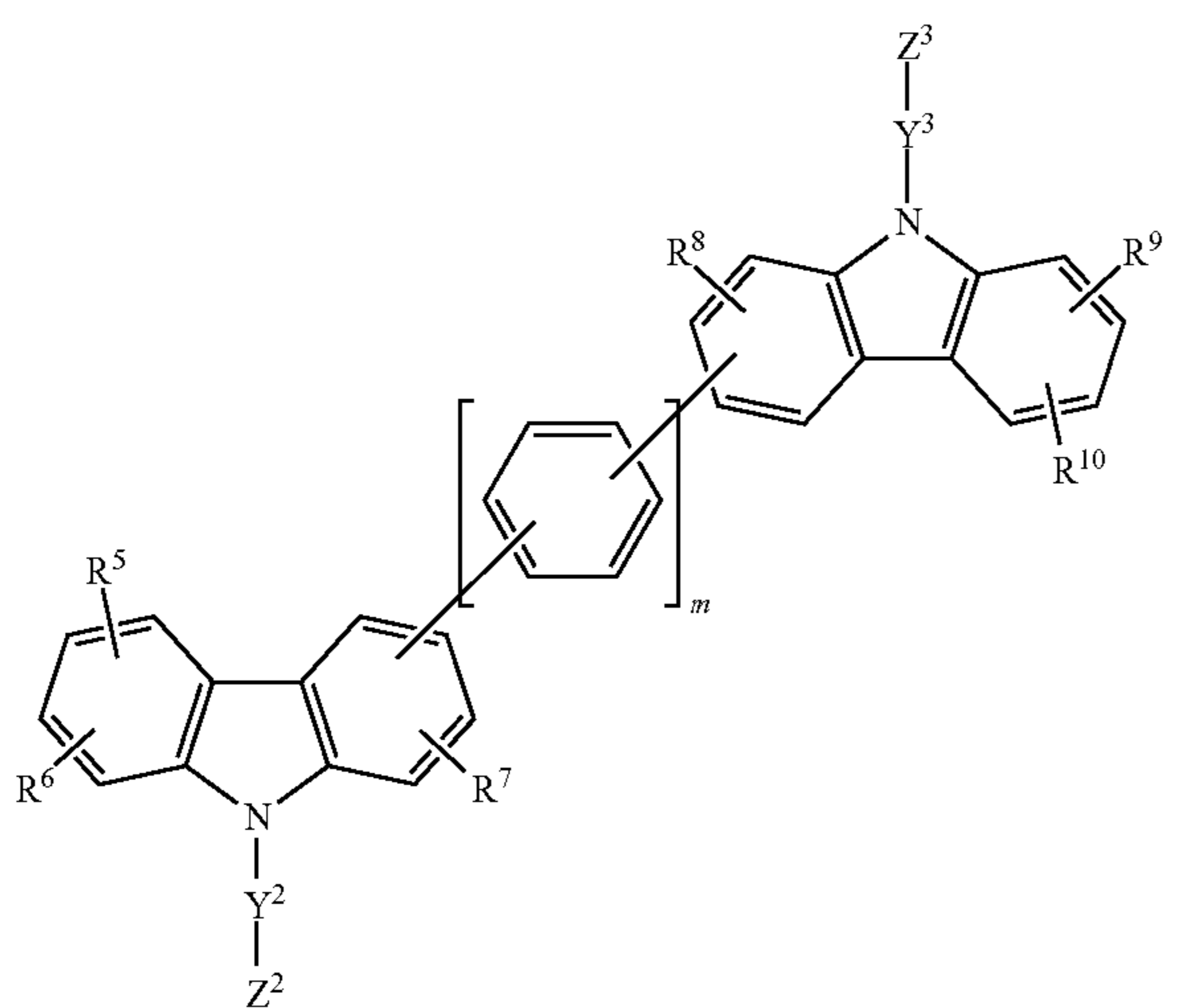
[Chemical Formula 2] 20
