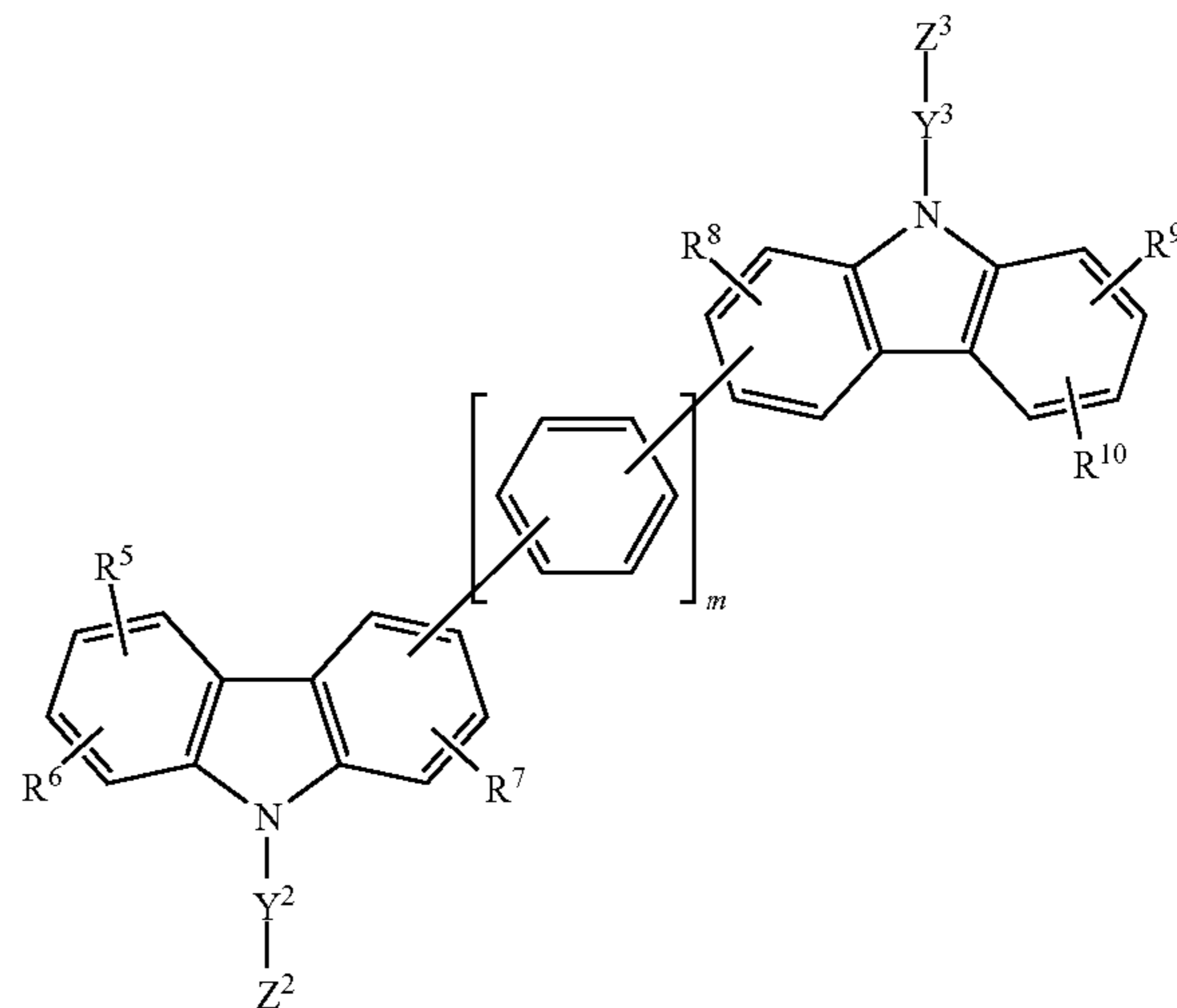
[Chemical Formula 2]
