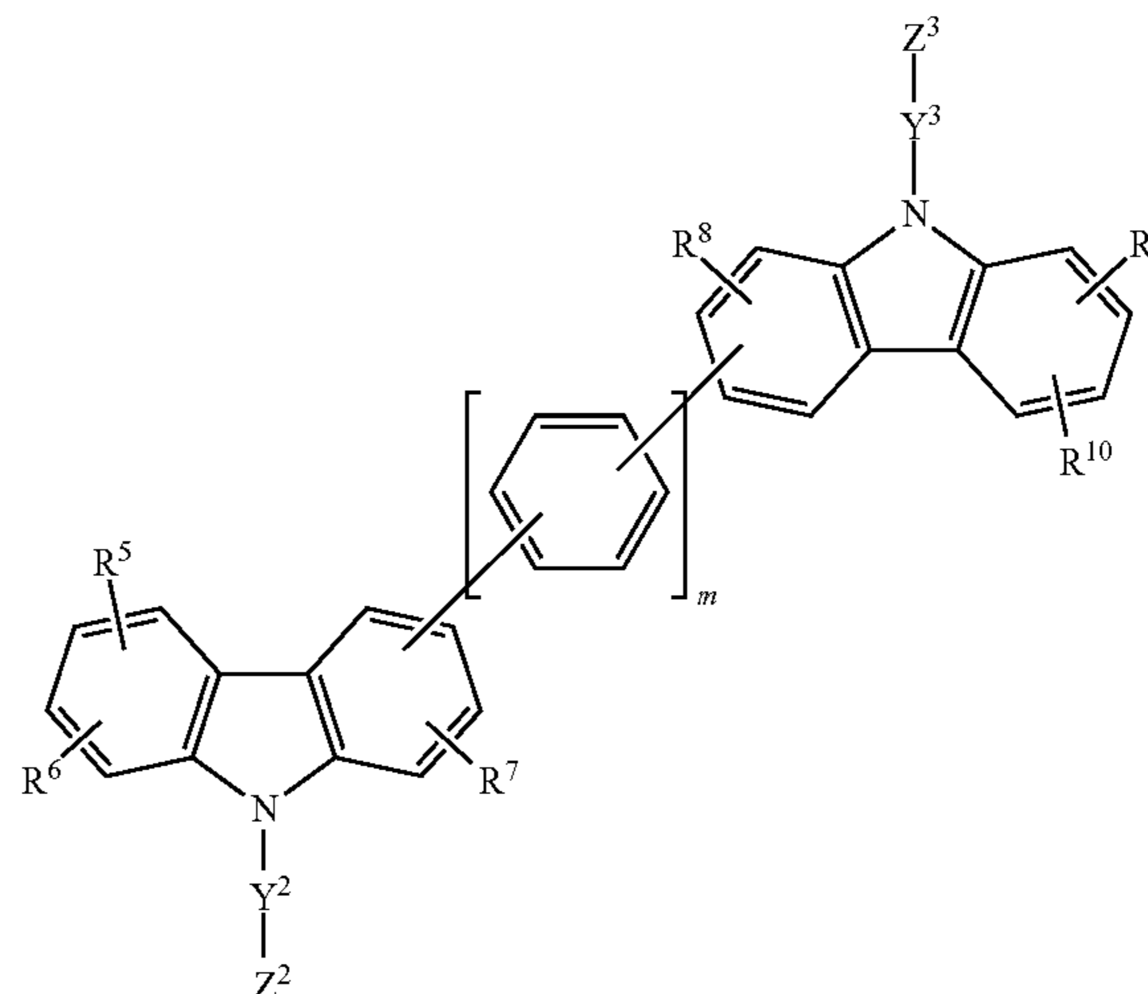
[Chemical Formula 2]
