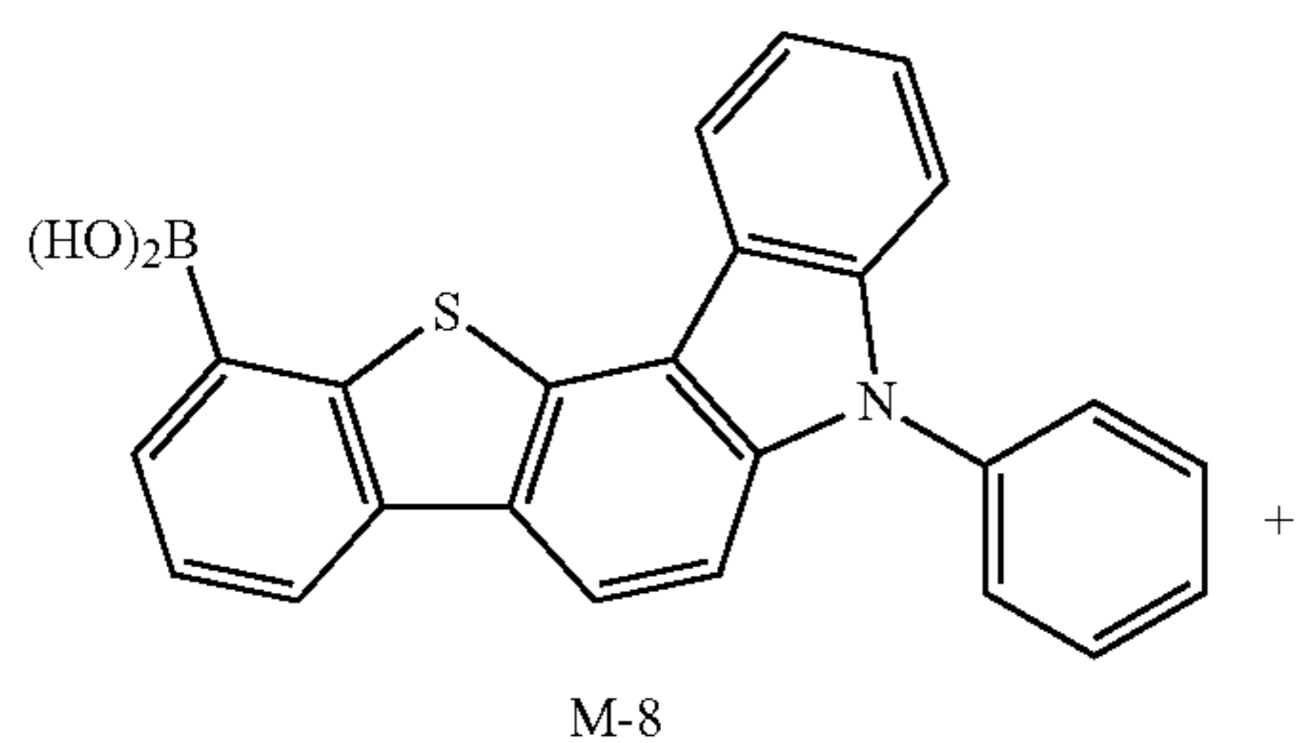
Reaction Scheme 14
