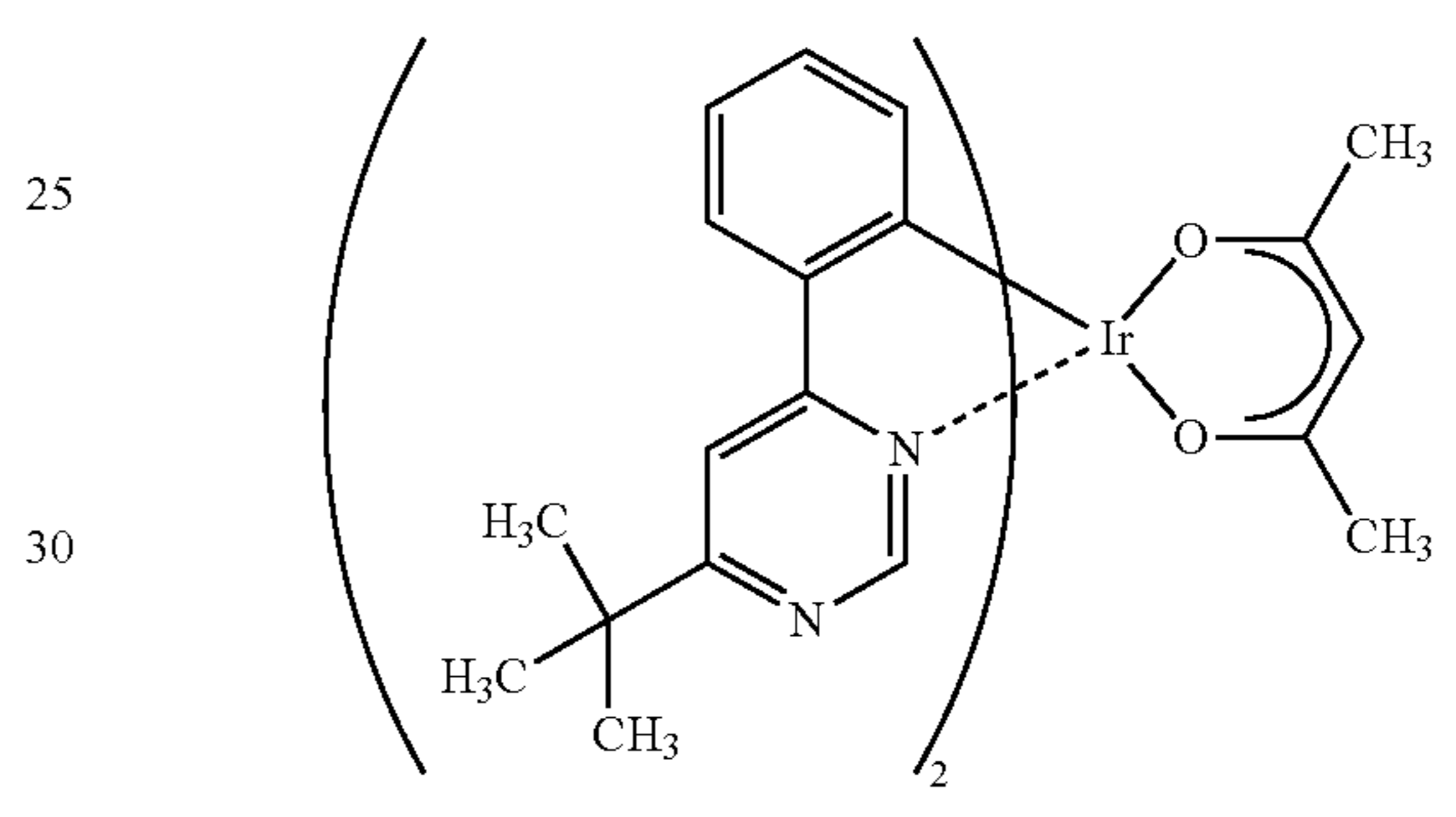
(xi) [Ir(tBuppm) 2 (acac)]
