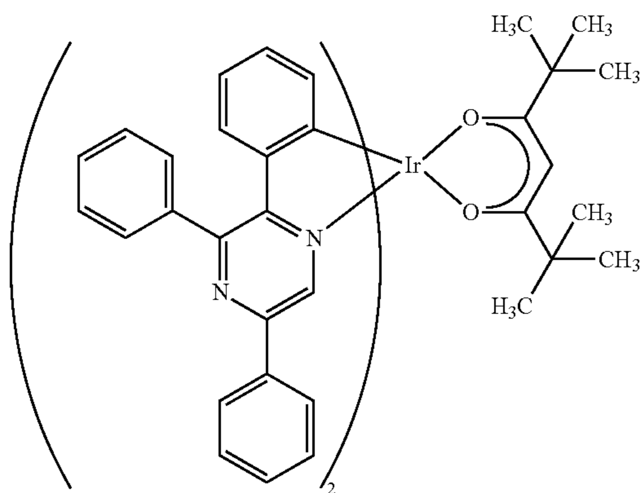
(v) [Ir(tppr) 2 (dpm)]
