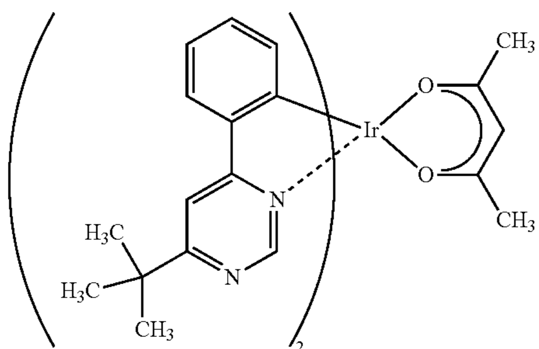
(xi) [Ir(tBuppm) 2 (acac)]
