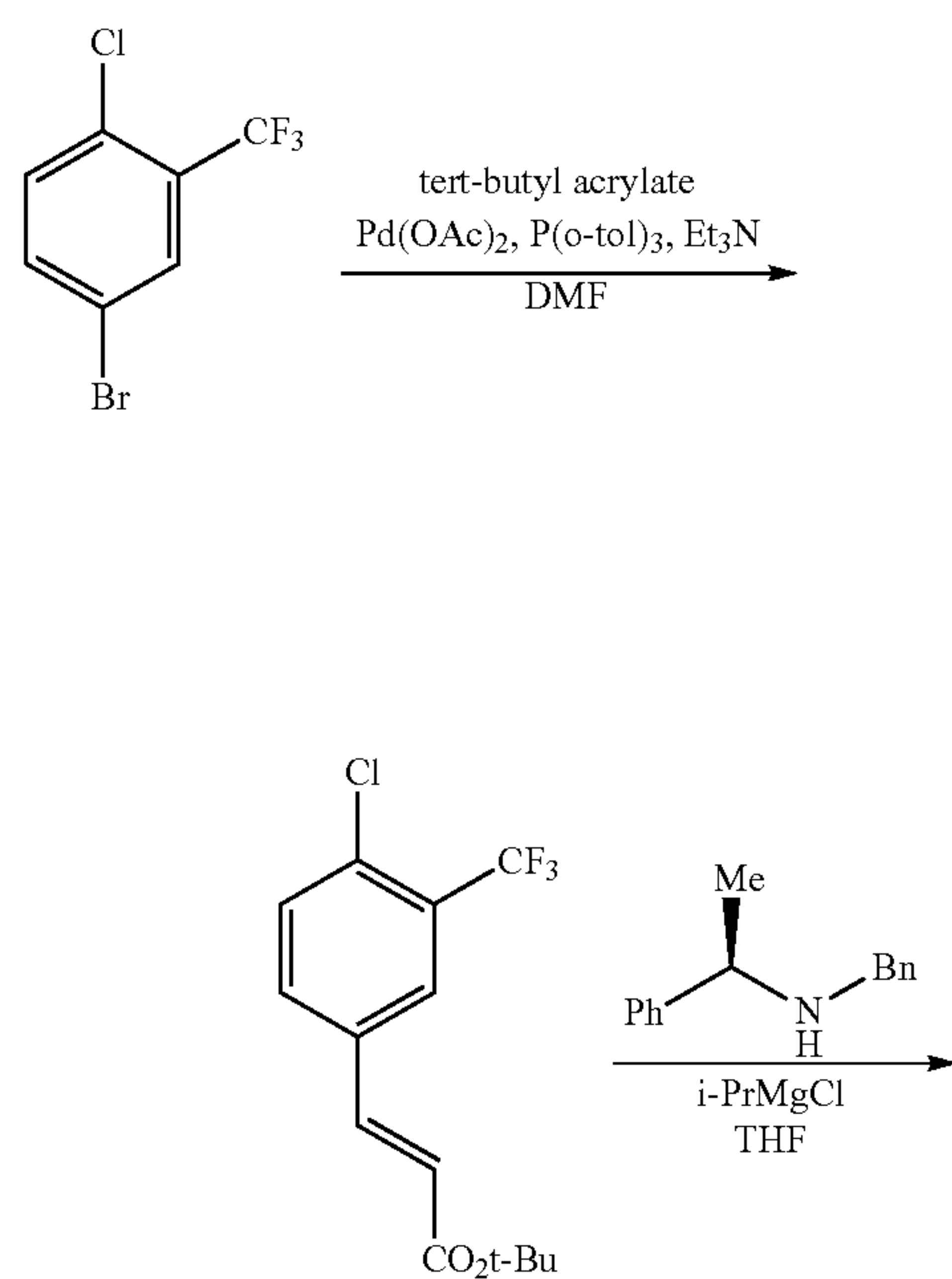
Scheme 4
