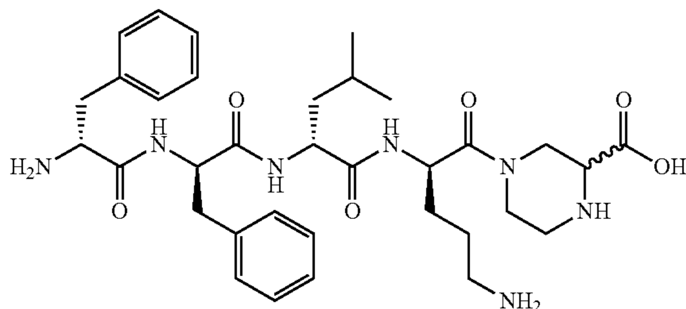
Compound (45)
