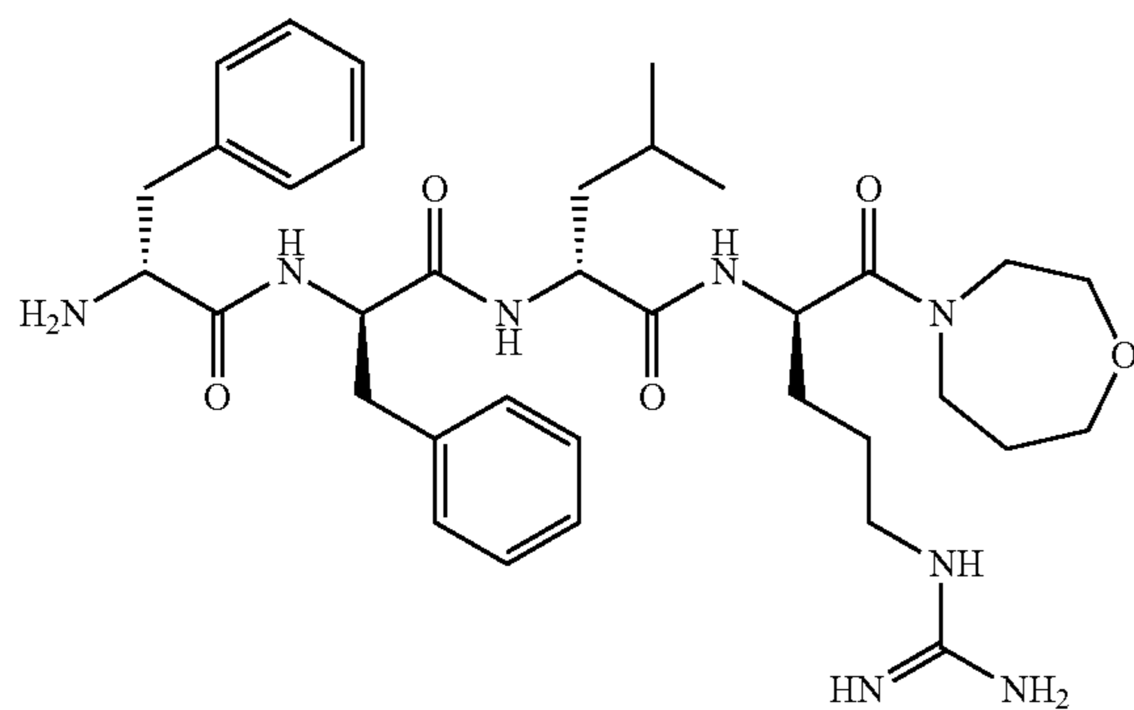
Compound (98)
