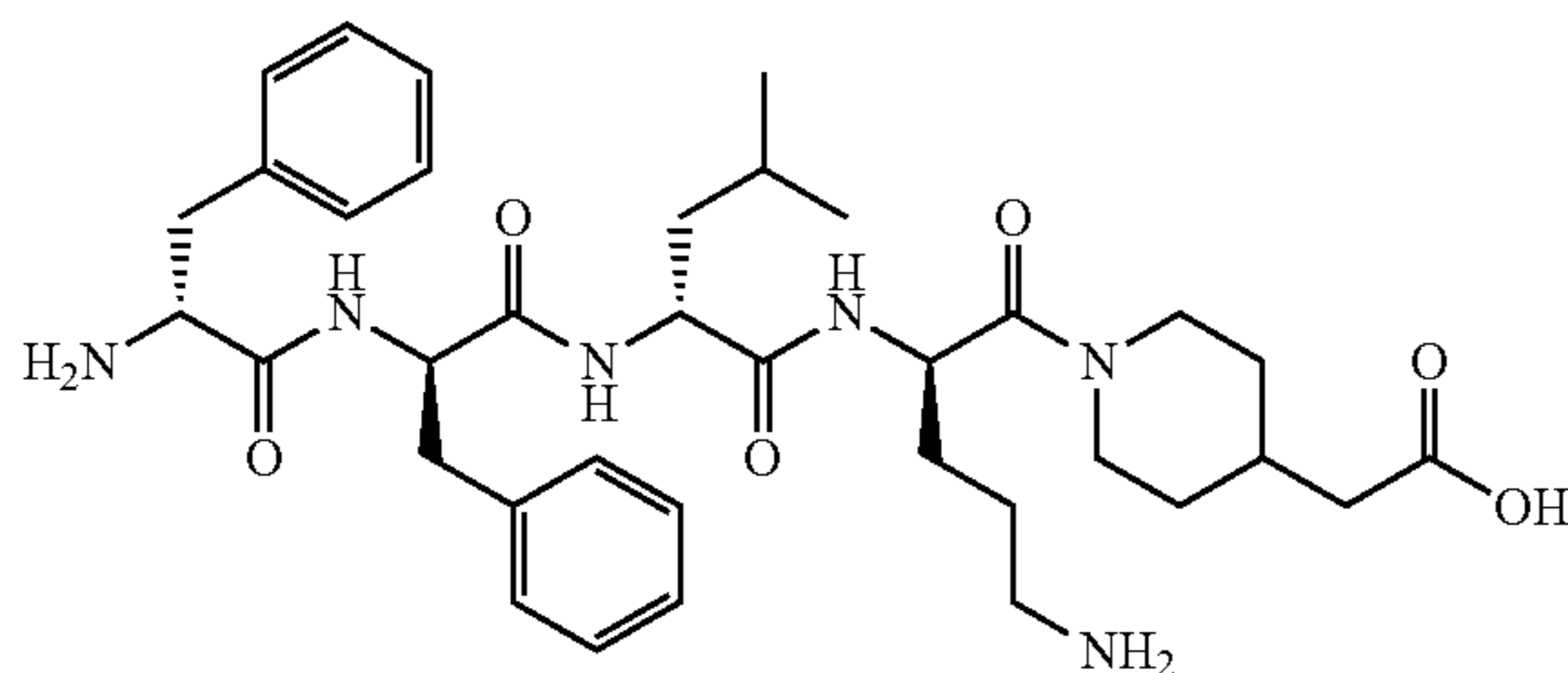
Compound (39)
