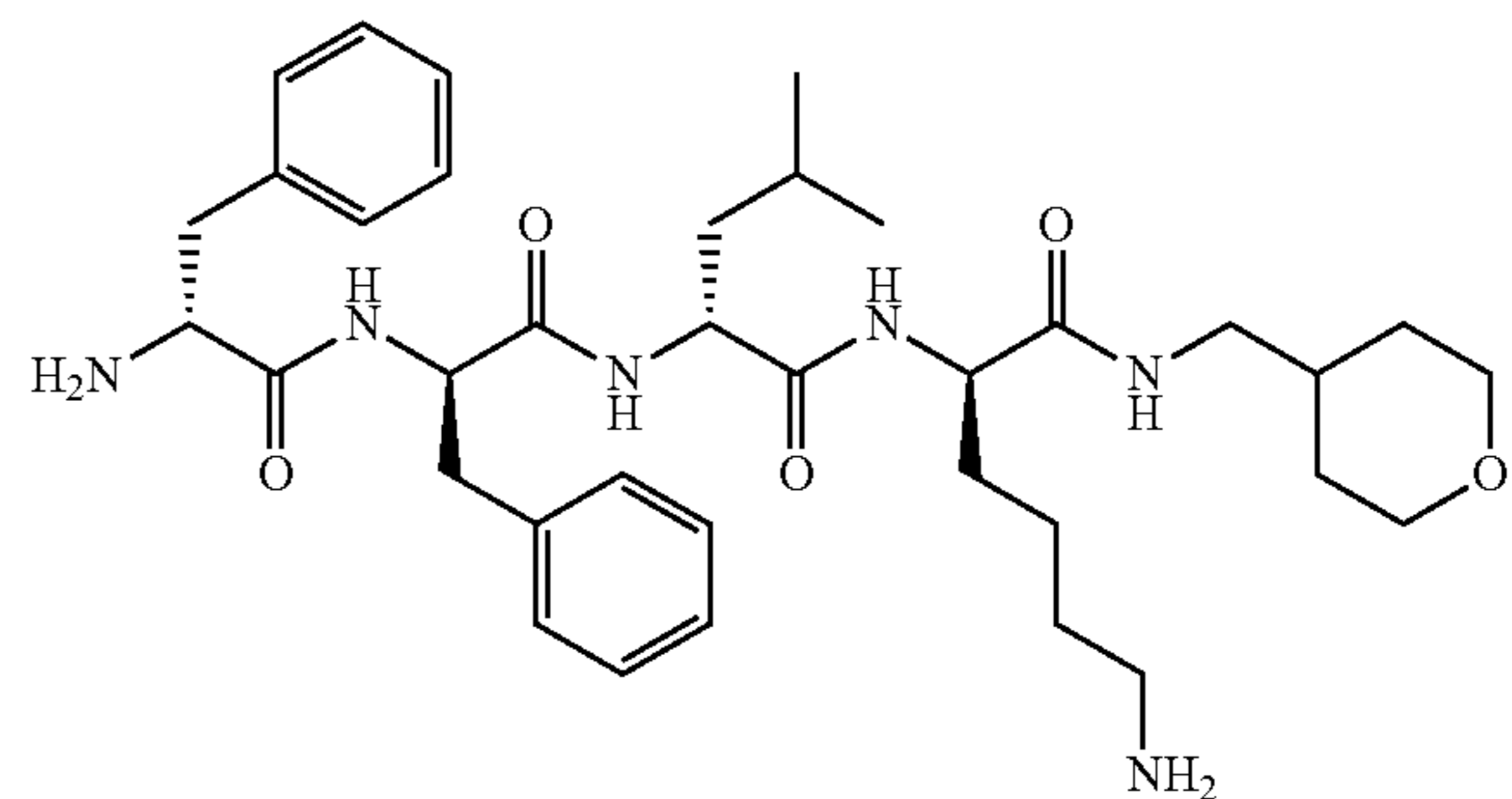
Compound (73)
