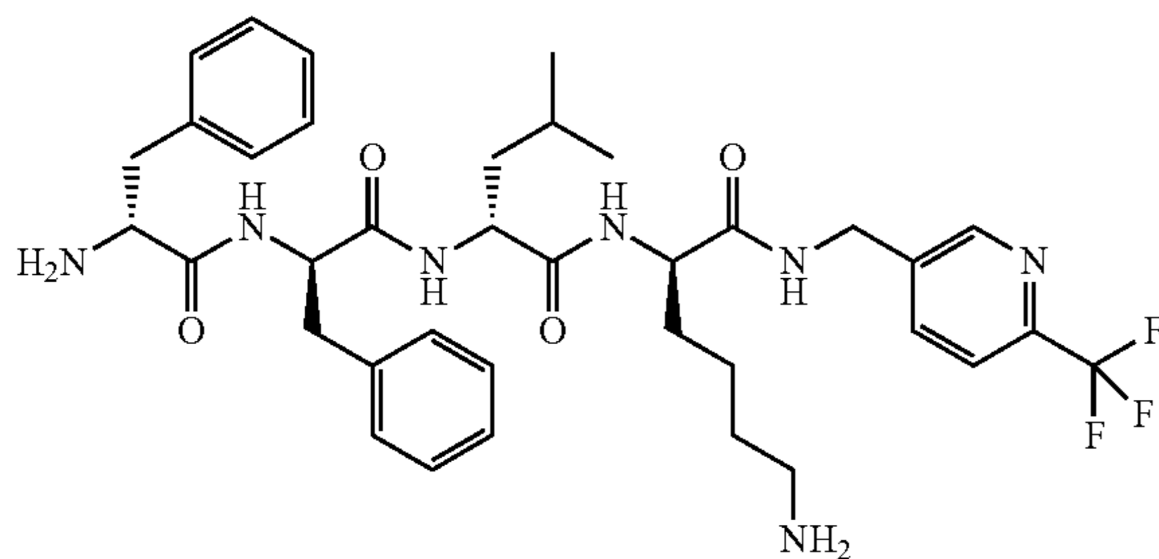
Compound (72)
