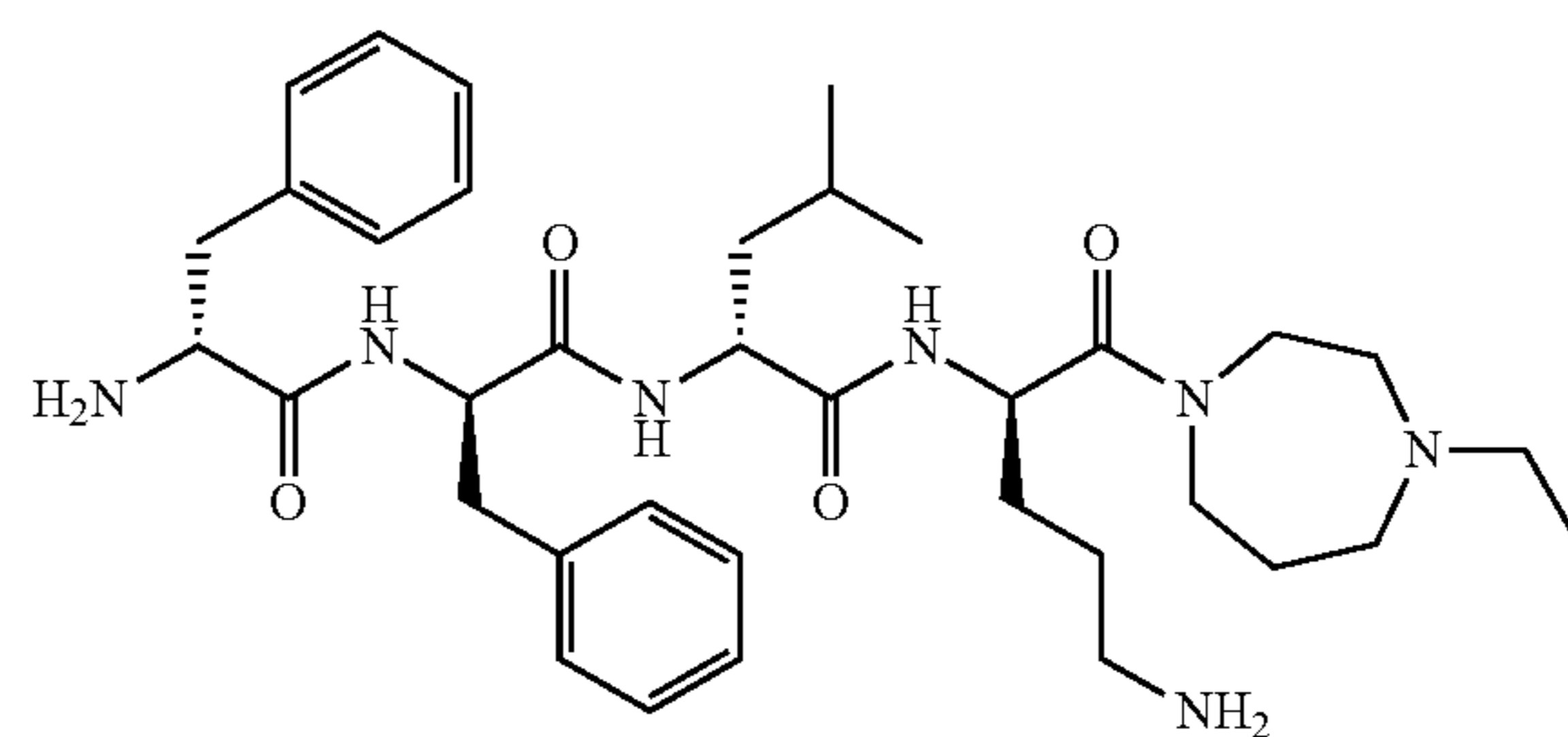
Compound (55)
