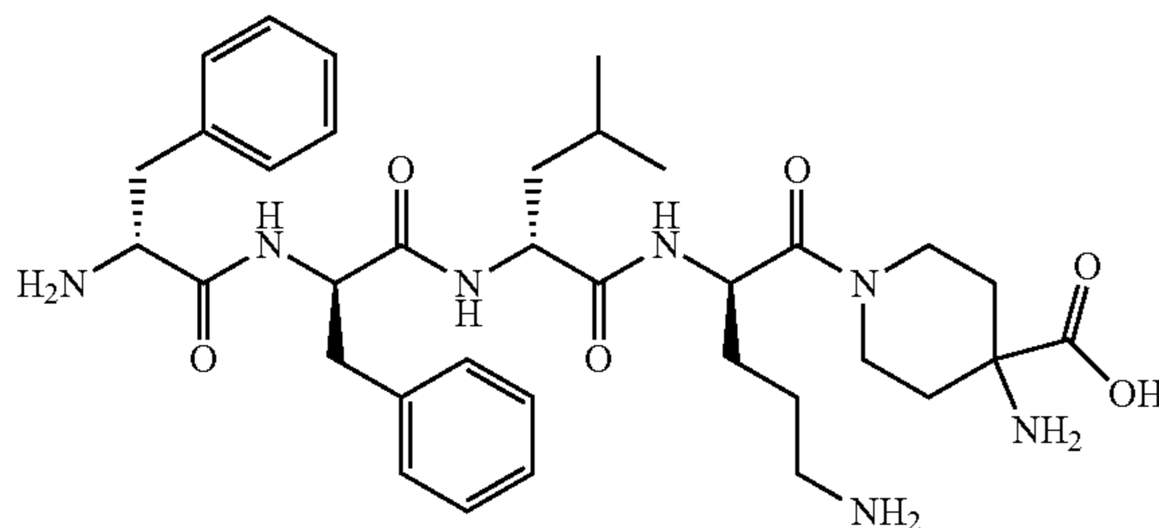
Compound (43)
