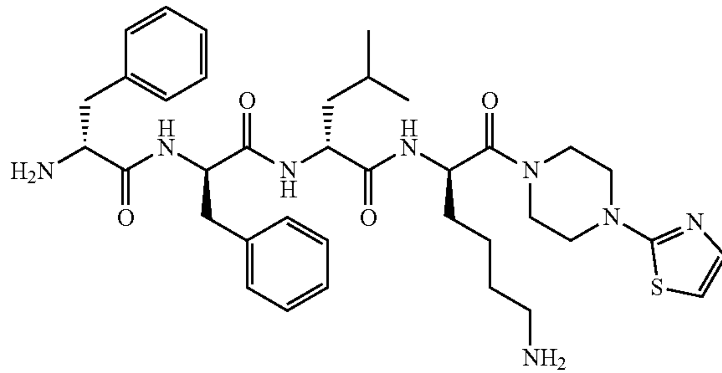
Compound (66)
