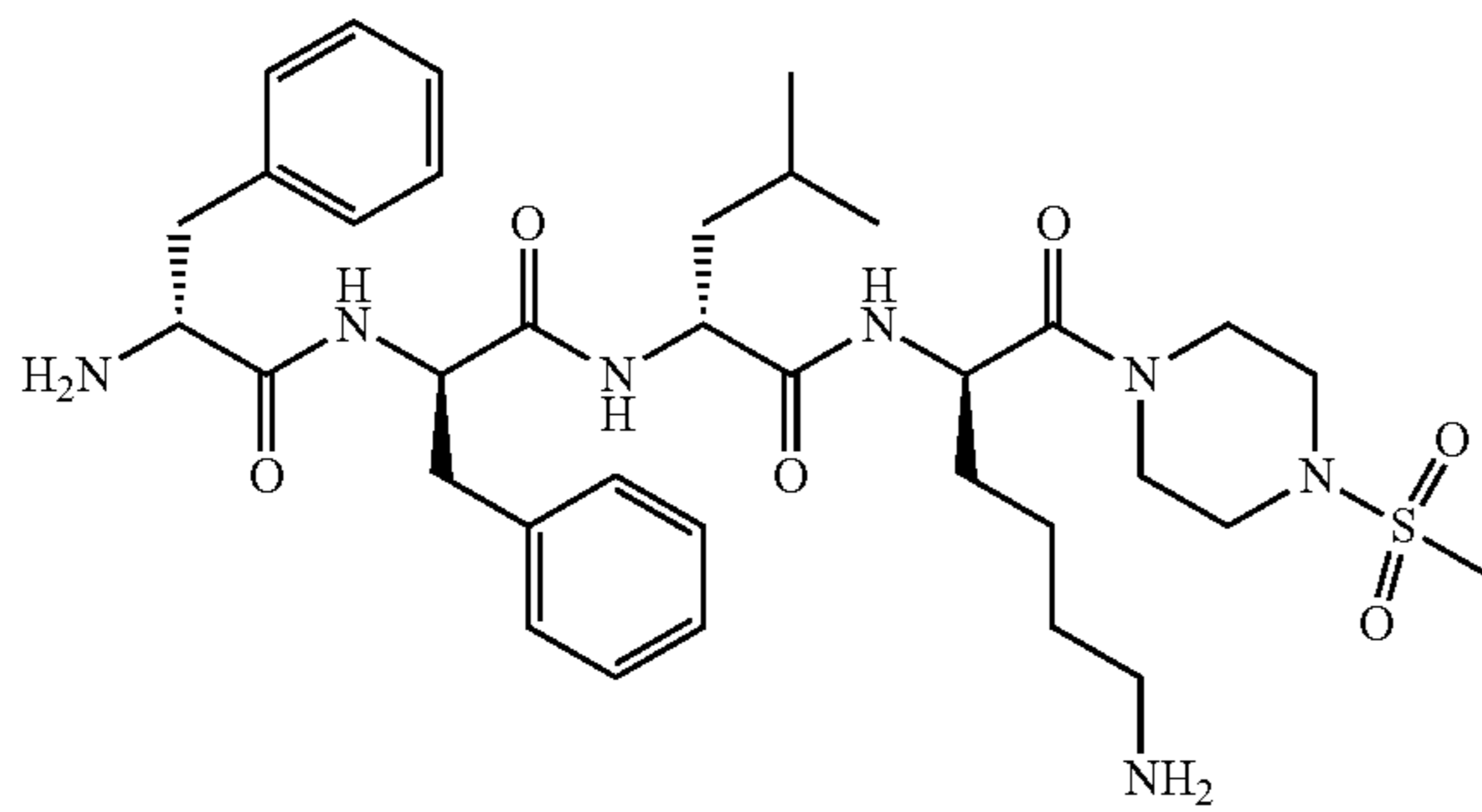
Compound (68)
