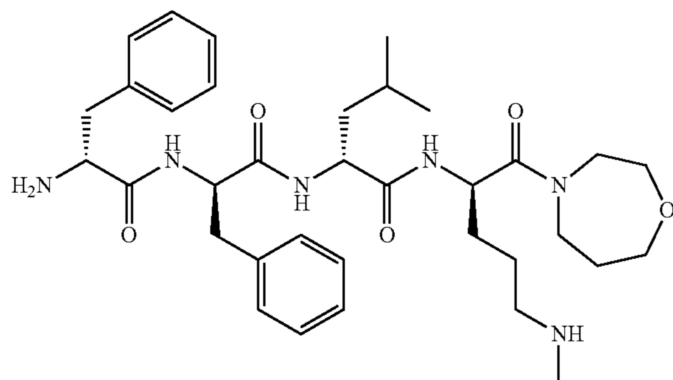
Compound (100)
