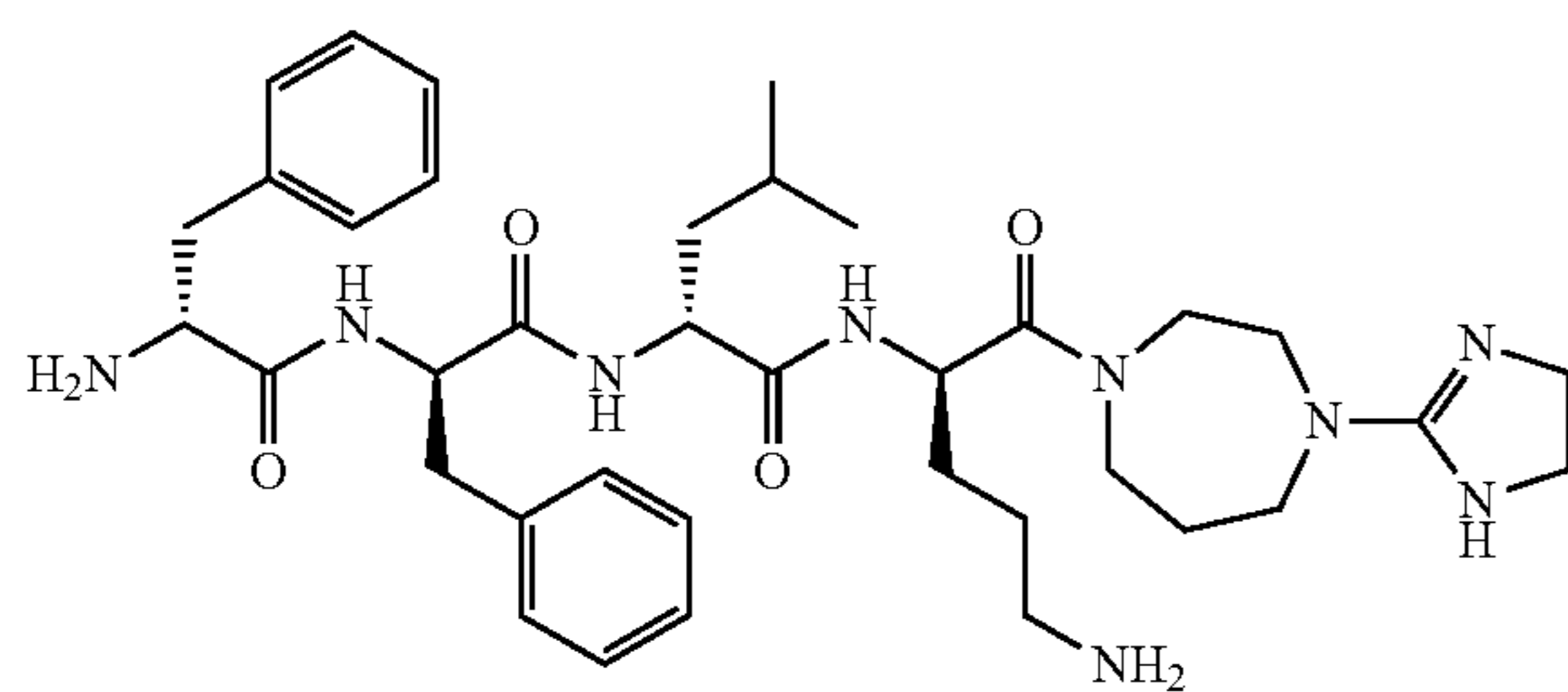
Compound (54)
