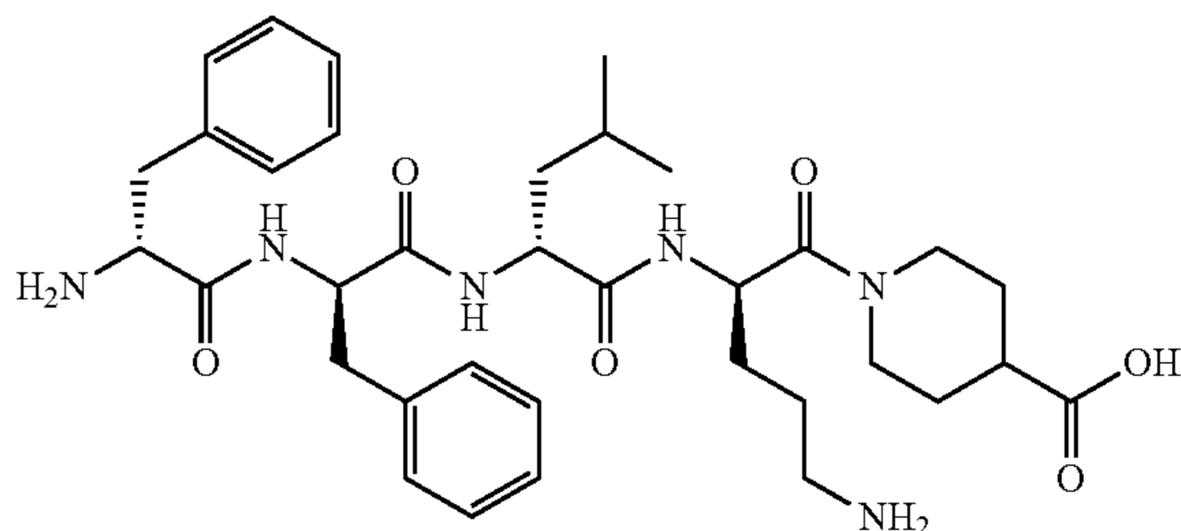
Compound (46)
