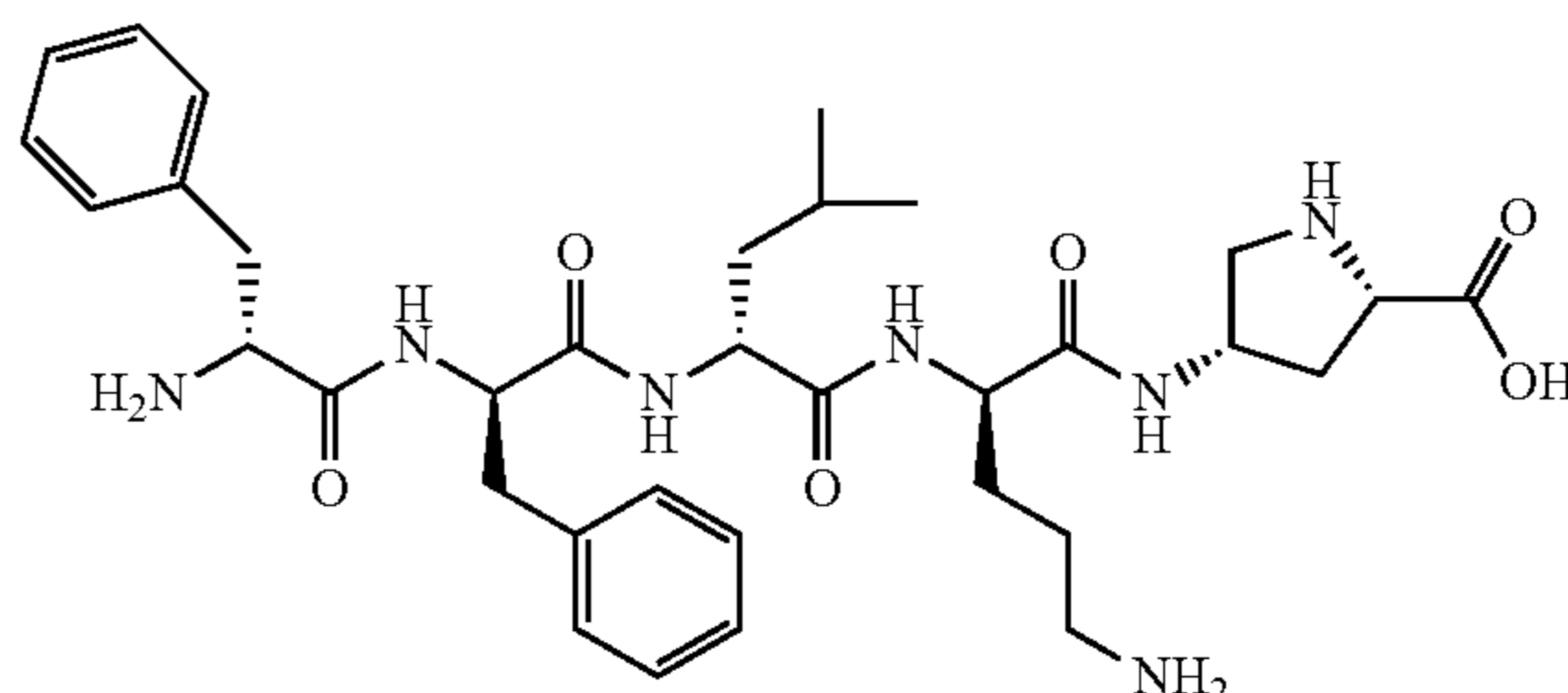
Compound (42)
