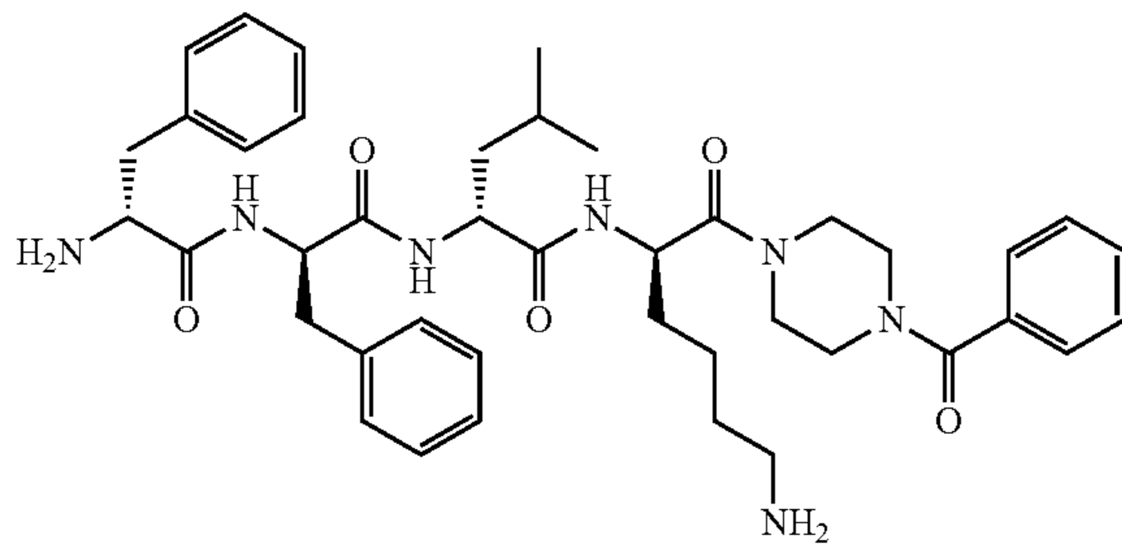
Compound (70)
