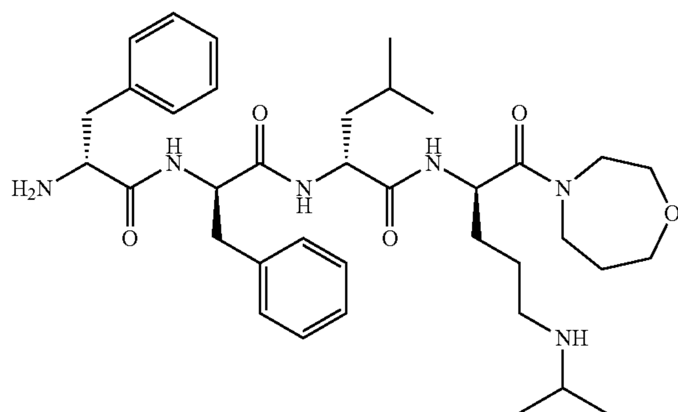
Compound (102)
