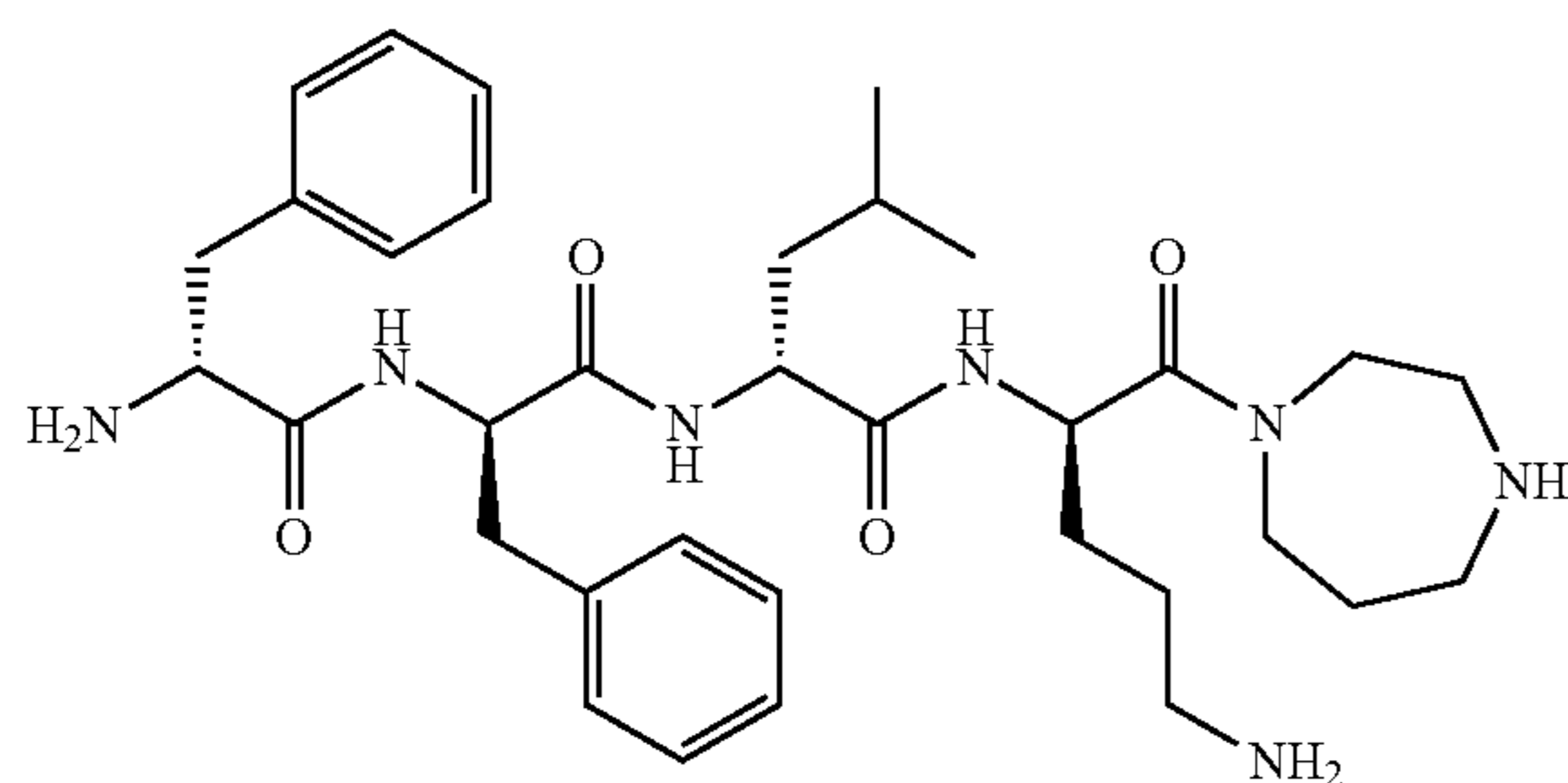
Compound (56)
