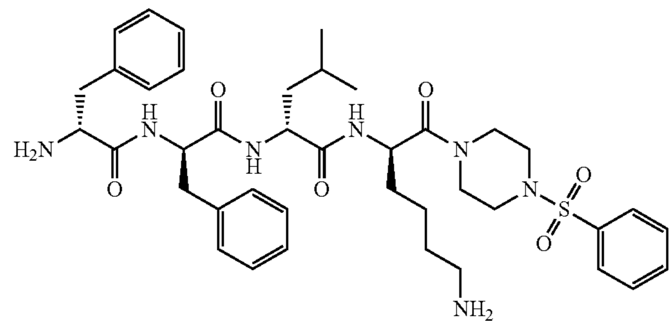
Compound (69)
