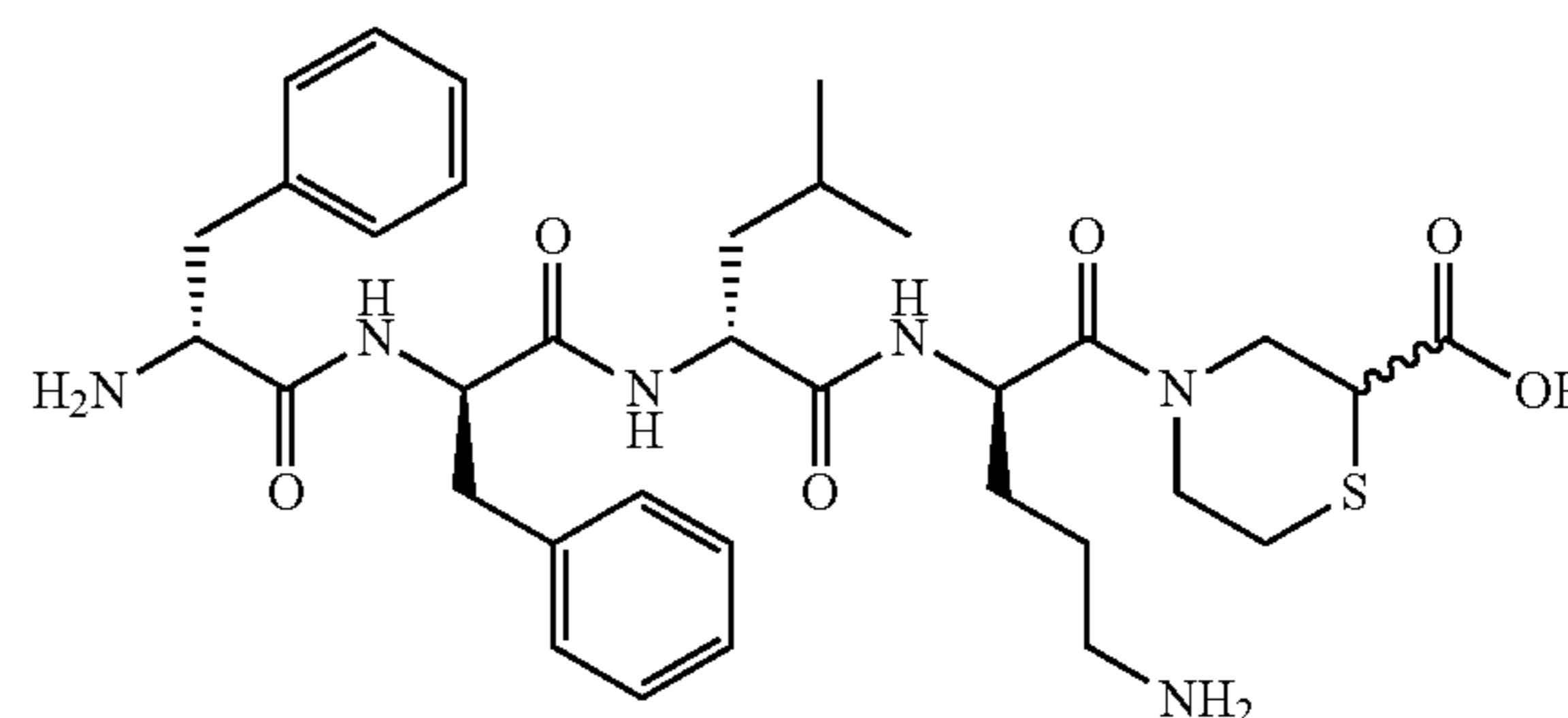
D-Phe-D-Phe-D-Leu-D-Orn-N(homothiomorpholine):
