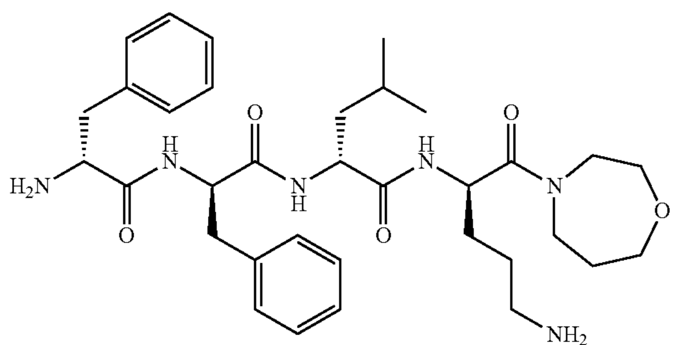
D-Phe-D-Phe-D-Leu-D-Dap(amidino)-[homomorpholine amide]:
