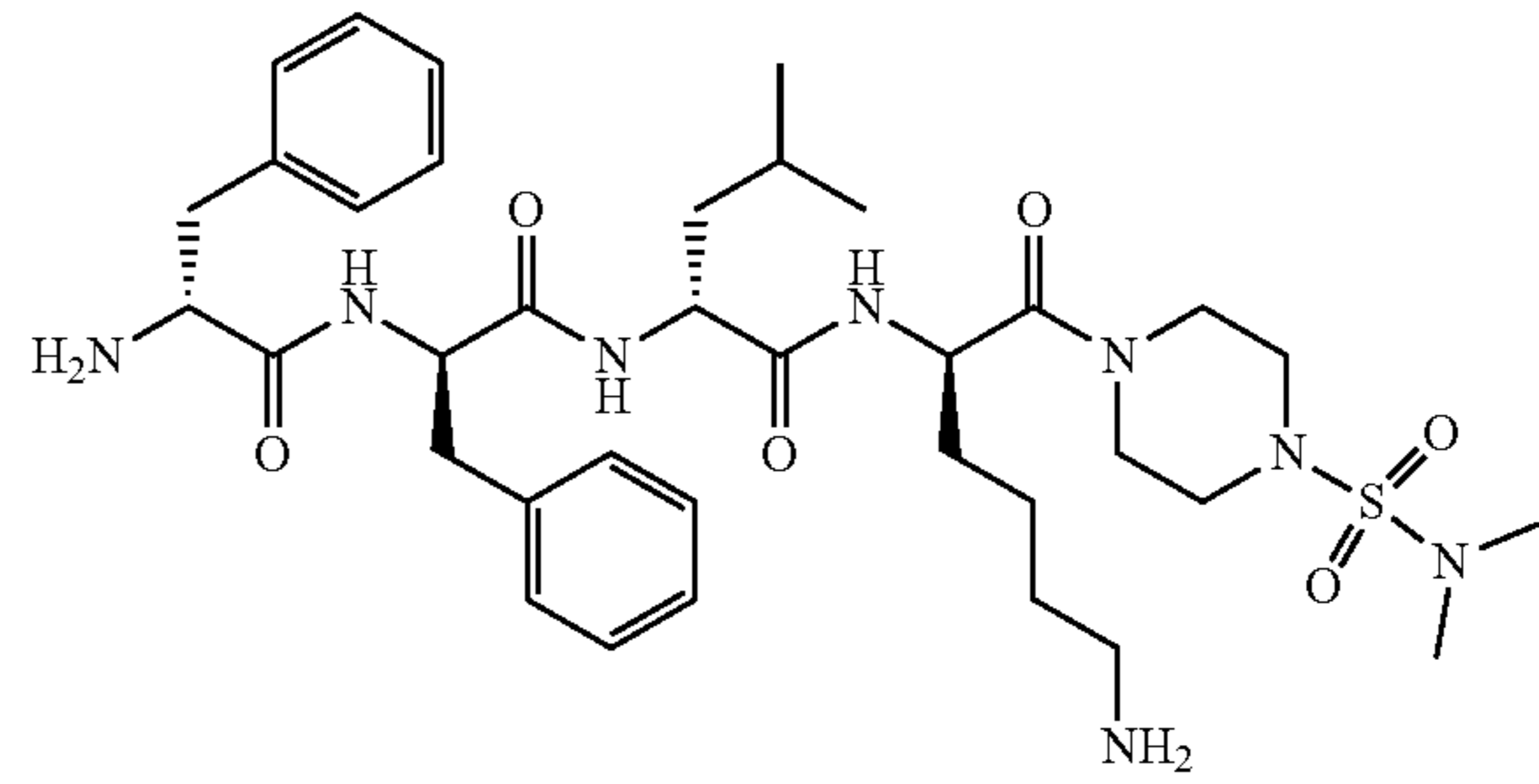
Compound (67)
