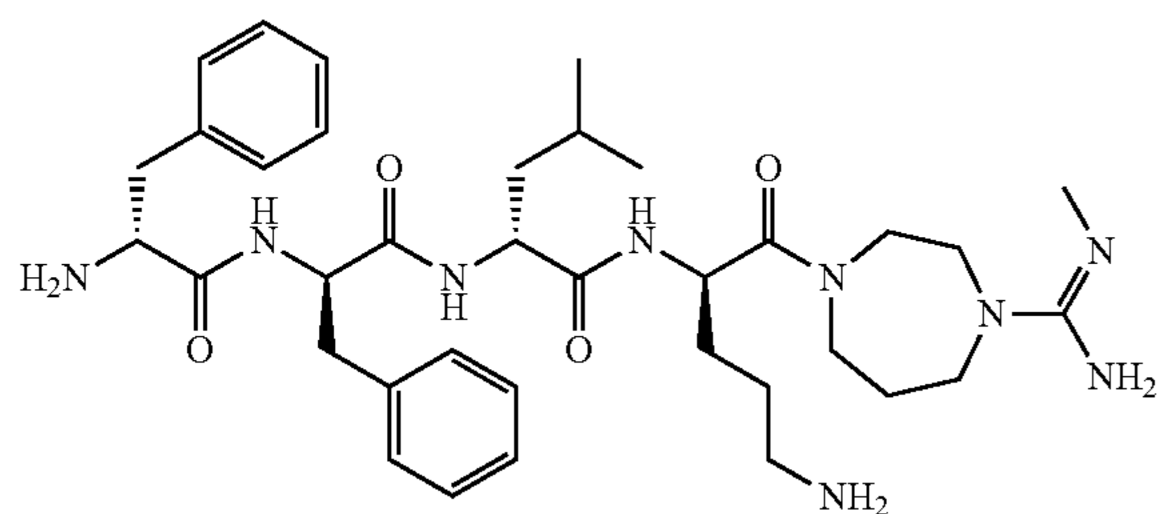
Compound (52)
