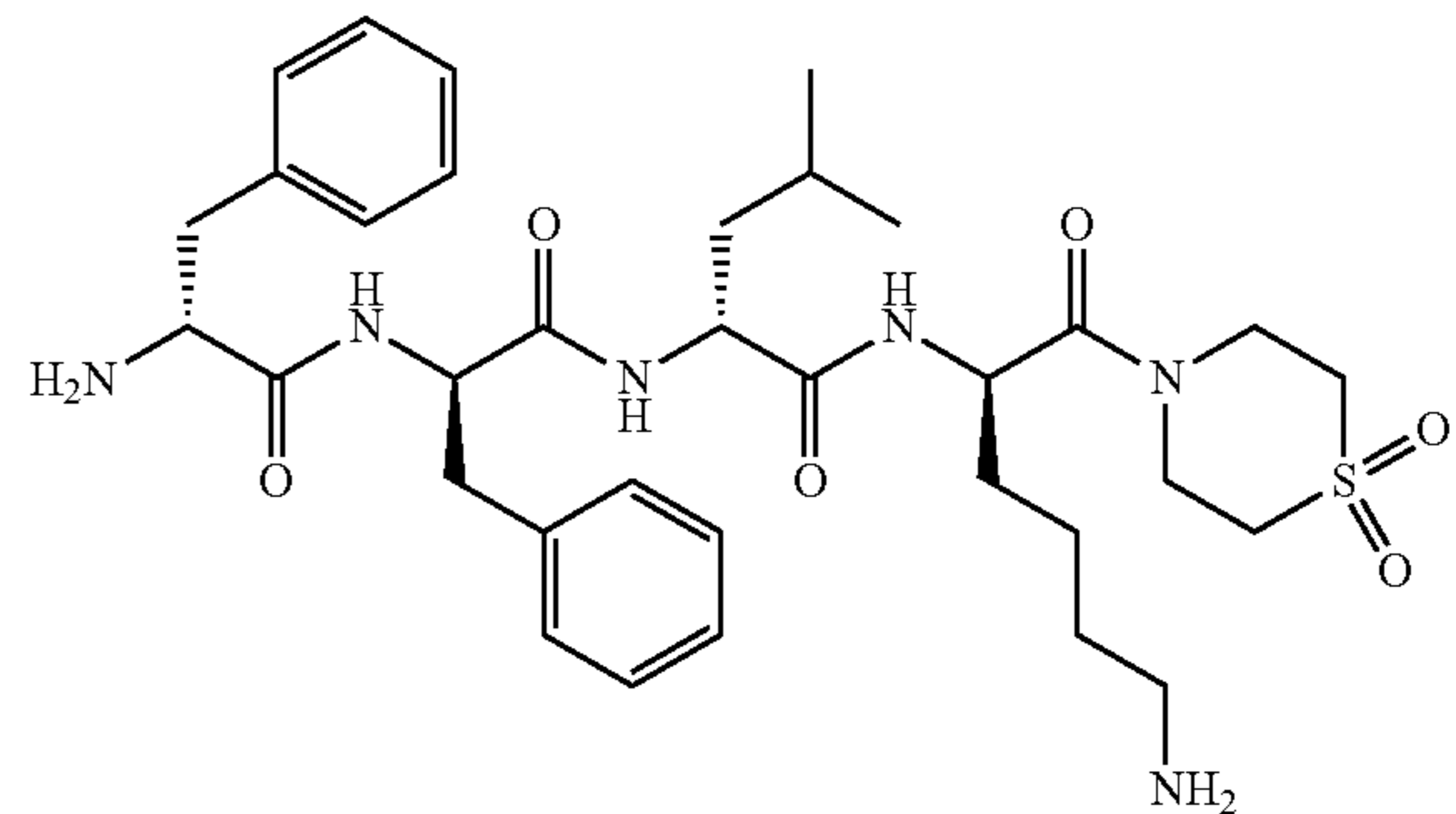
Compound (71)
