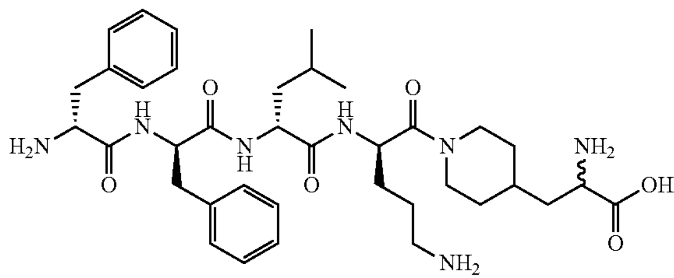
Compound (44)
