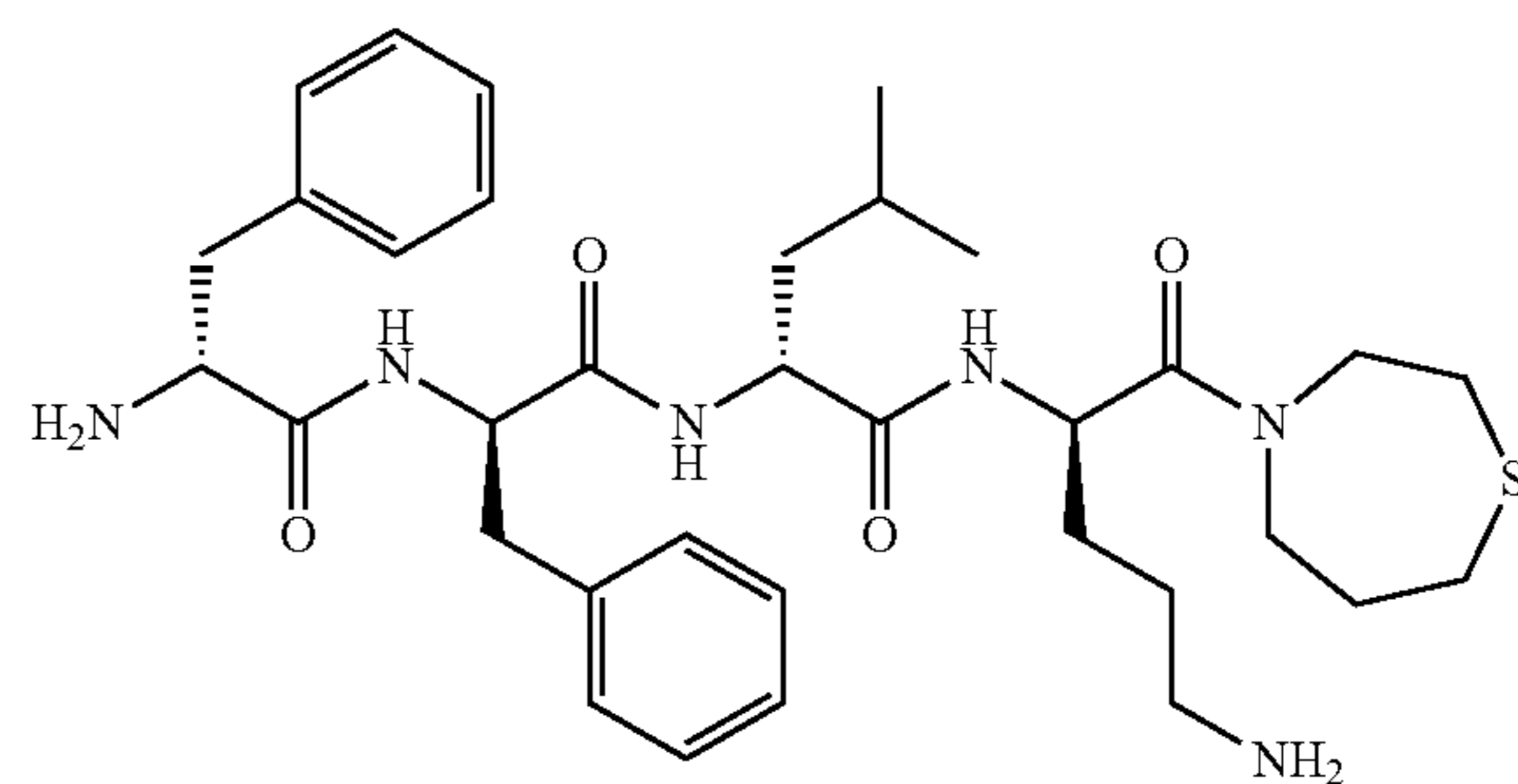
D-Phe-D-Phe-D-Leu-D-Dap(amidino)-[homothiomorpholine amide]:
