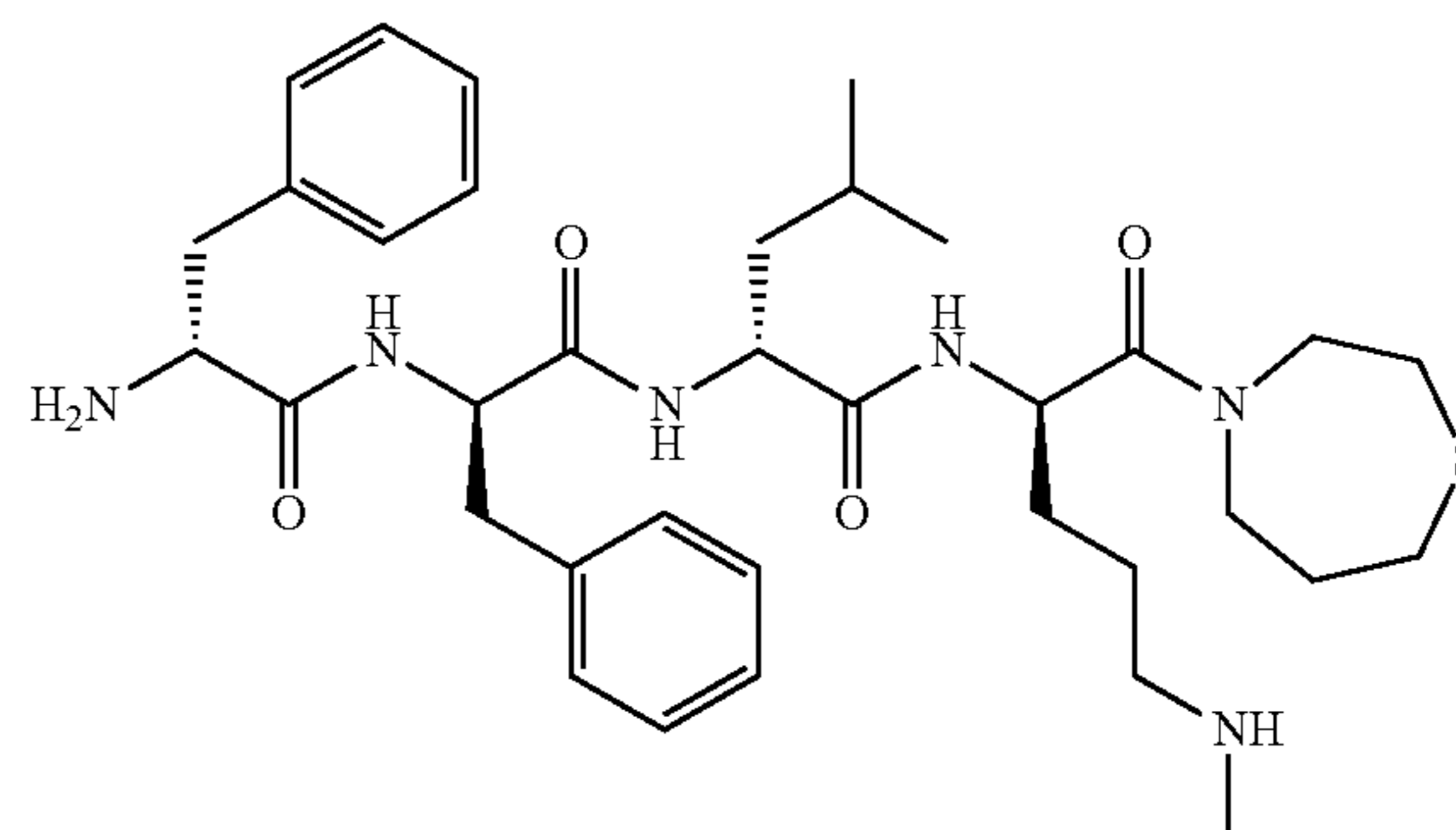
Compound (101)
