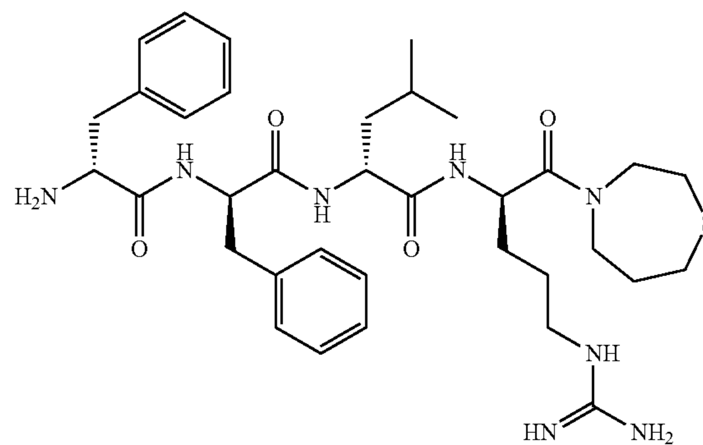
Compound (99)
