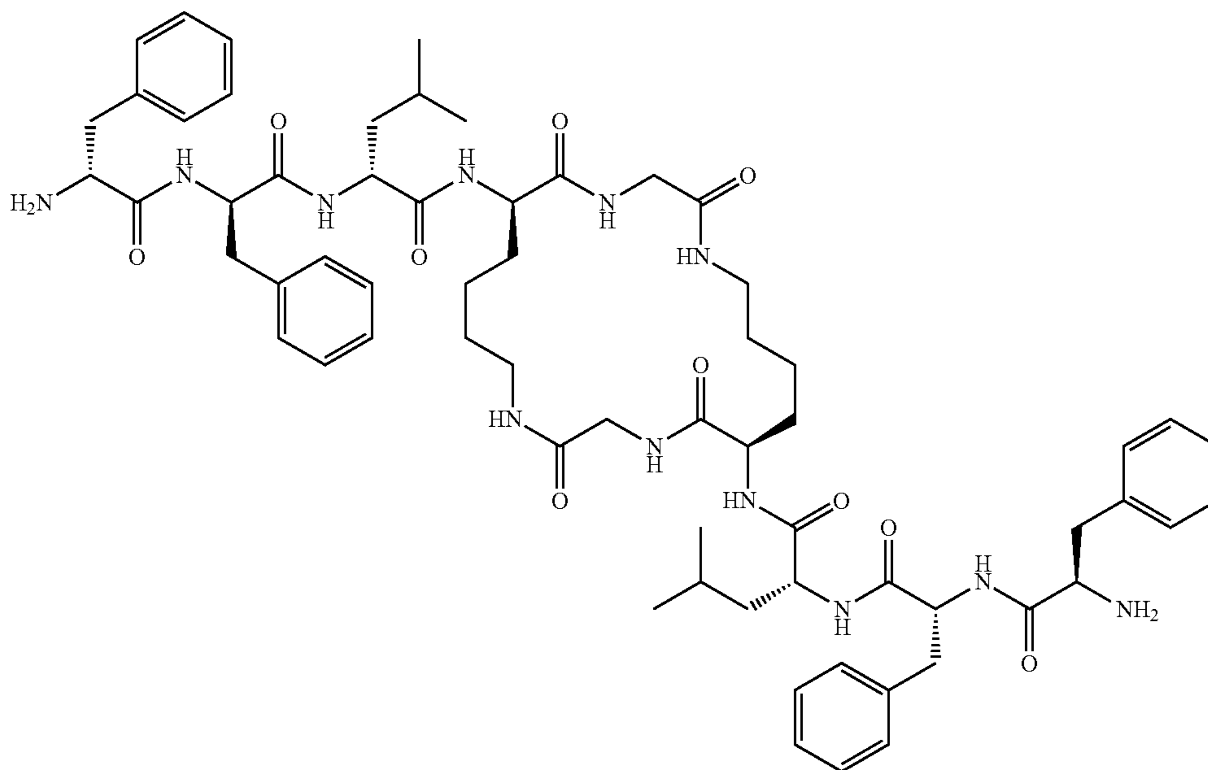
D-Phe-D-Phe-D-Leu-D-Orn-[R/S-2-carboxymorpholine]-OH:
