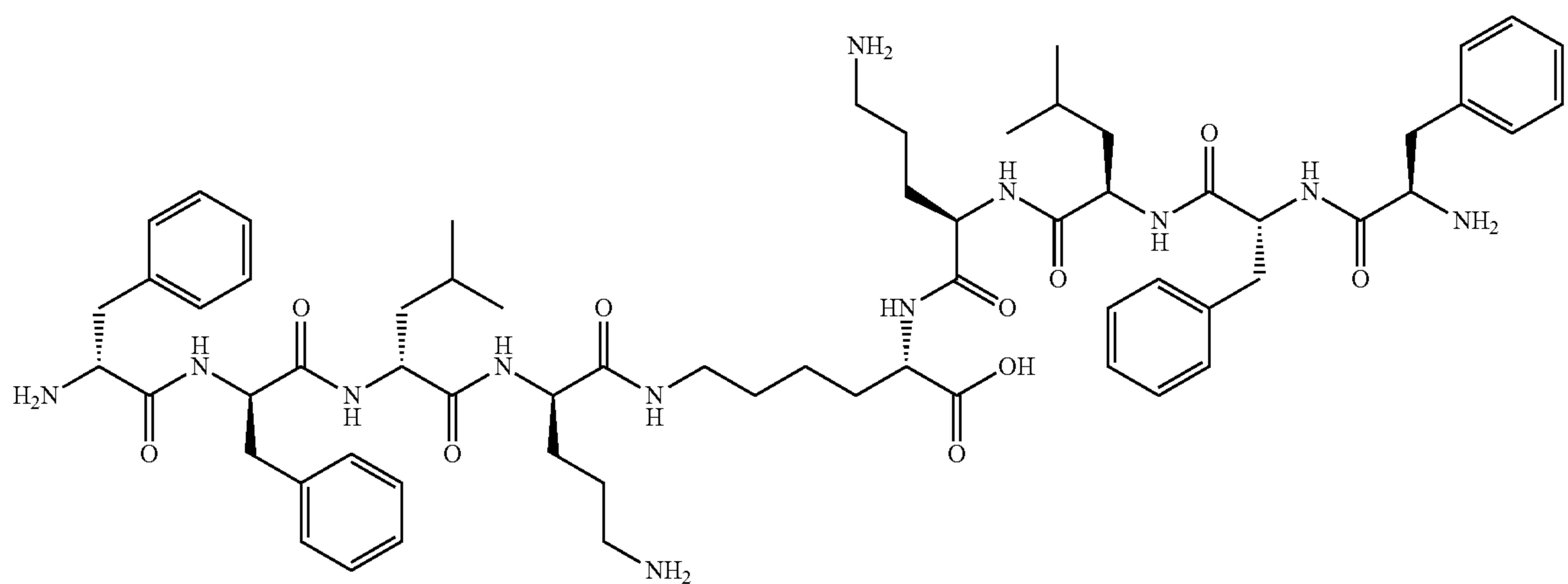
Compound (76)
