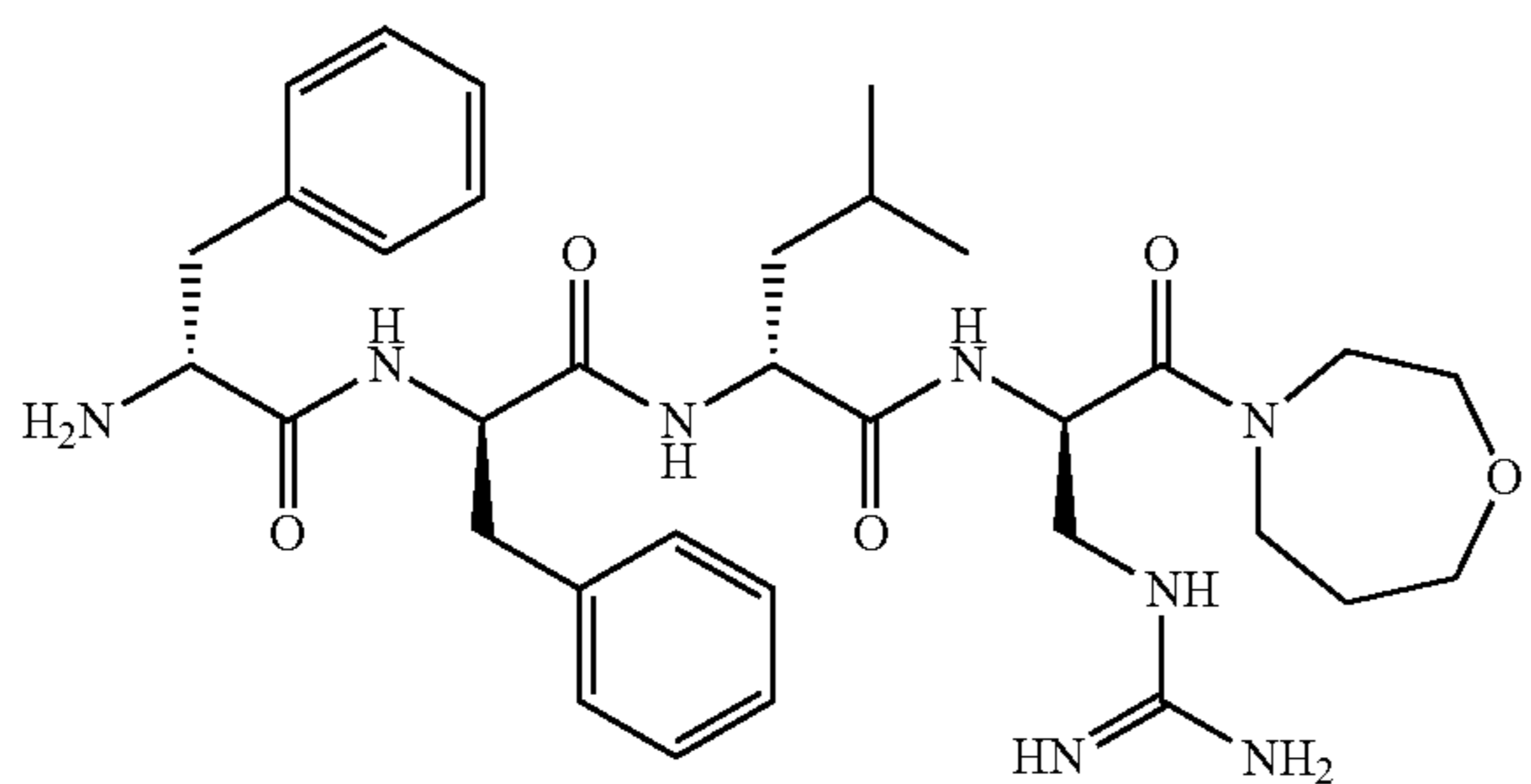
Compound (94)
