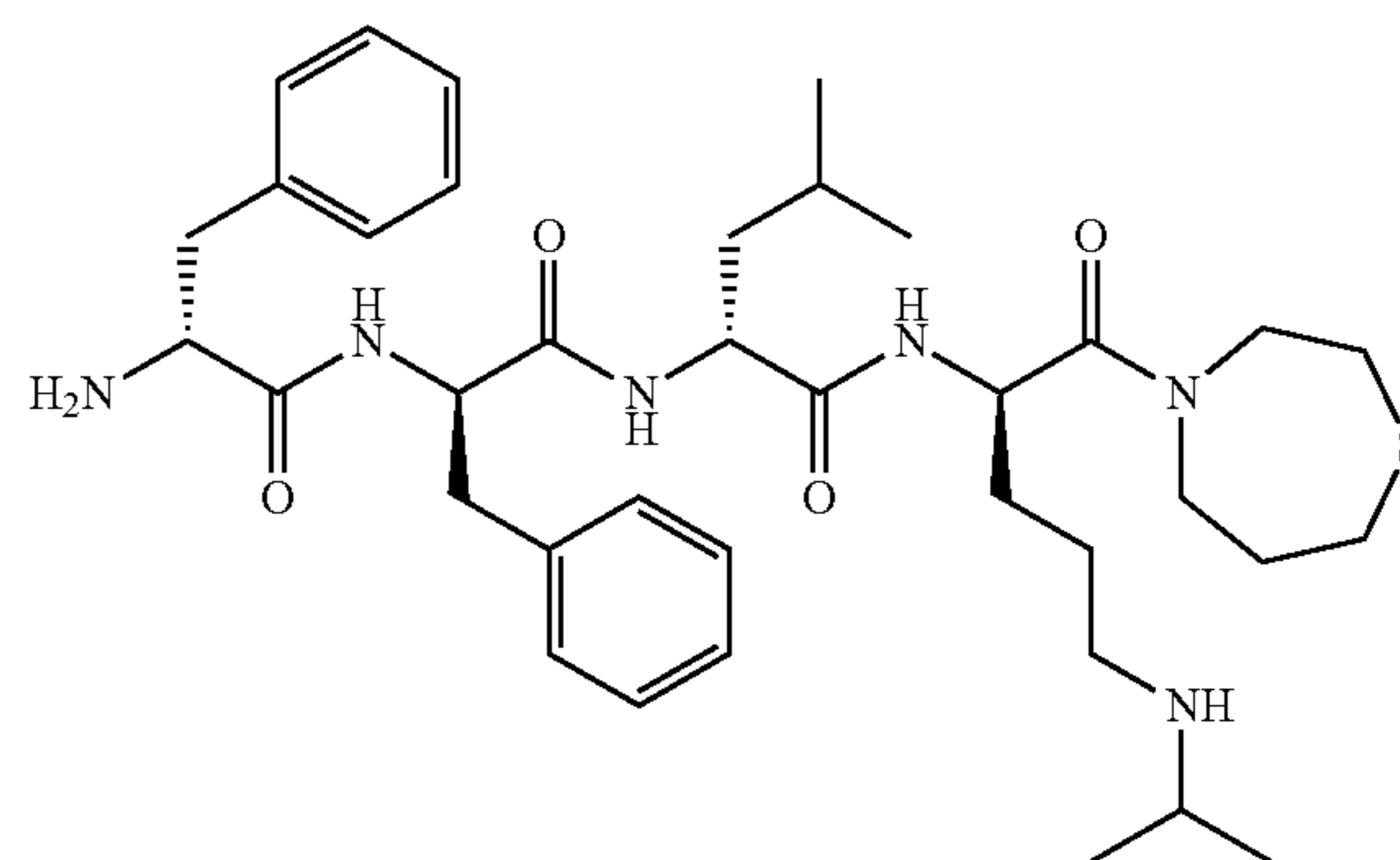
Compound (103)
