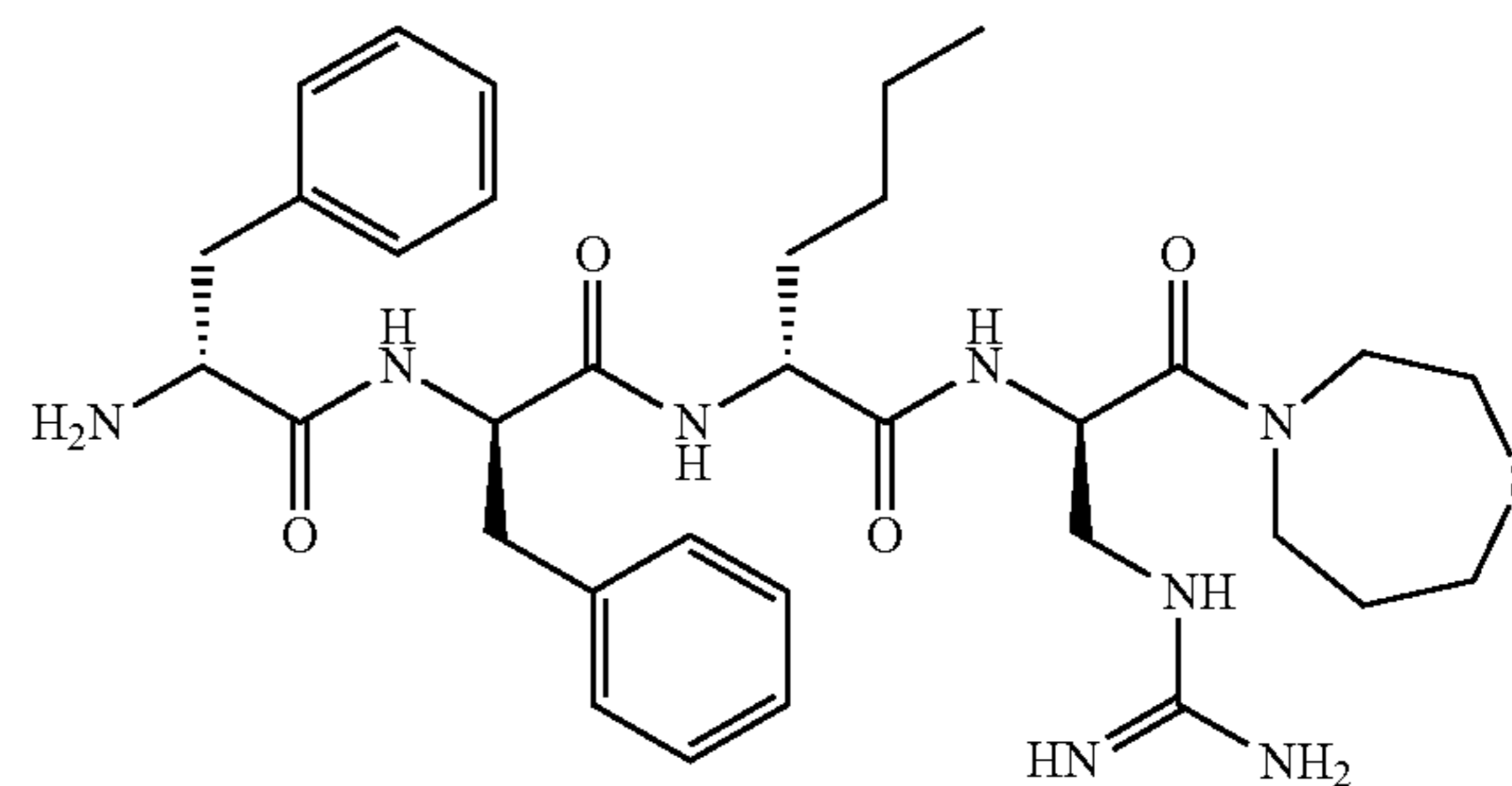
Compound (97)
