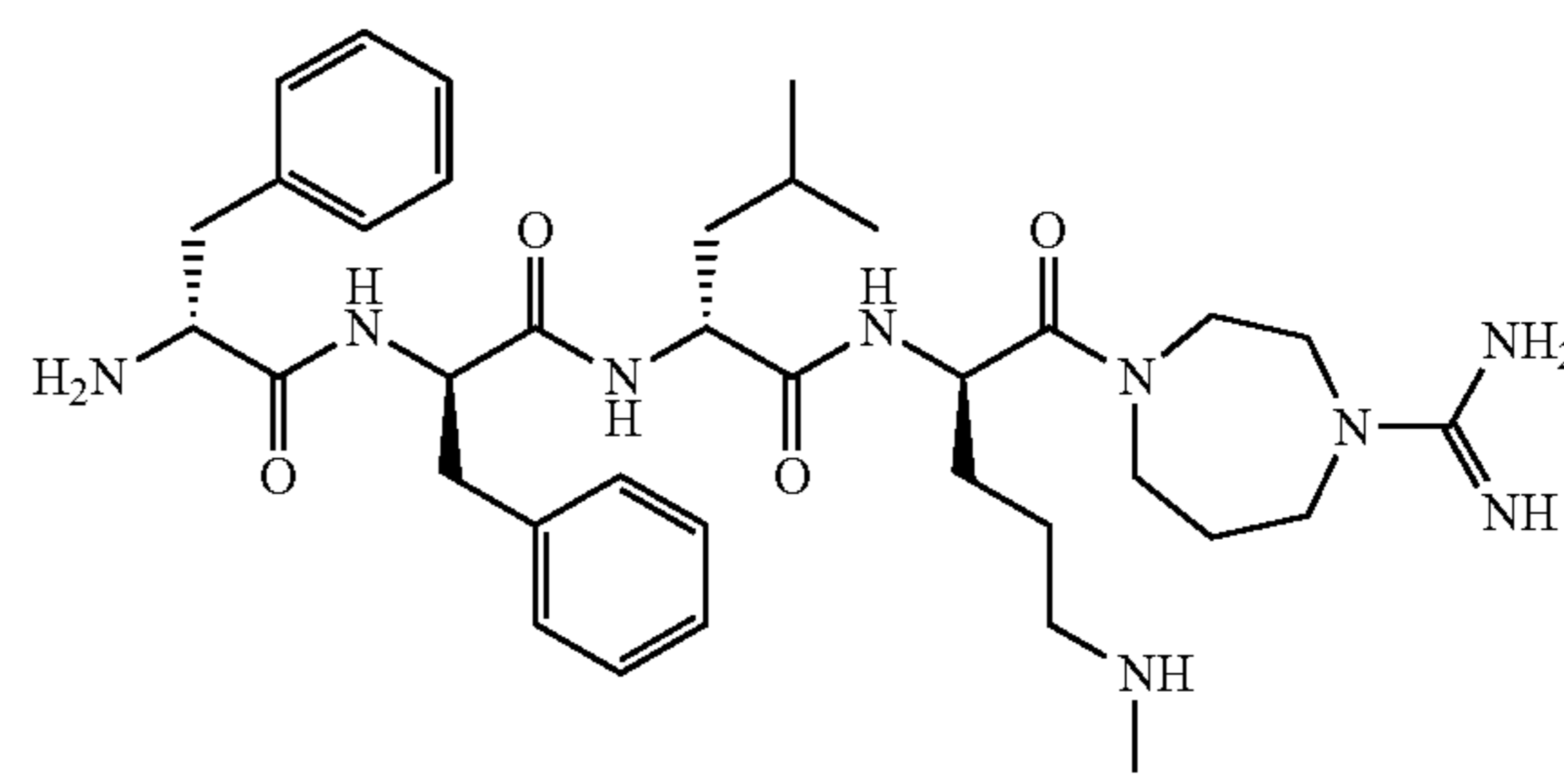
Compound (57)
