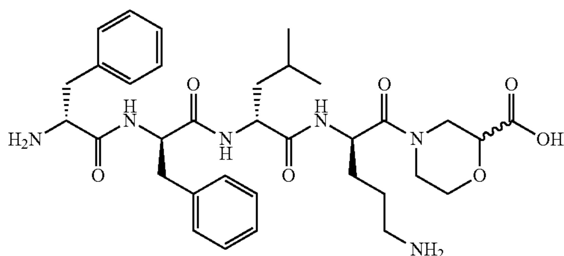
D-Phe-D-Phe-D-Leu-D-Orn-N(homomorpholine):
