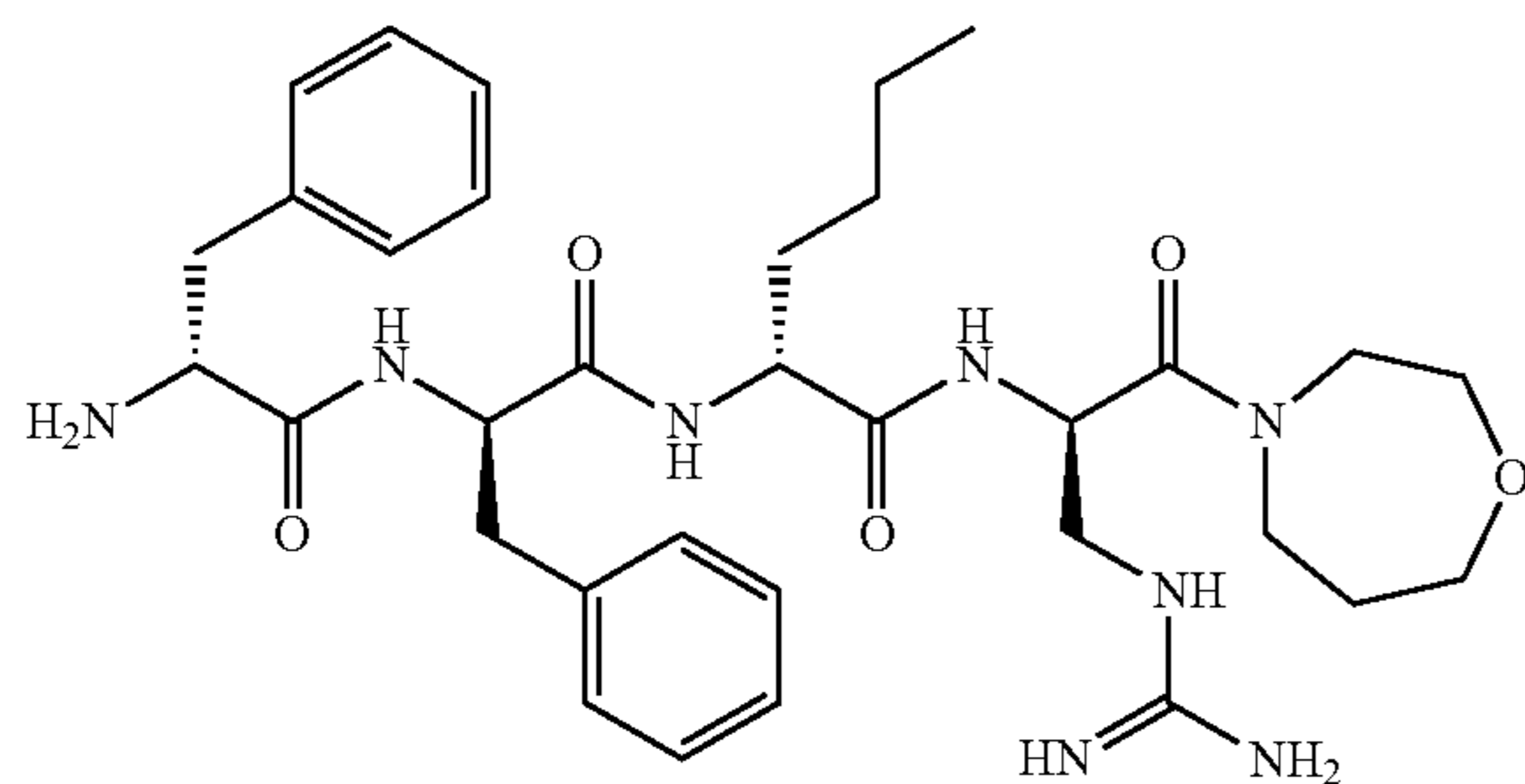
Compound (96)
