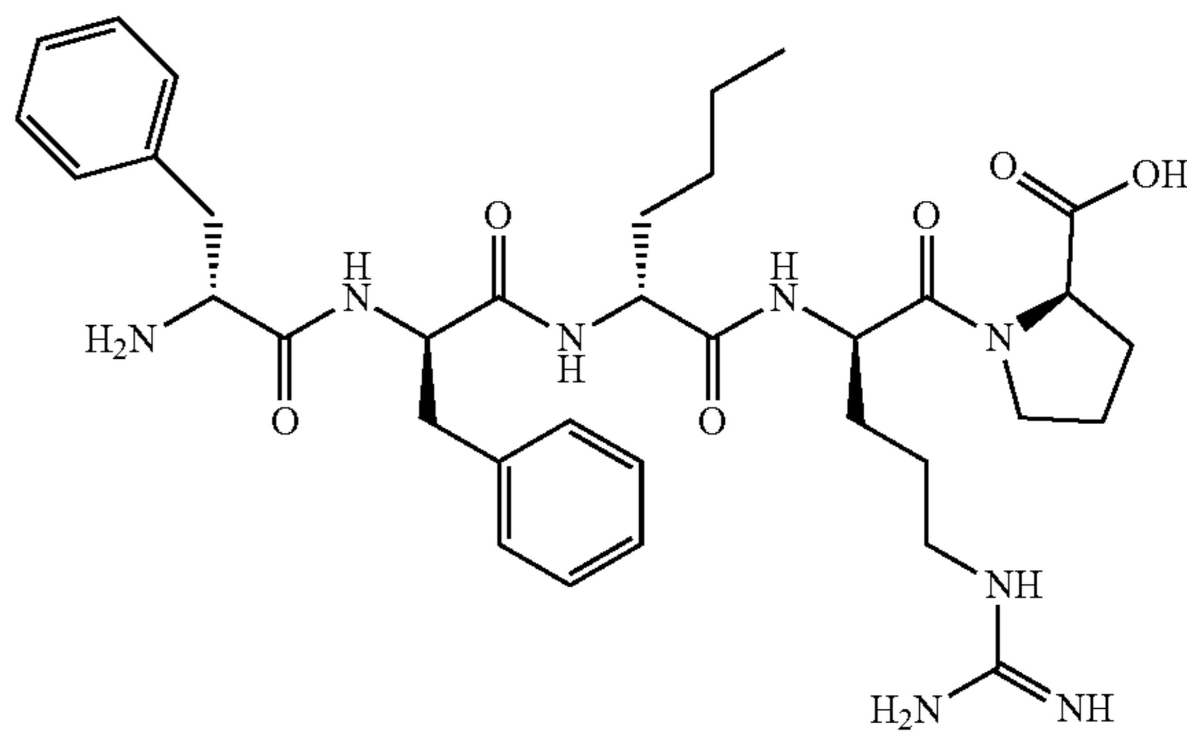
Compound (40)
