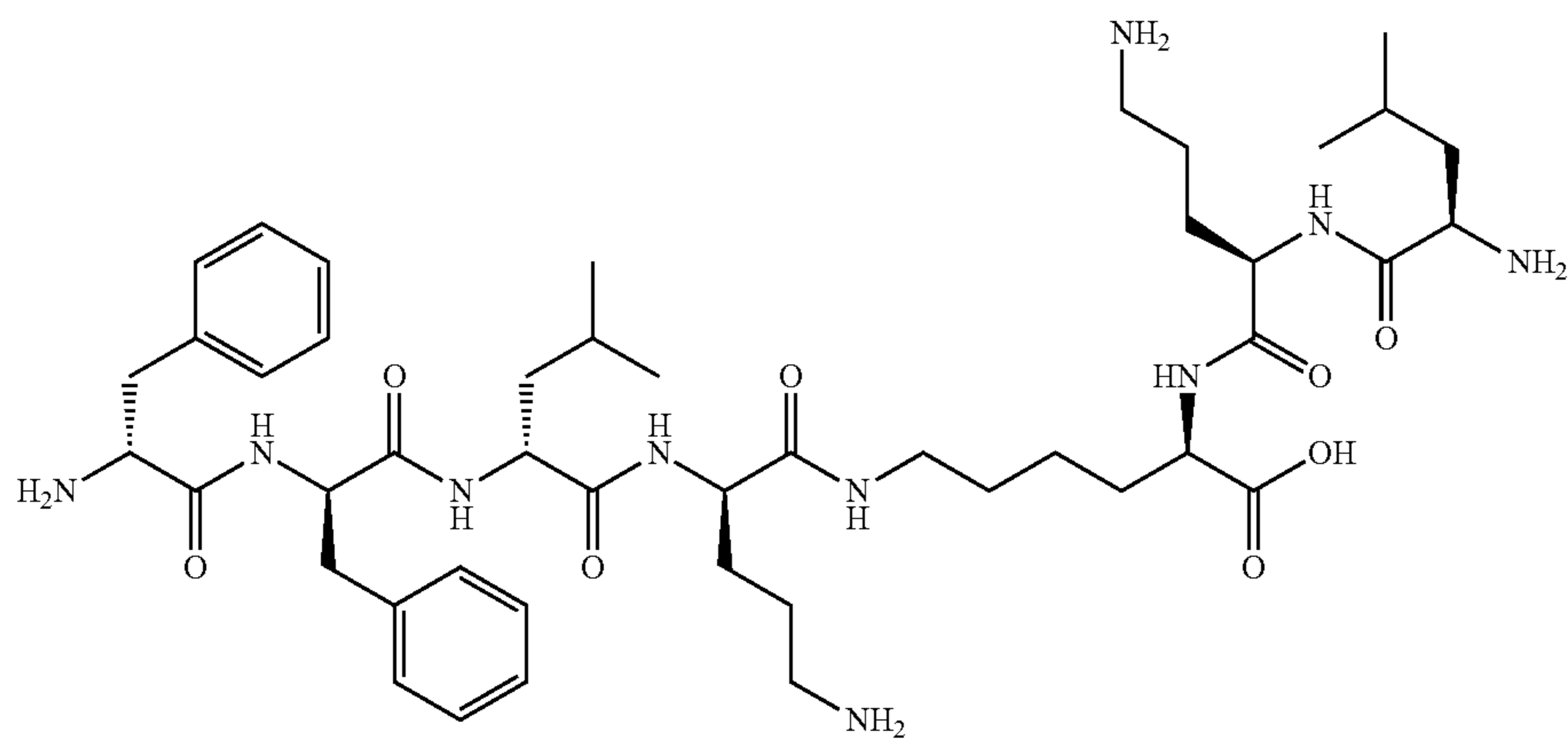
D-Phe-D-Phe-D-Leu-D-Orn-εLys-OH | D-Phe-D-Leu-D-Orn
