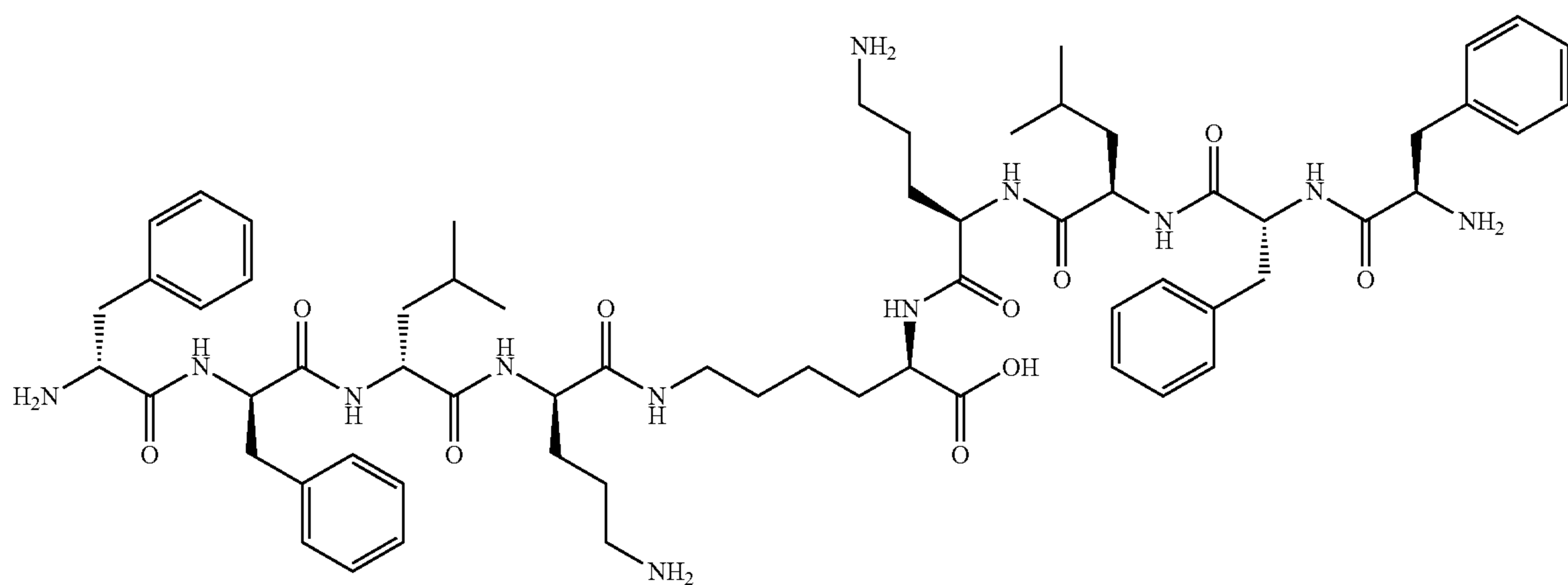
Compound (85)
