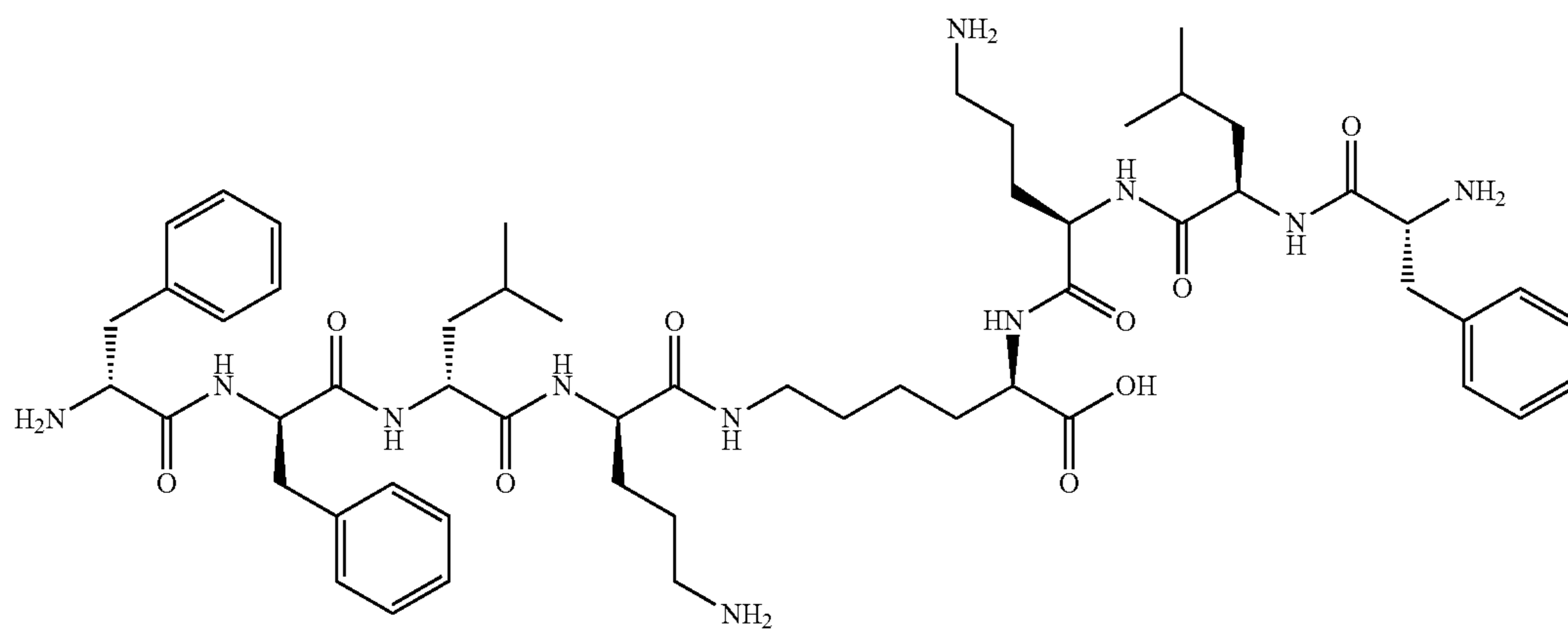
D-Phe-D-Phe-D-Leu-D-Orn-εLys-OH | D-Phe-D-Phe-D-Leu-D-Orn
