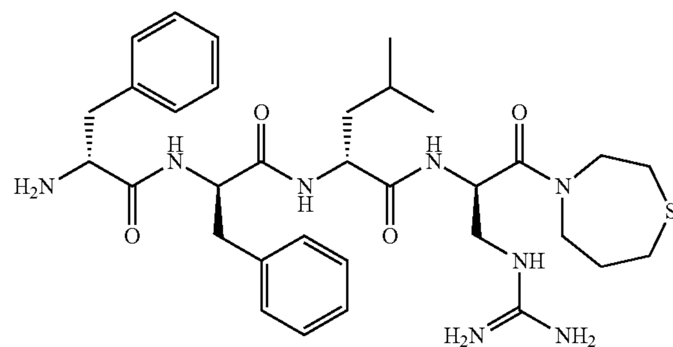
Compound (95)
