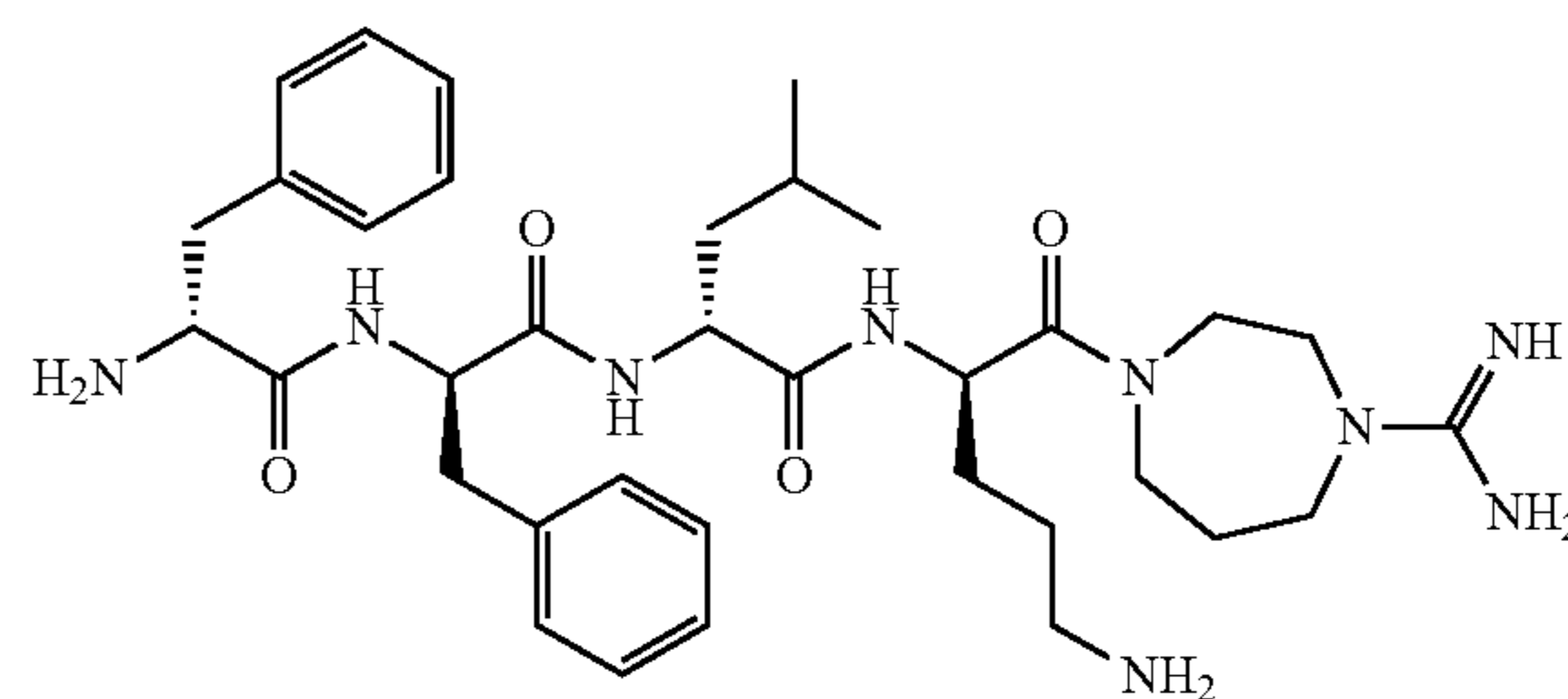
Compound (53)
