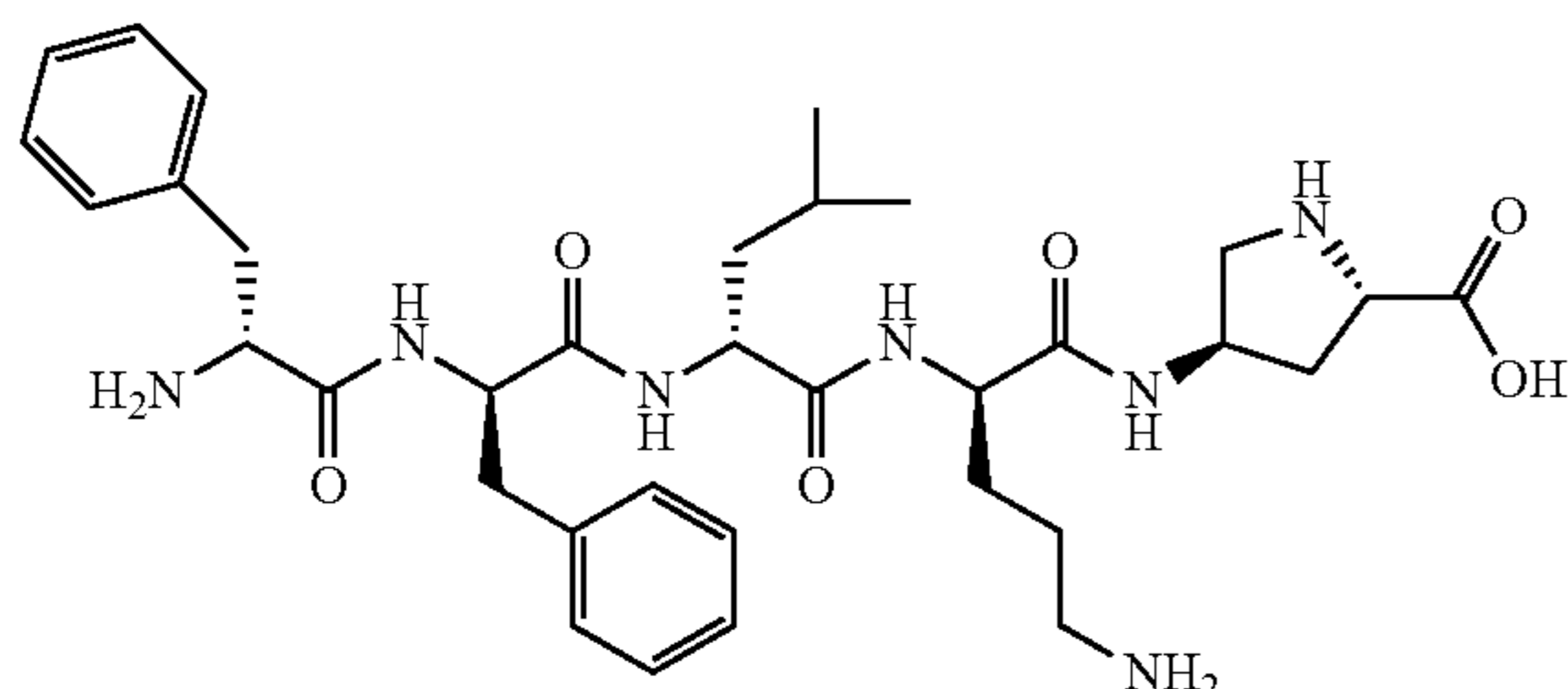
Compound (41)
