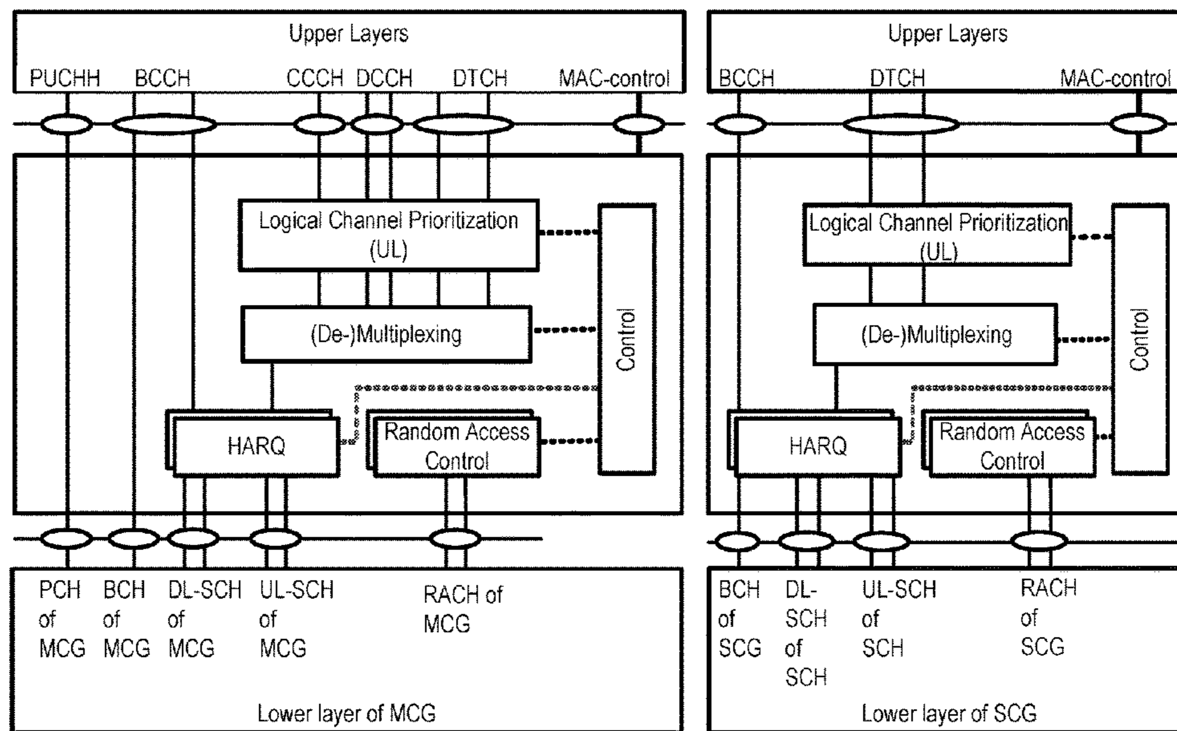
Dual-Connectivity- two MAC entities at UE side
