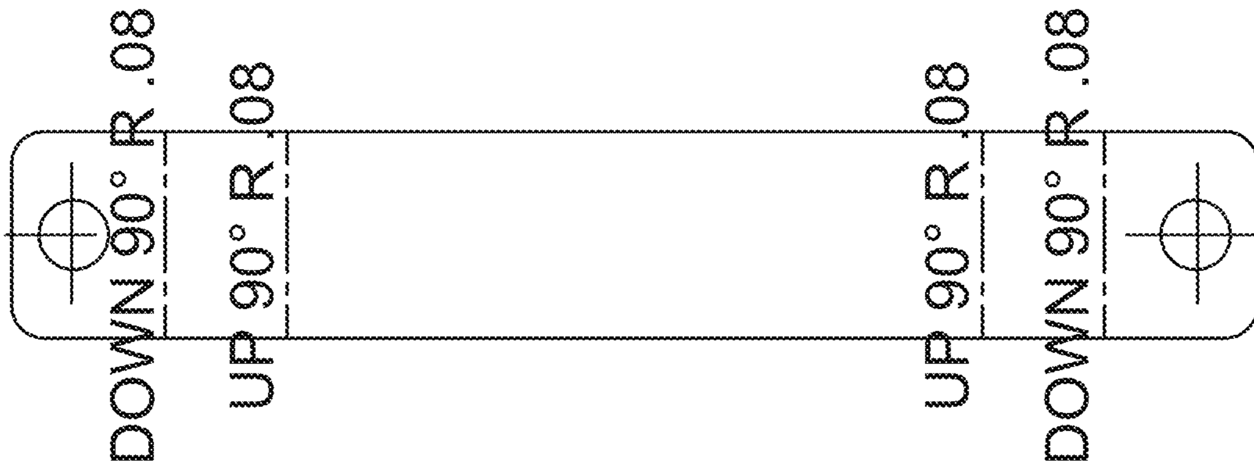
FLAT PATTERN
