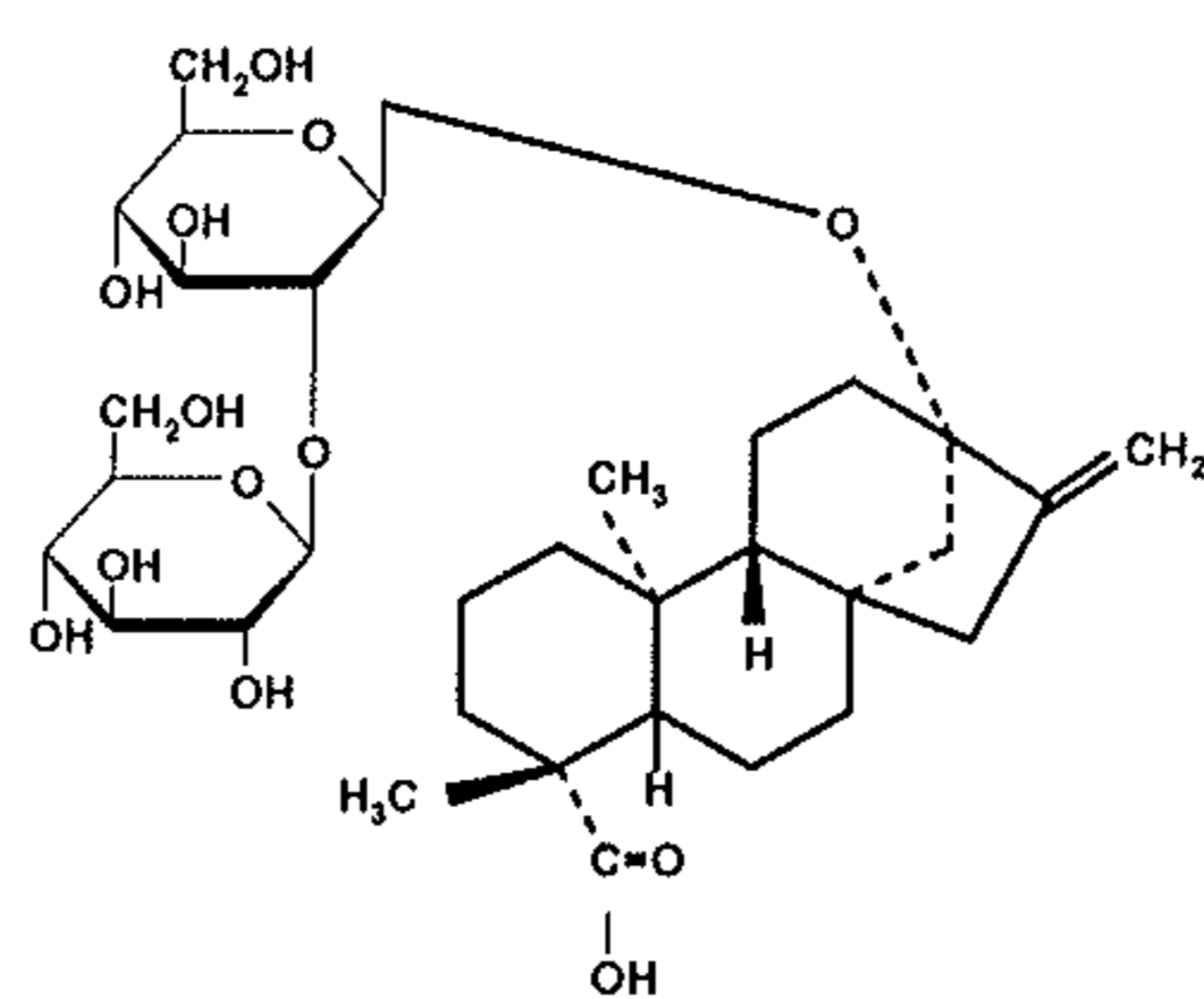
Steviolbioside
