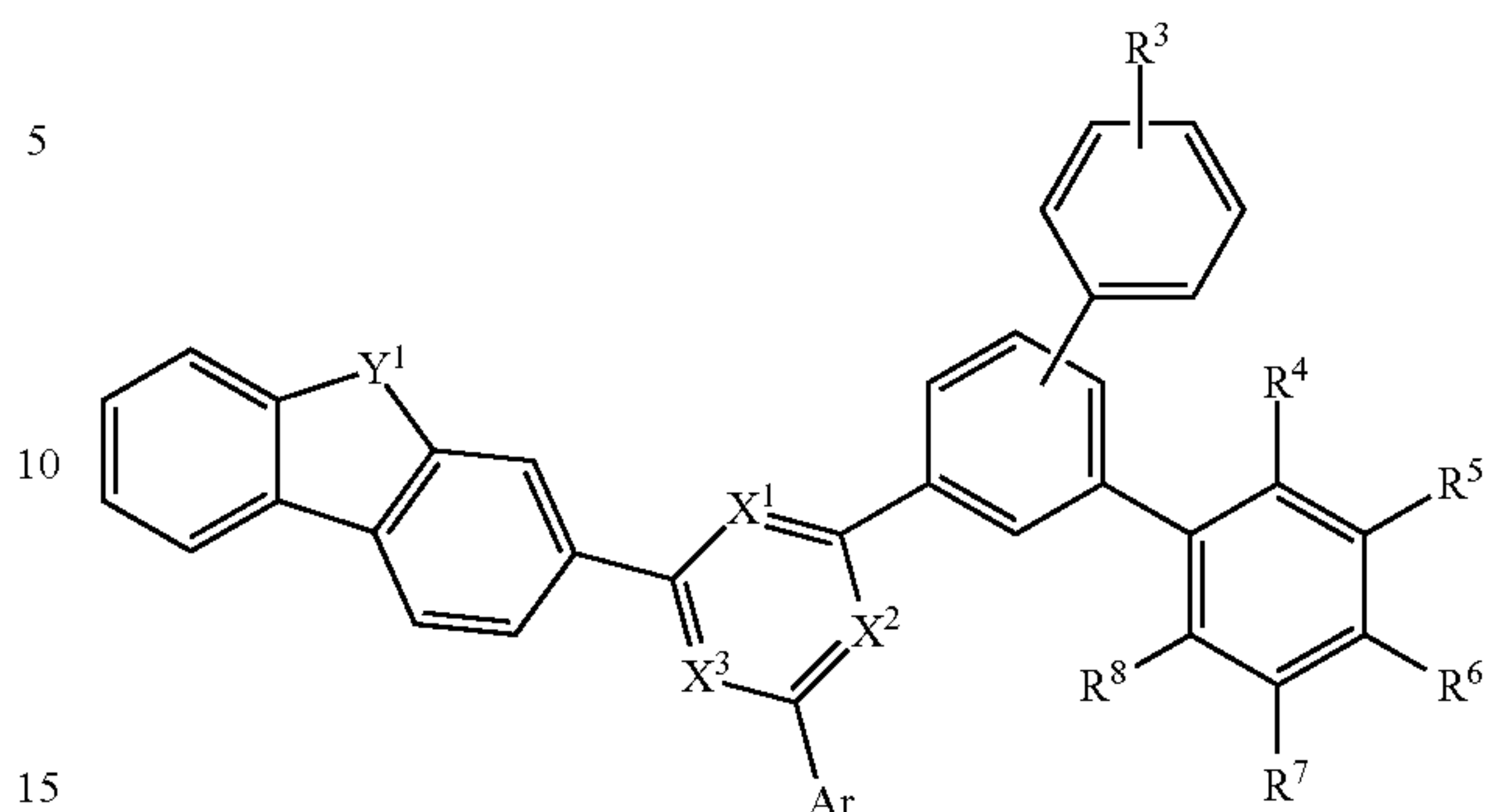
[Chemical Formula 1-2]
