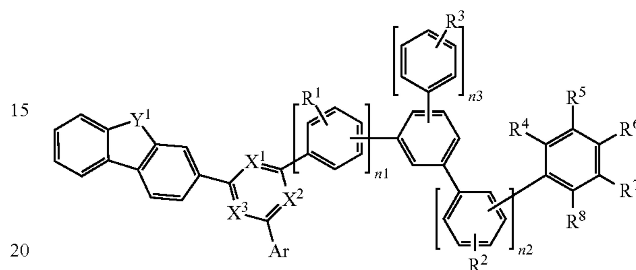
[Chemical Formula 1]
