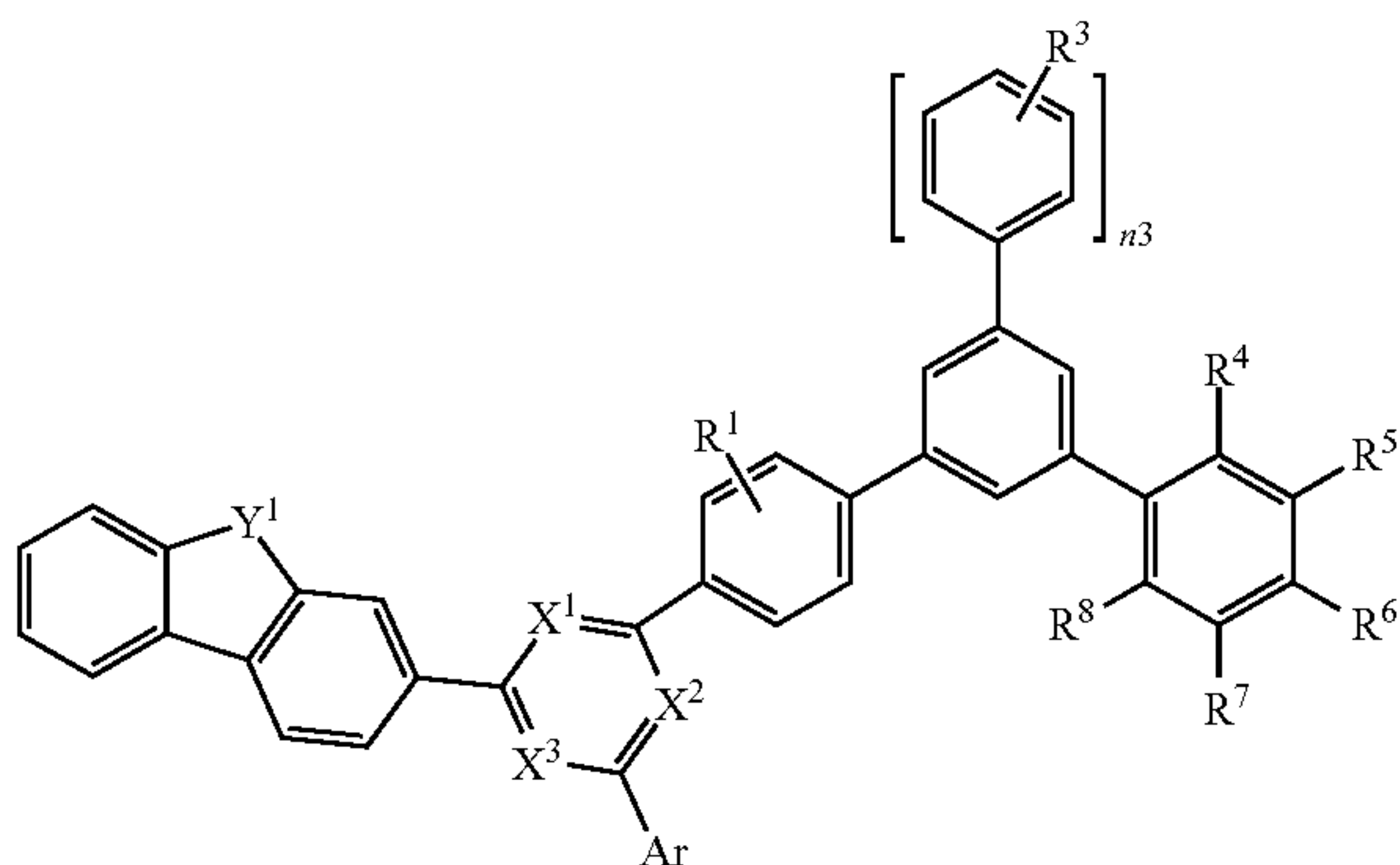
[Chemical Formula 1-3a]
