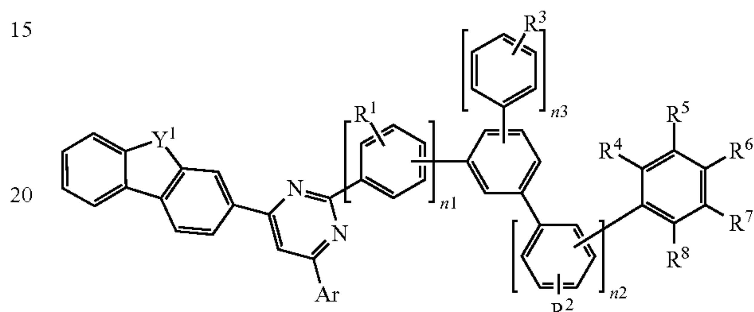
[Chemical Formula 1-III]
