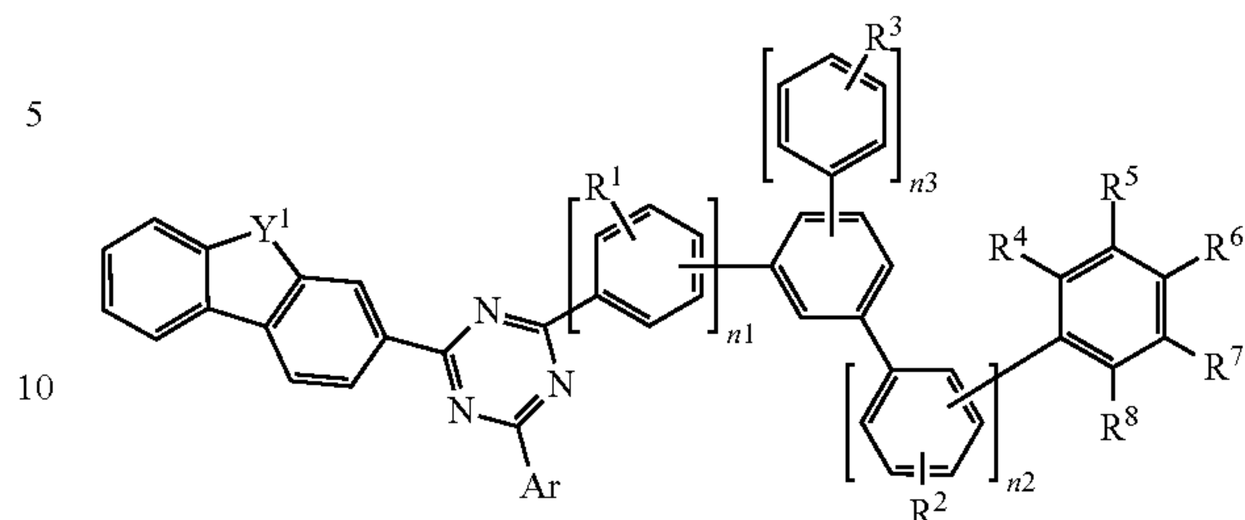
[Chemical Formula 1-II]
