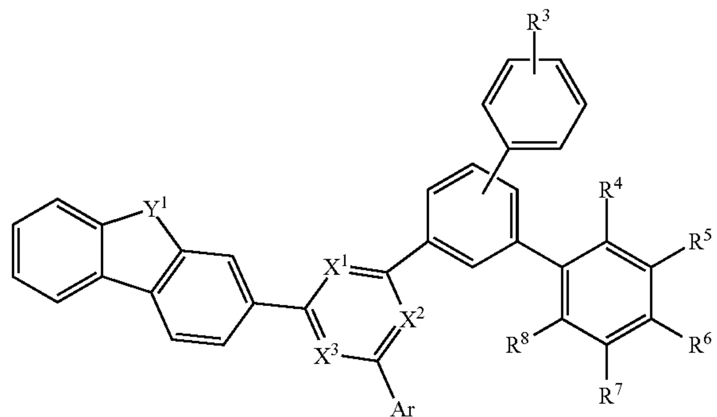
[Chemical Formula 1-1]
