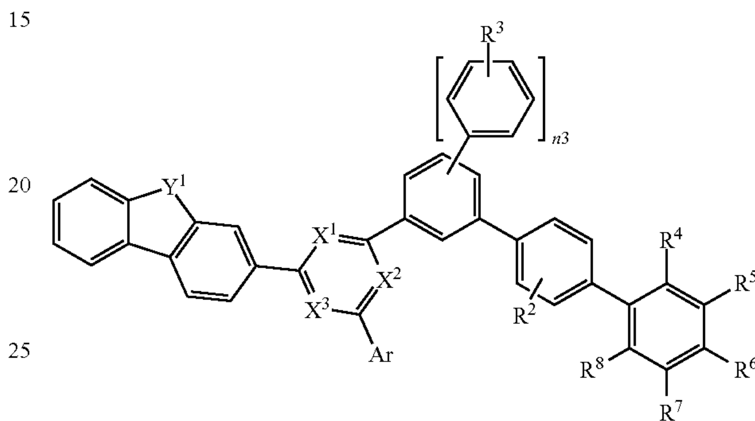
[Chemical Formula 1-5]
