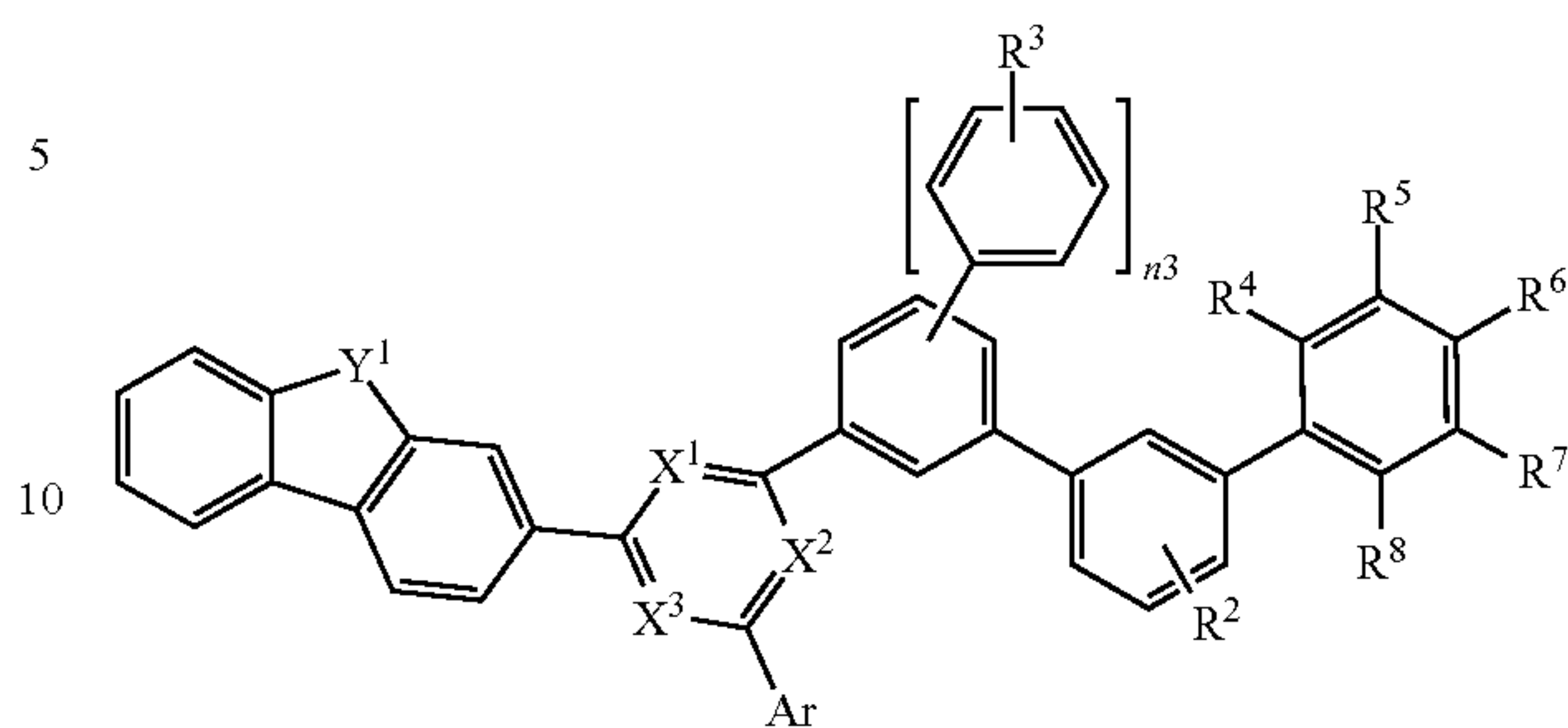
[Chemical Formula 1-5]
