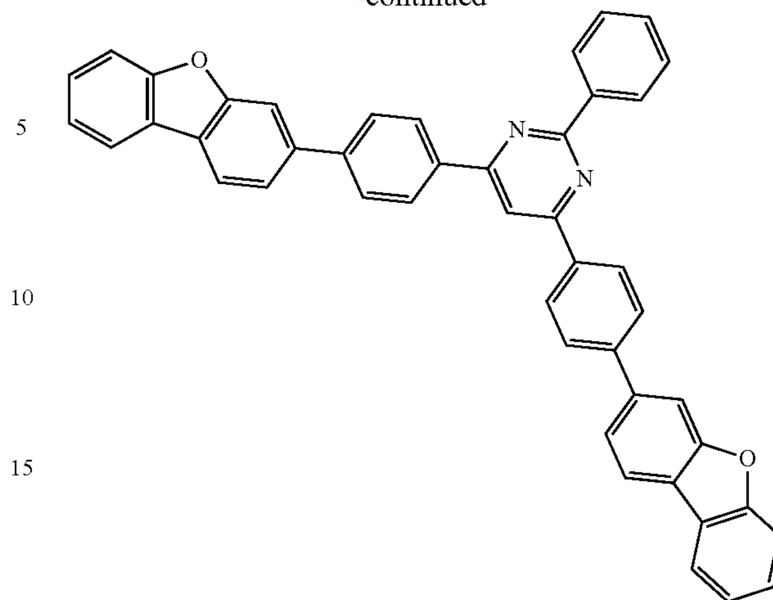
Comparative Compound 5
