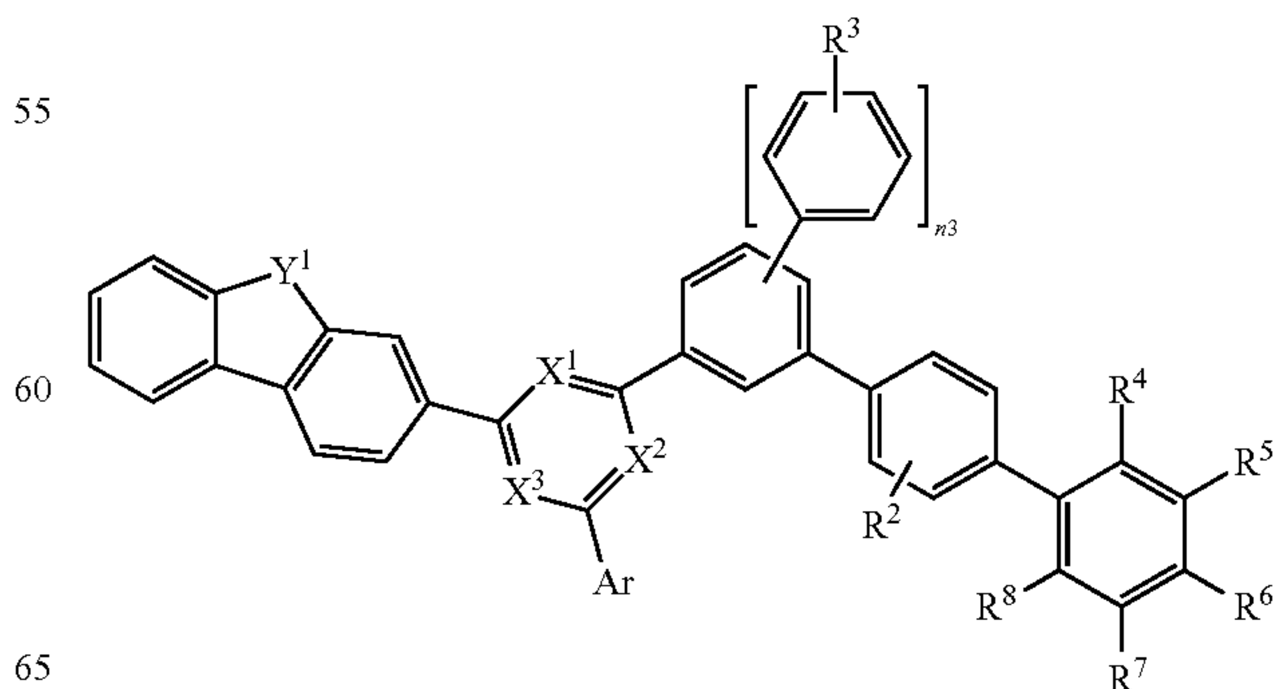
[Chemical Formula 1-5]
