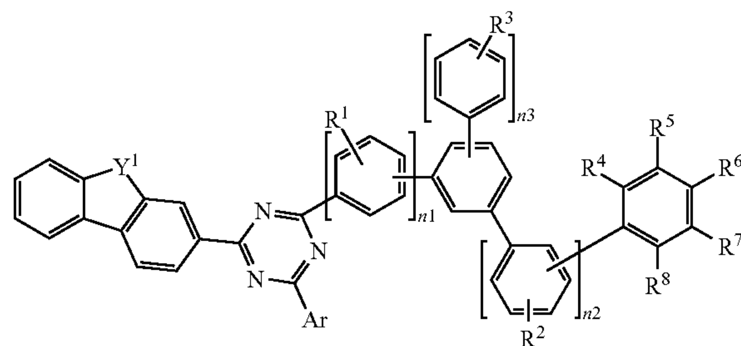
[Chemical Formula 1-I]
