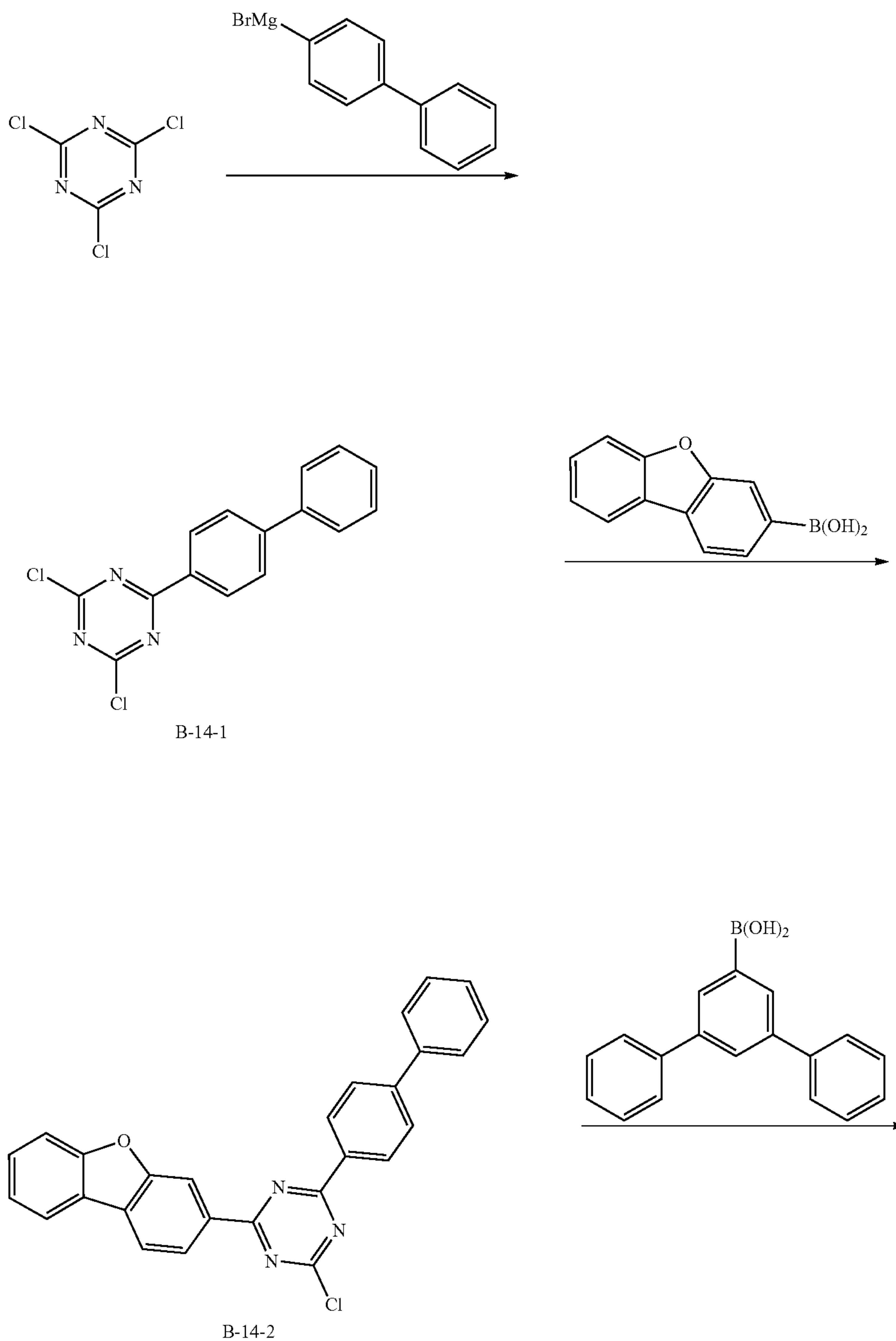
[Reaction Scheme 6]
