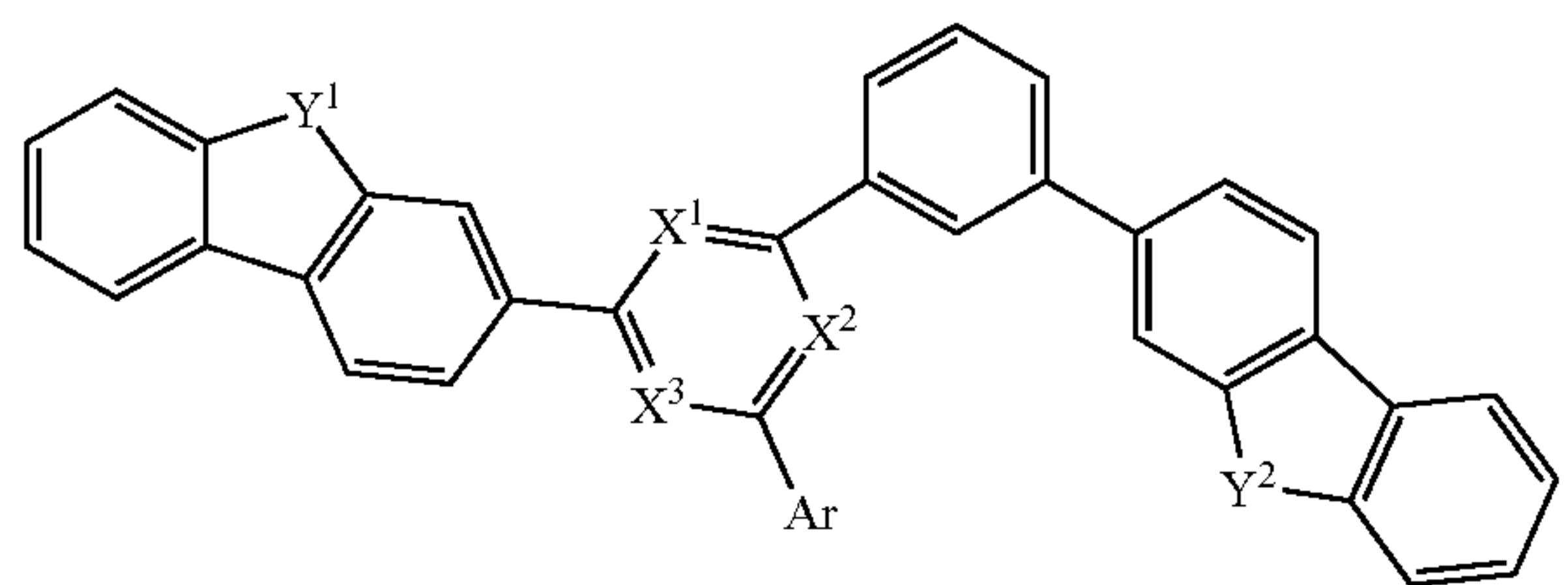
[Chemical Formula 1-2]
