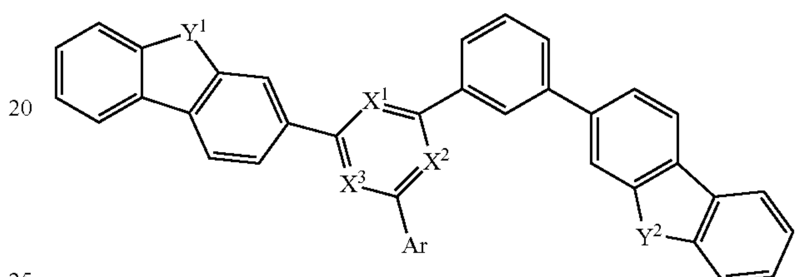
[Chemical Formula 1-3]
