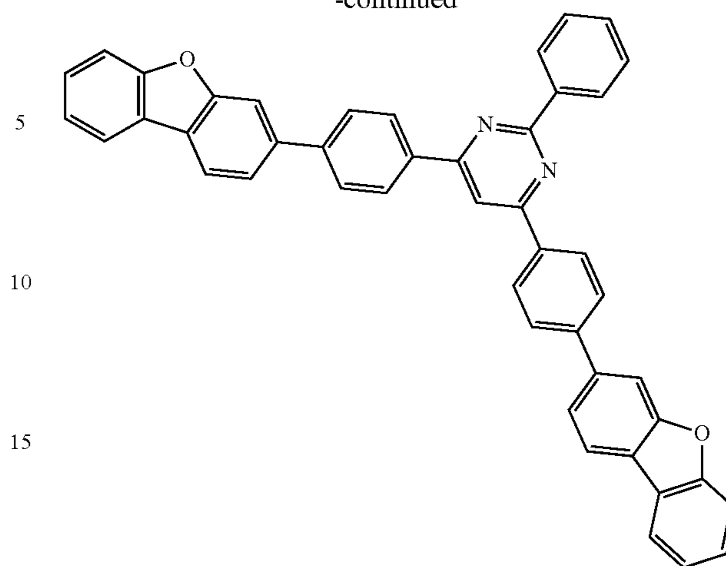
Comparative Compound 5
