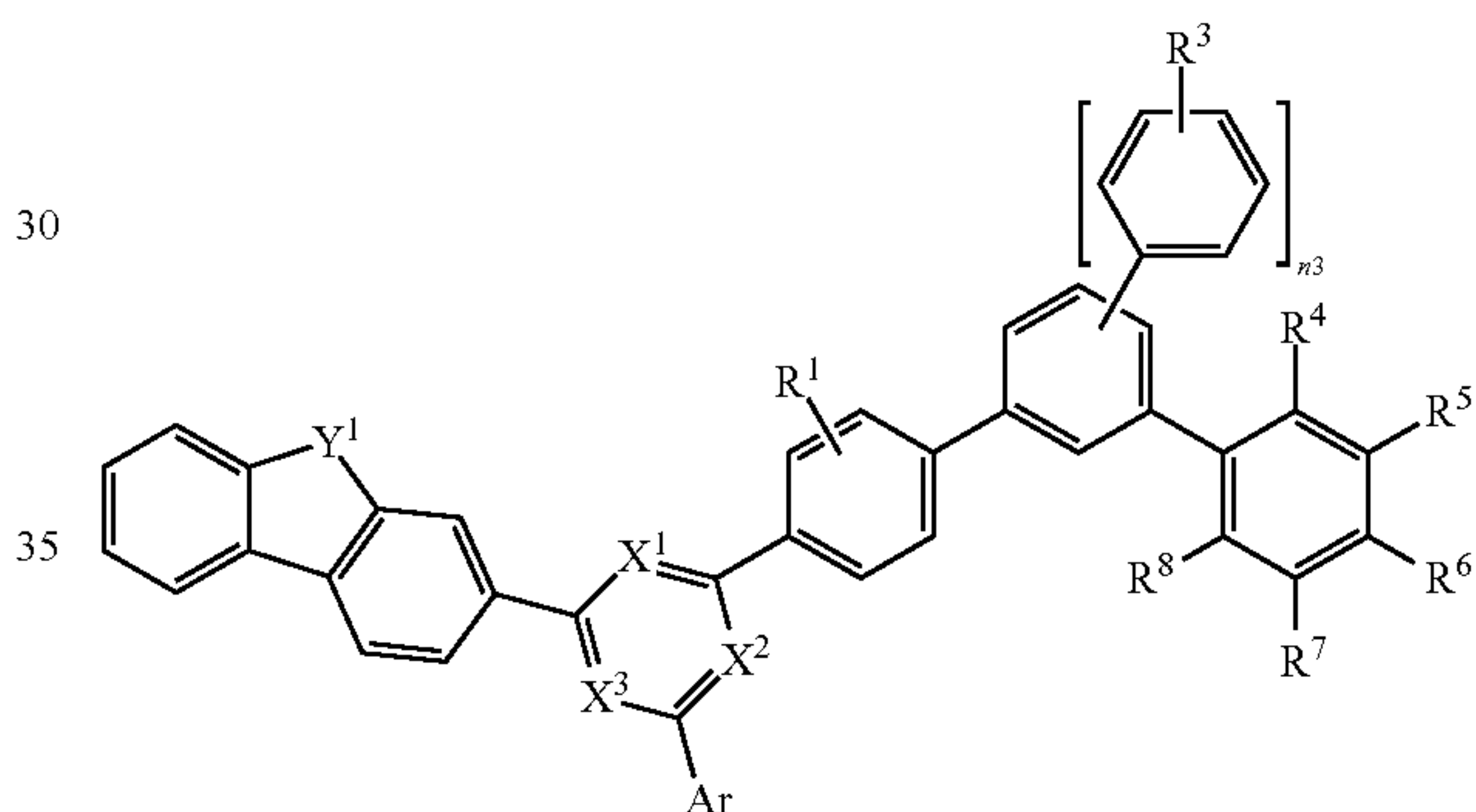
[Chemical Formula 1-4]
