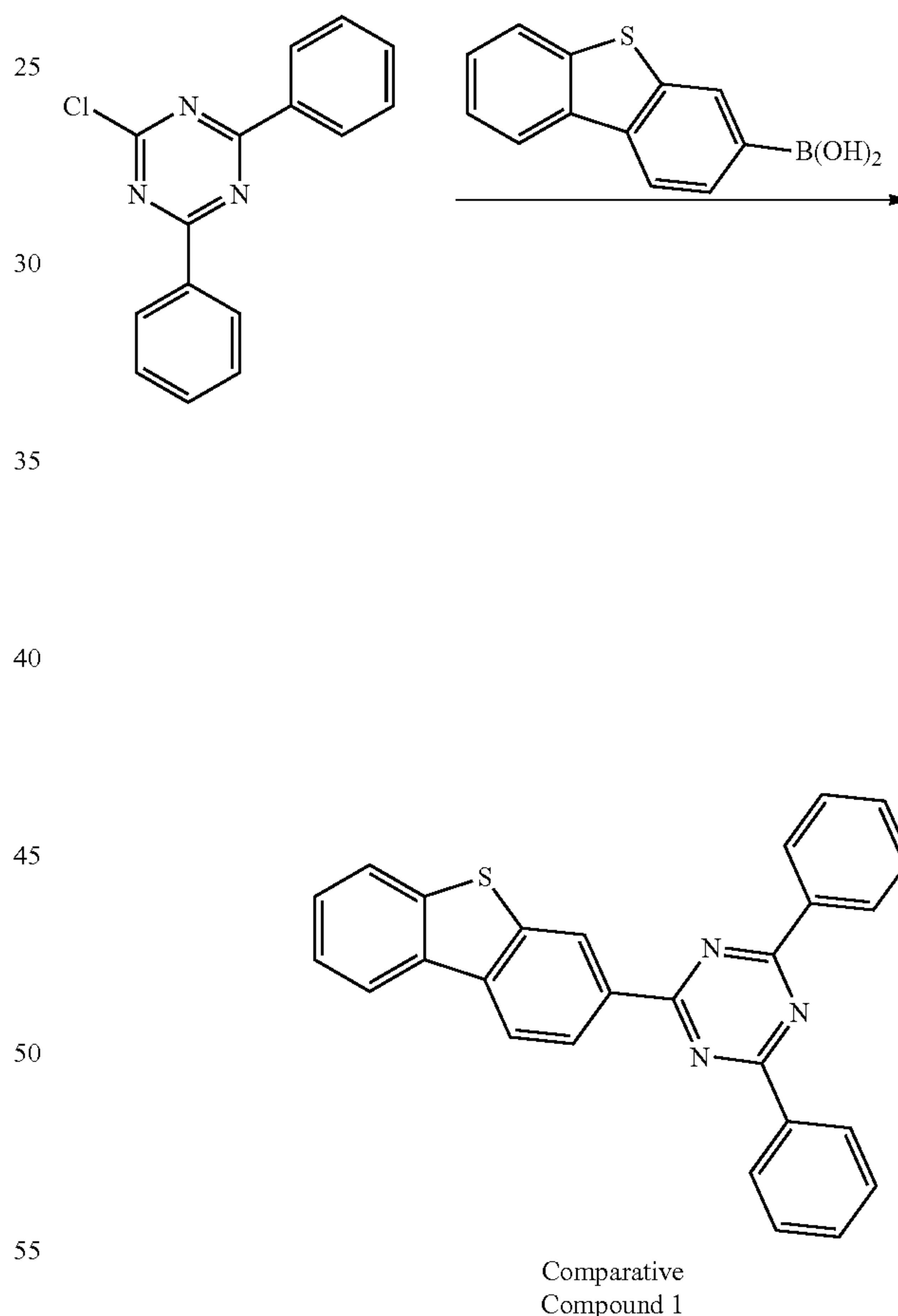
[Reaction Scheme 14]
