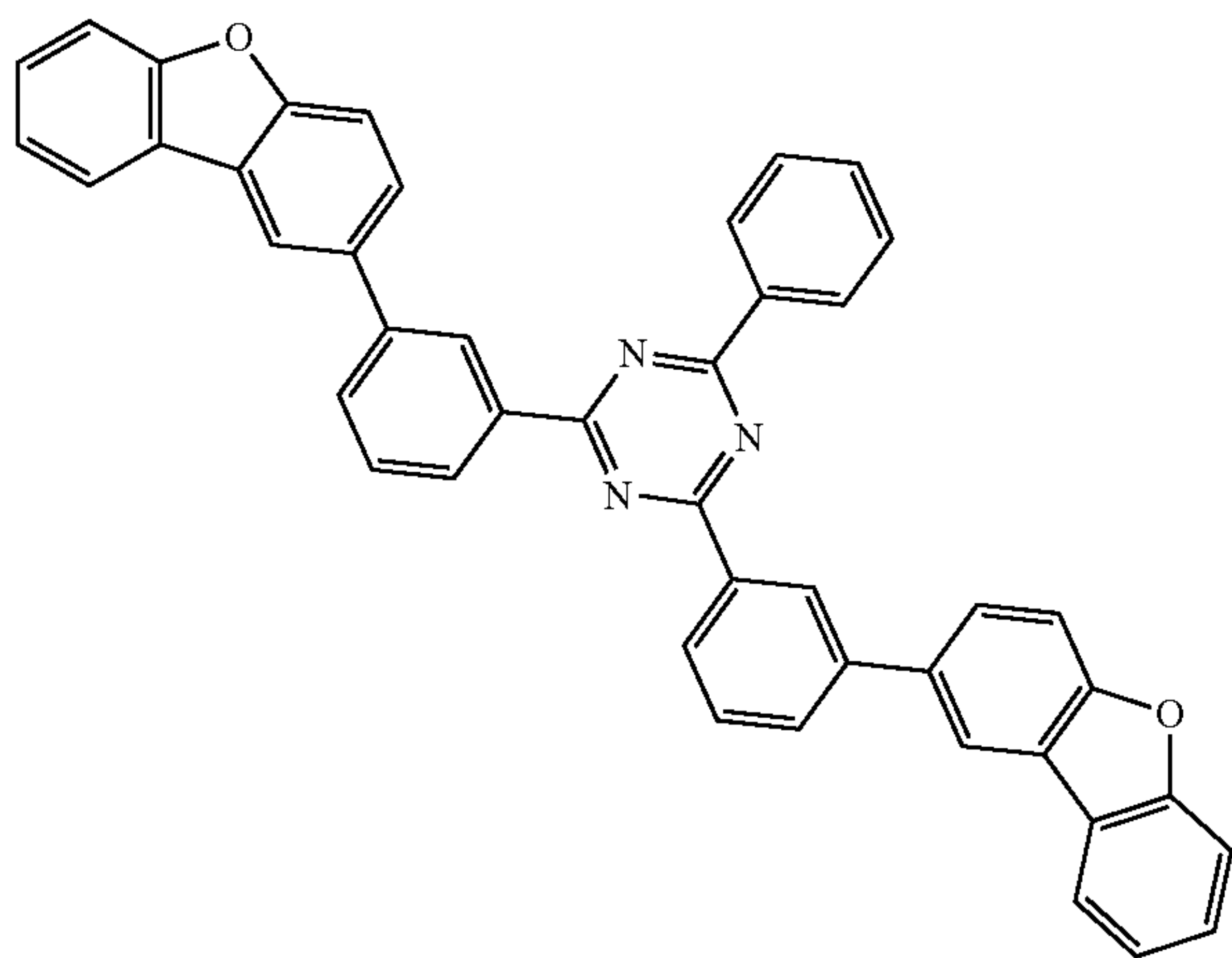
Comparative Compound 4
