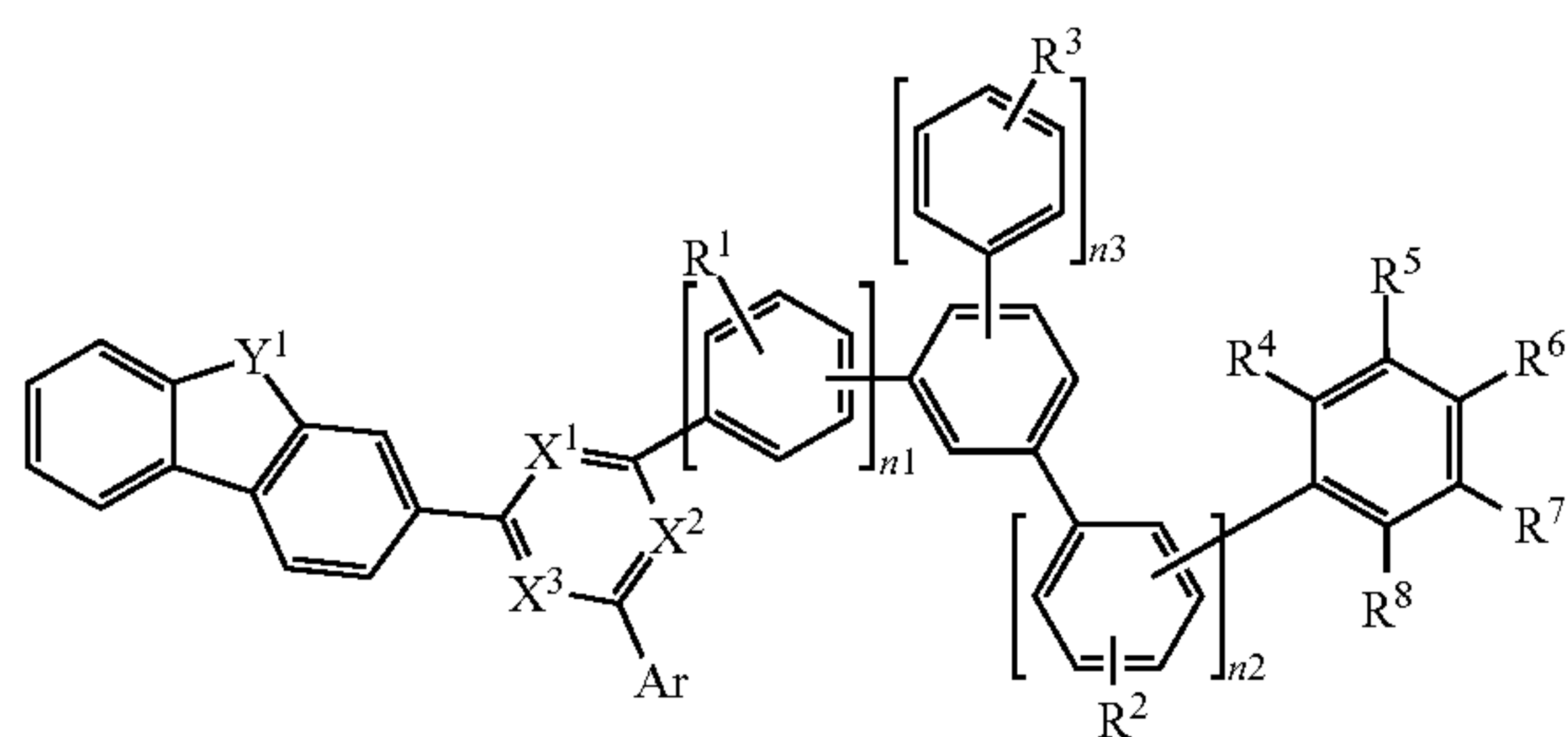
[Chemical Formula 1]
