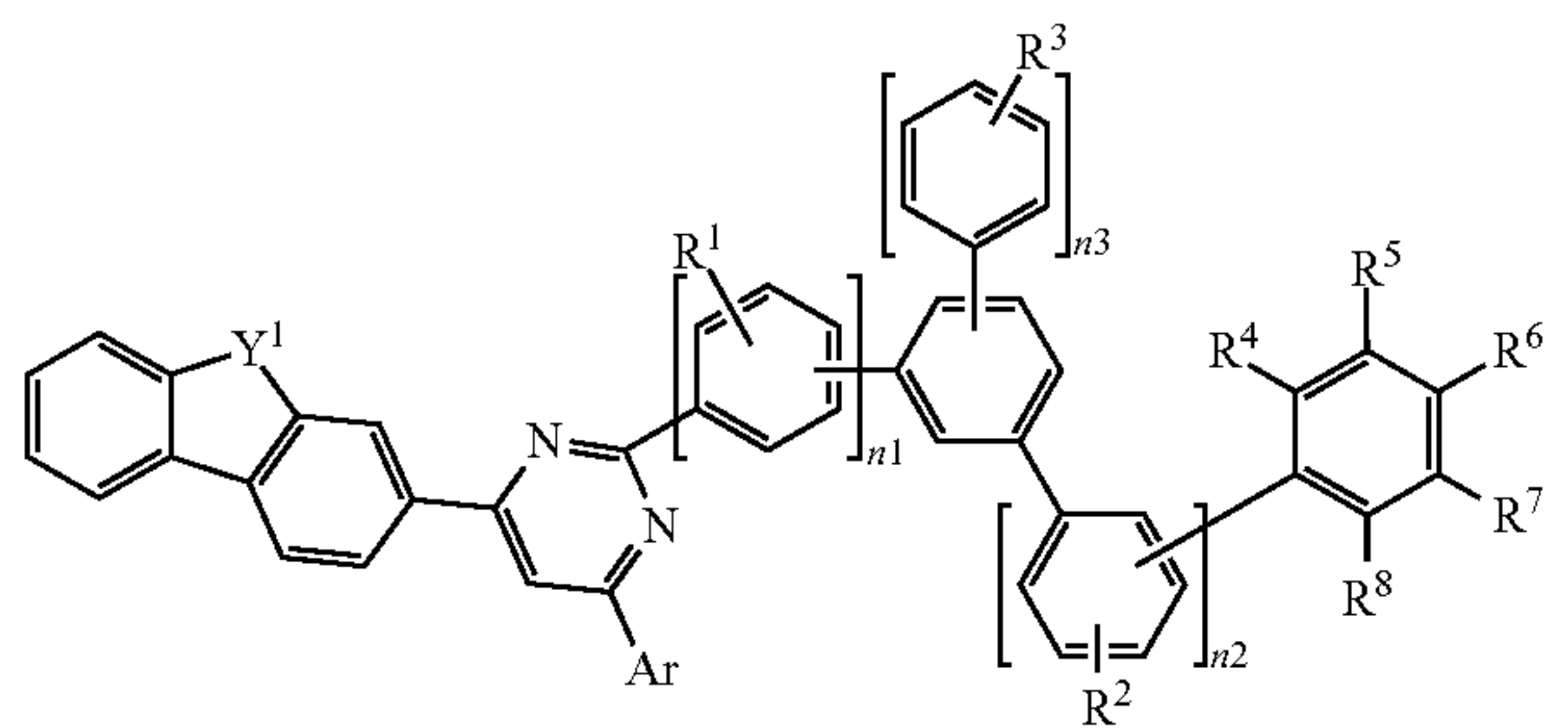
[Chemical Formula 1-II]
