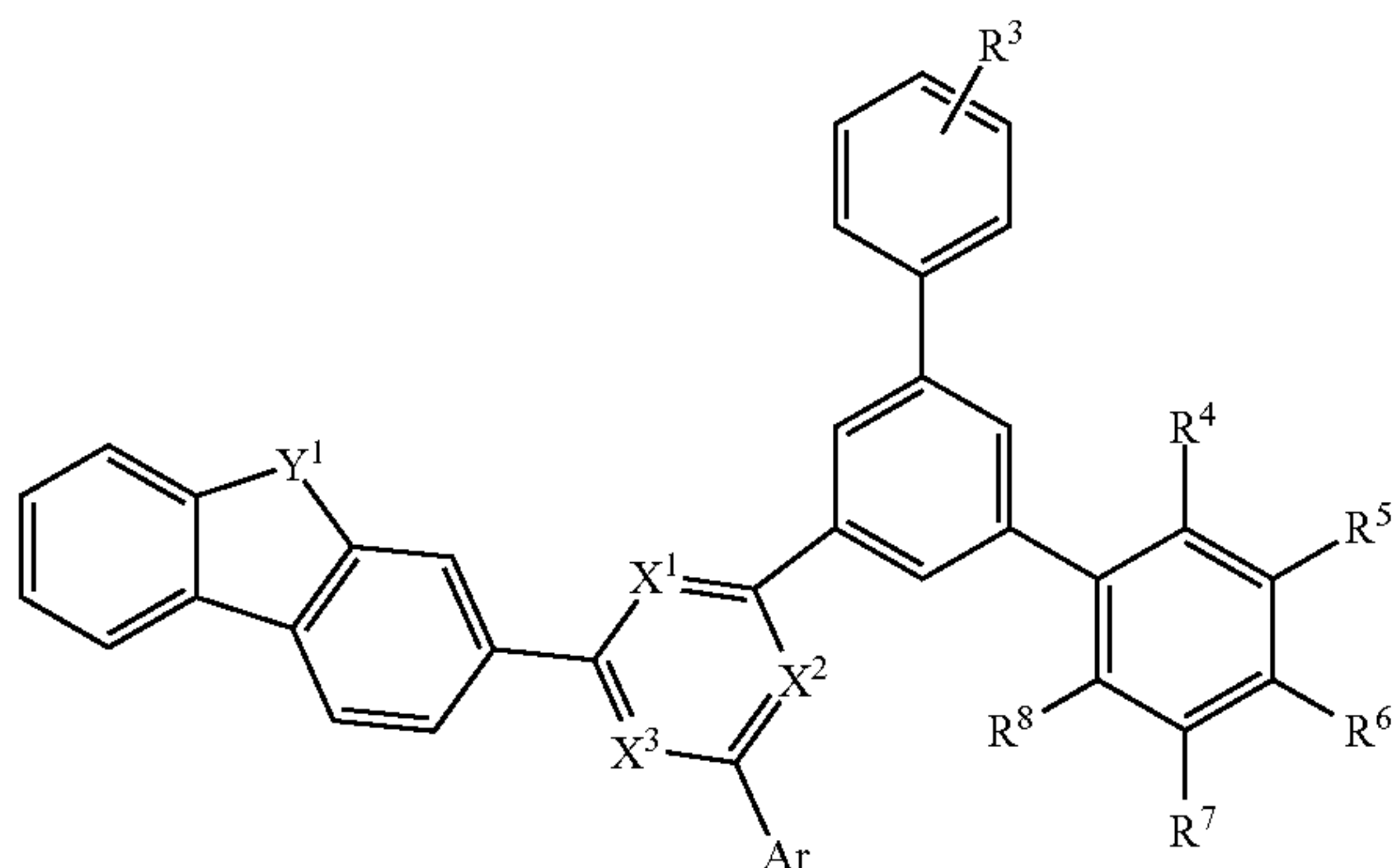
[Chemical Formula 1-1a]
