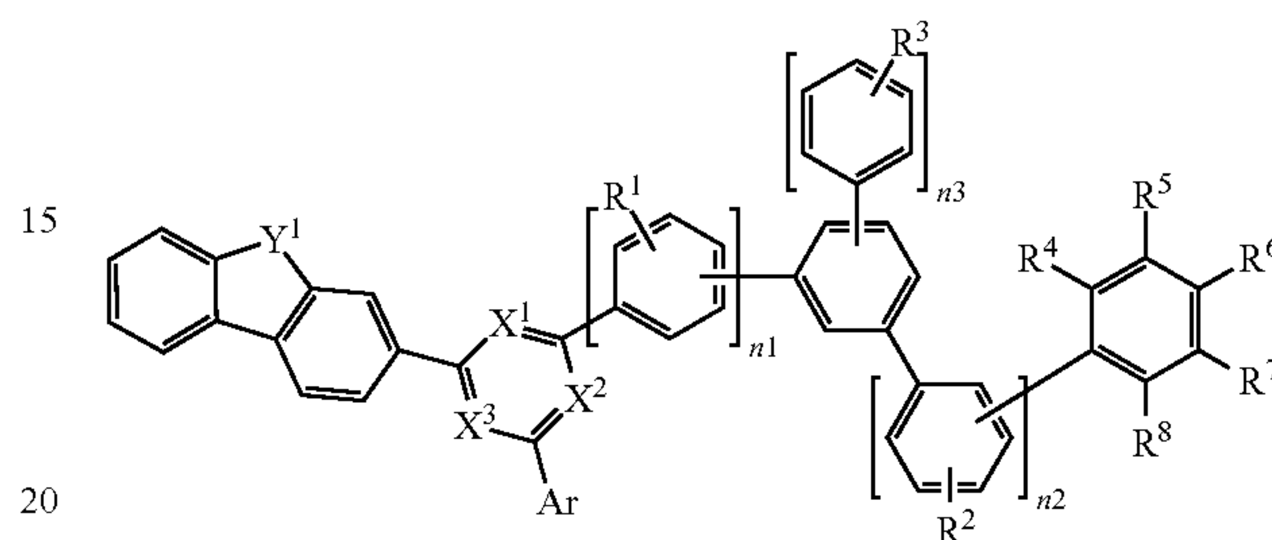
[Chemical Formula 1]
