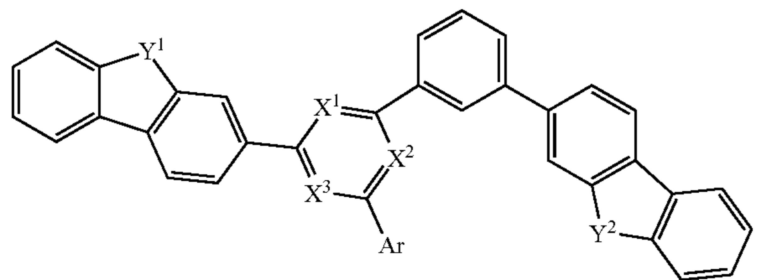
[Chemical Formula 1-2]
