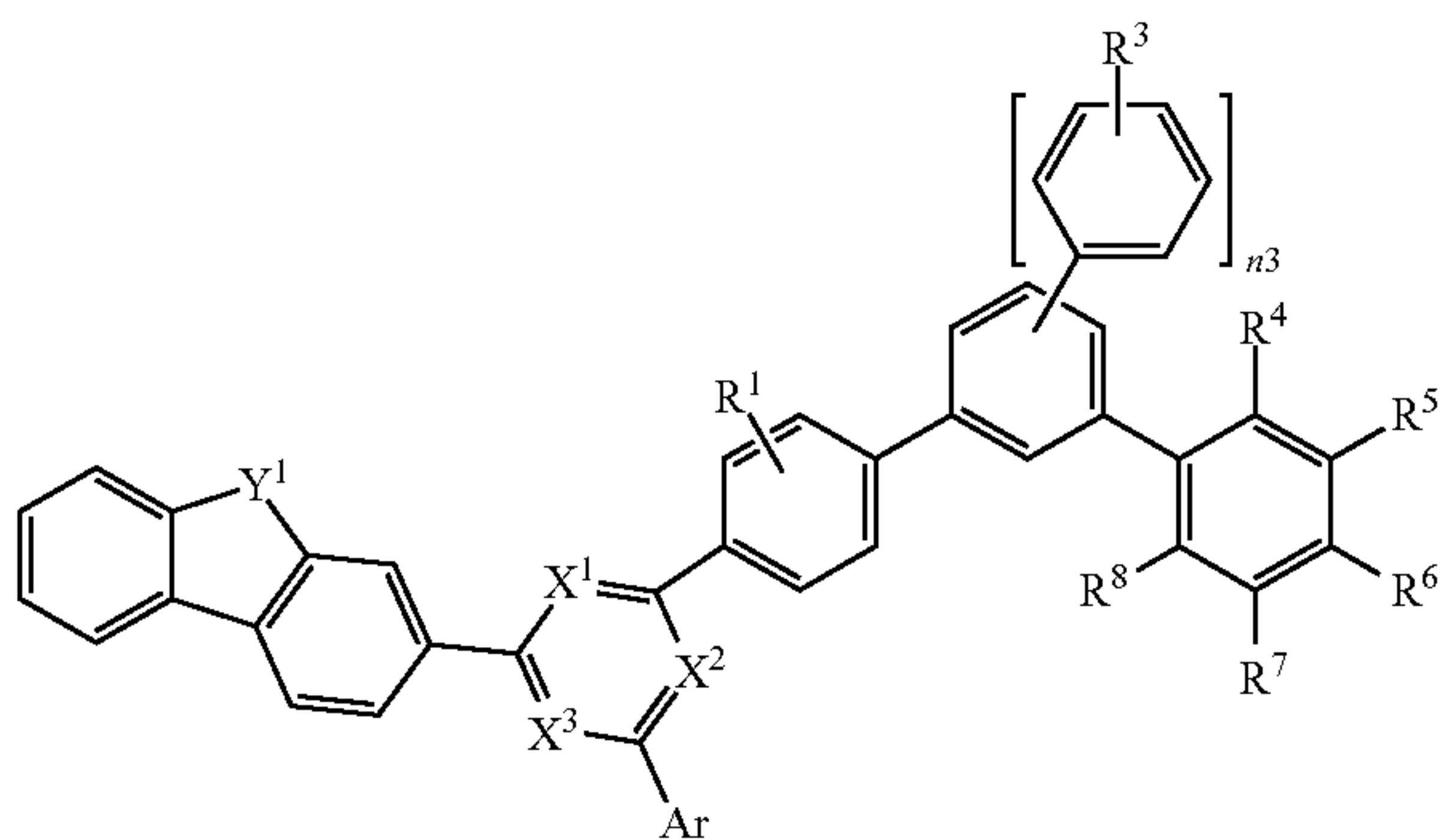
[Chemical Formula 1-3]
