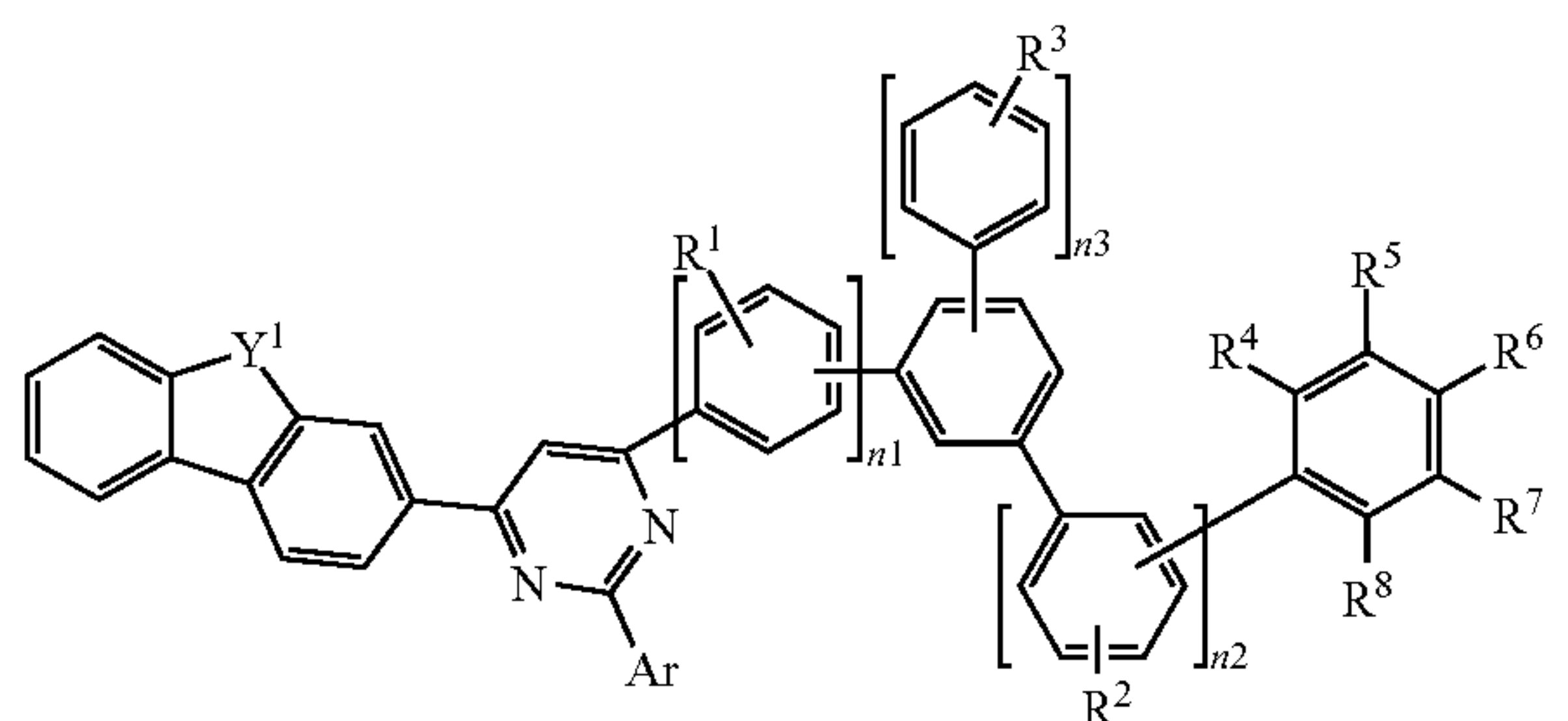
[Chemical Formula 1-III]
