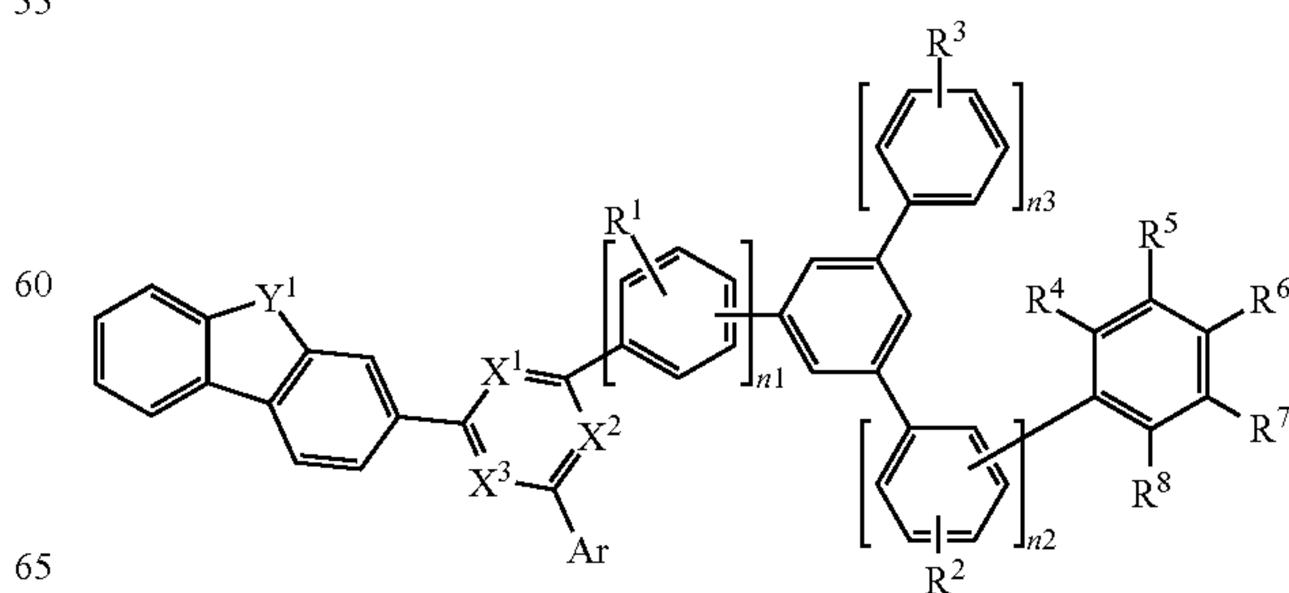
[Chemical Formula 1a]
