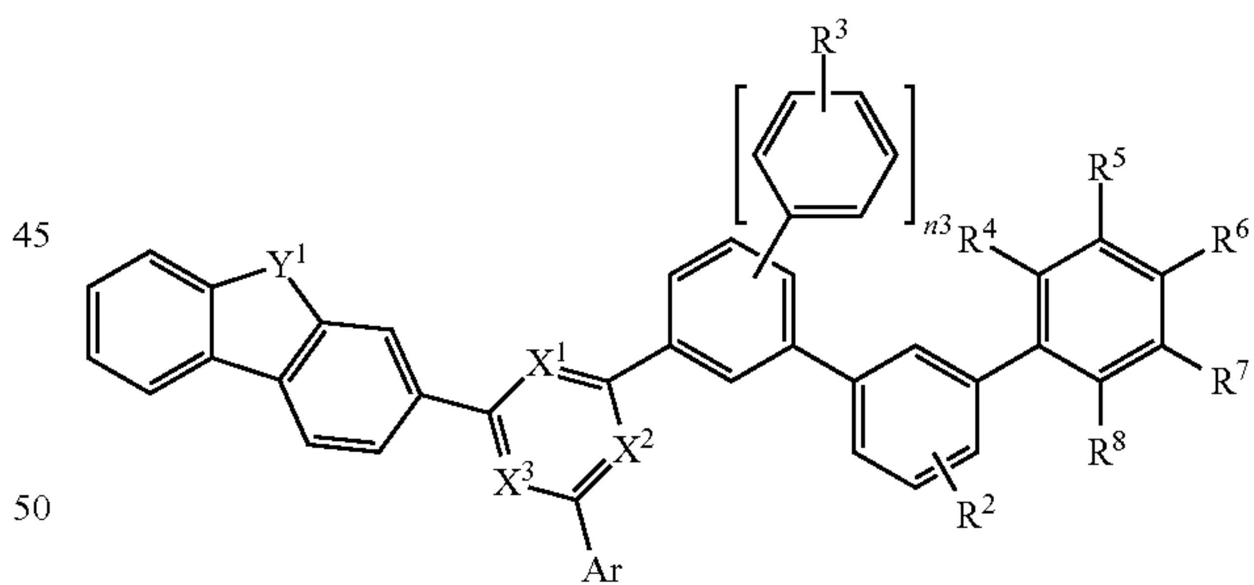
[Chemical Formula 1-5]
