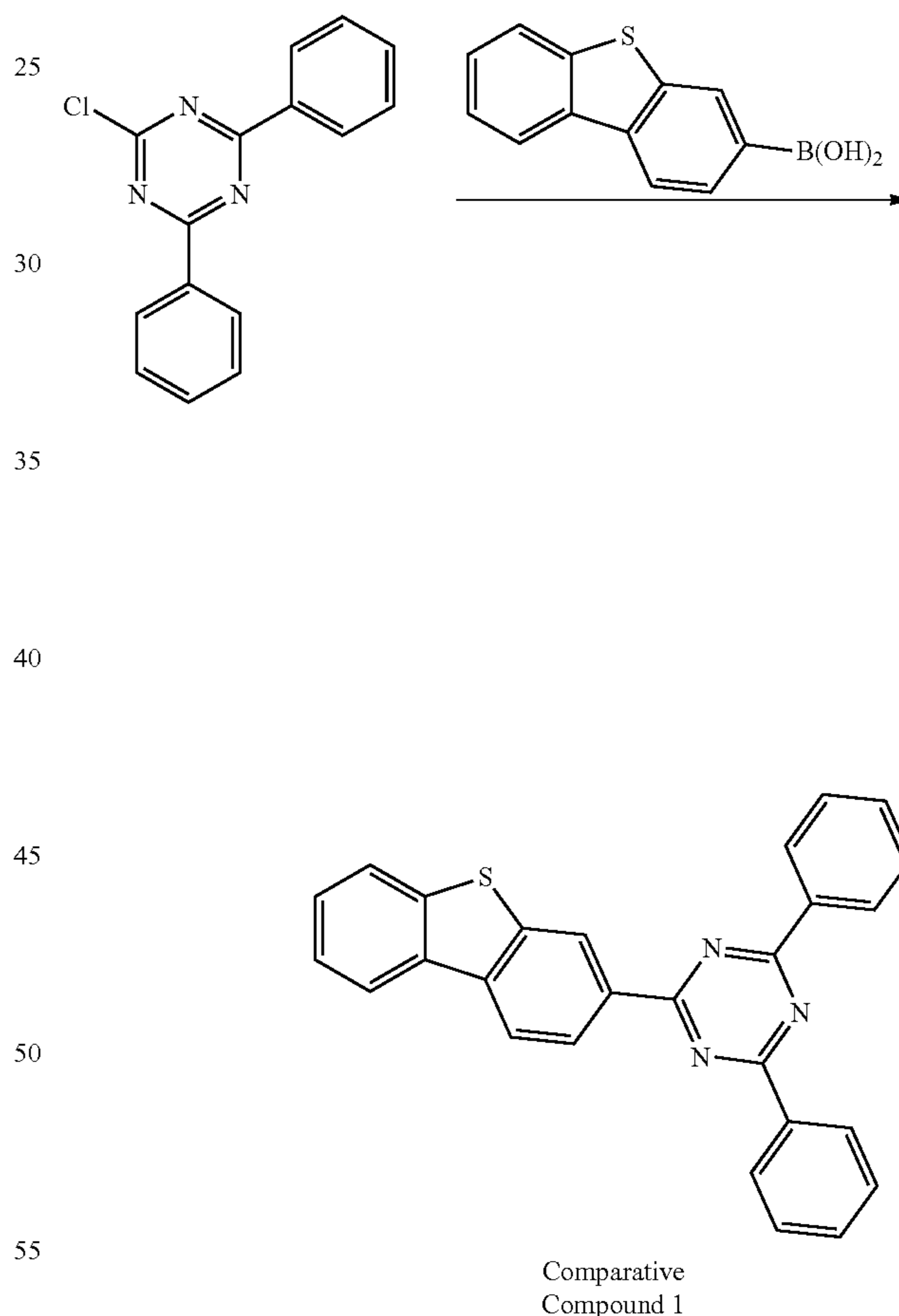
[Reaction Scheme 14]
