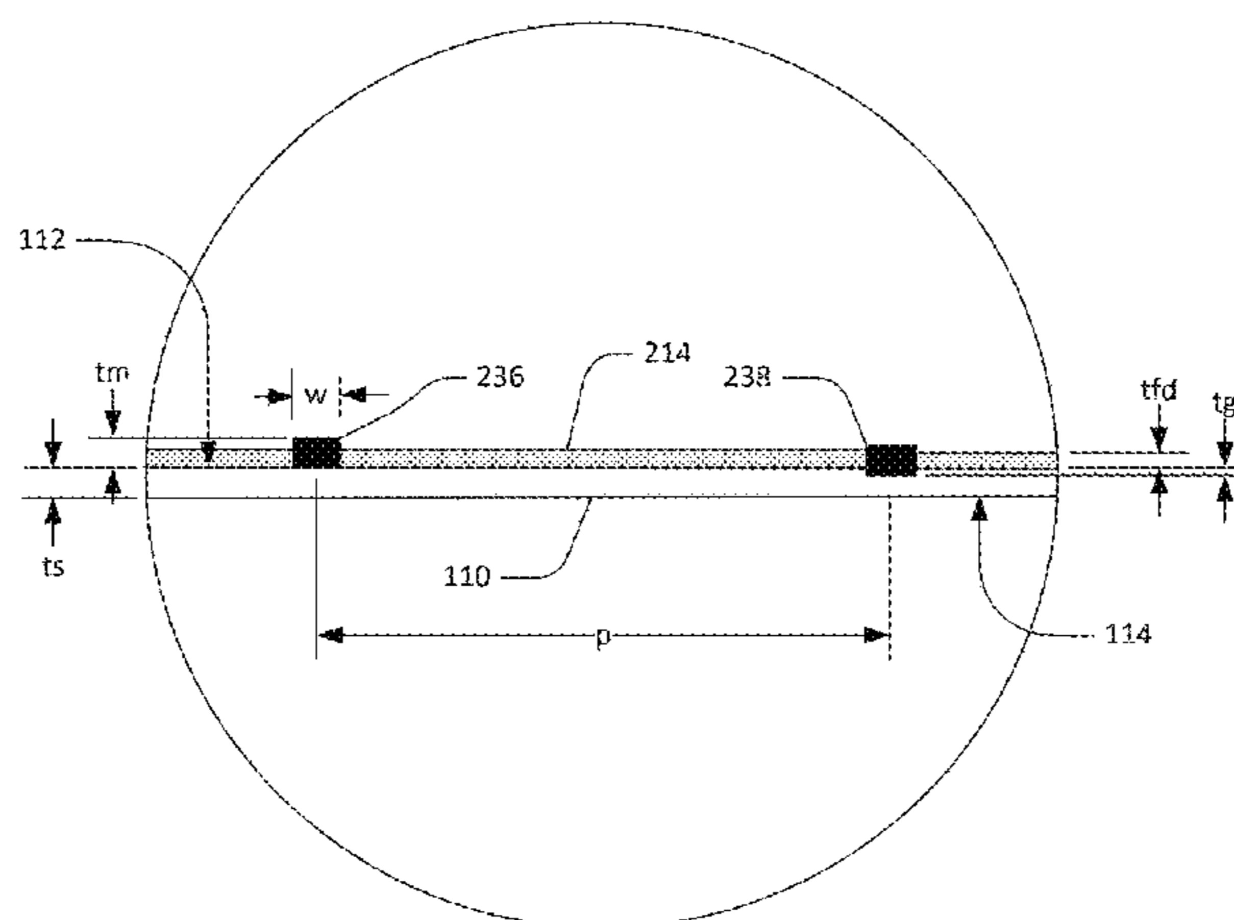
DETAIL C
