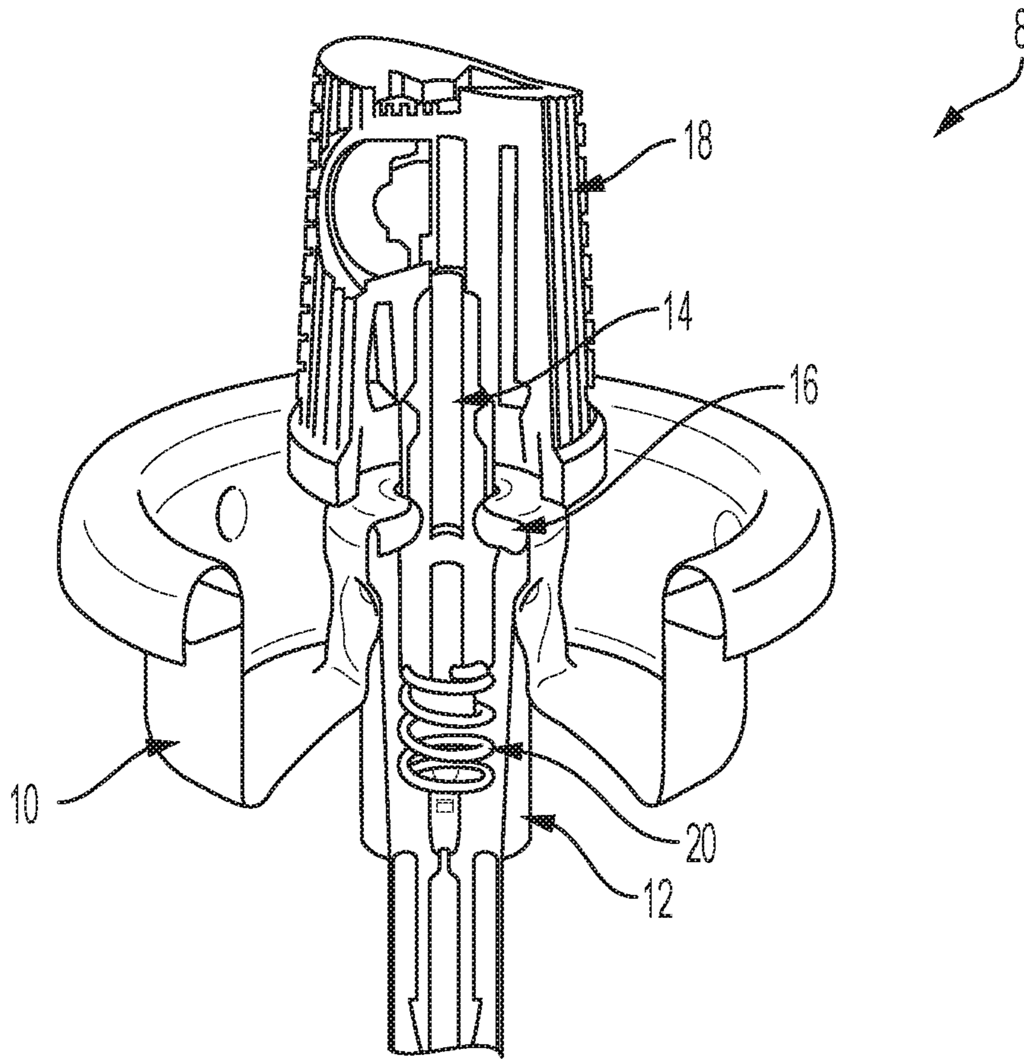
FIG. 1 PRIOR ART
