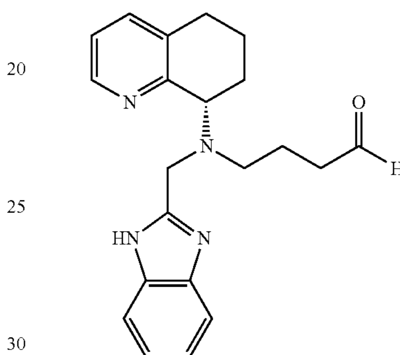
aldehyde D
