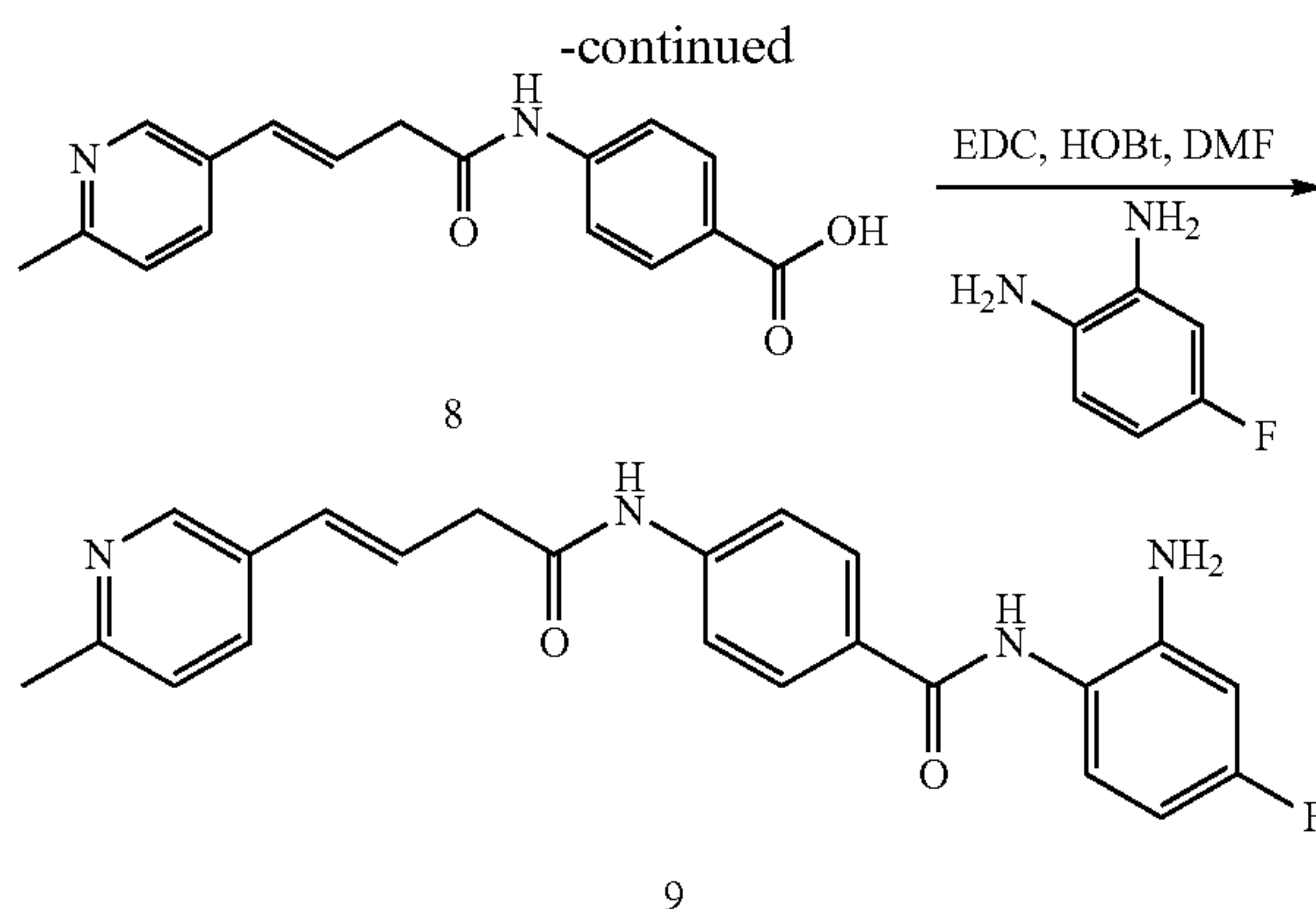
4-((E)-4-(6-methylpyridin-3-yl)but-3-enamido)benzoic acid (8)
