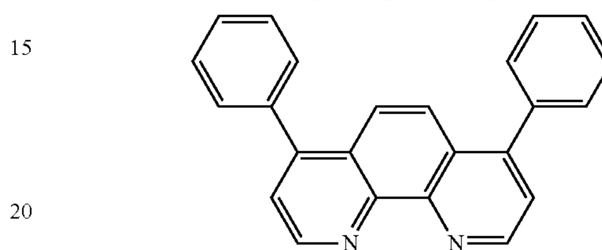
BPhen
