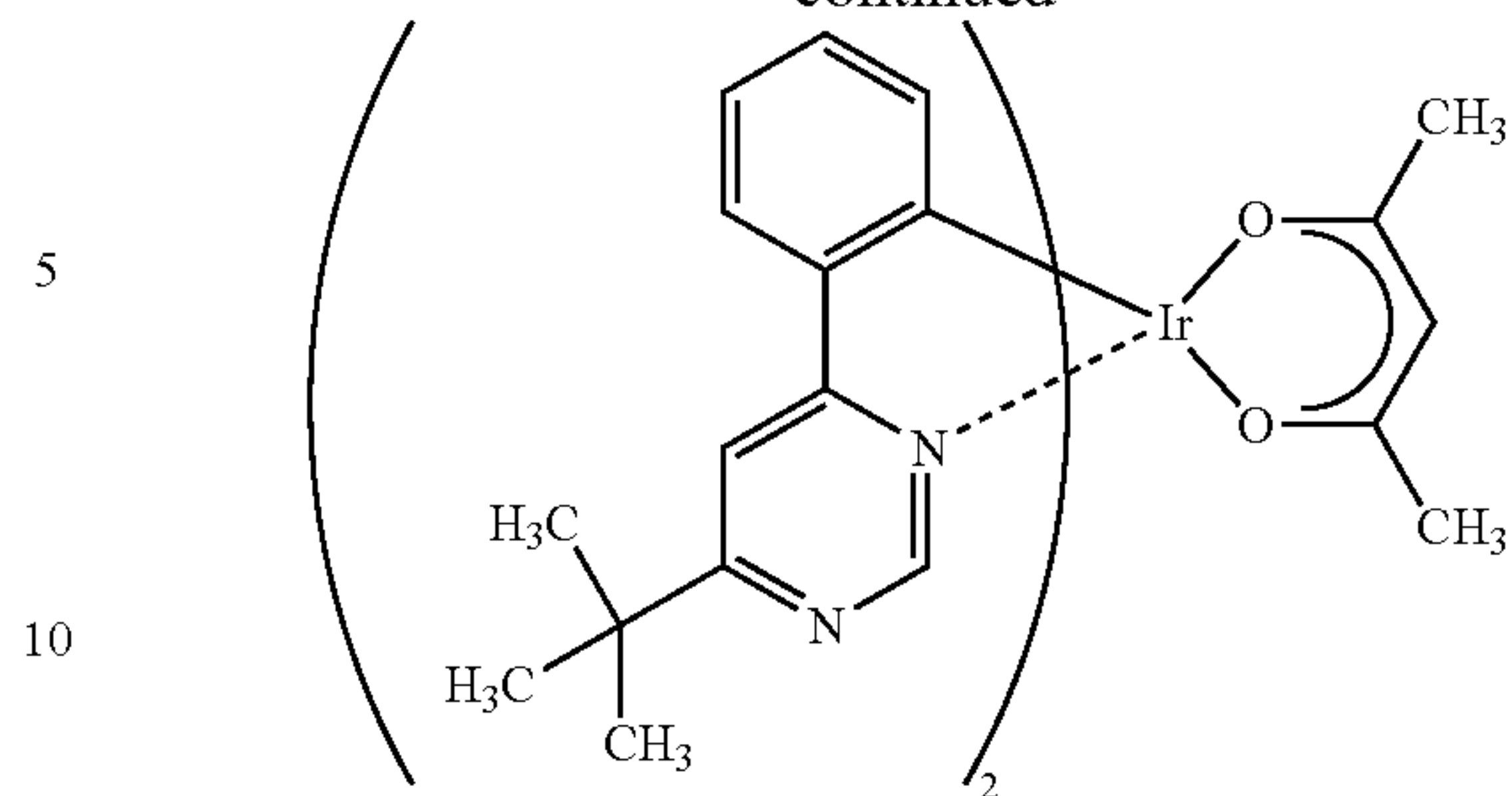
[Ir(tBuppm) 2 (acac)]
