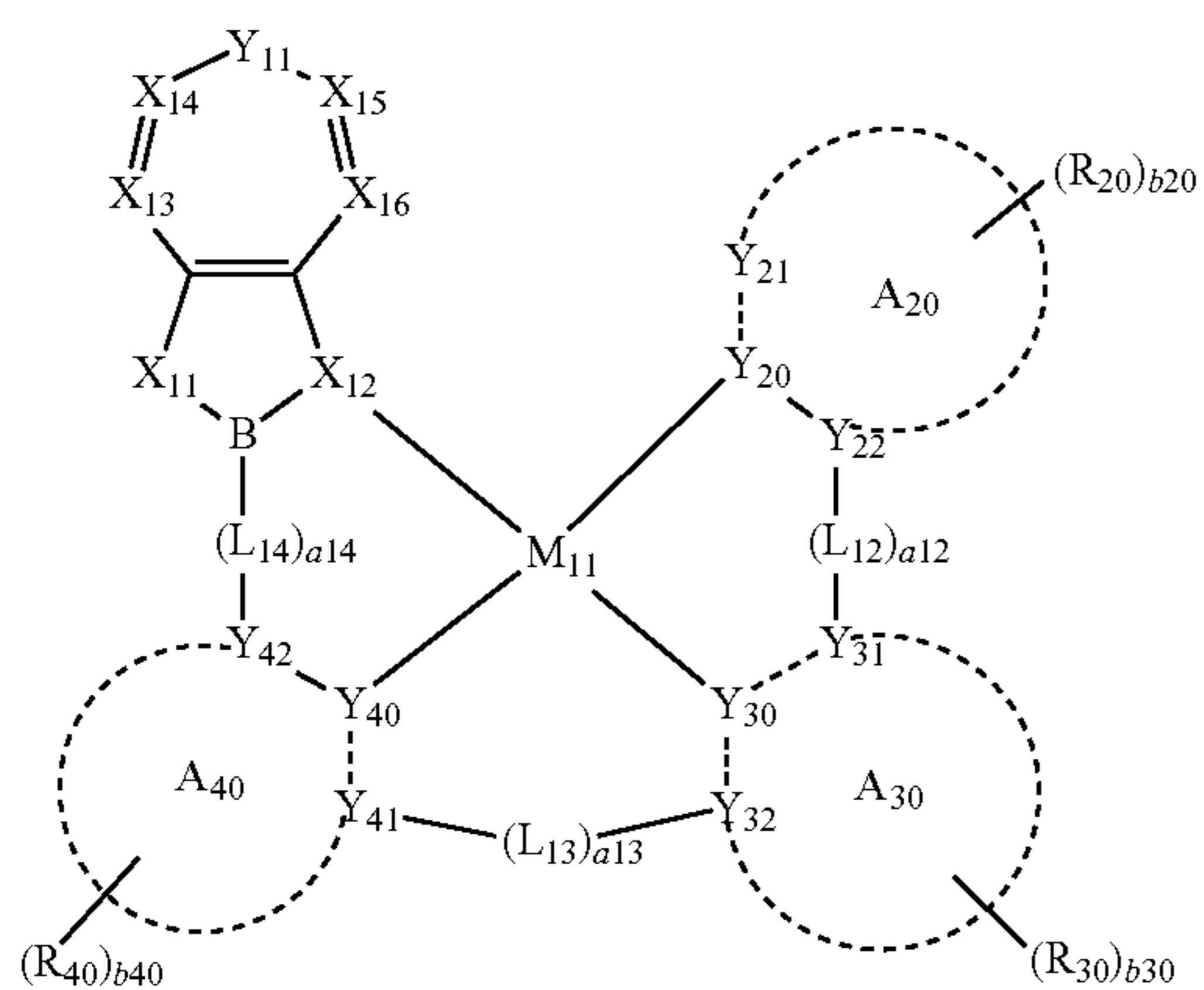
Formula 1G
