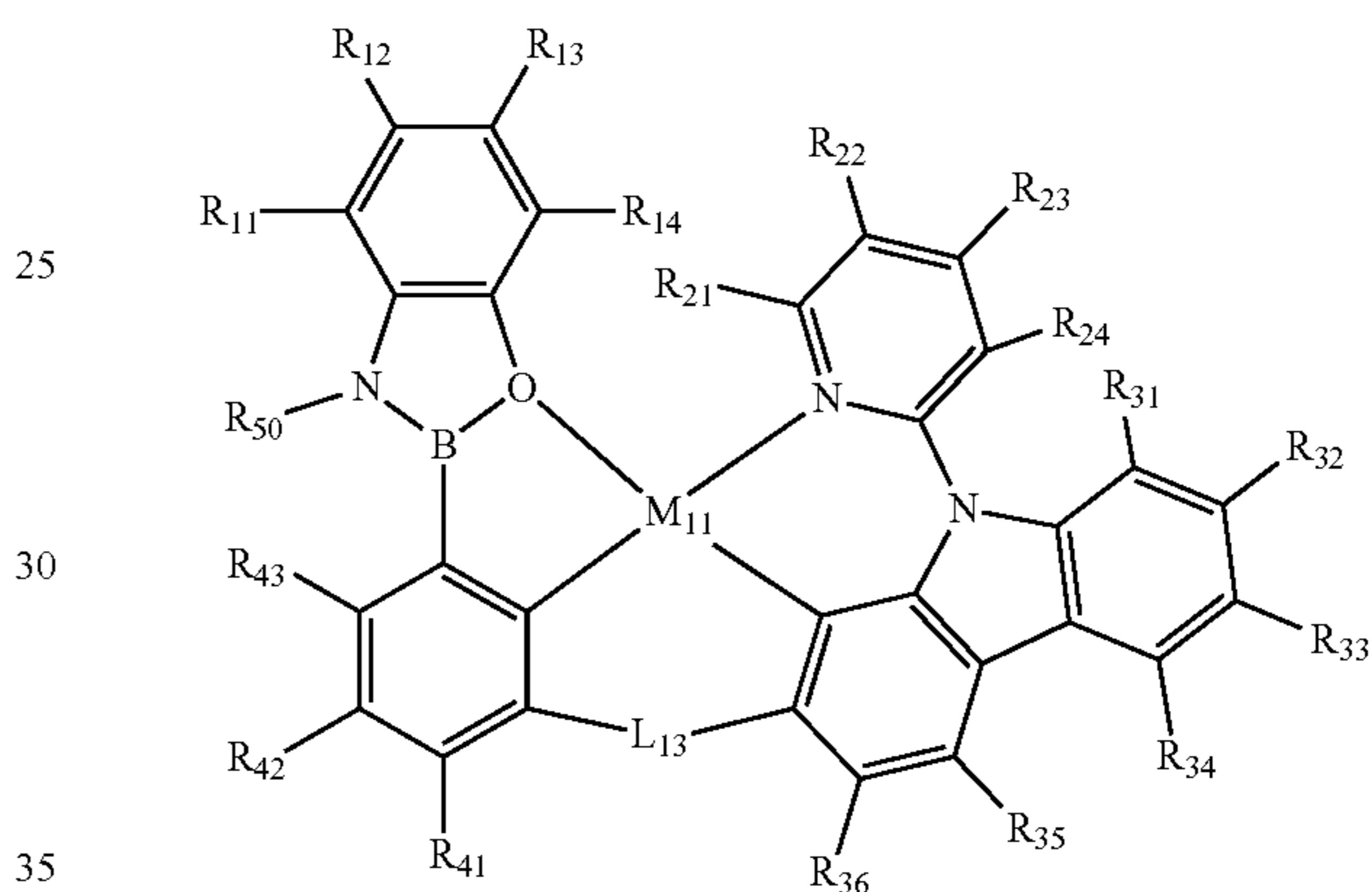
Formula 1G
