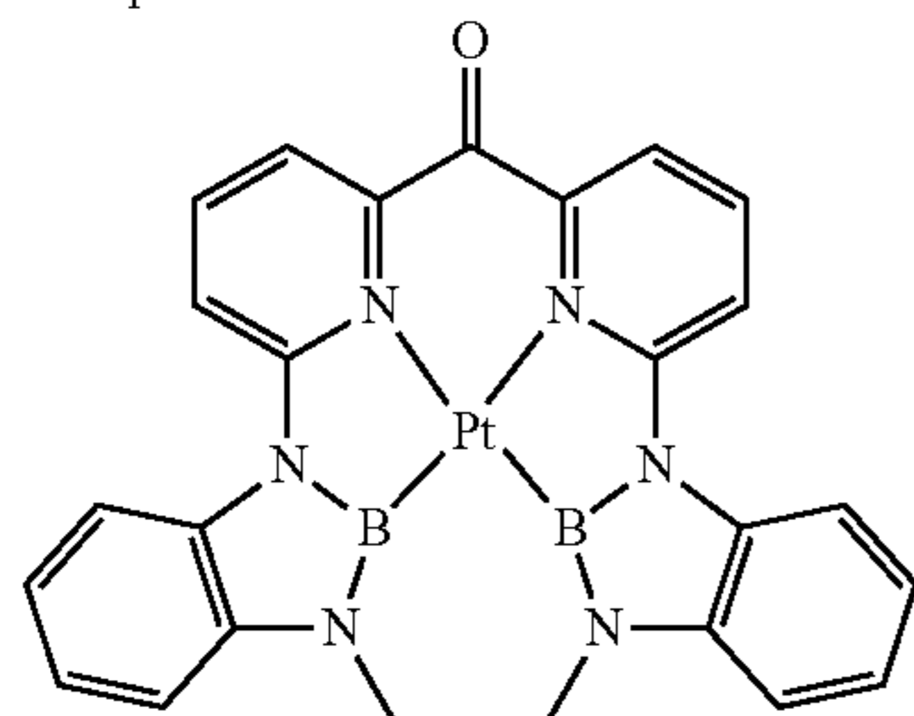
Compound B
