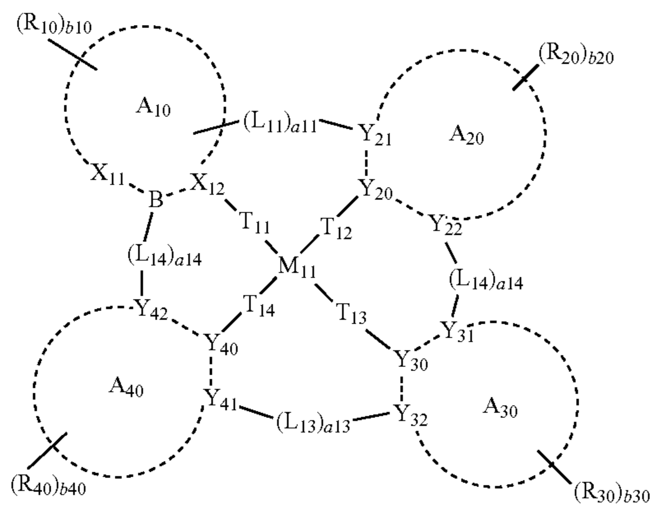
Formula 1
