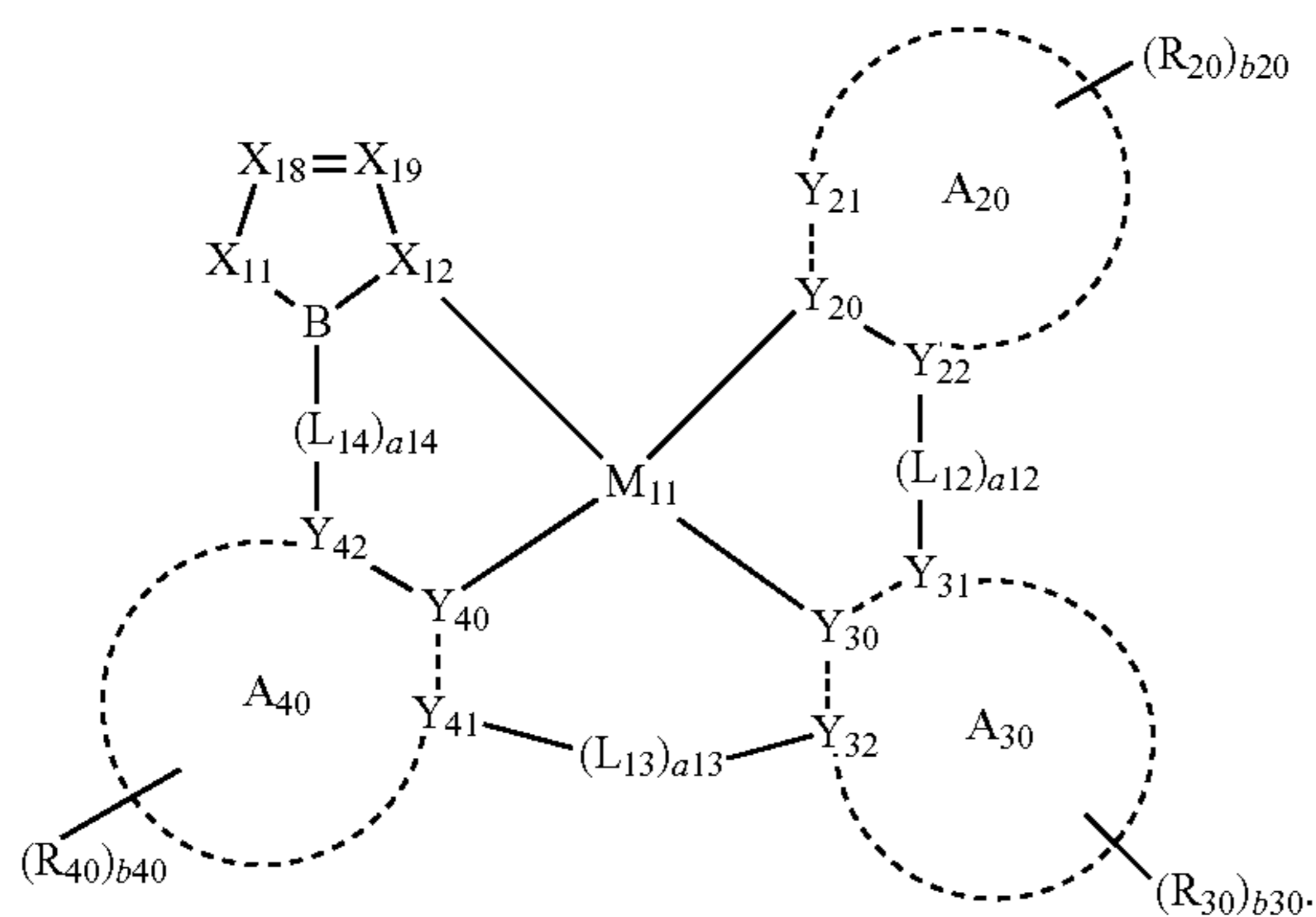
Formula 1G
