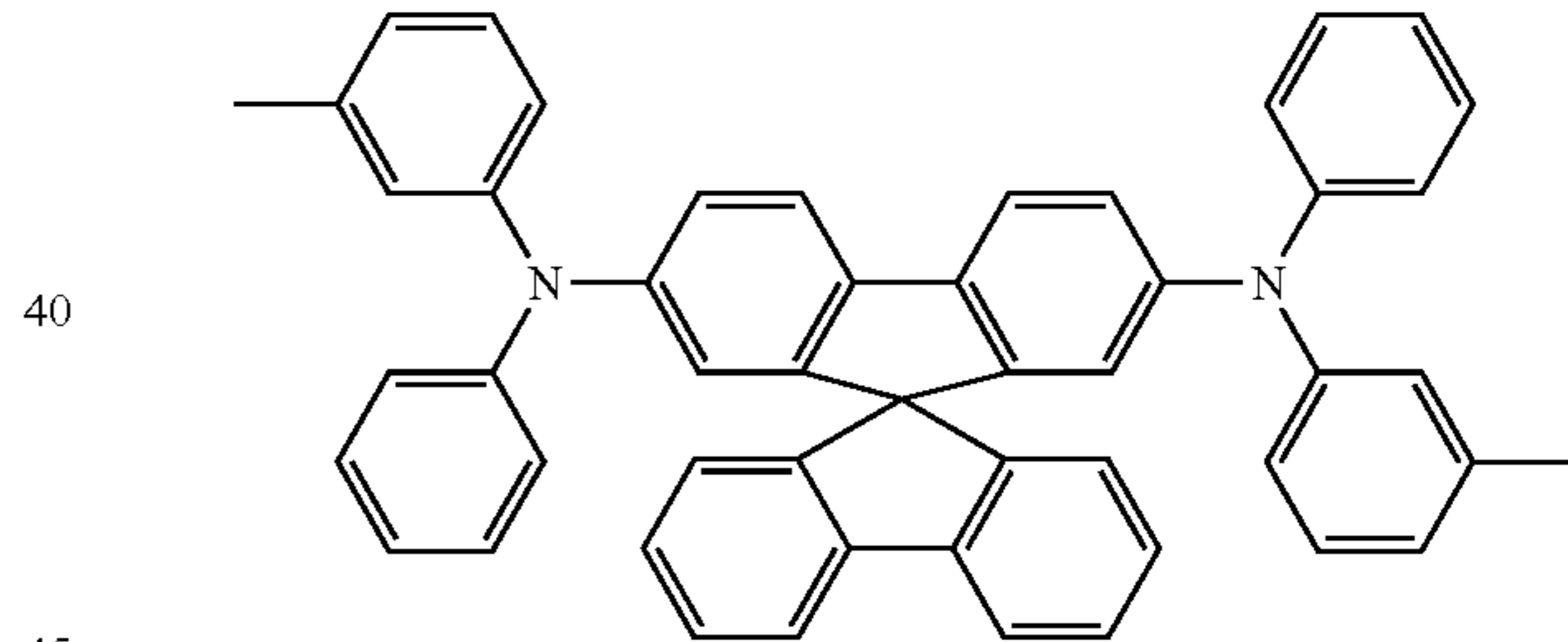
Spiro-TPD
