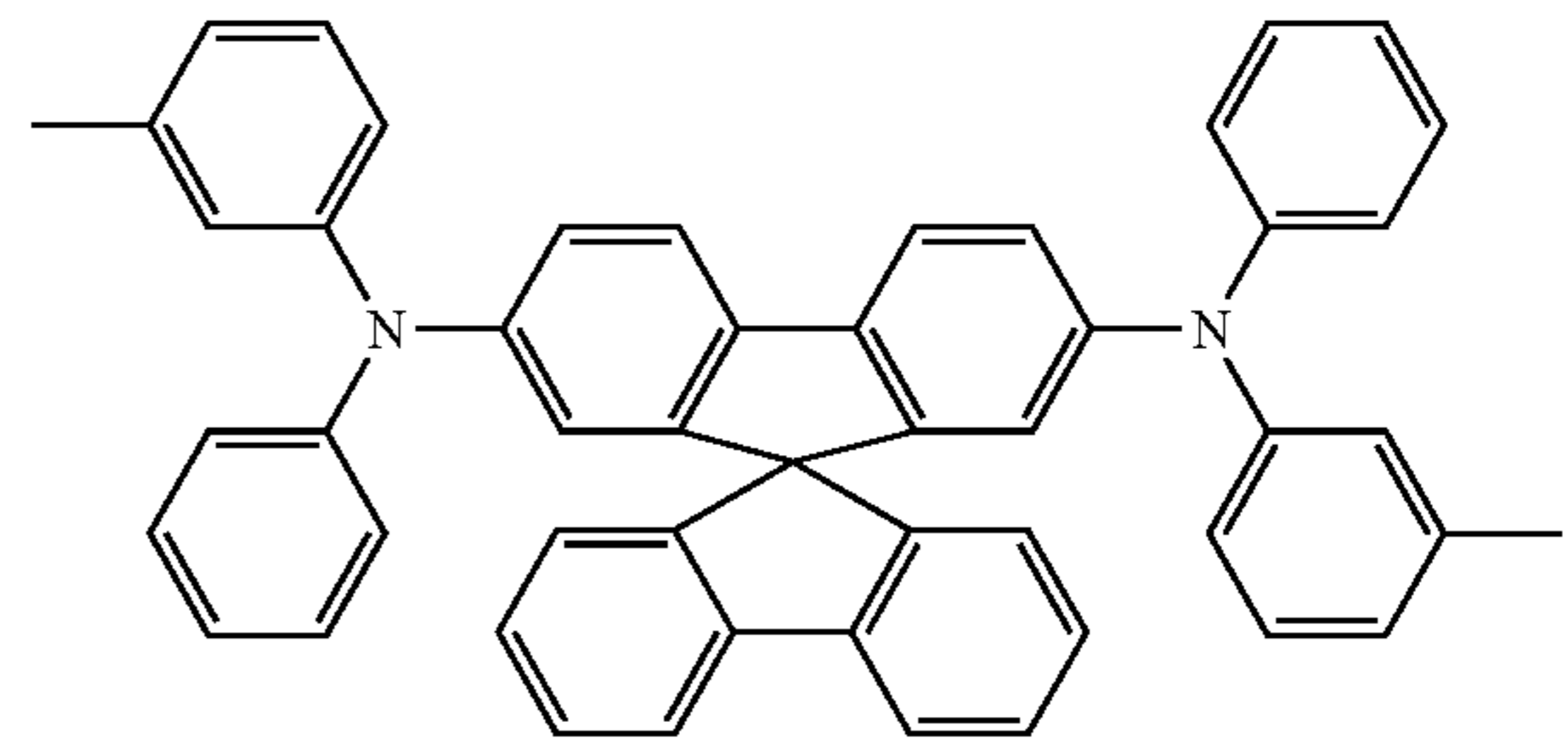
Spiro-TPD
