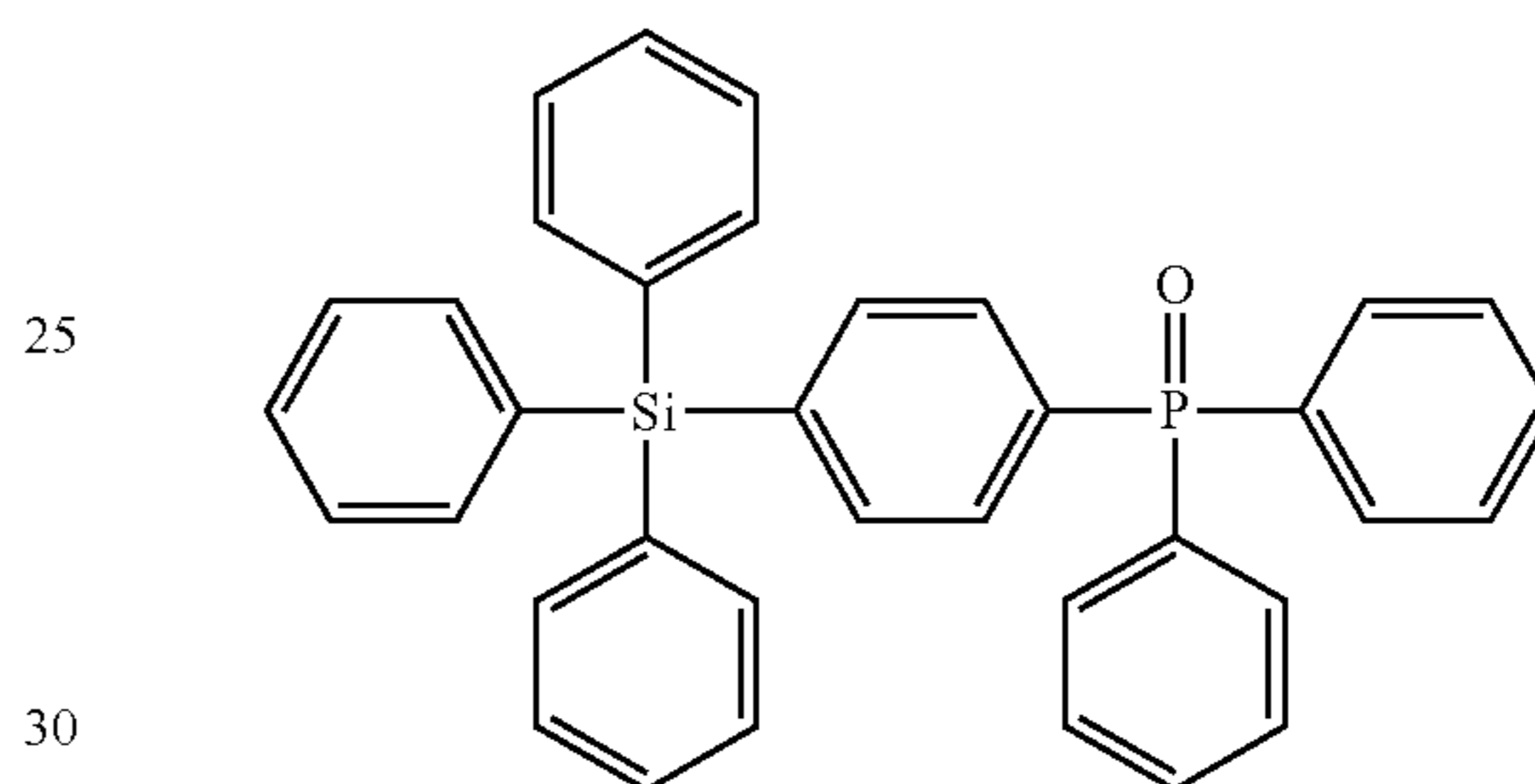
TSP01
