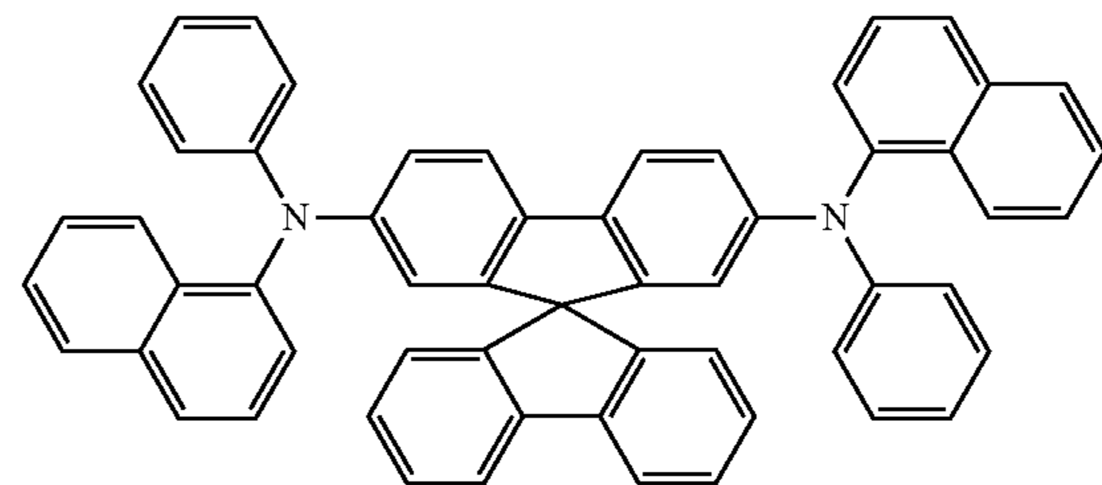
Spiro-NPB
