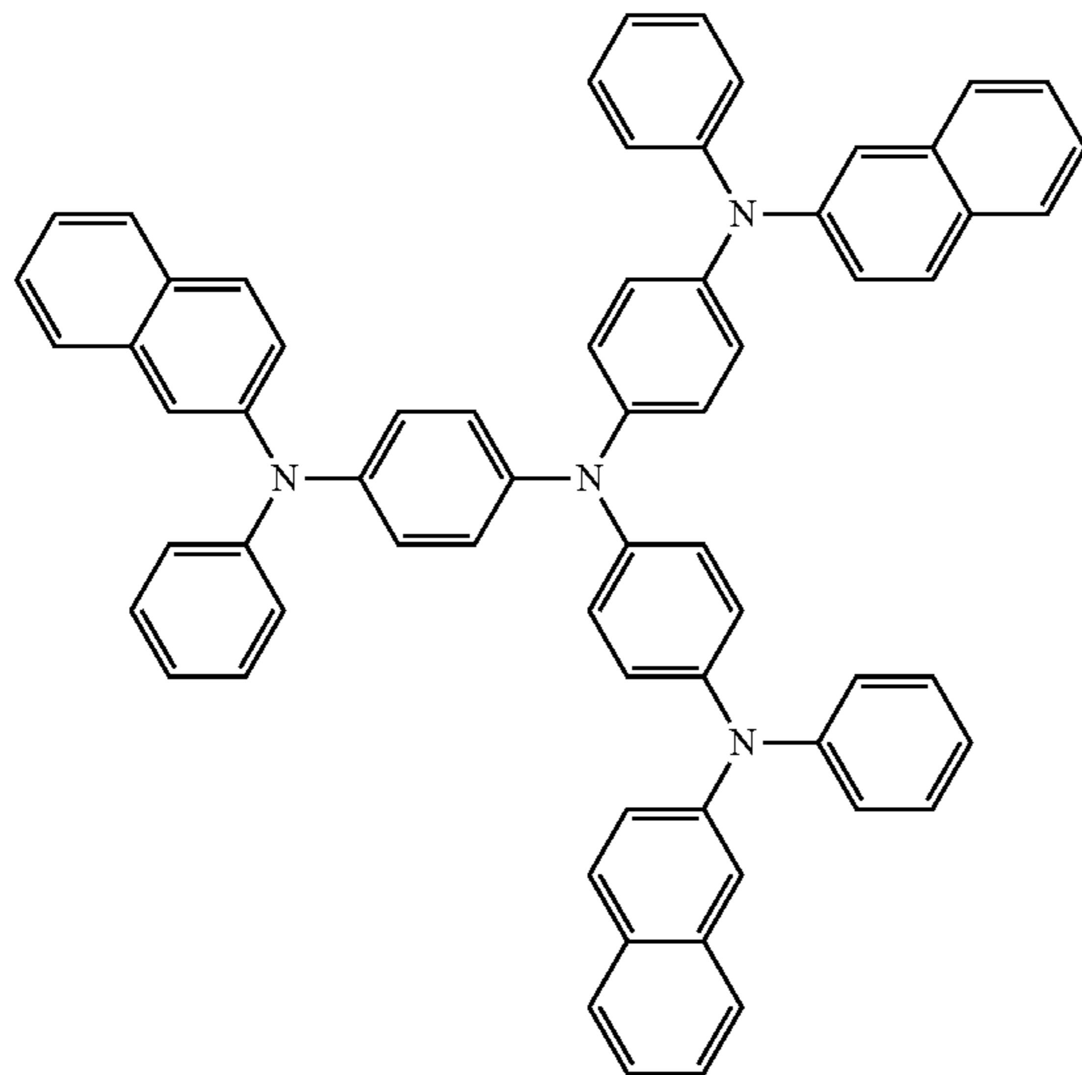
2-TNATA
