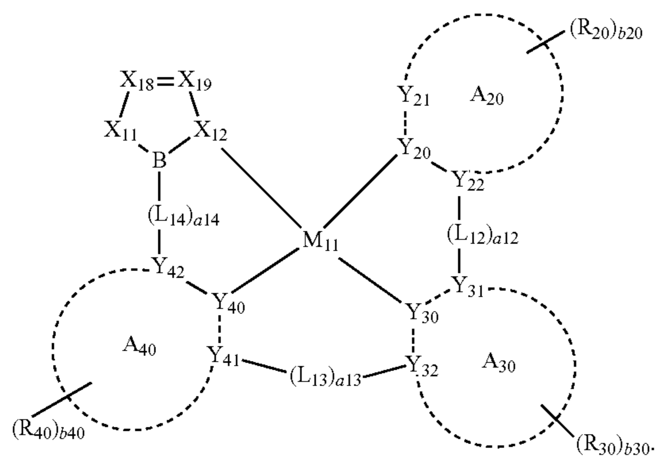
Formula 1G
