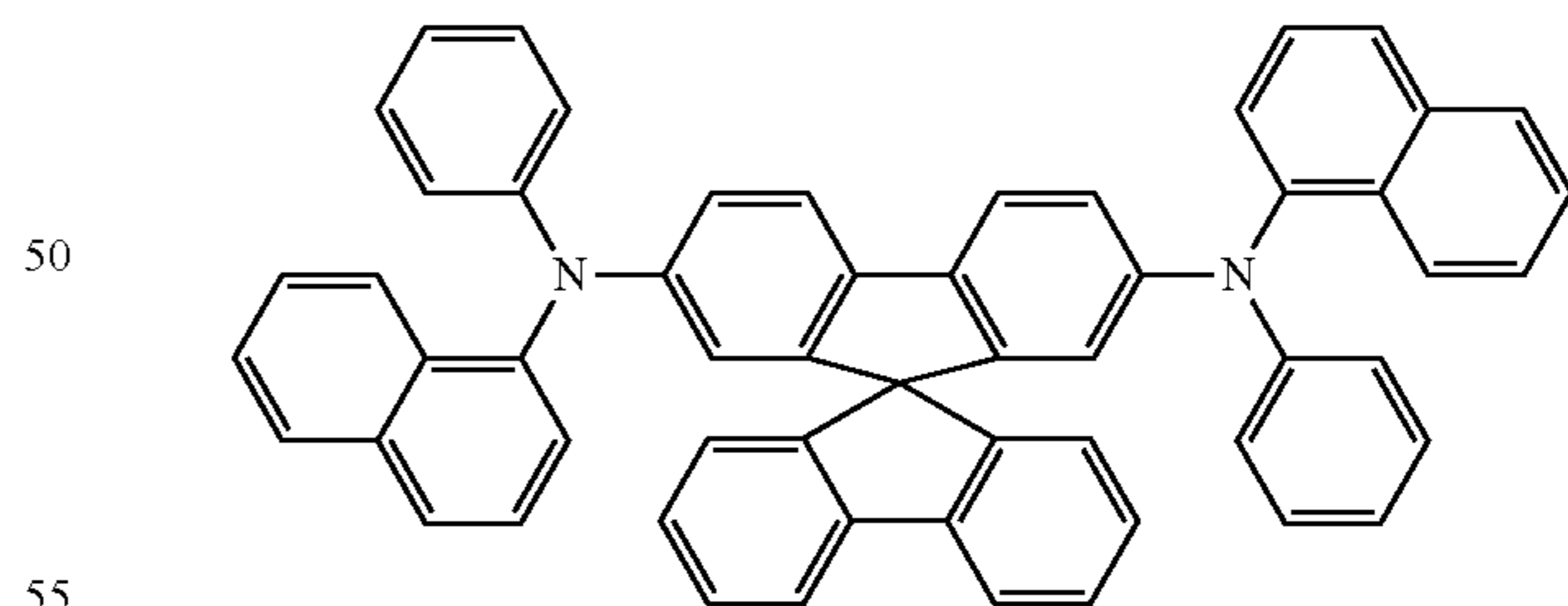
Spiro-NPB
