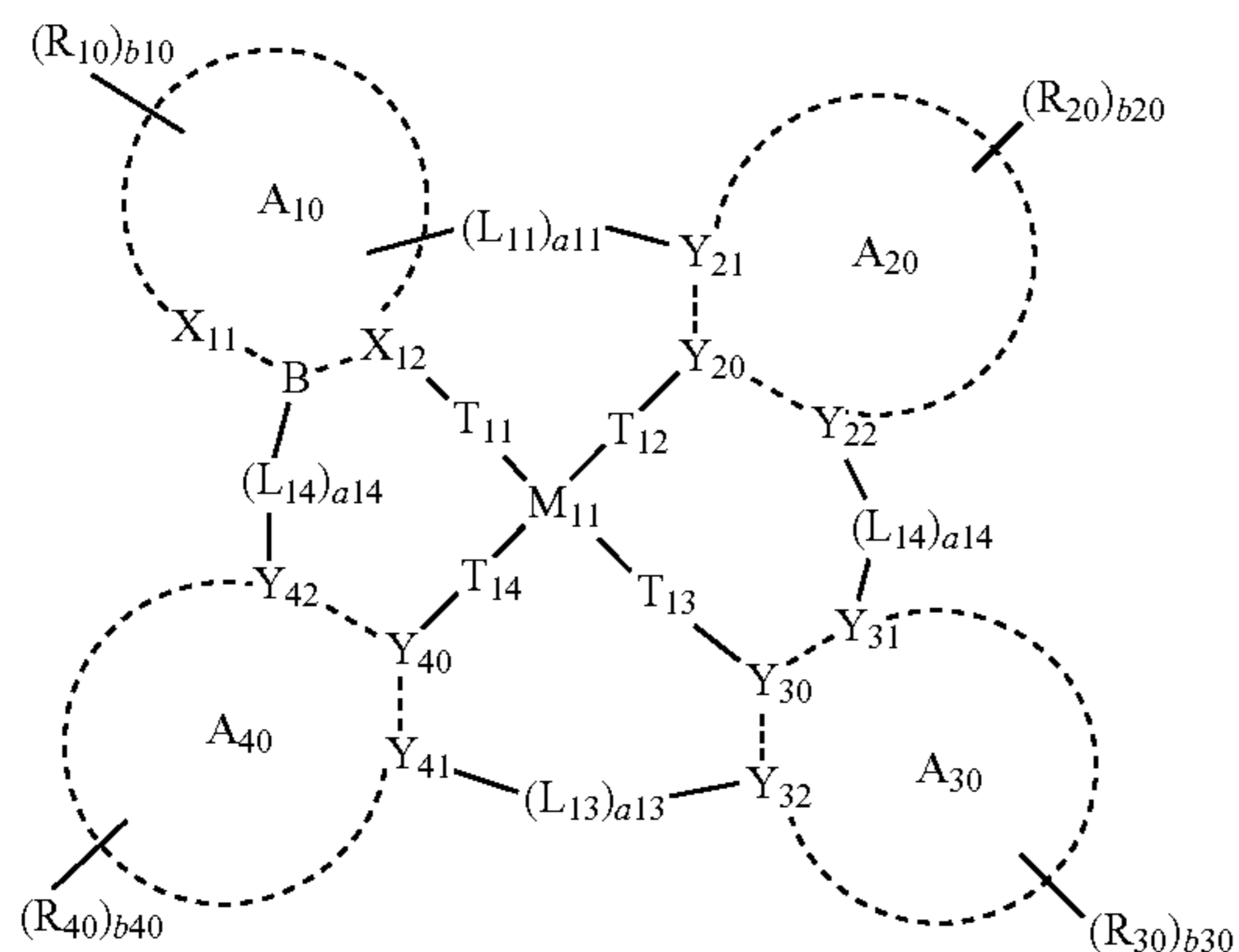
Formula 1
