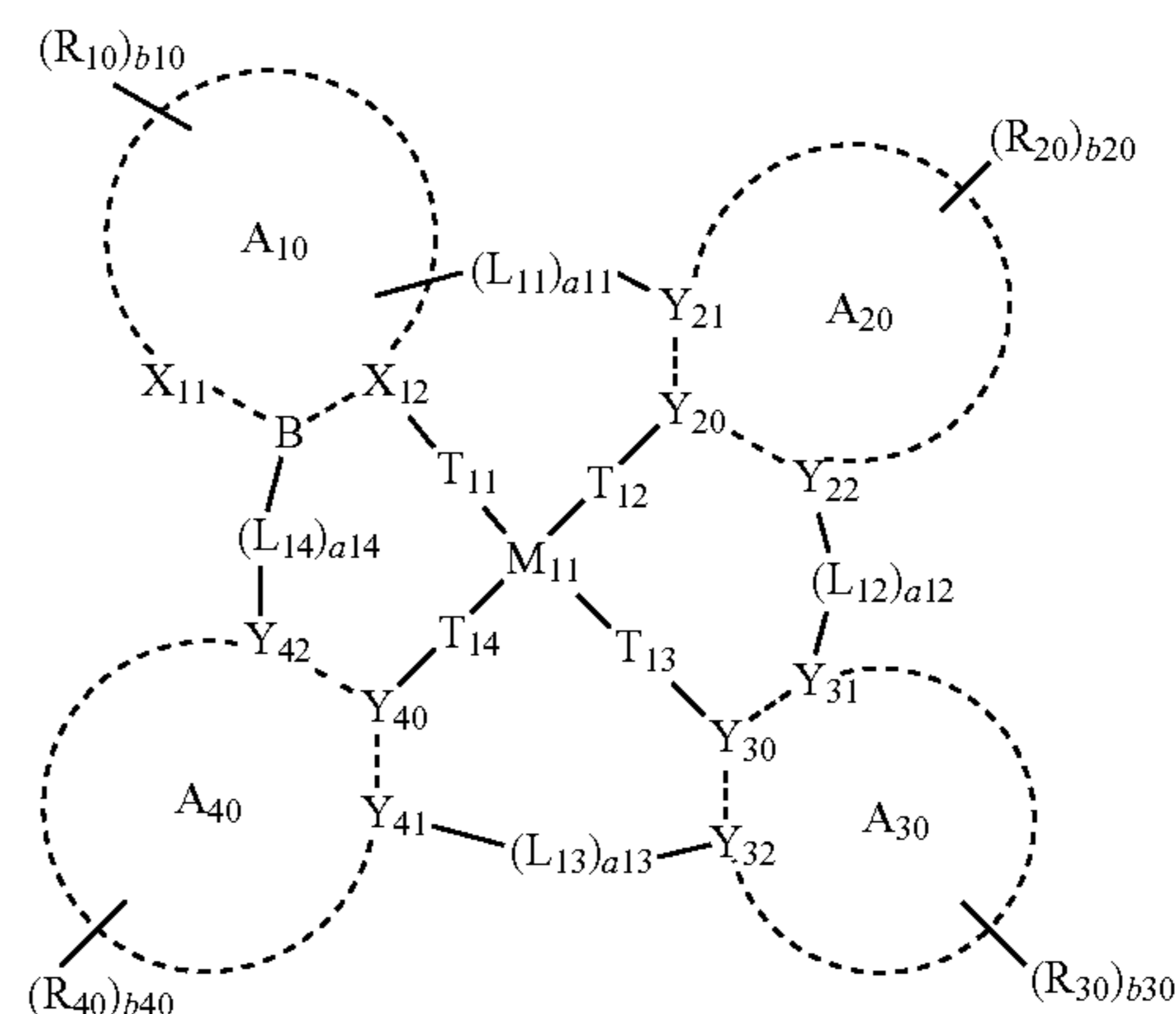
Formula 1
