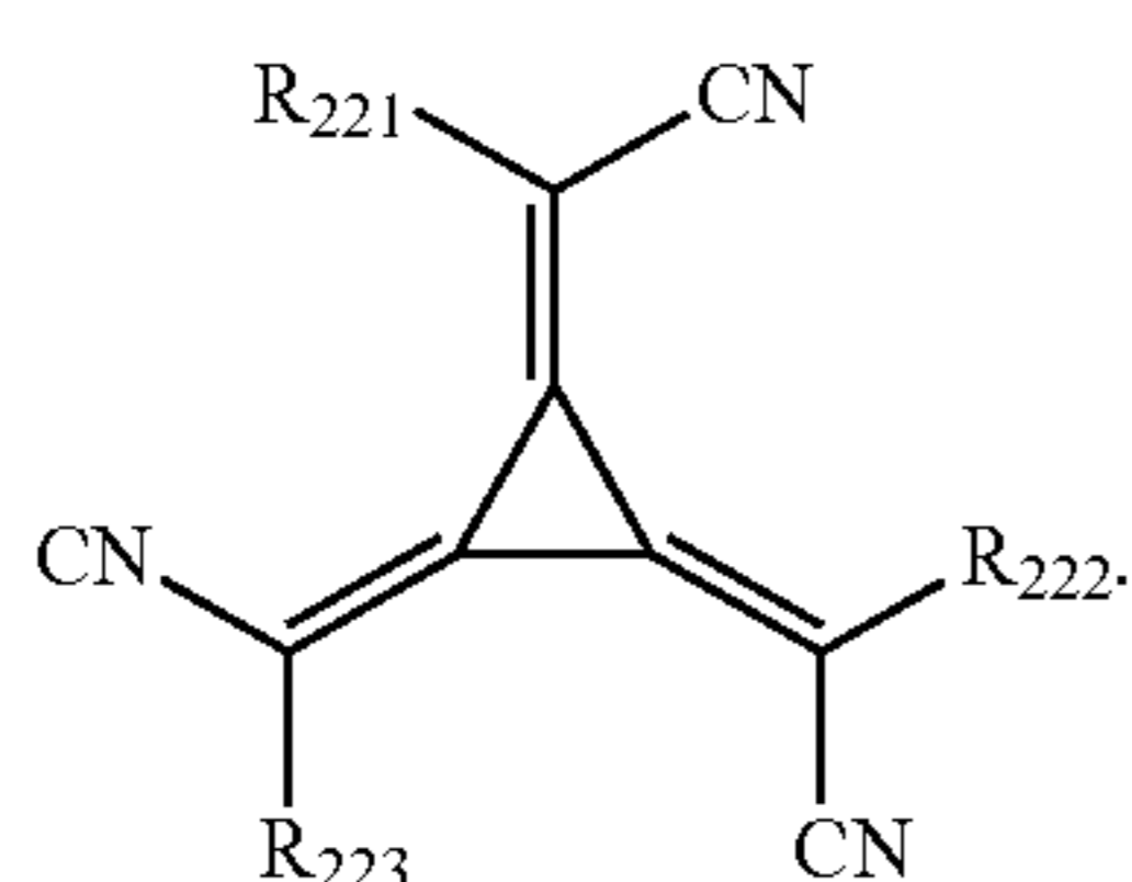
F4-TCNQ
