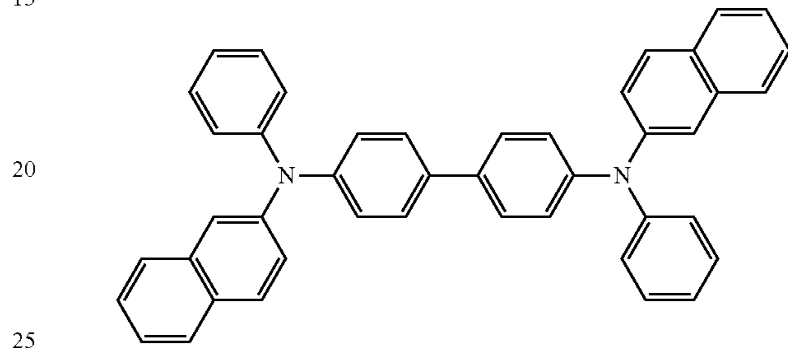
\beta -NPB
