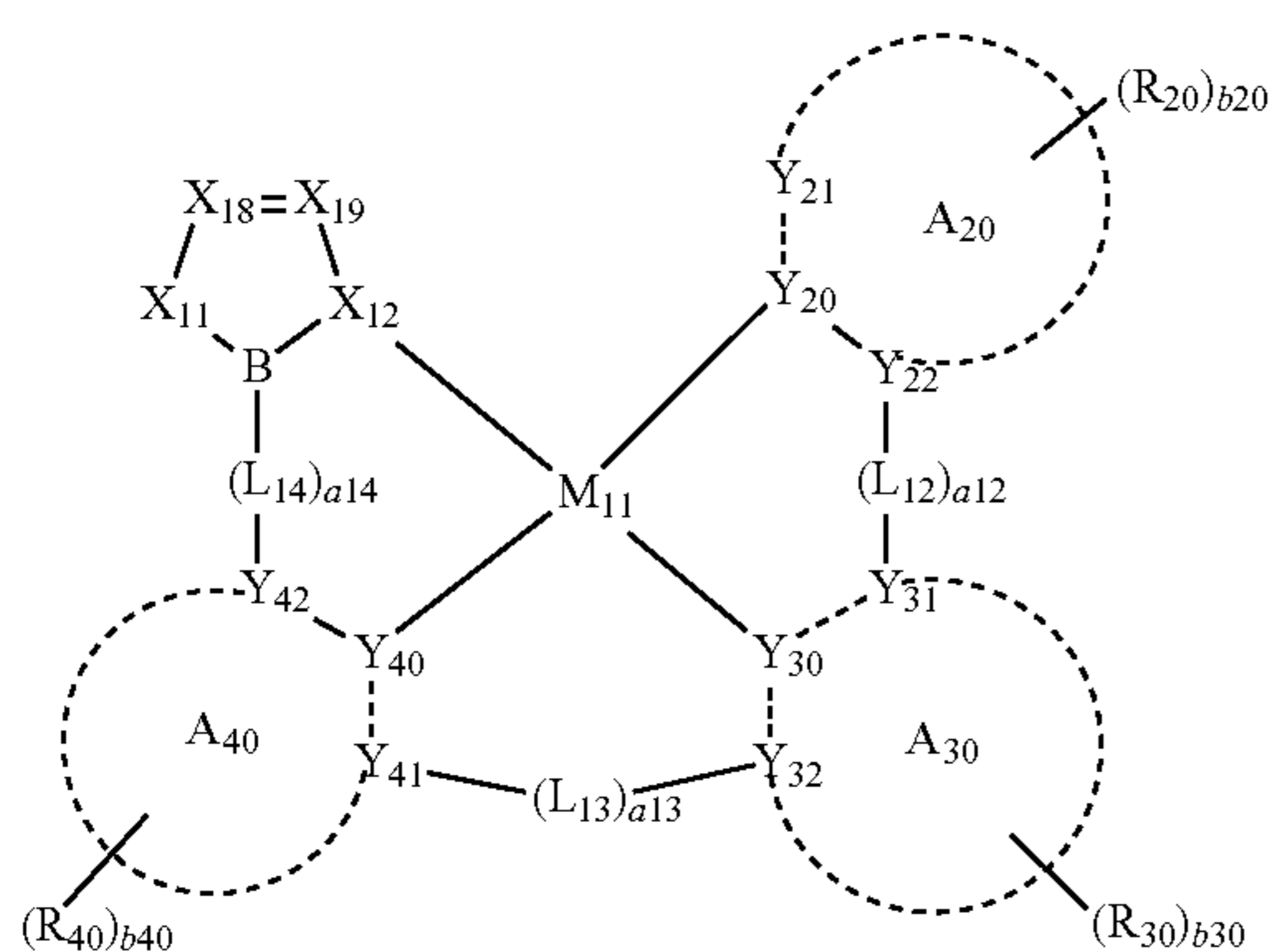
Formula 1G
