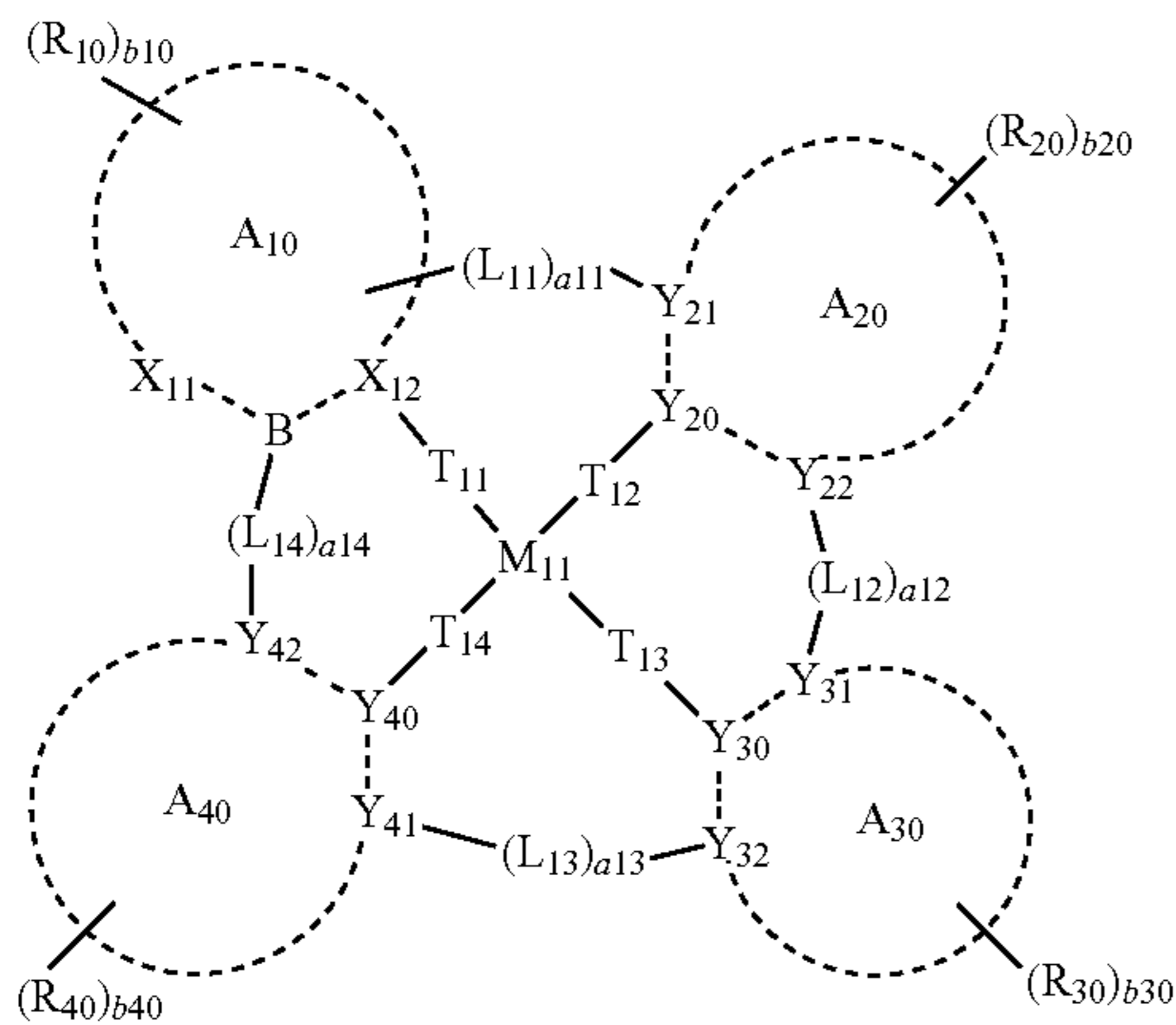
Formula 1
