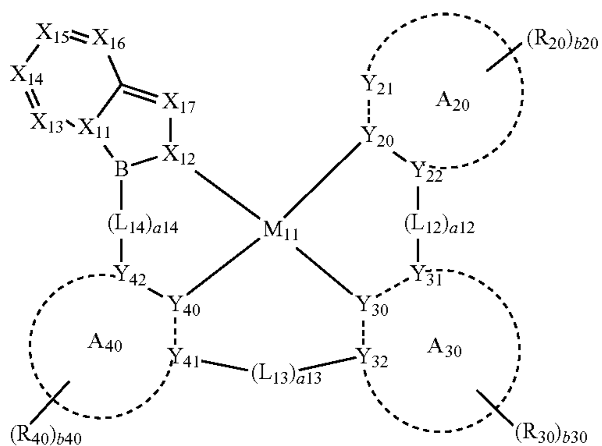
Formula 1F
