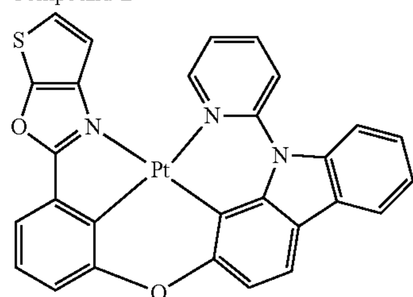
Compound B
