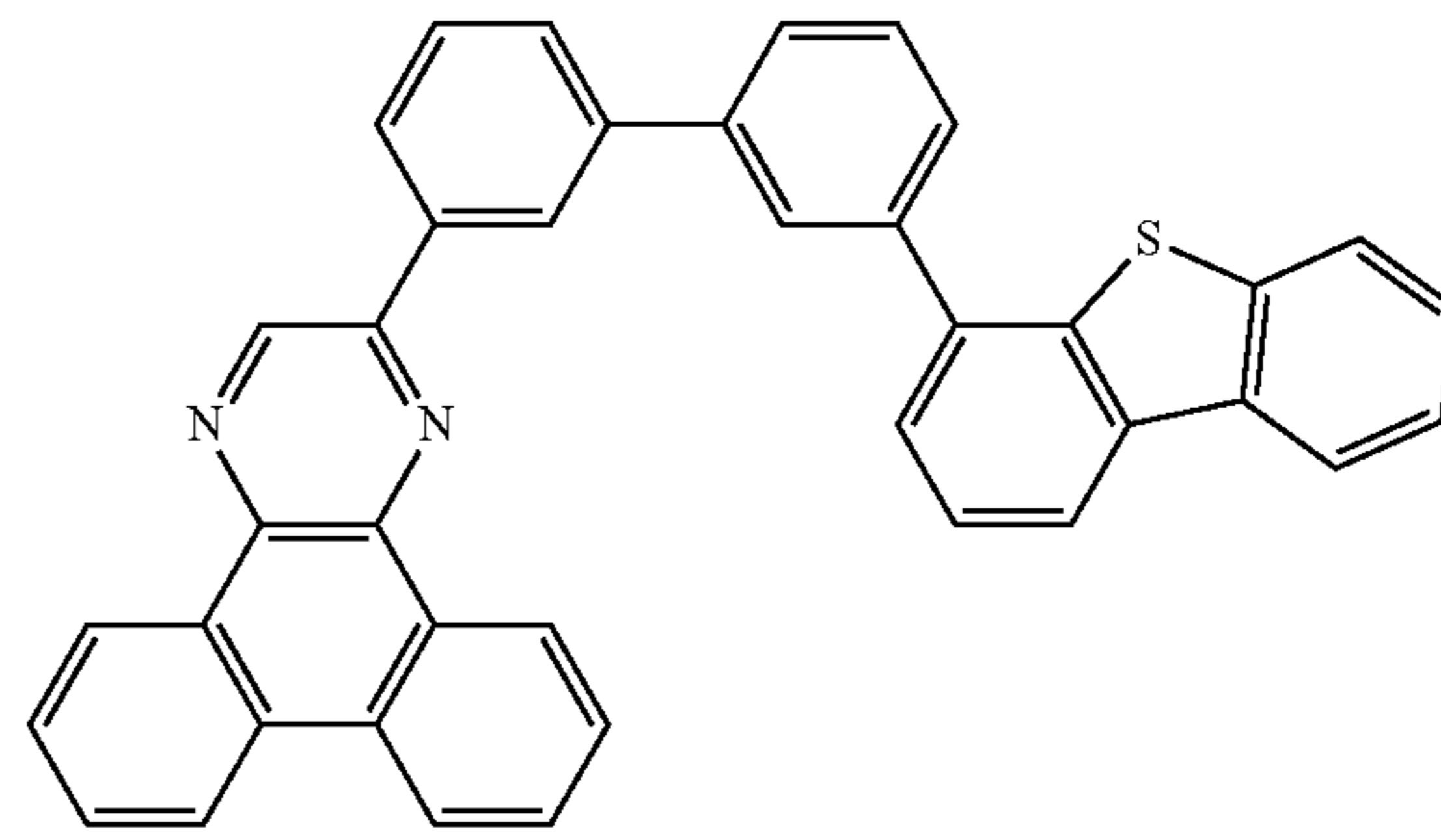
2mDBTBPDq-II
