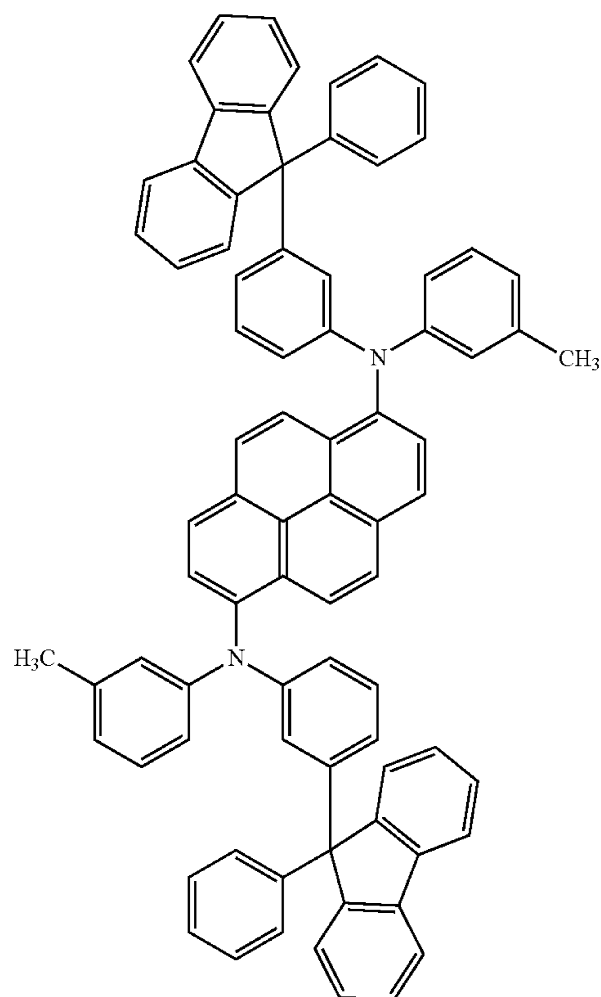
1,6mMemFLAPrn
