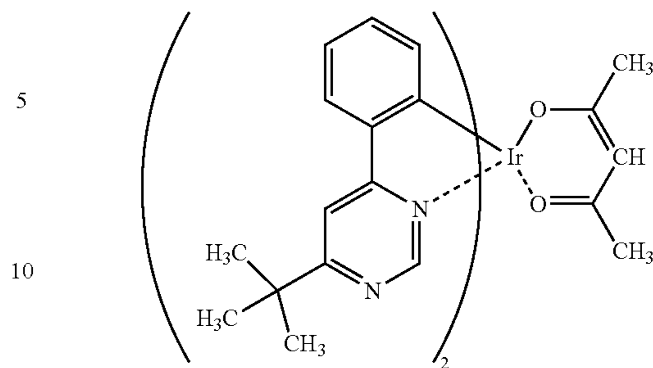
[Ir(tBuppm) 2 (acac)]
