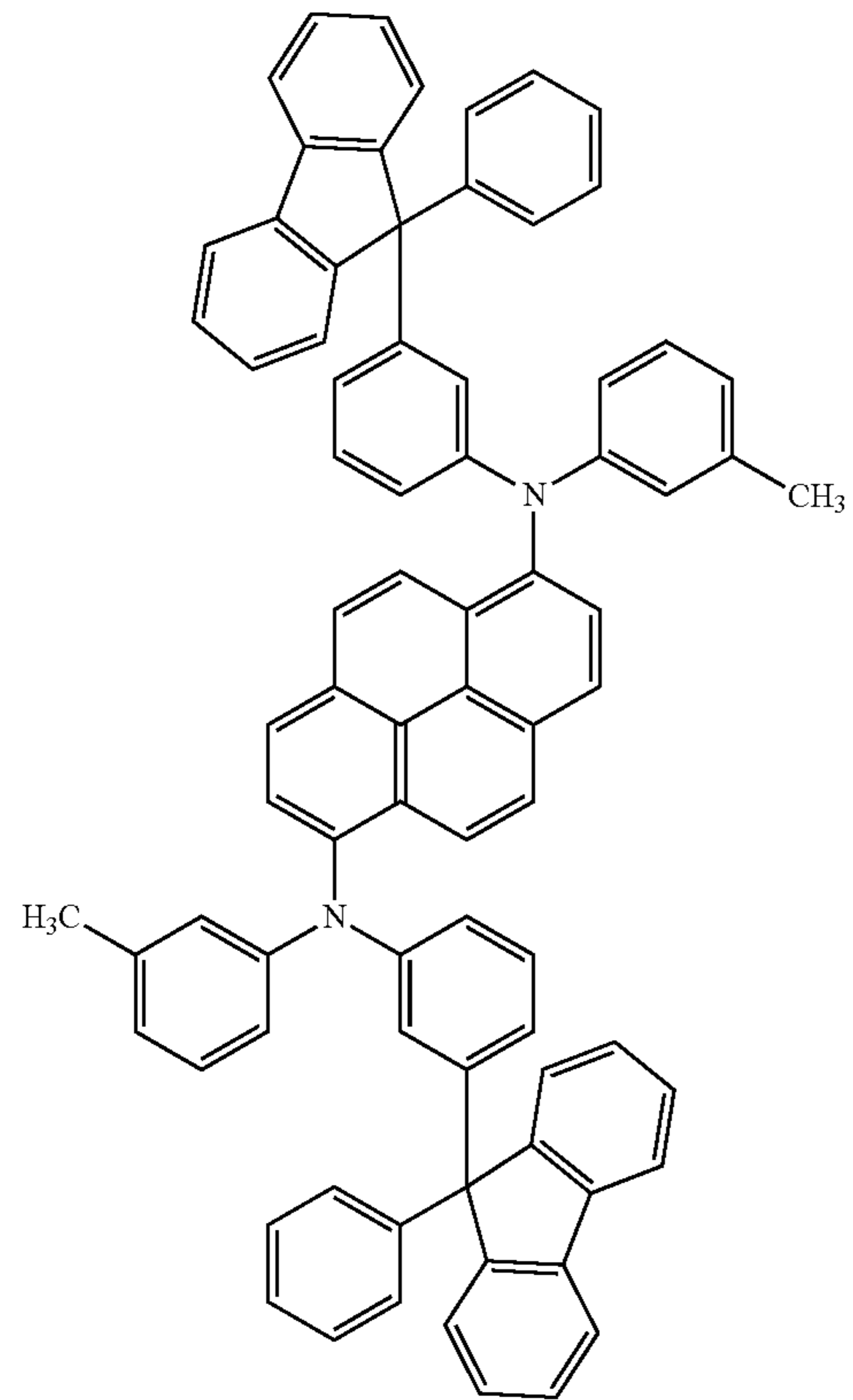
1,6mMemFLAPrn
