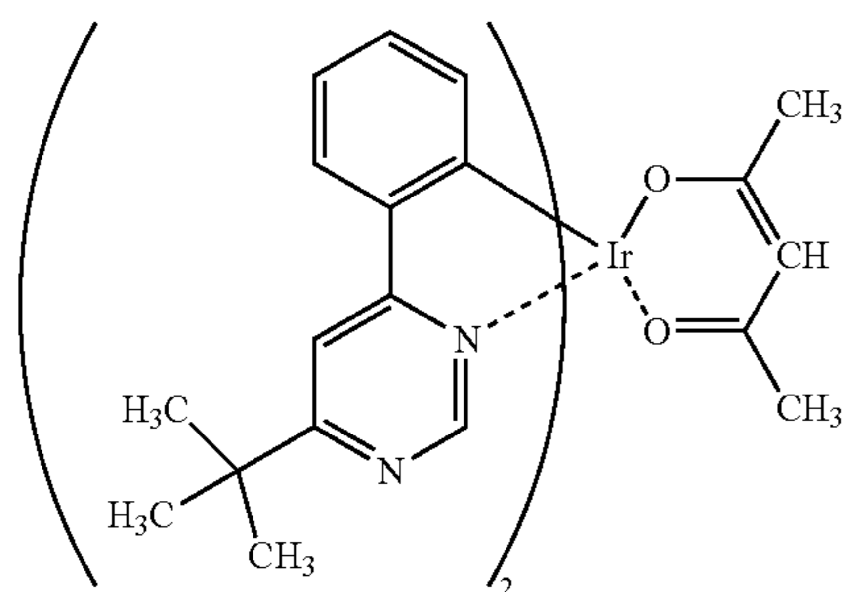
[\text{Ir}(\text{tBuppm})_2(\text{acac})]
