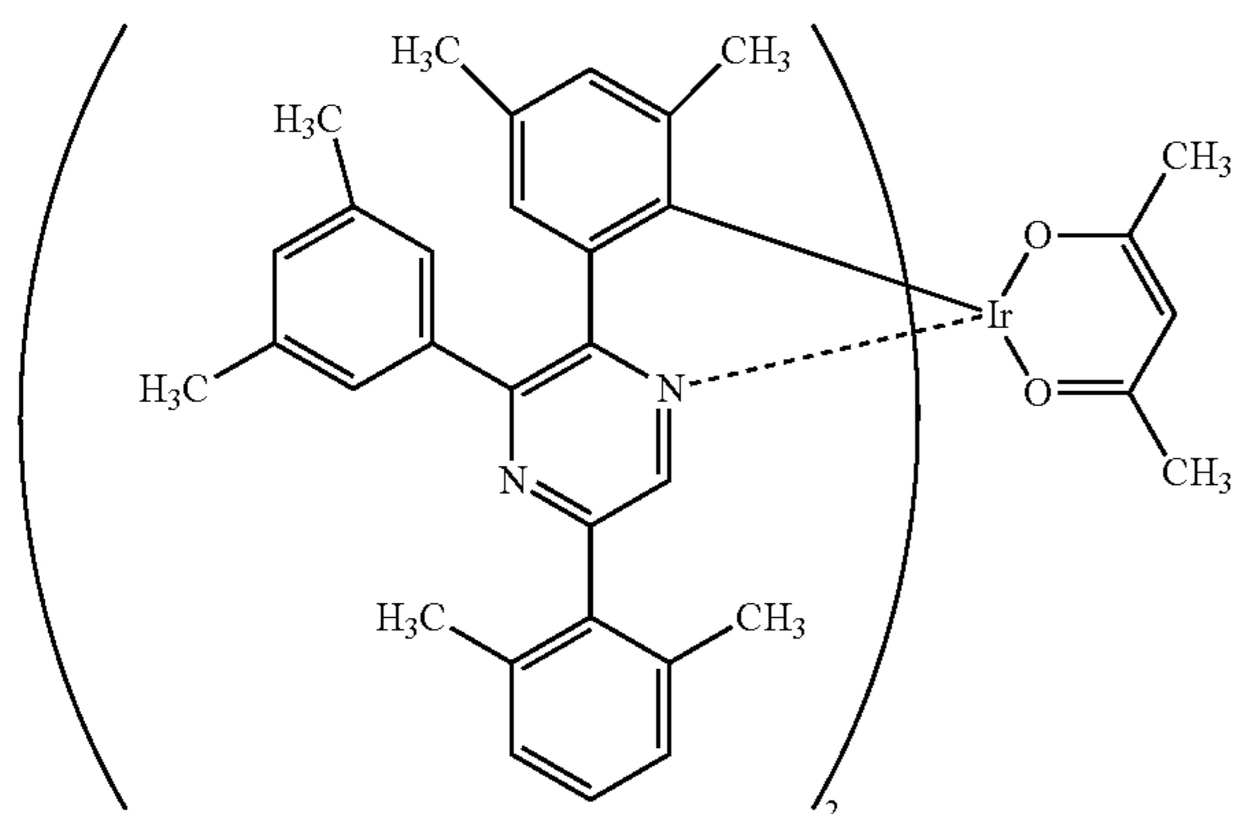
[Ir(dmdppr-dmp) 2 (acac)]
