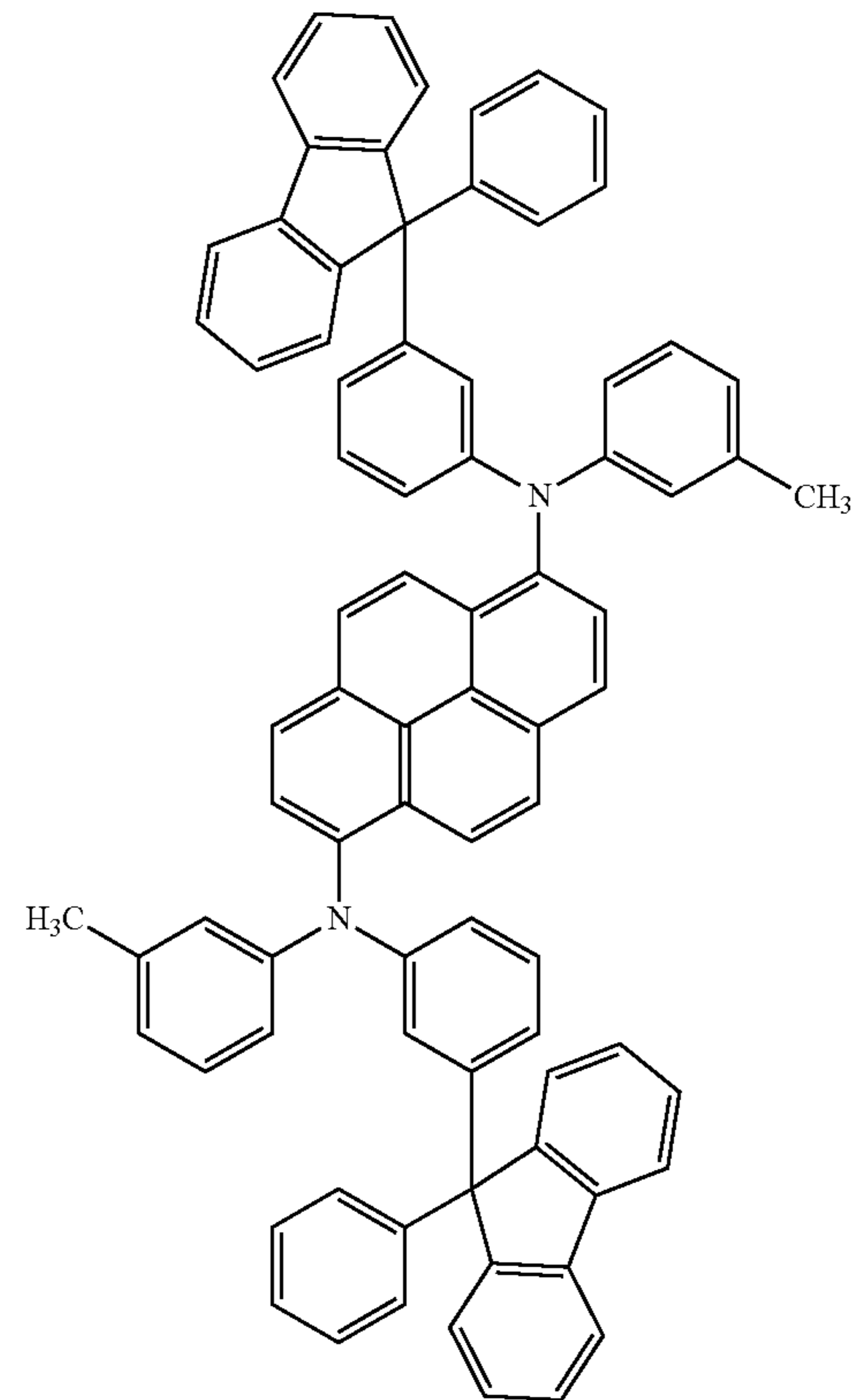
1,6mMemFLAPrn
