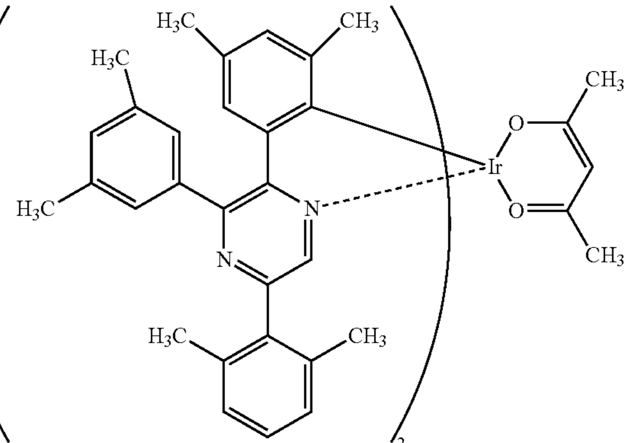
[Ir(dmdppr-dmp) 2 (acac)]
