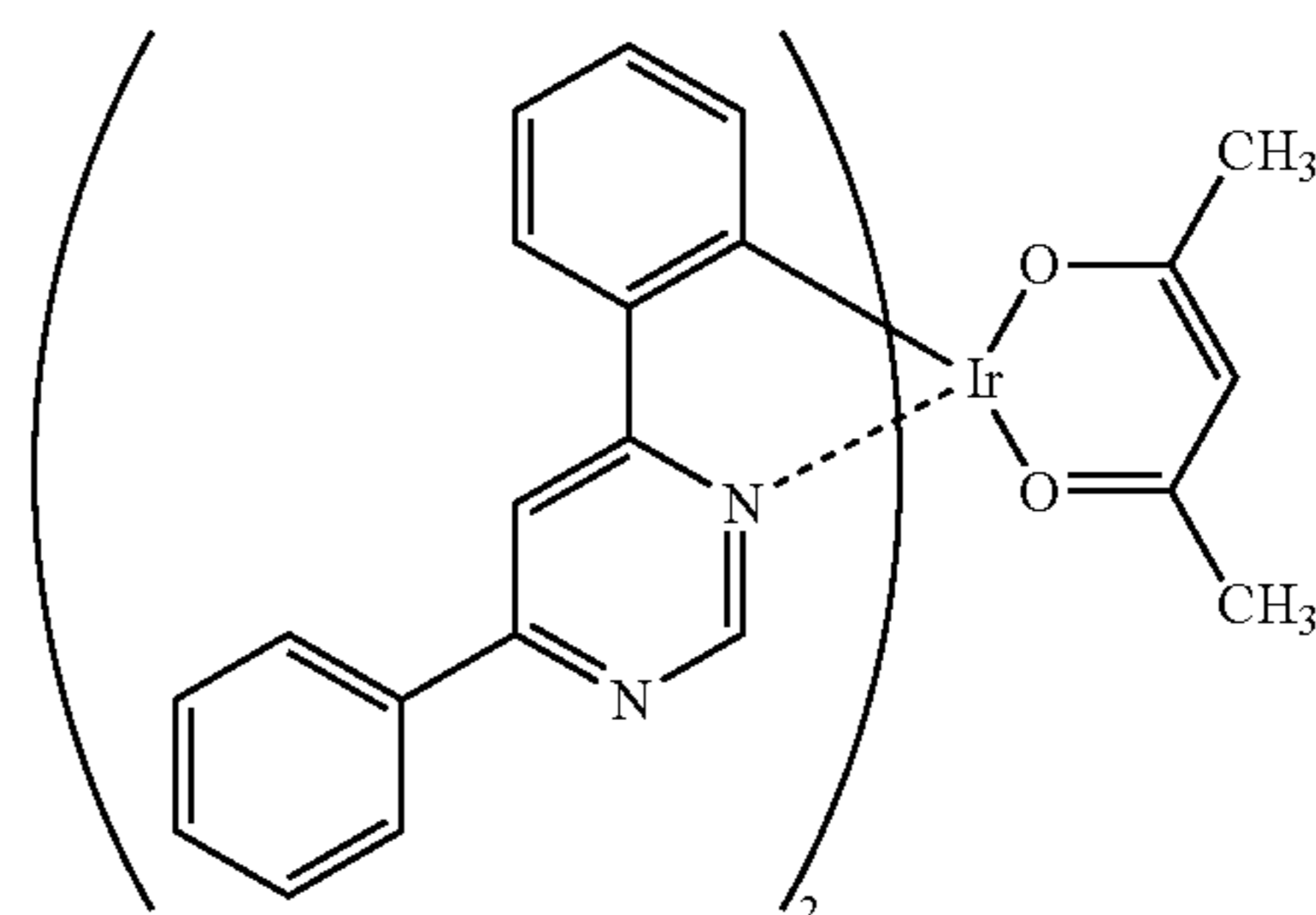
[Ir(dppm) 2 (acac)]
