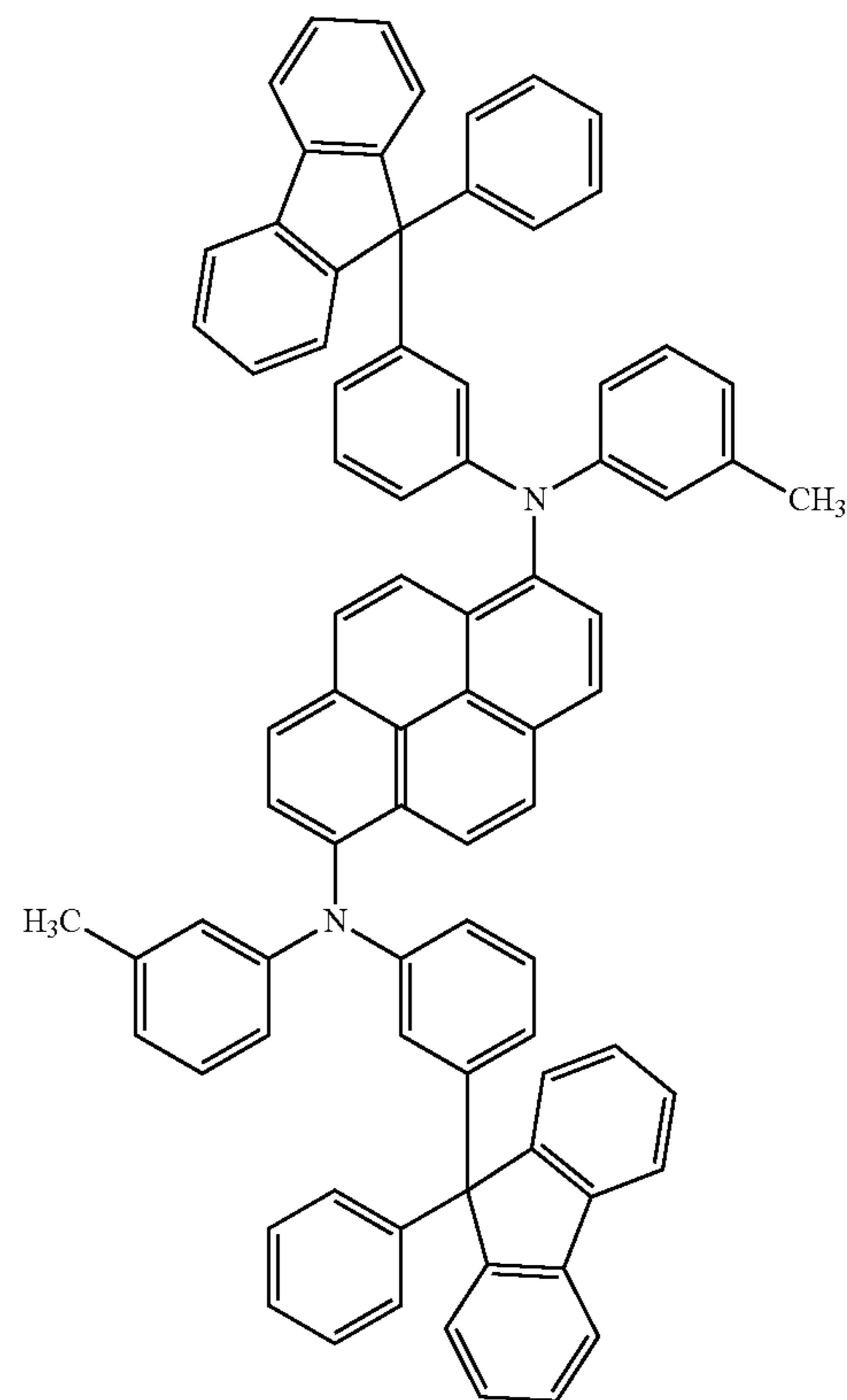
1,6mMemFLAPrn
