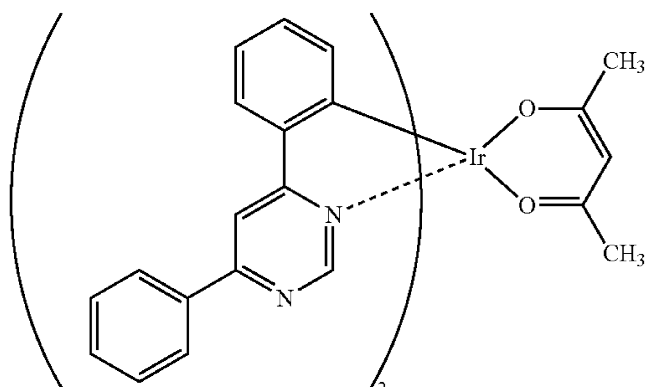
Ir(dppm) 2 (acac)
