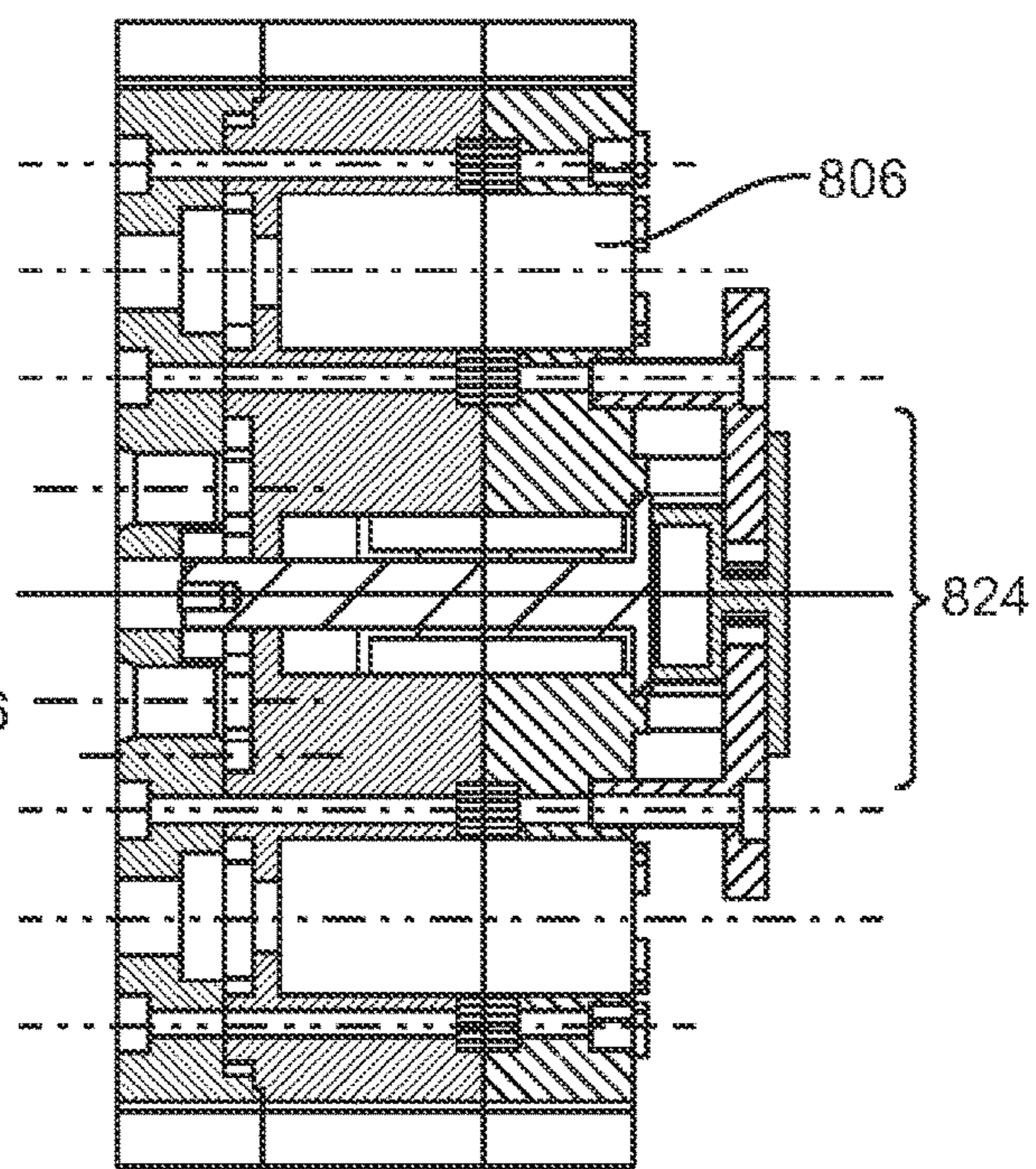
Section B-B
