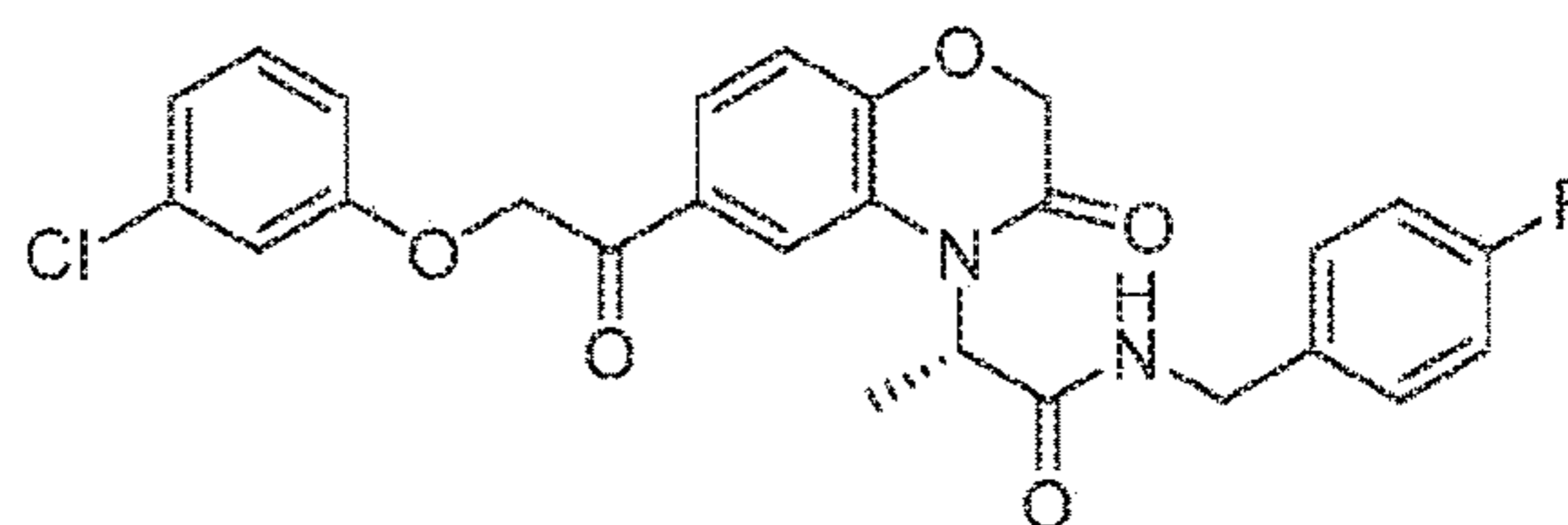
Compound 6
