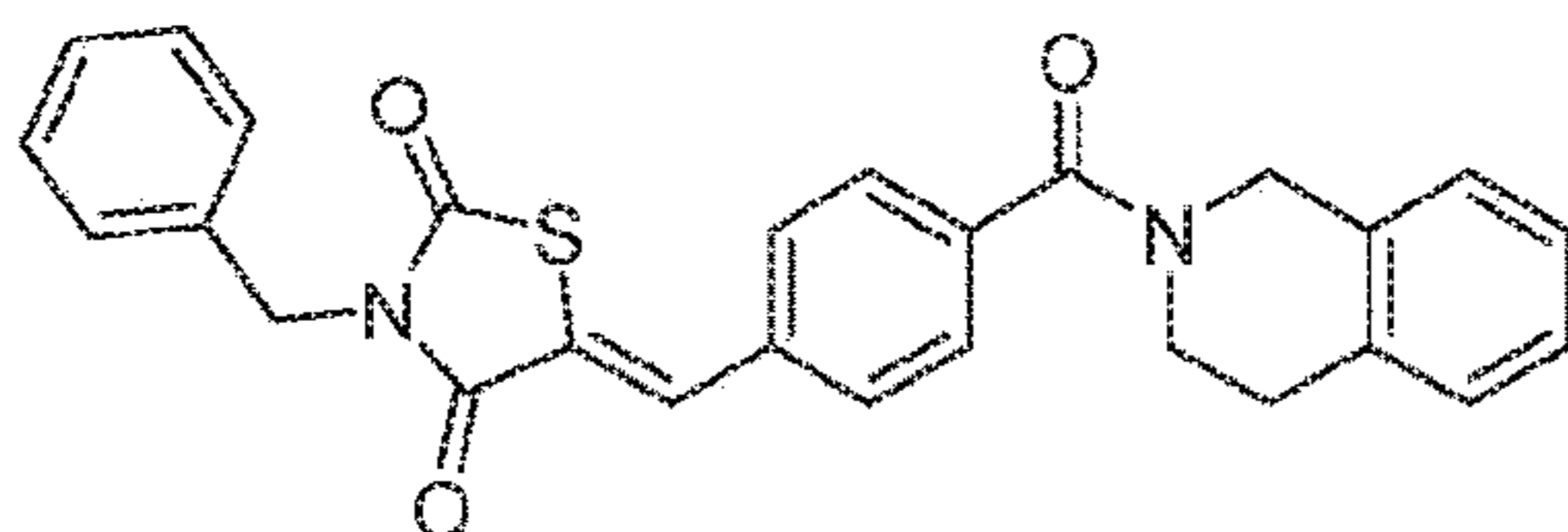
Compound 4
