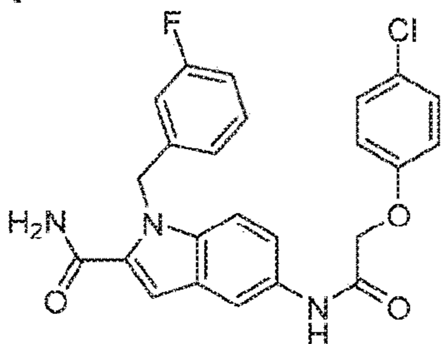
Compound 2
