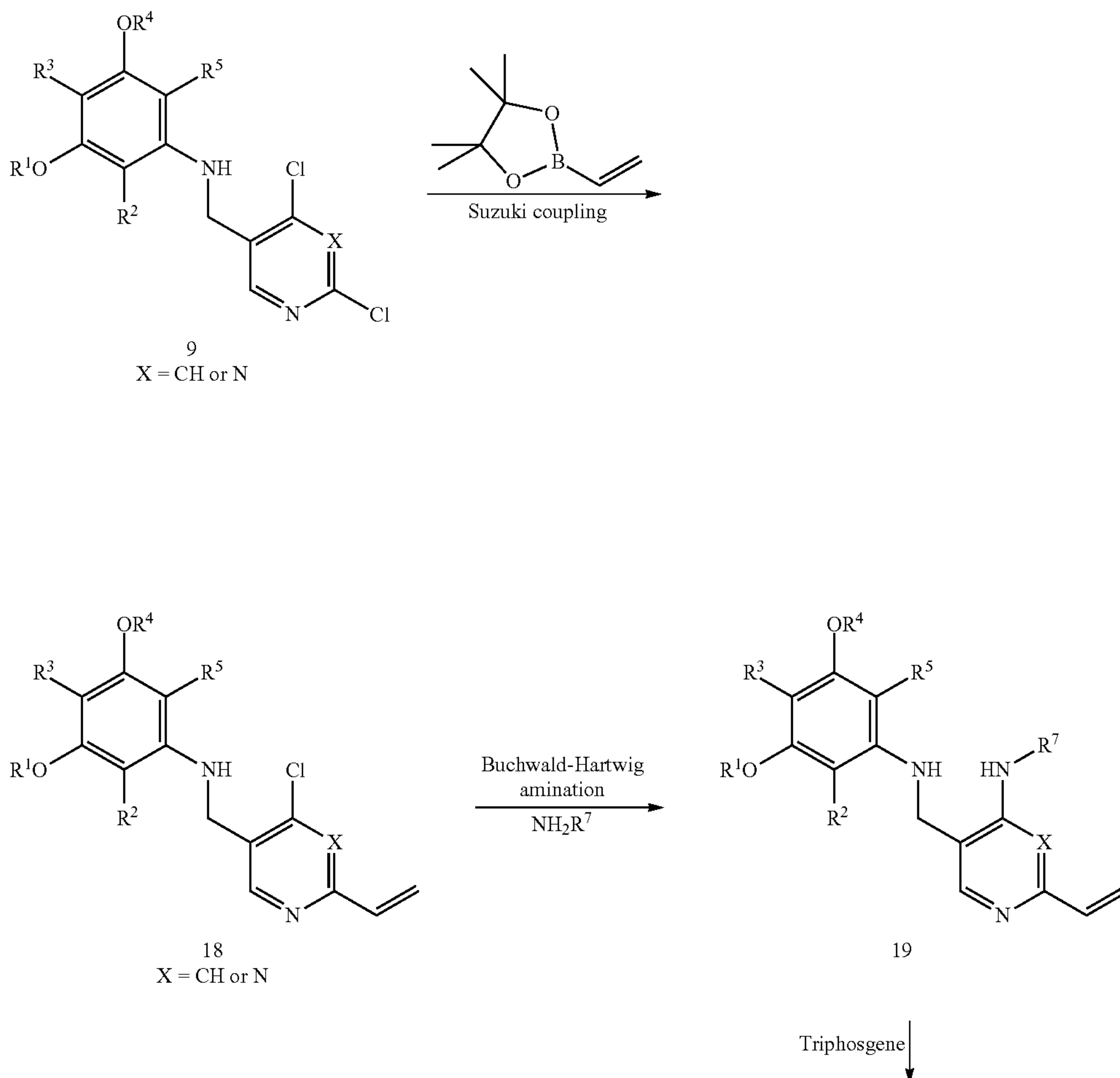
Scheme 5
