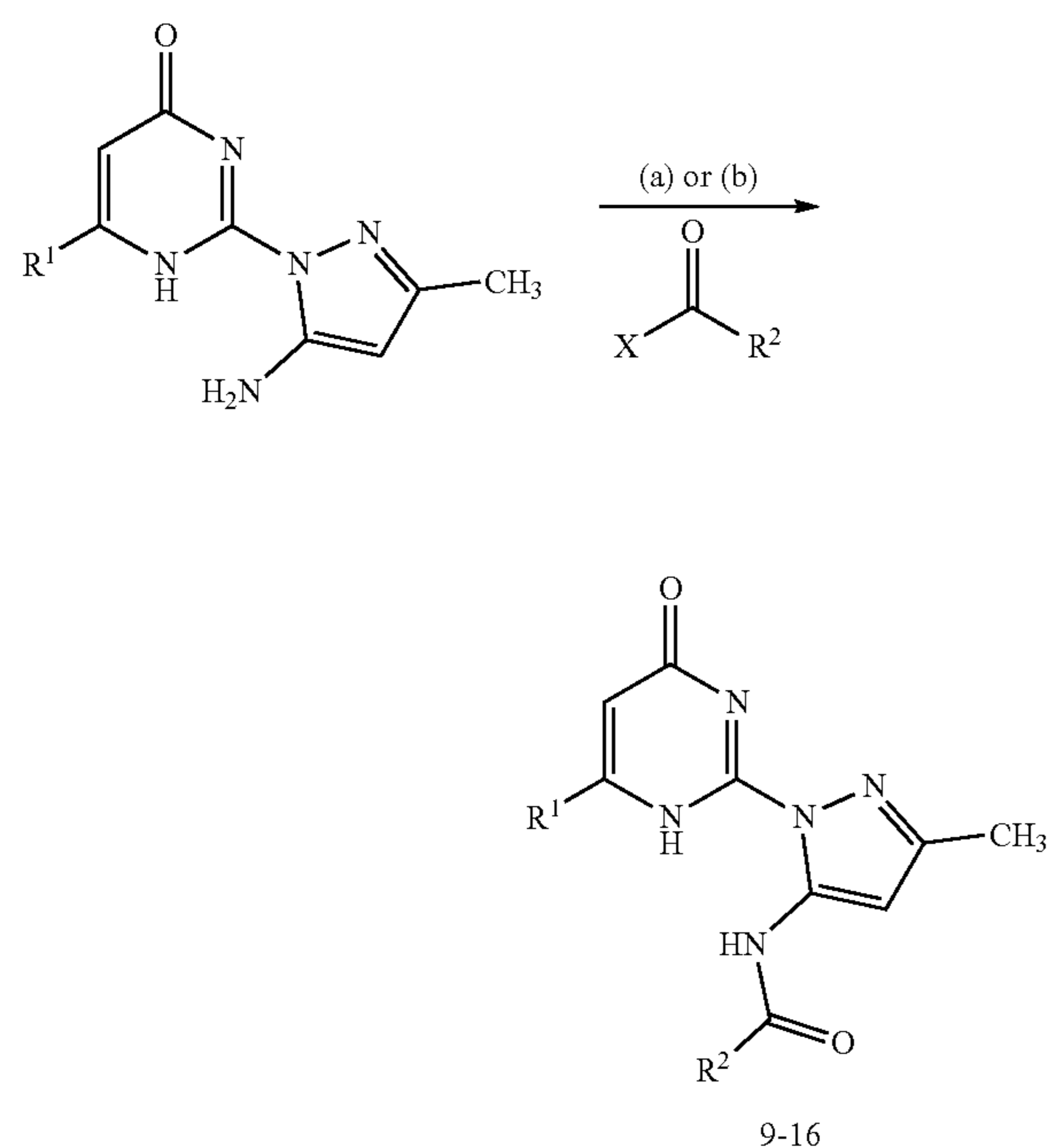
Scheme 3. Chemical Synthesis for Dihydropyrimidine based AC1 inhibitors*
