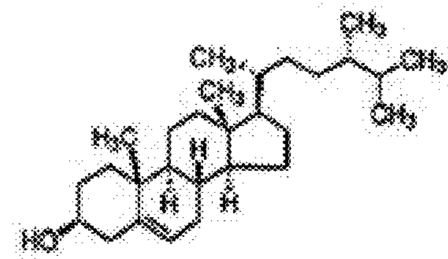
Campesterol
