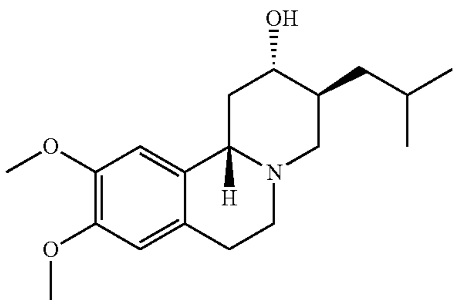
(-)-α-HTBZ
