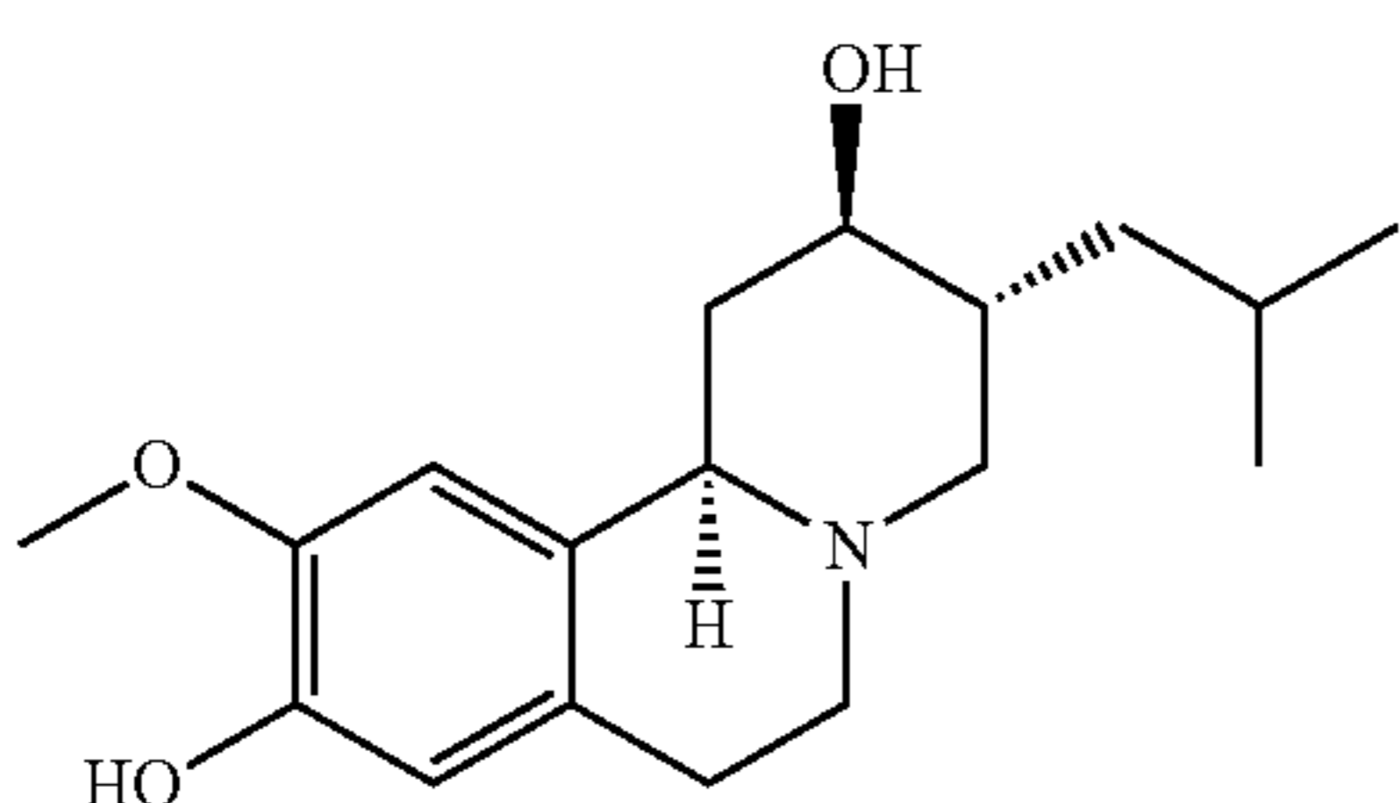
(+)-9-O-desmethyl-α-HTBZ
