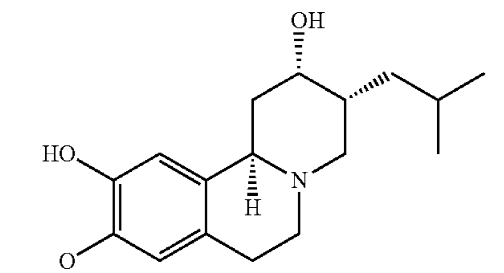
(+)-d 3 -10-O-desmethyl-β-HTBZ
