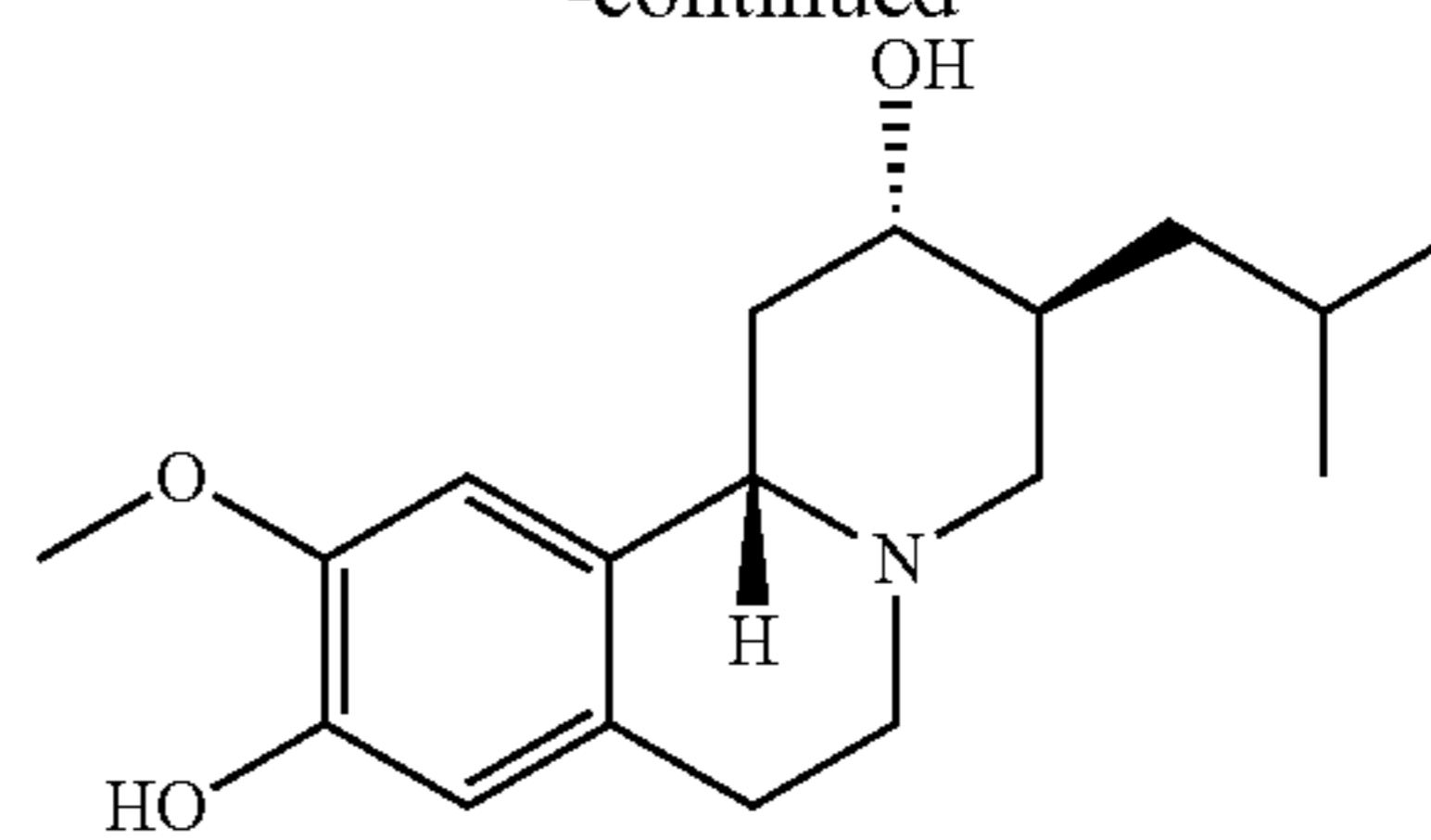
(-)-9-O-desmethyl-α-HTBZ
