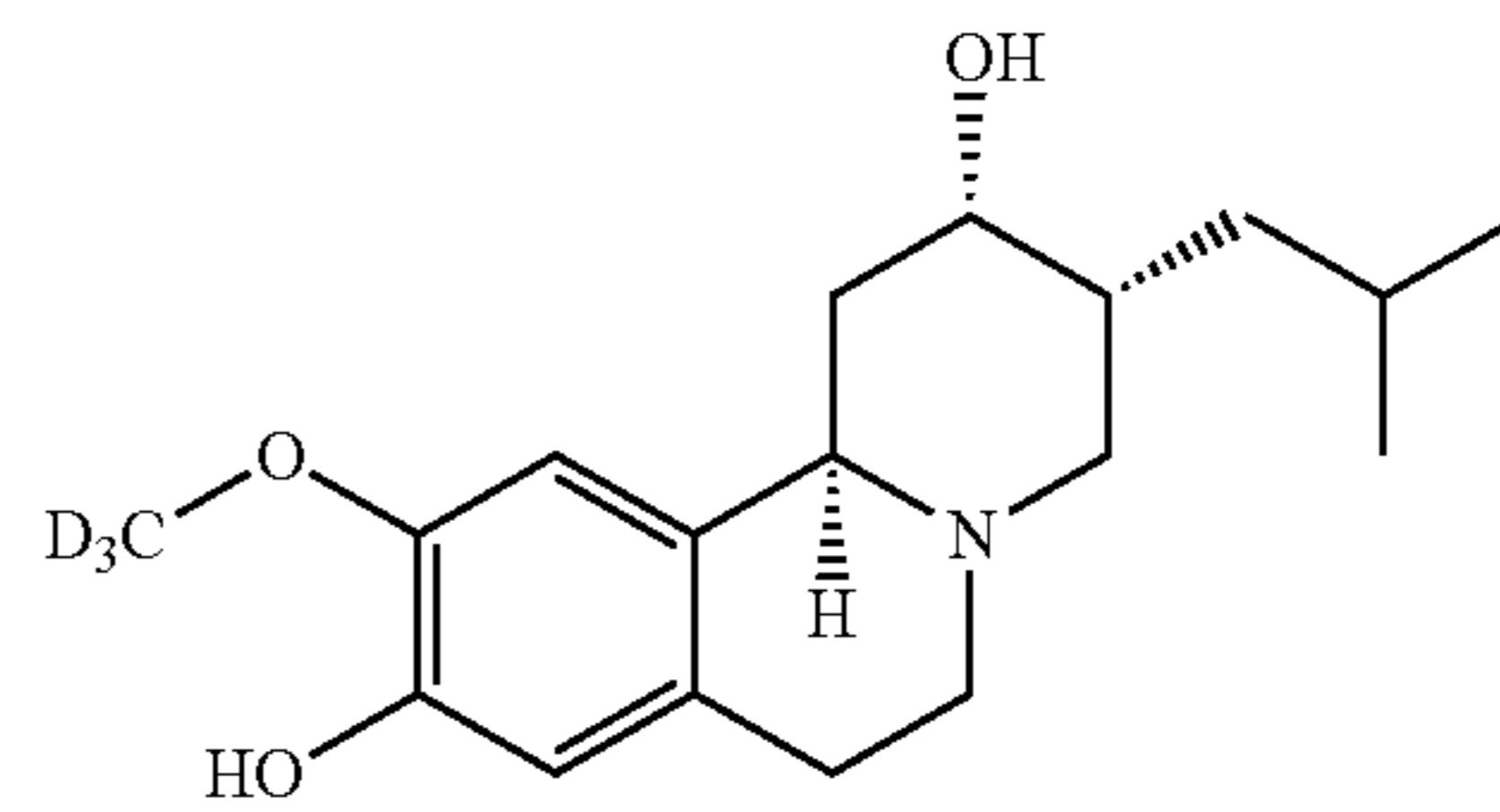
(+)-d 3 -9-O-desmethyl-β-HTBZ
