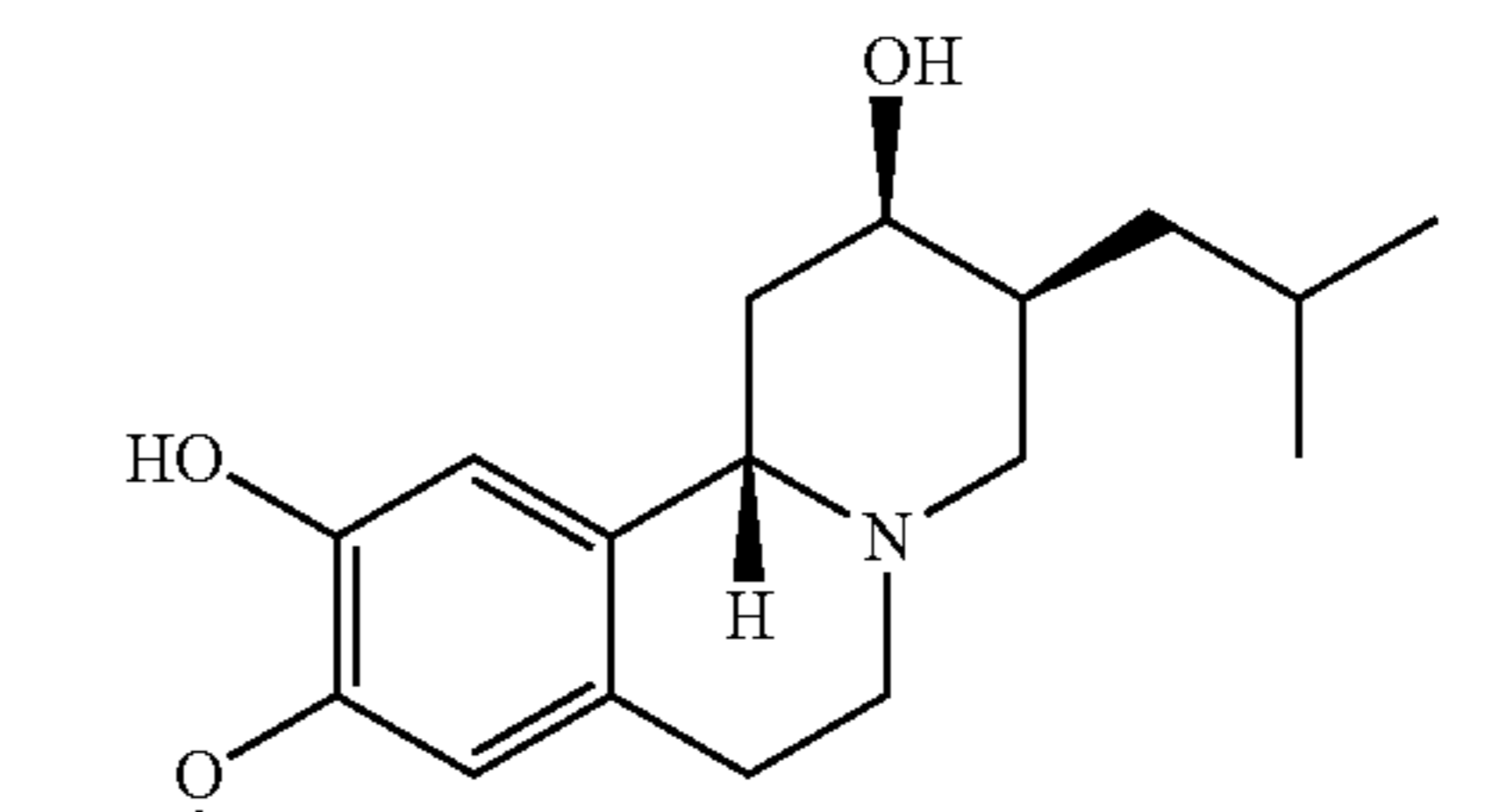
(+)-d 3 -10-O-desmethyl-β-HTBZ
