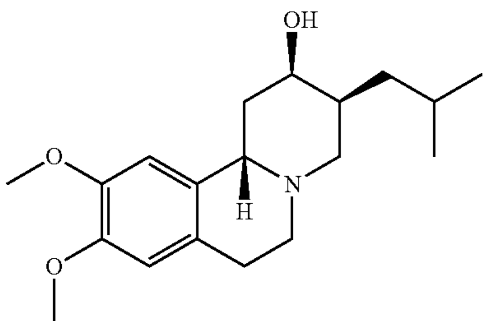
(-)-β-HTBZ
