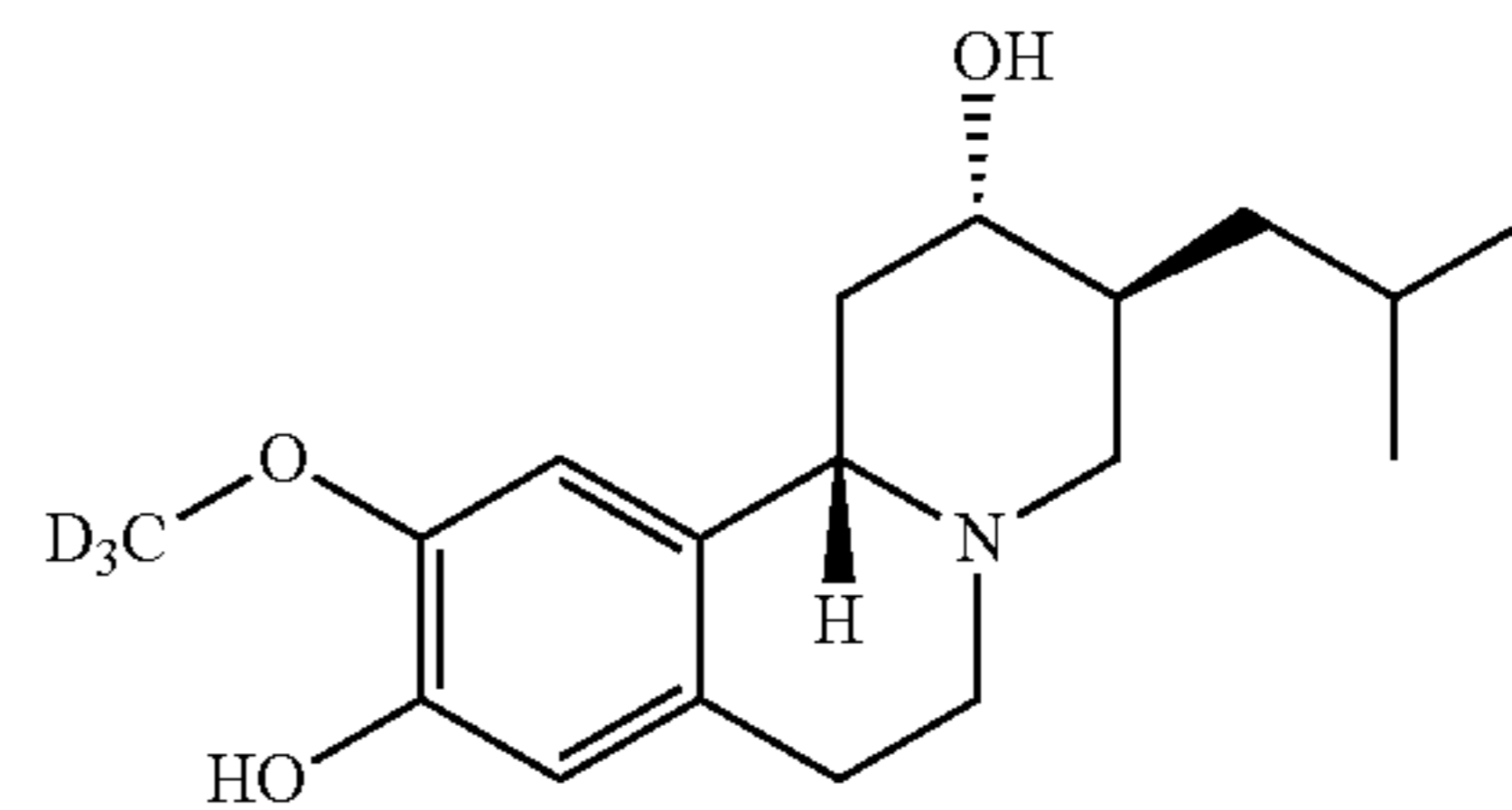
(-)-d 3 -9-O-desmethyl-α-HTBZ
