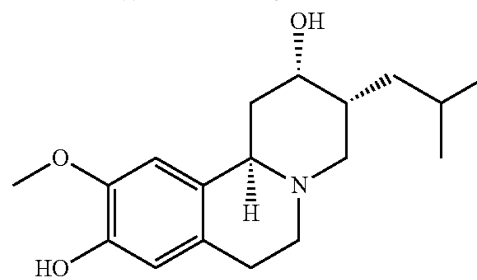
(+)-9-O-desmethyl-β-HTBZ
