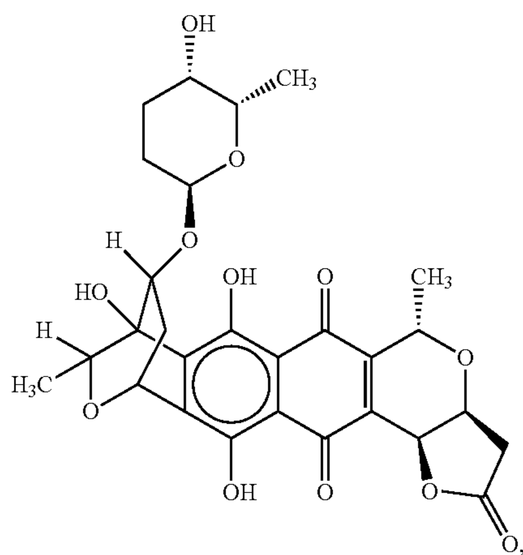
granatin B
