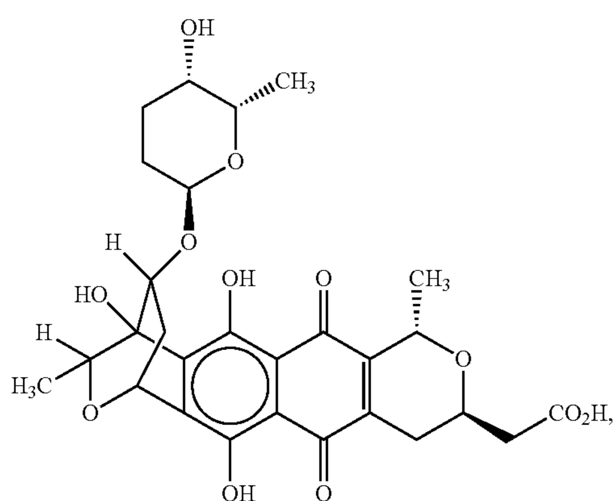
dihydrogranatin B
