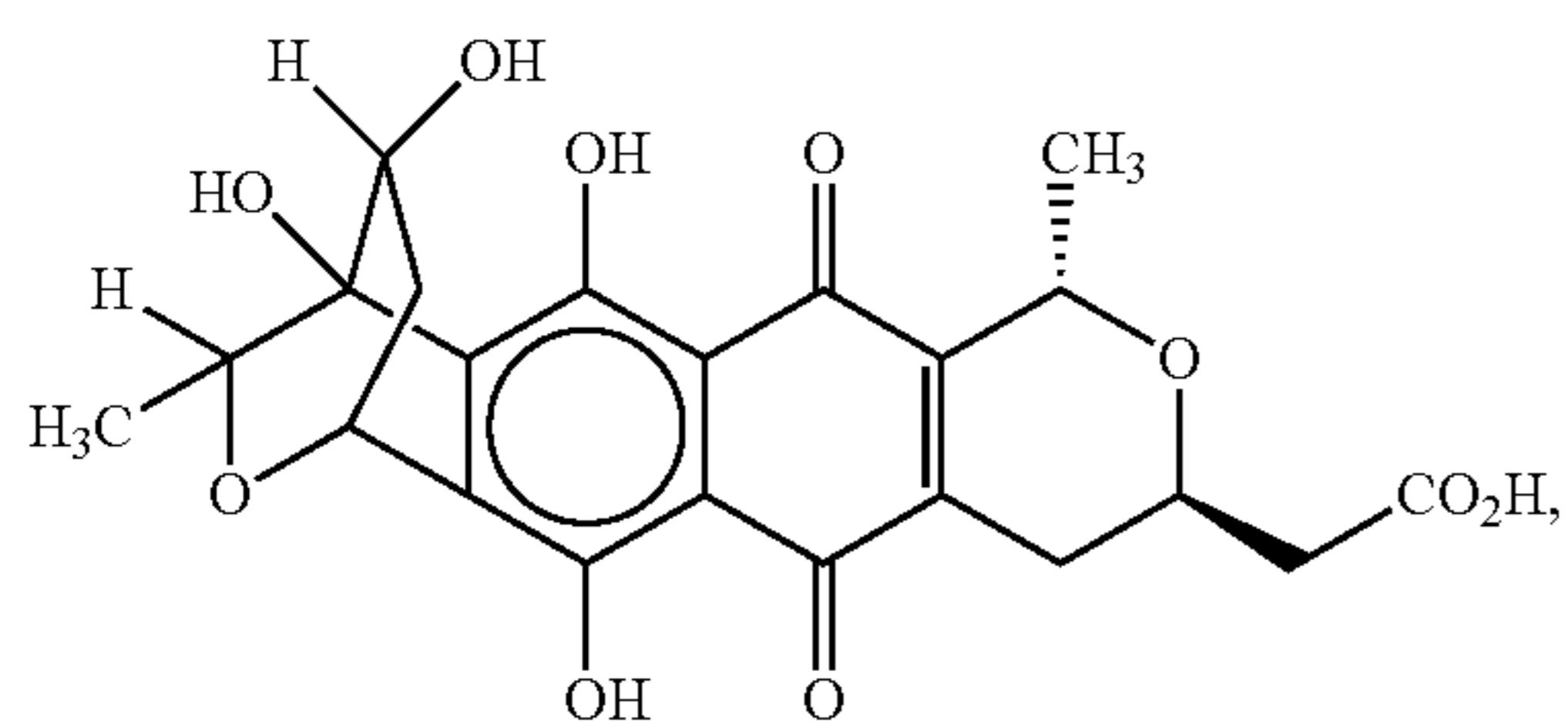
dihydrogranatin A
