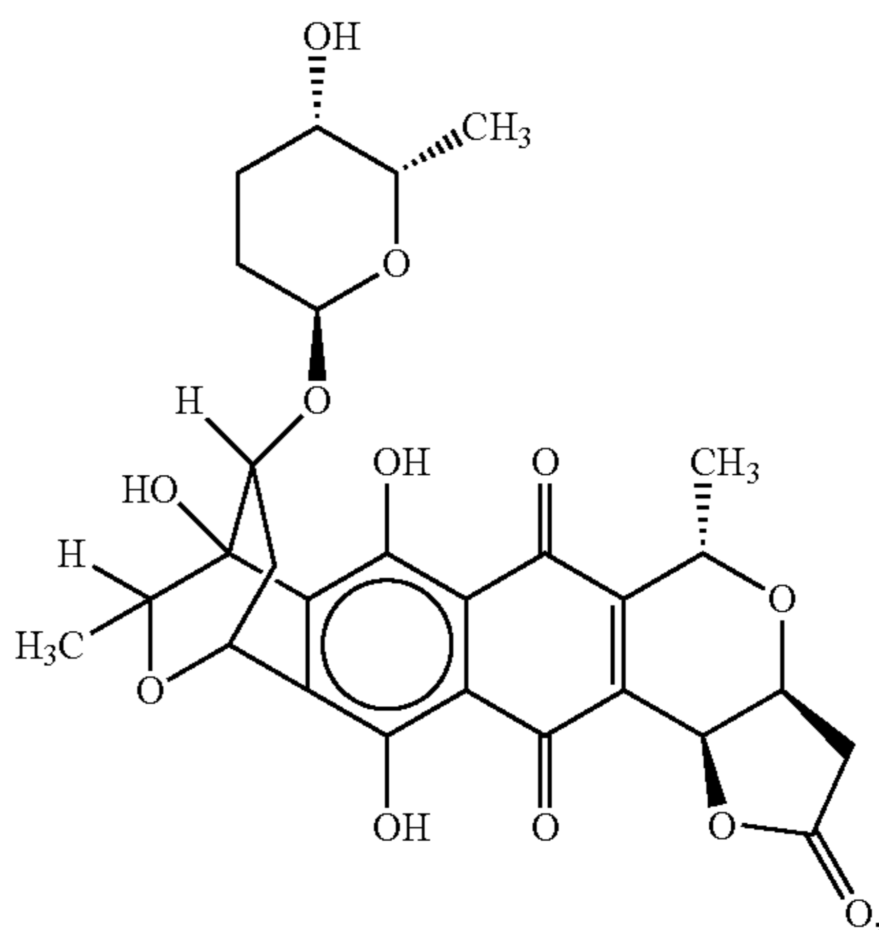
granaticin B
