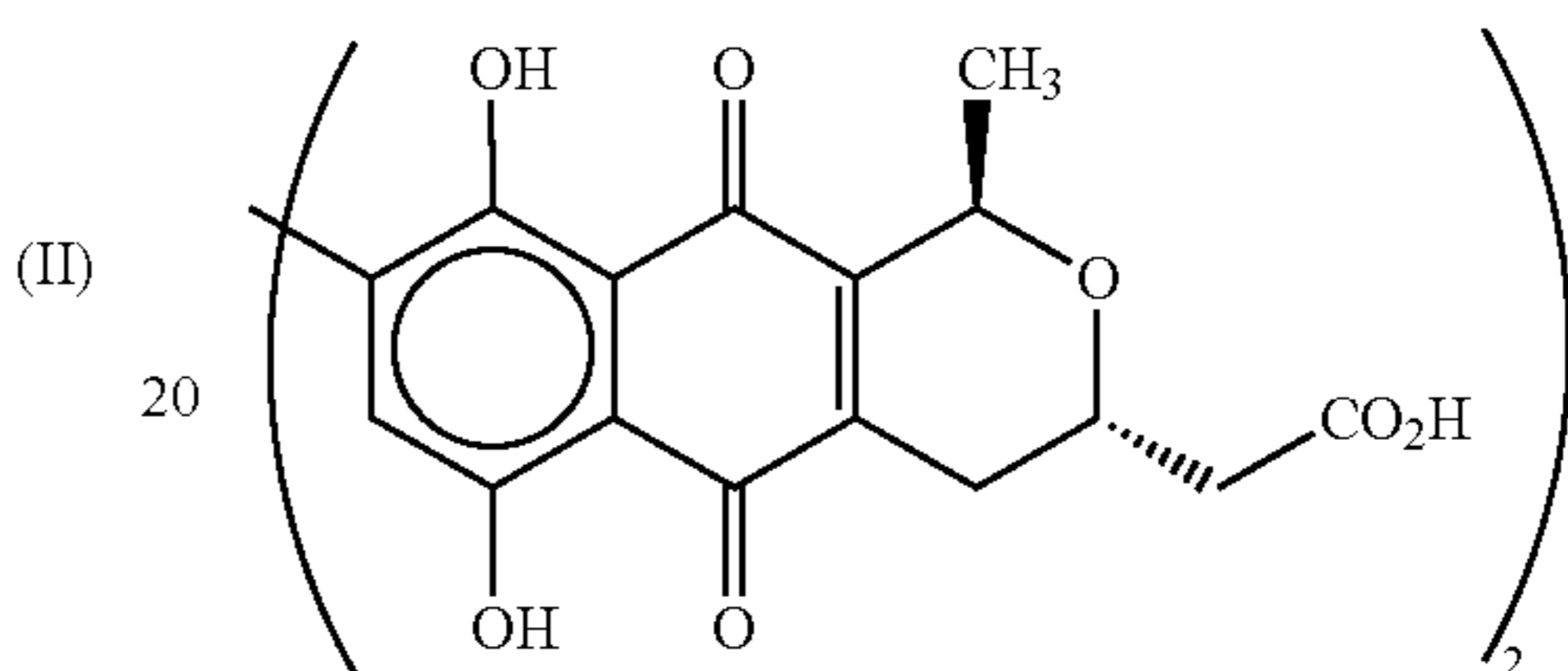
actinorhodin
