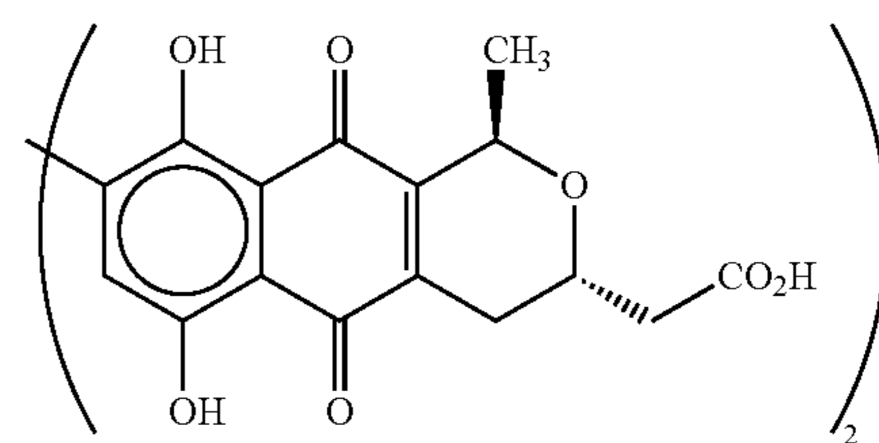
actinorhodin
