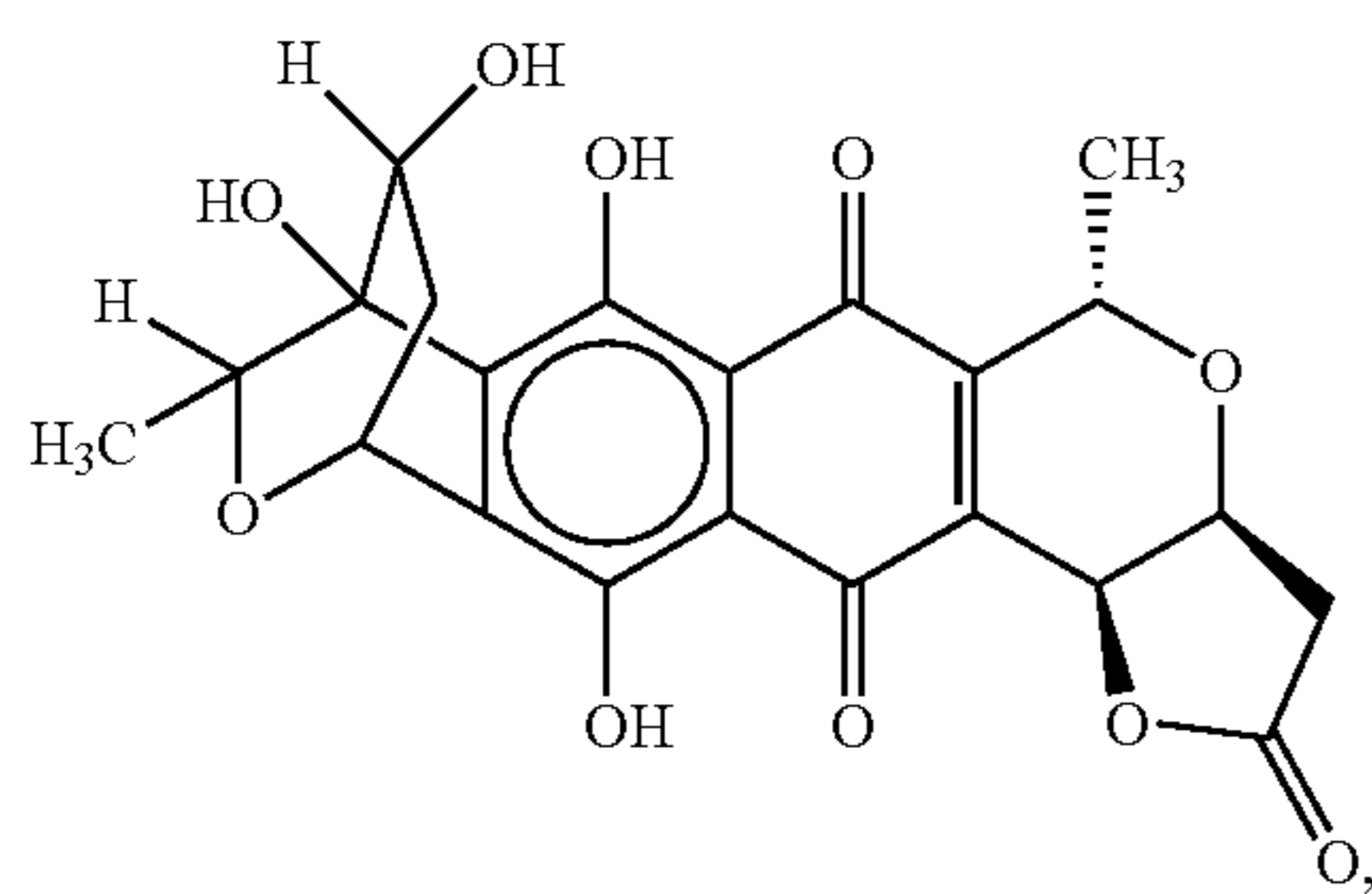
granatin A
