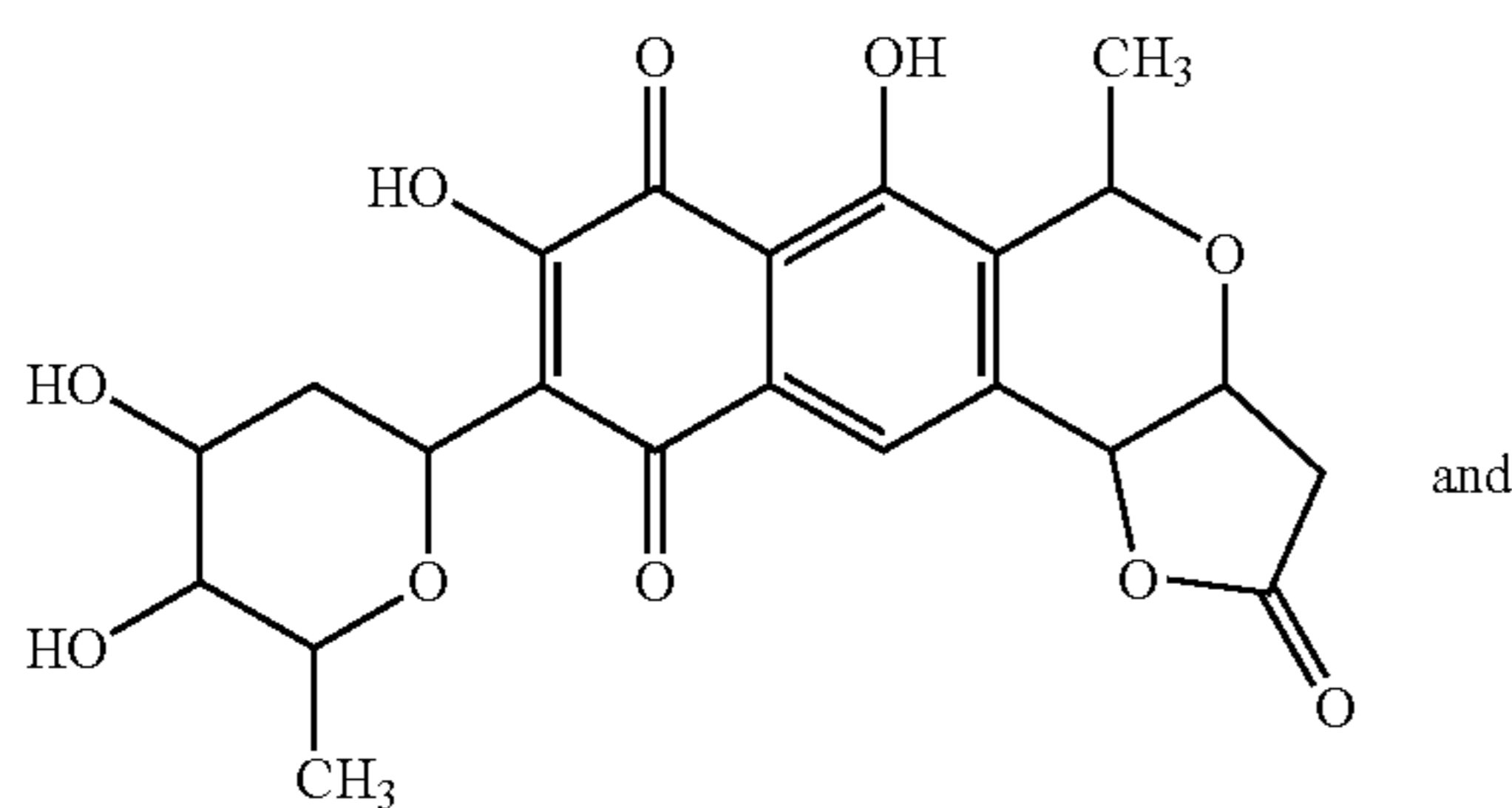
Derivative 1
