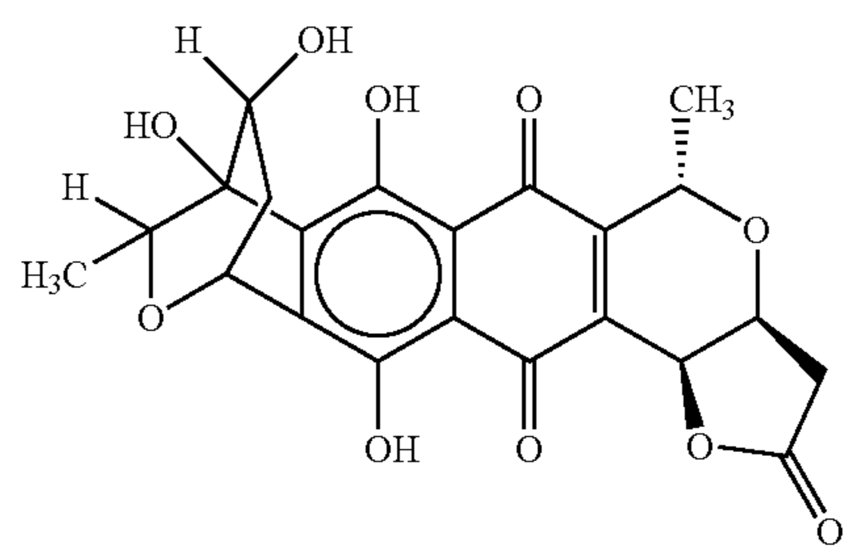
granaticin A
