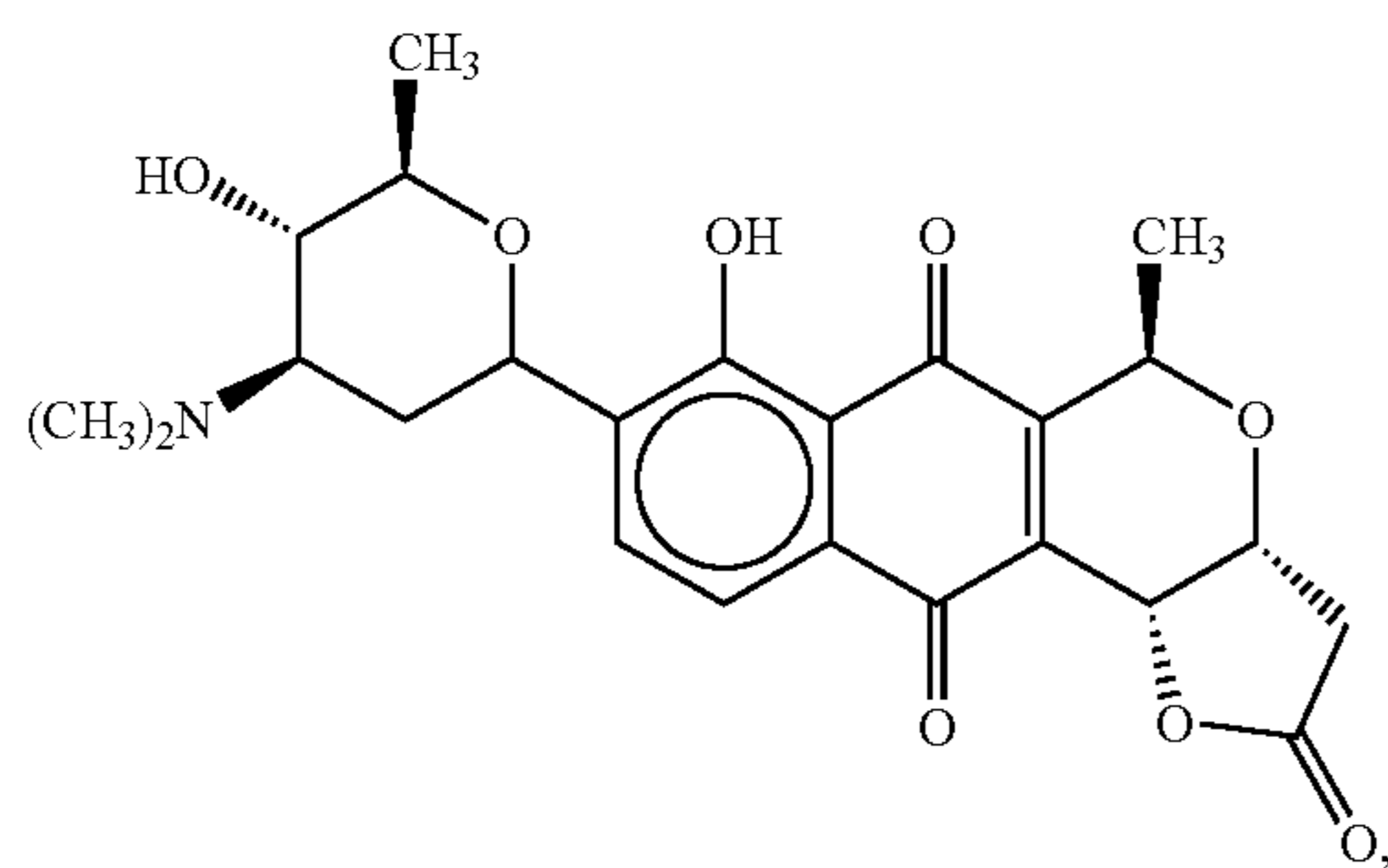
medermycin
