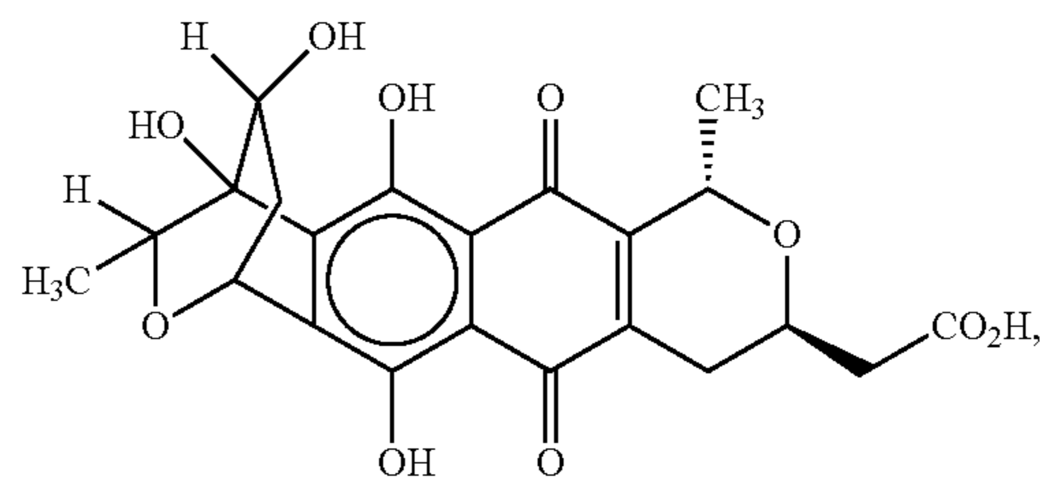
dihydrogranaticin A
