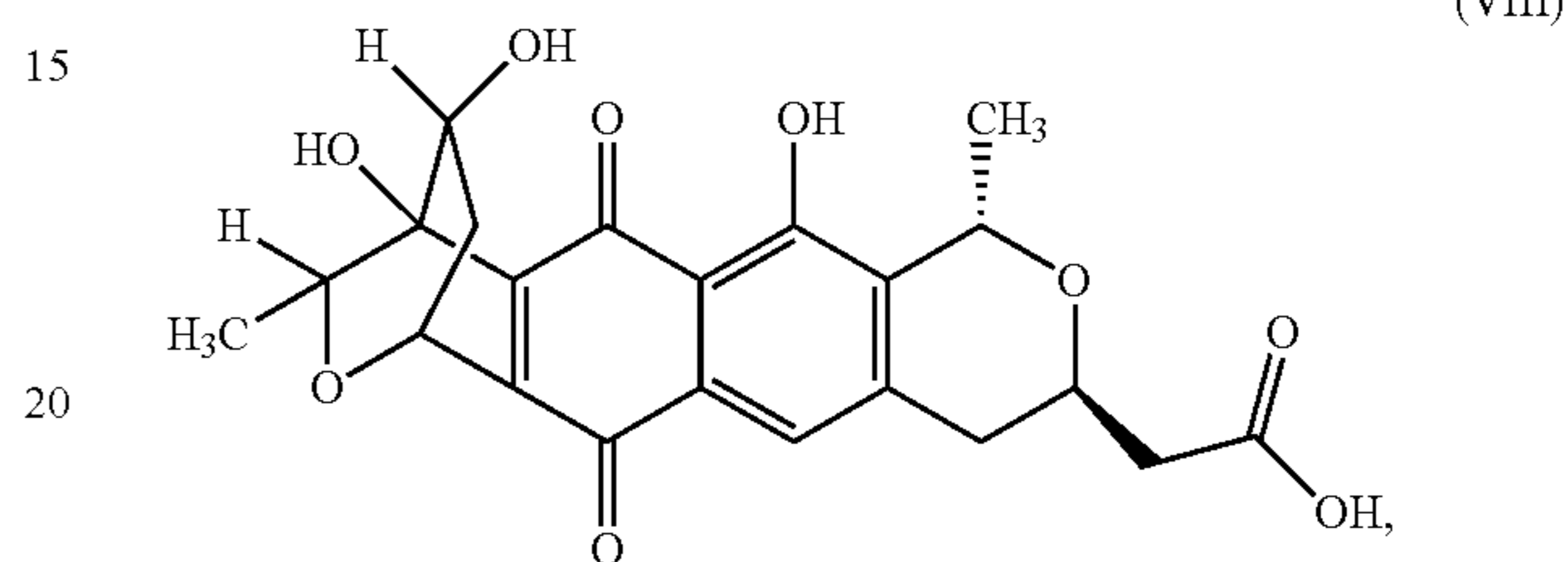
Derivative 2
