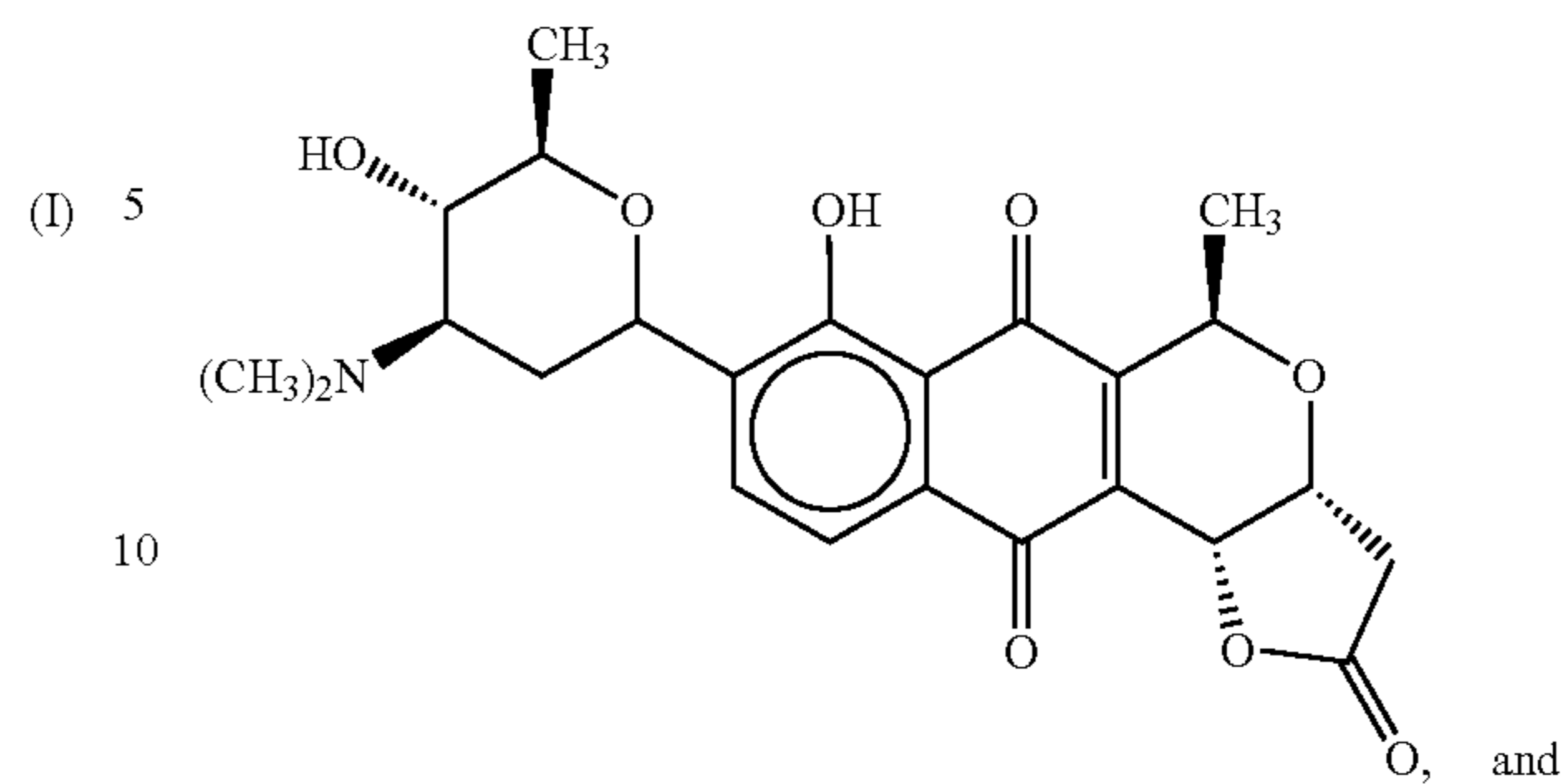
medemycin
