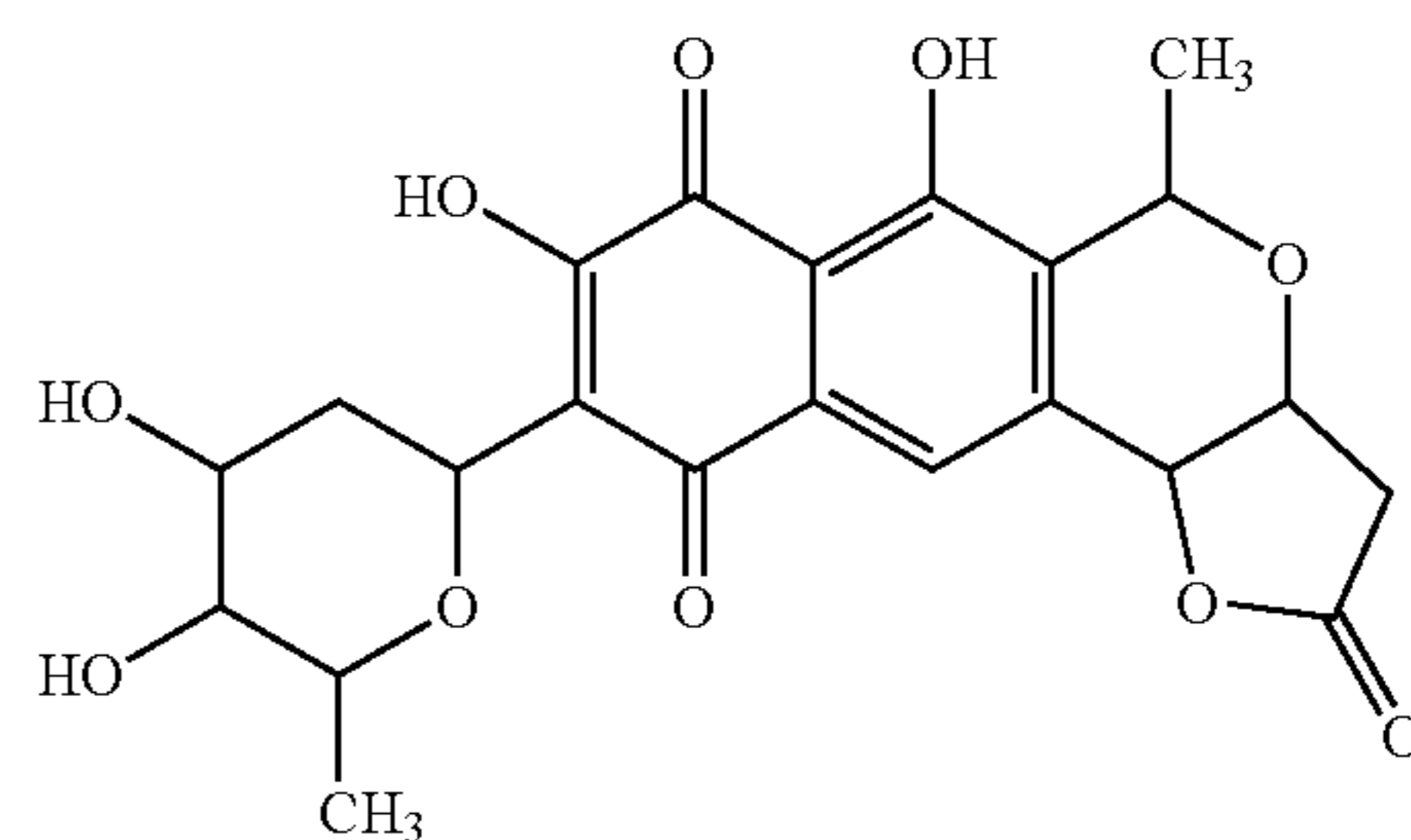
Derivative 1
