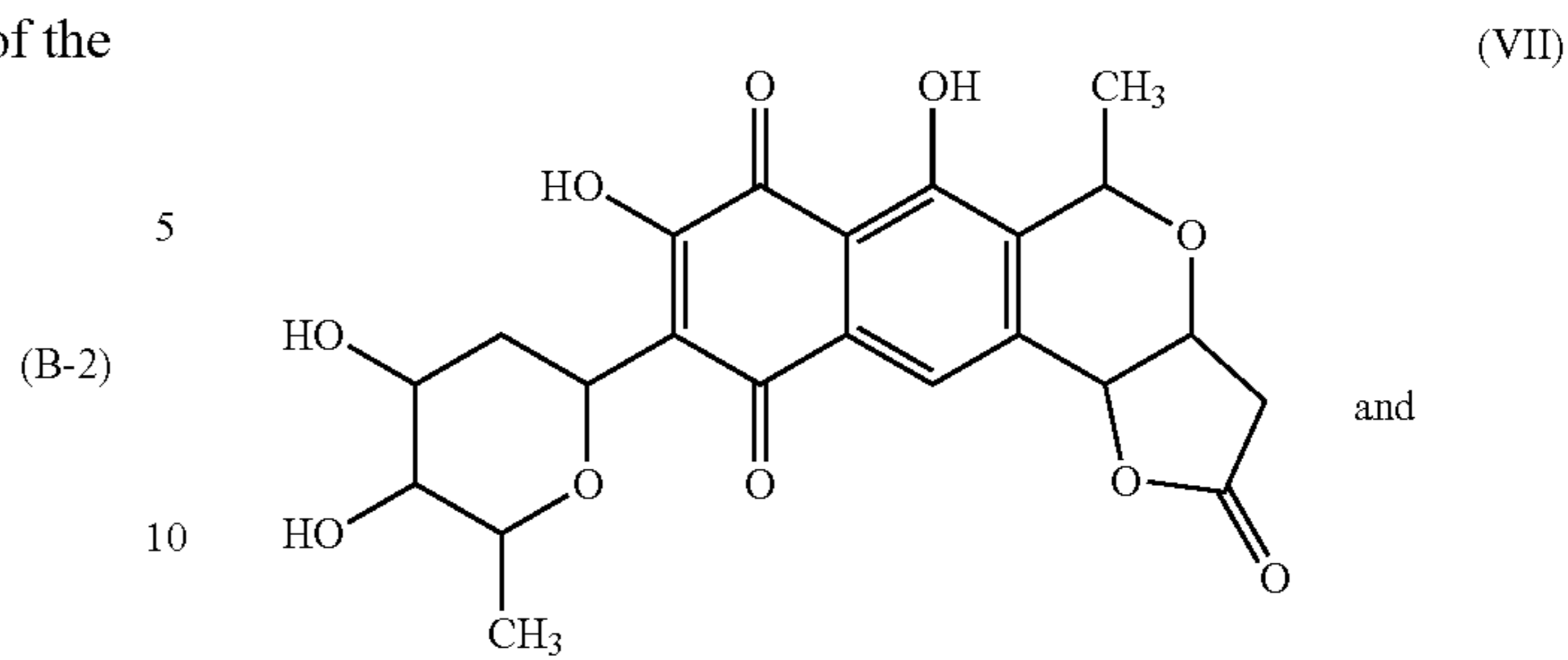
Derivative 1
