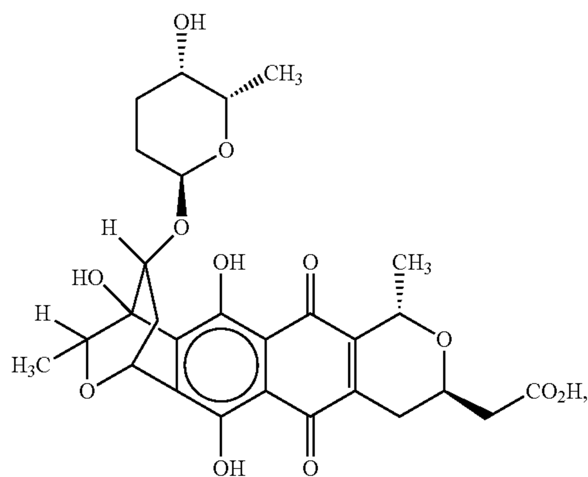
dihydrogranaticin A
