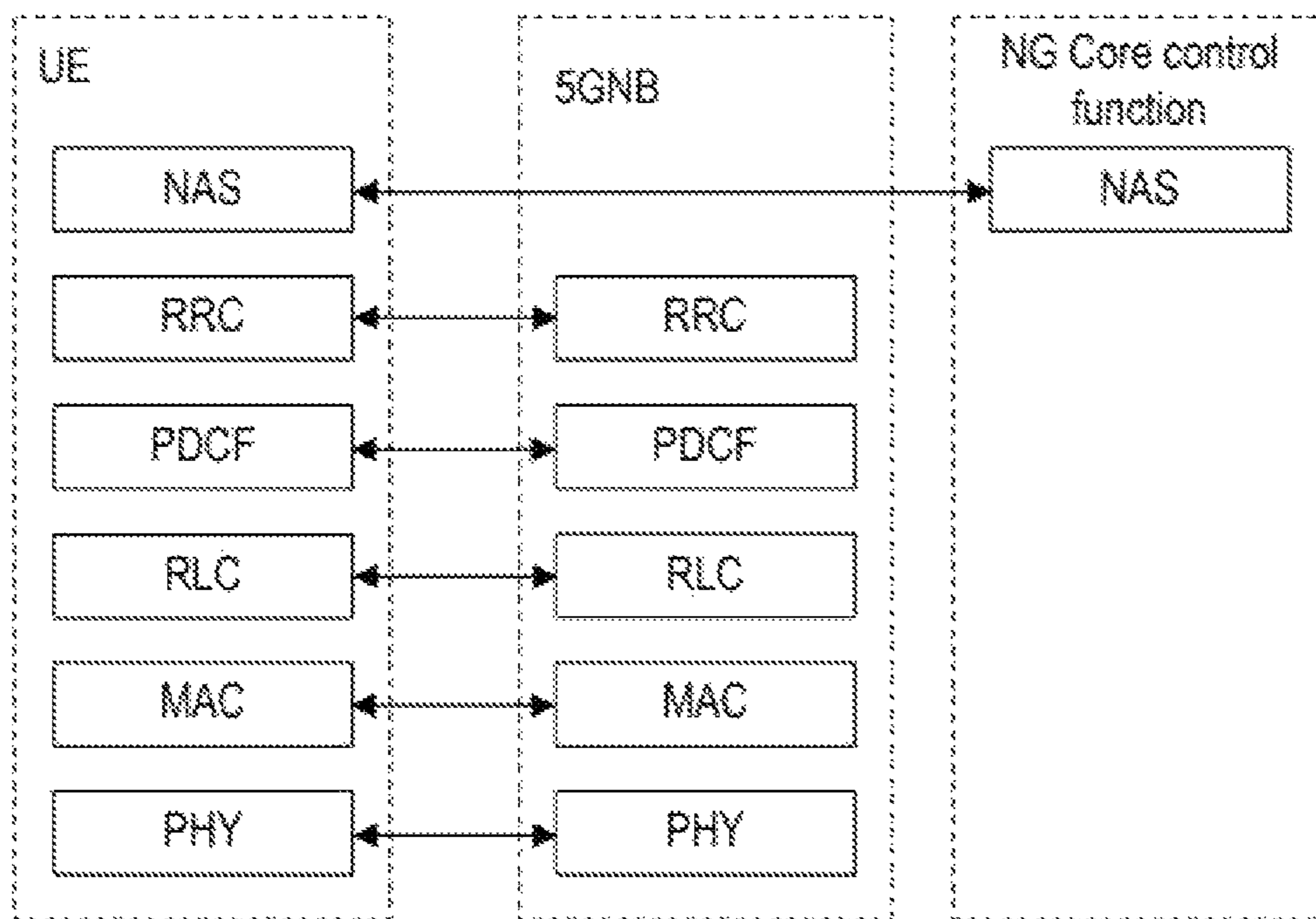
Control Plane Protocol Stack
