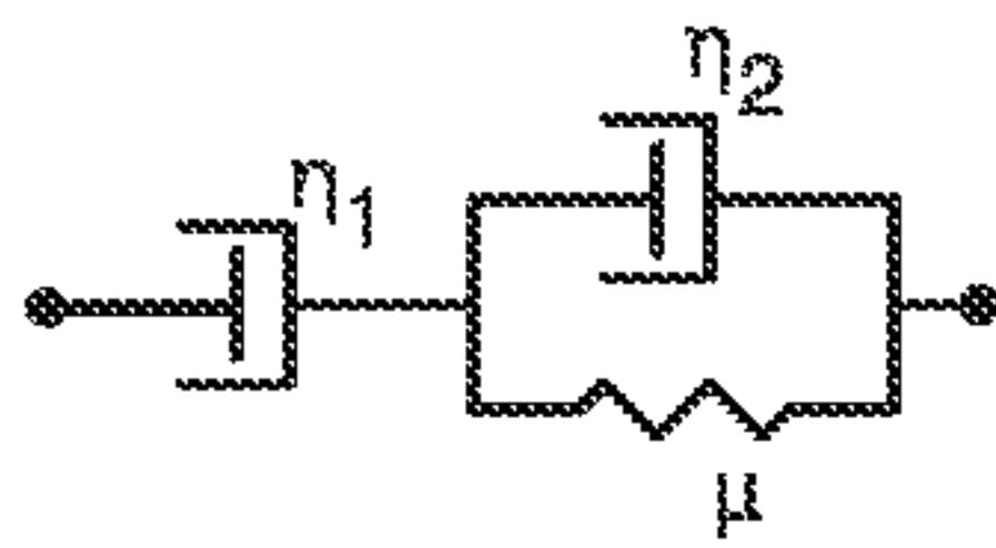
Jeffrey Model
