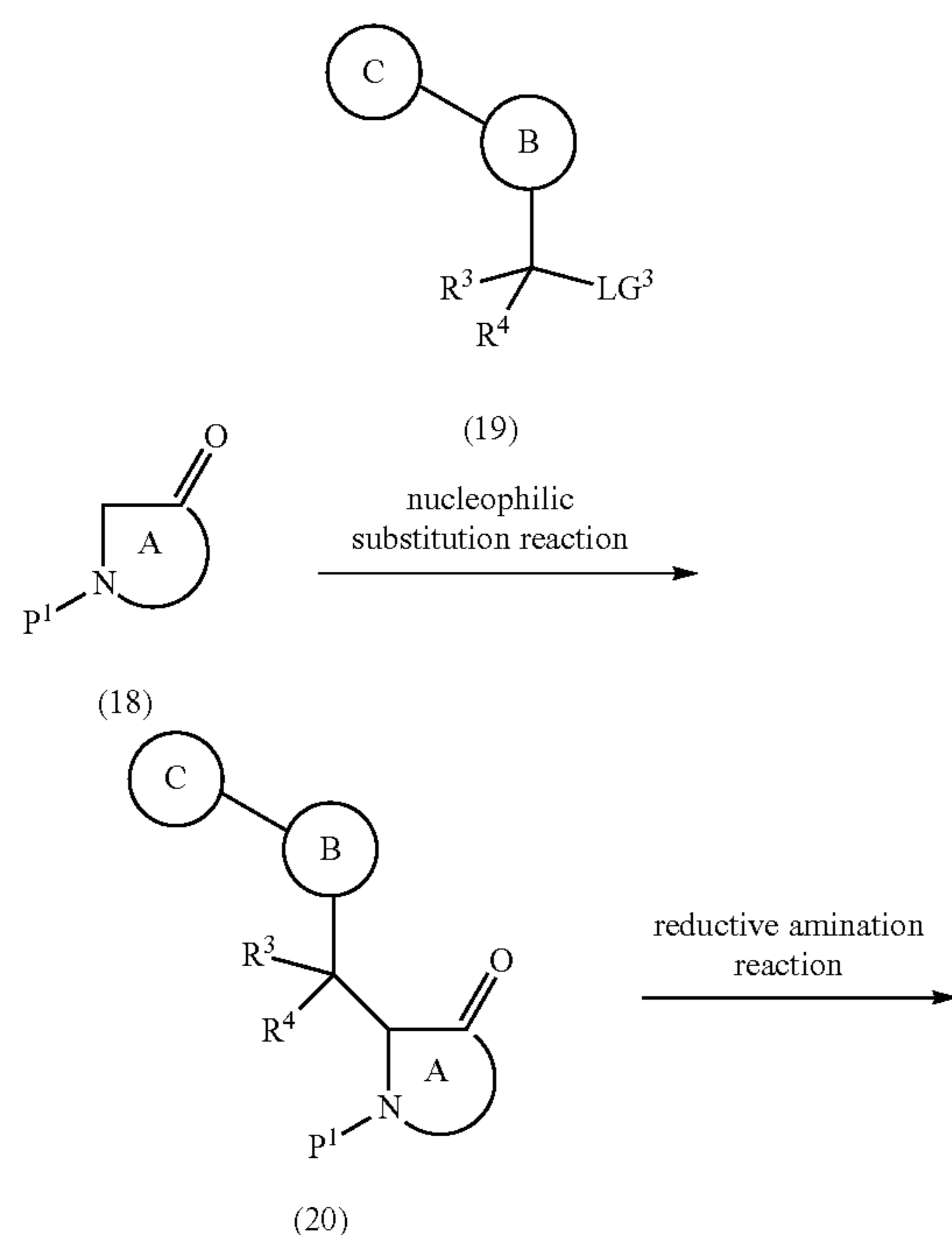
Reaction Scheme 4
