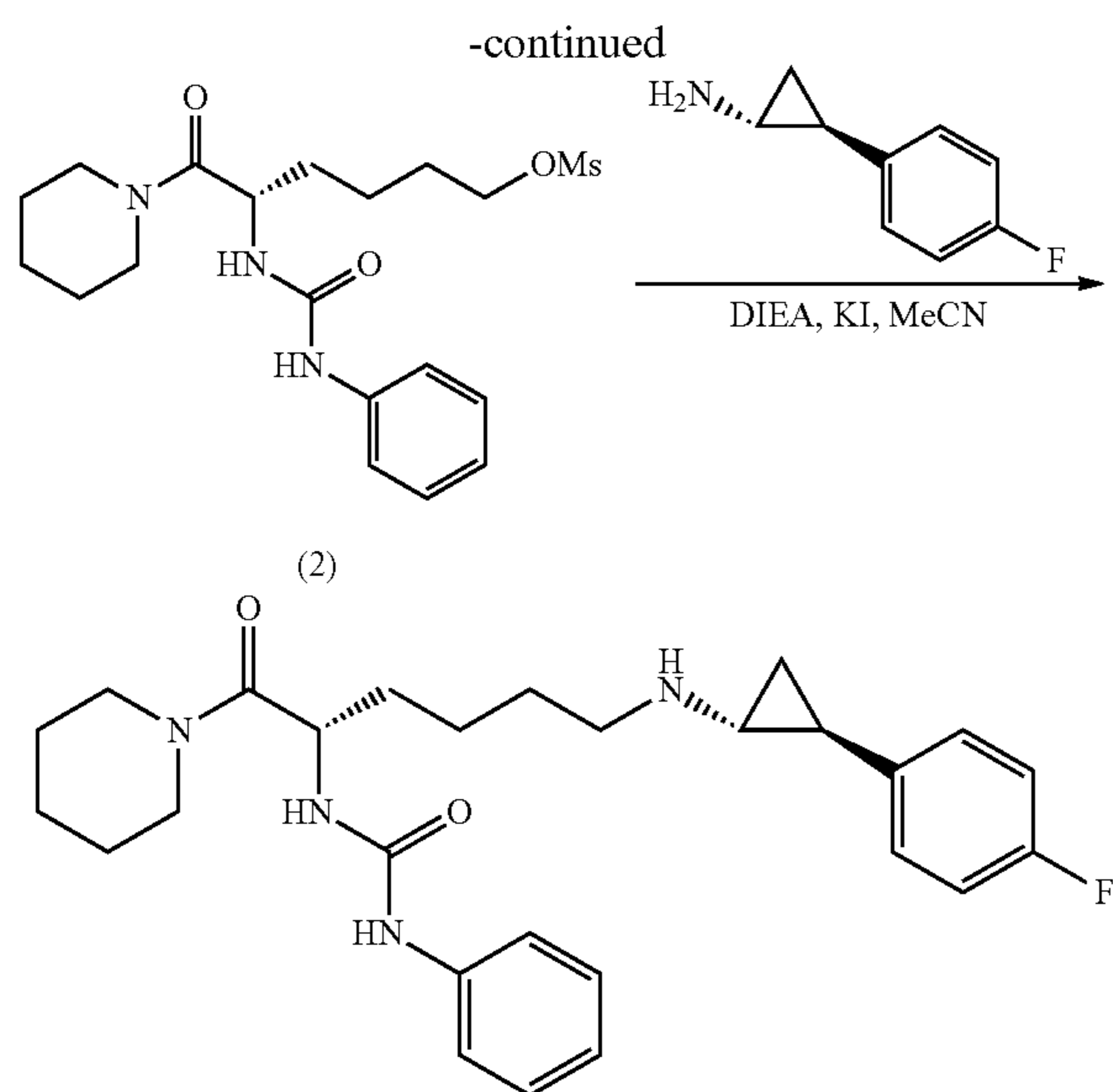
Step 1. (S)-1-(6-hydroxy-1-oxo-1-(piperidin-1-yl)hexan-2-yl)-3-phenylurea (1)
