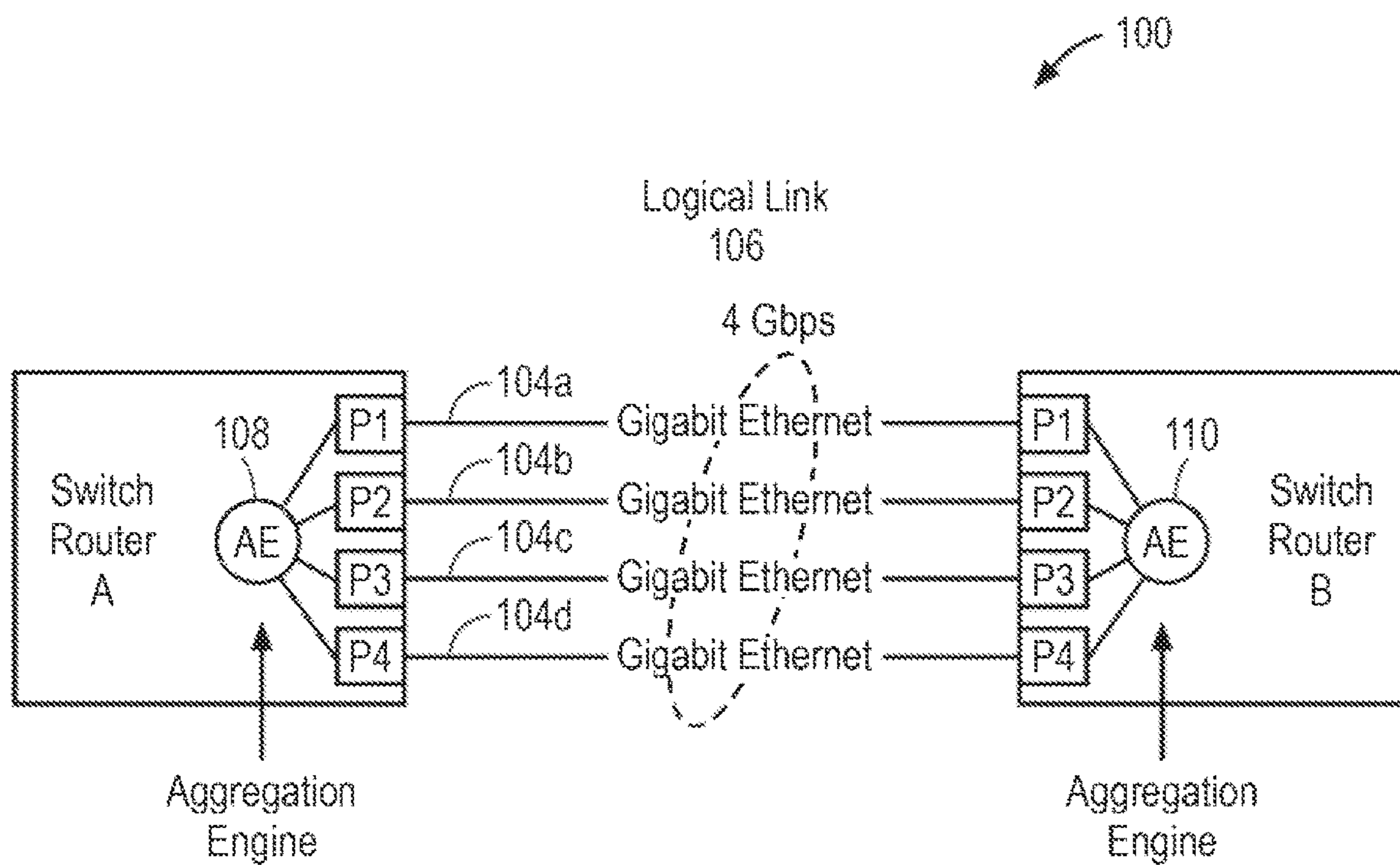
FIG. 1 (PRIOR ART)
