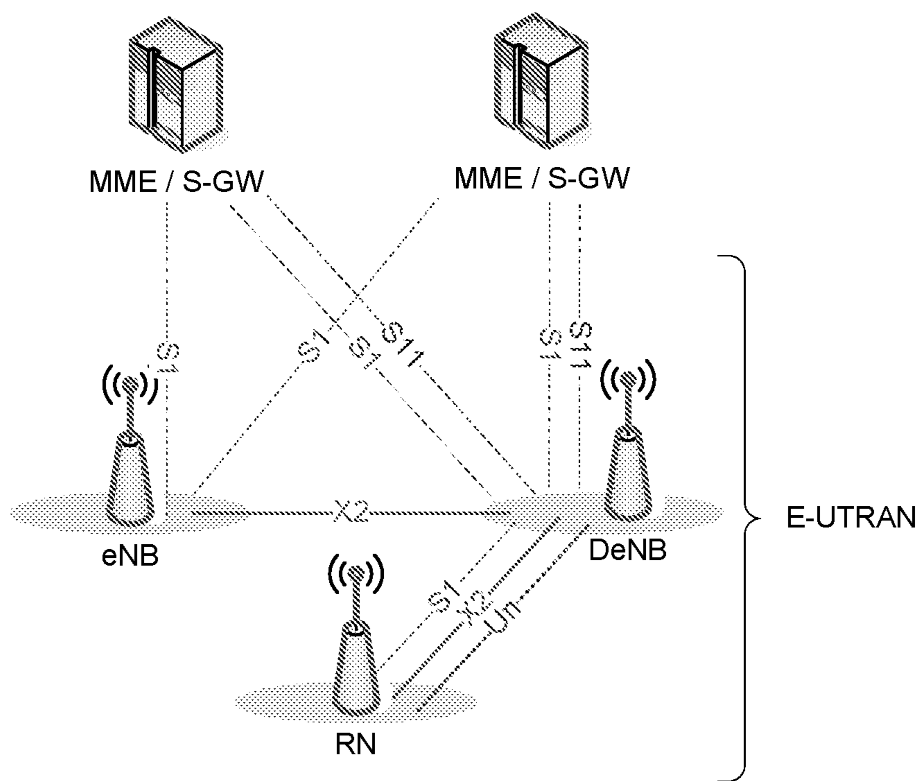
FIG. 16 (PRIOR ART)
