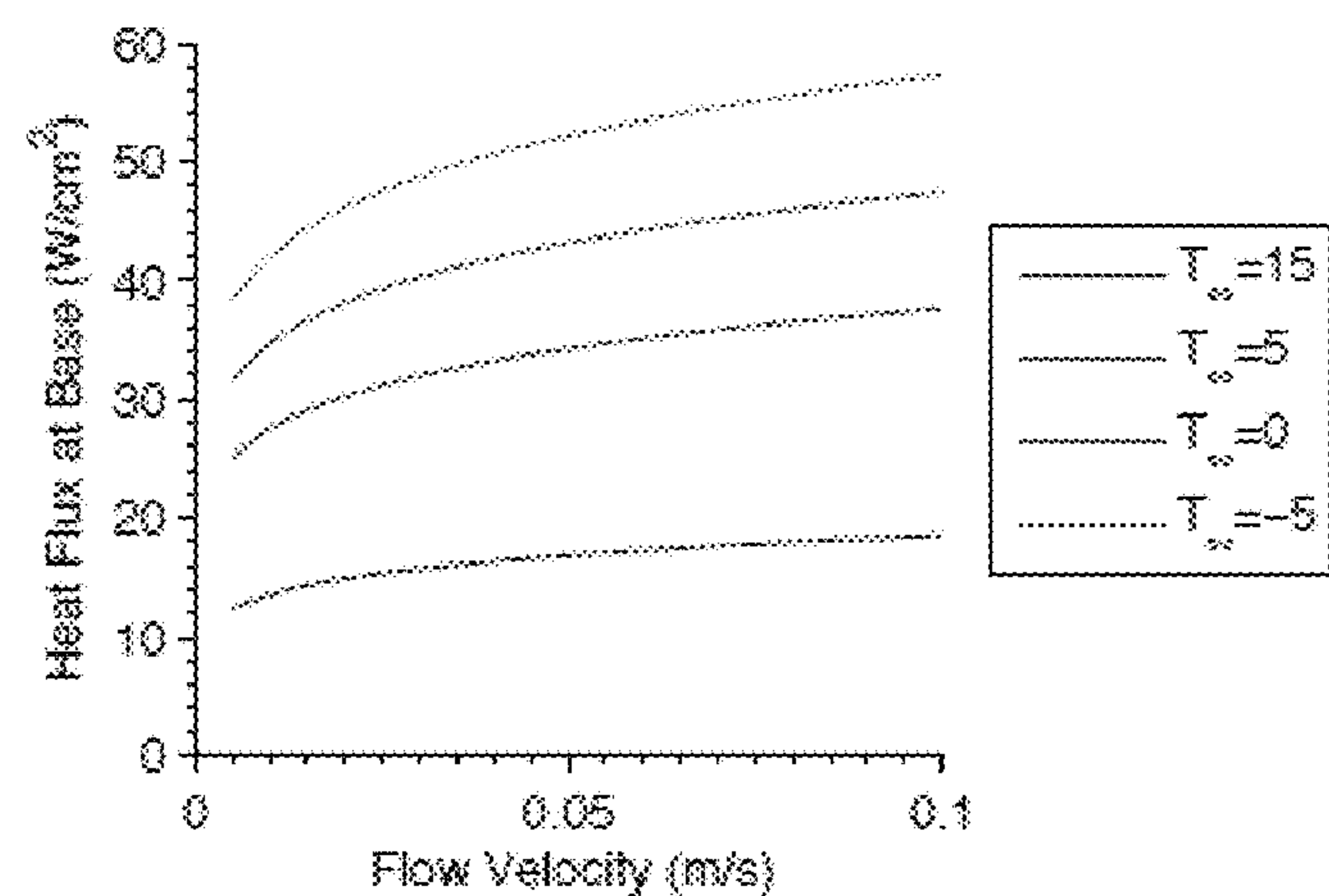
(b) Heat Flux at Base
