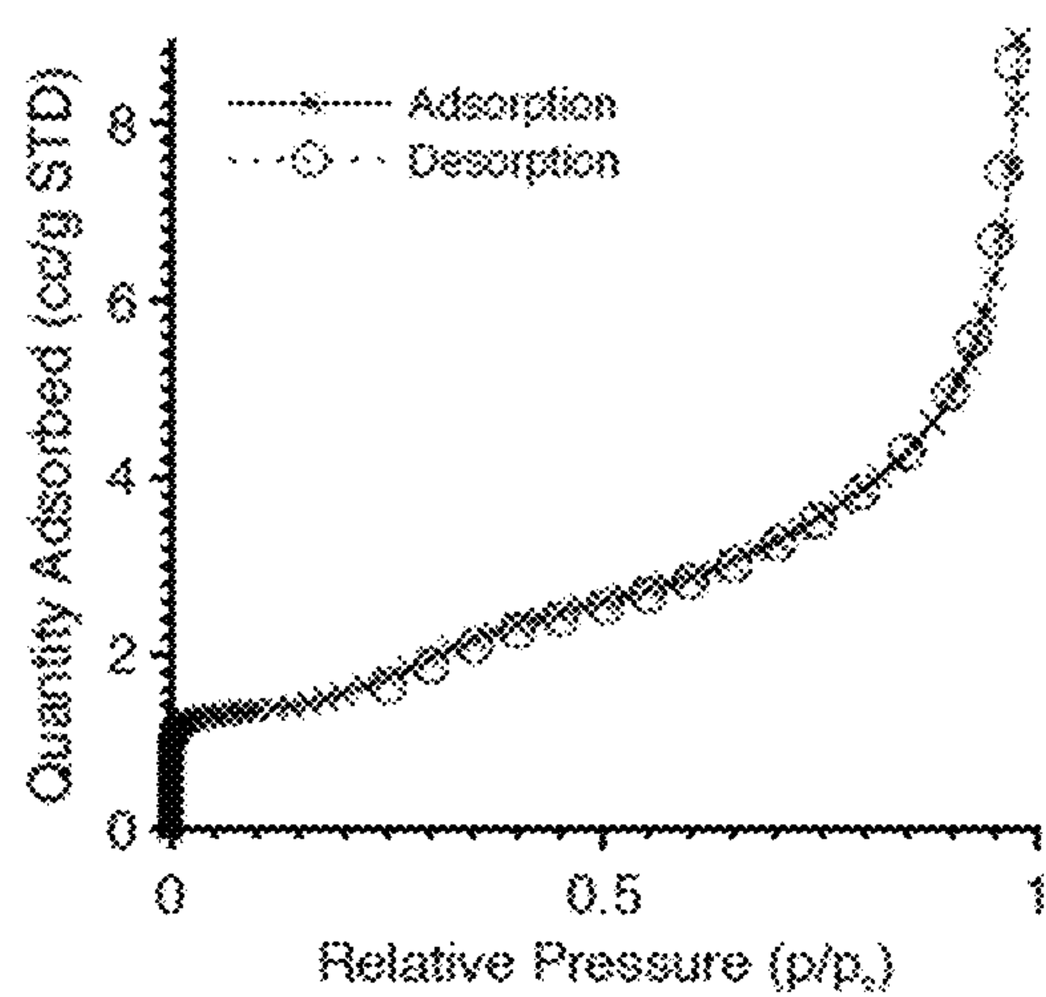
(a) Nitrogen Isotherm
