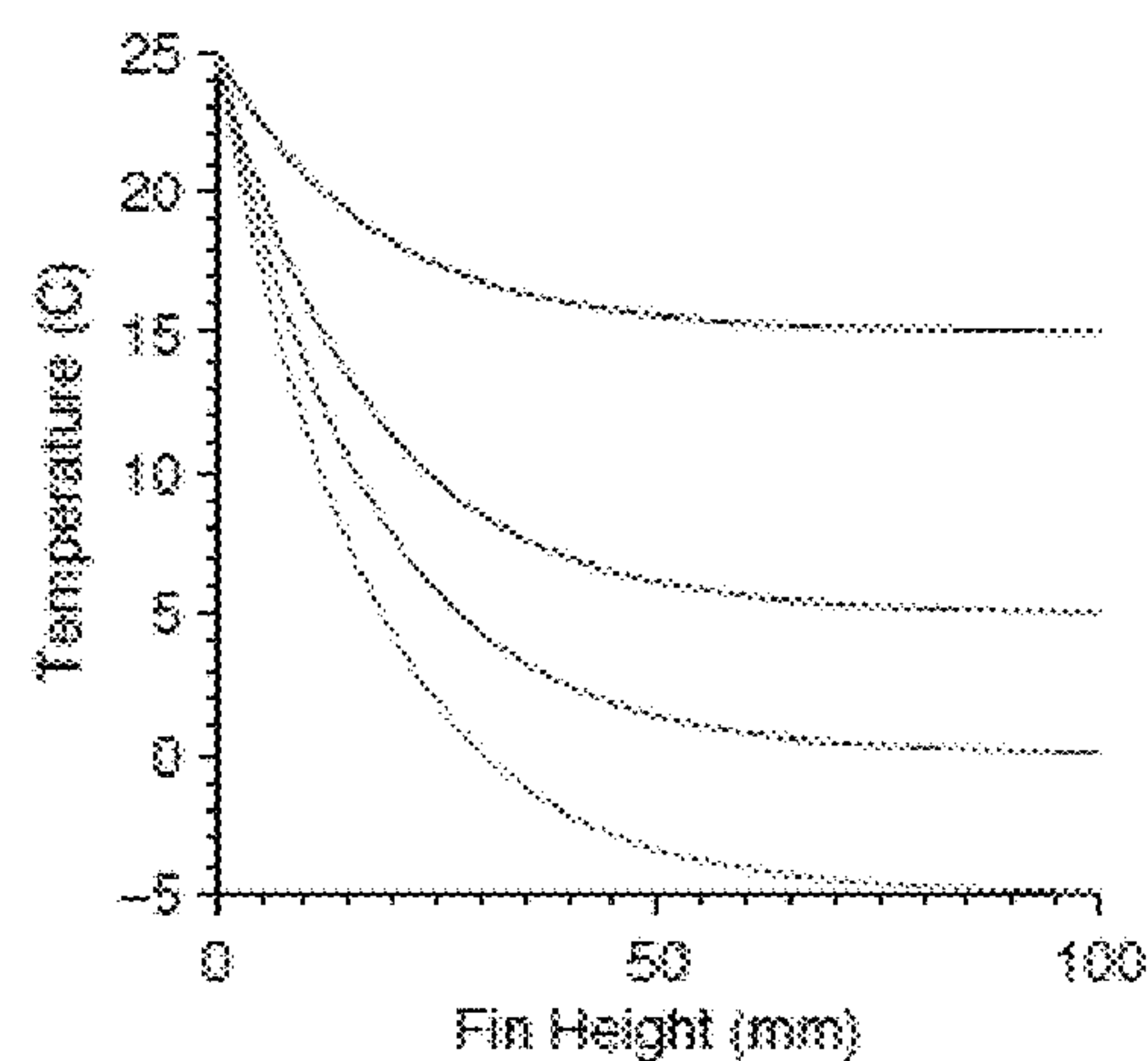
(a) Temperature for U = 0.1 m/s
