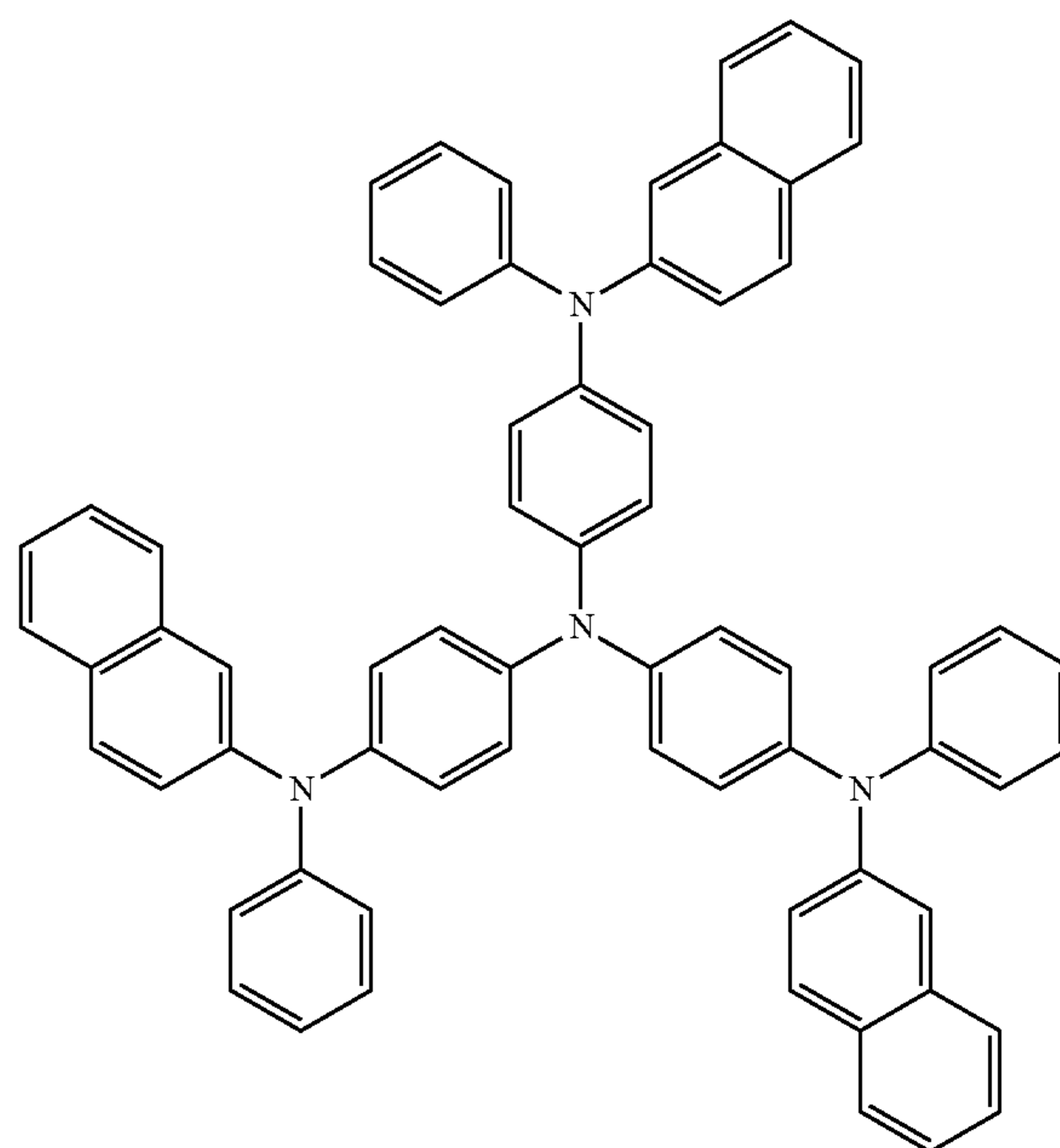
2-TNATA
