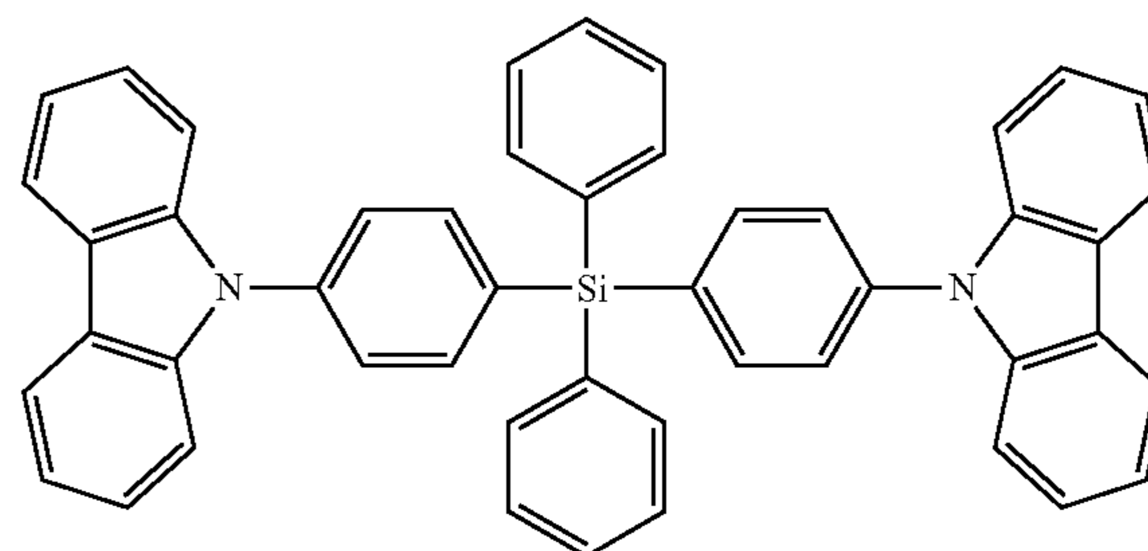
BCPDS
