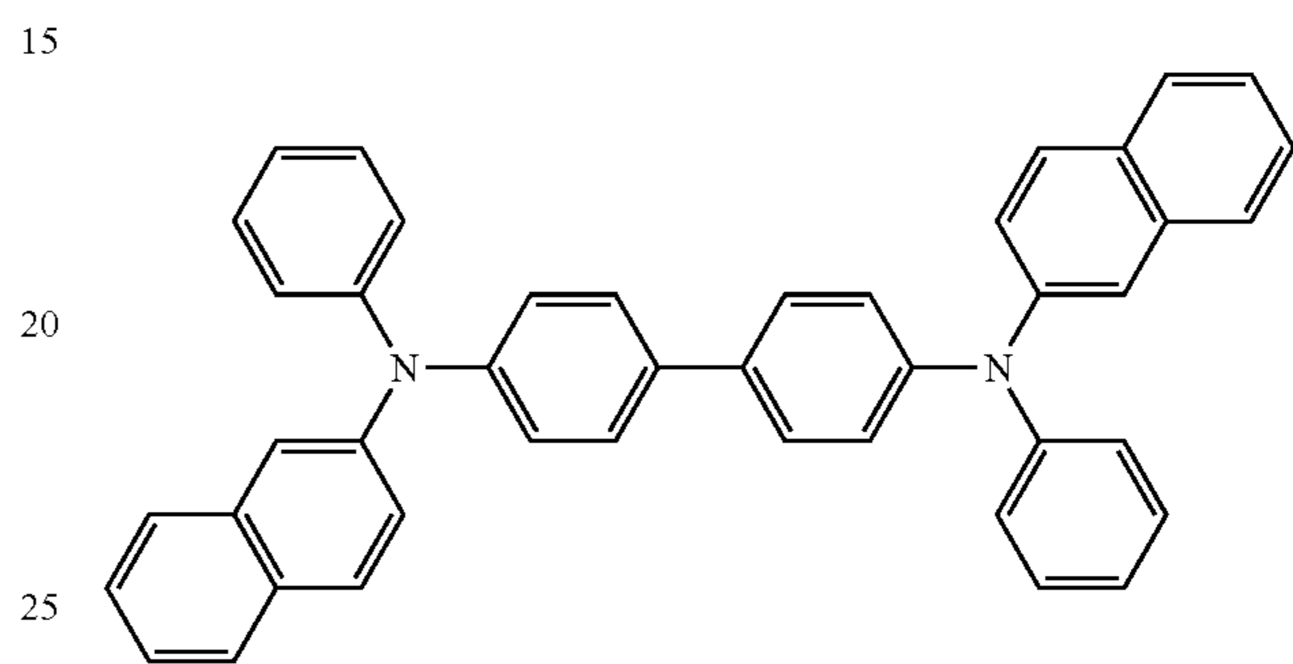
\beta -NPB
