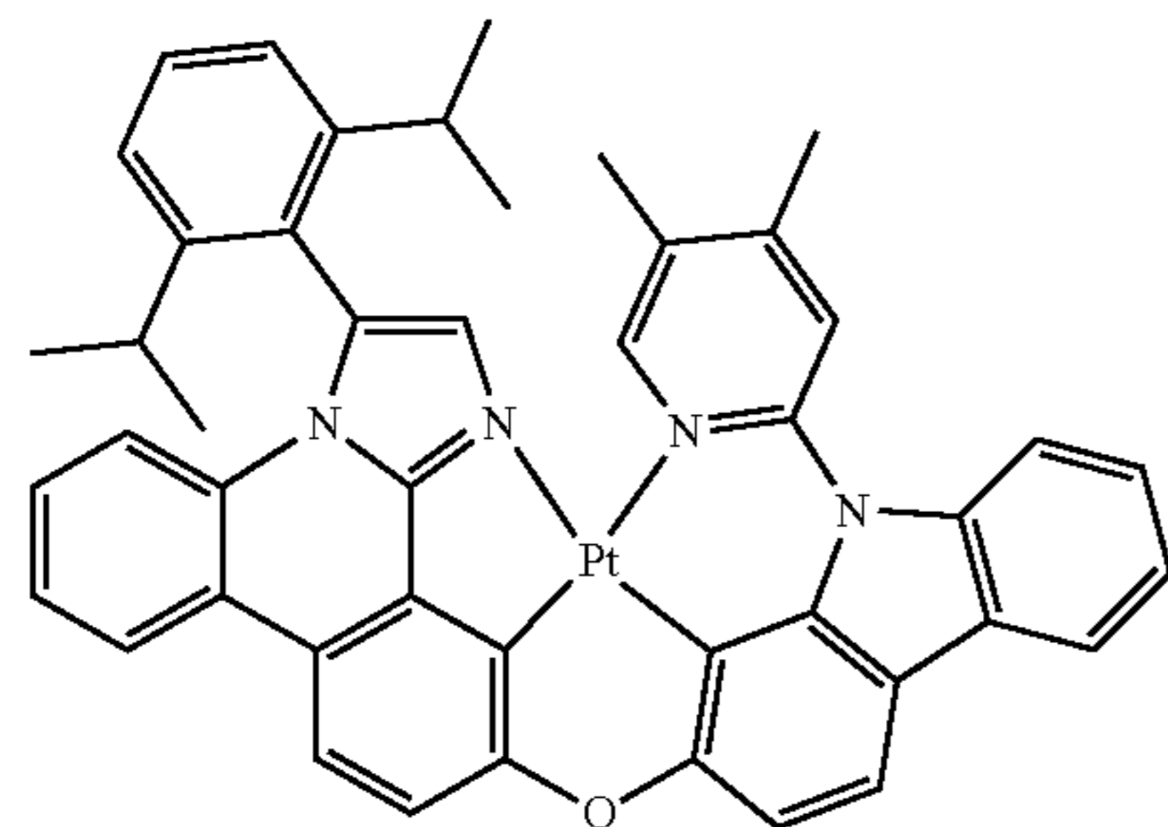
Compound B
