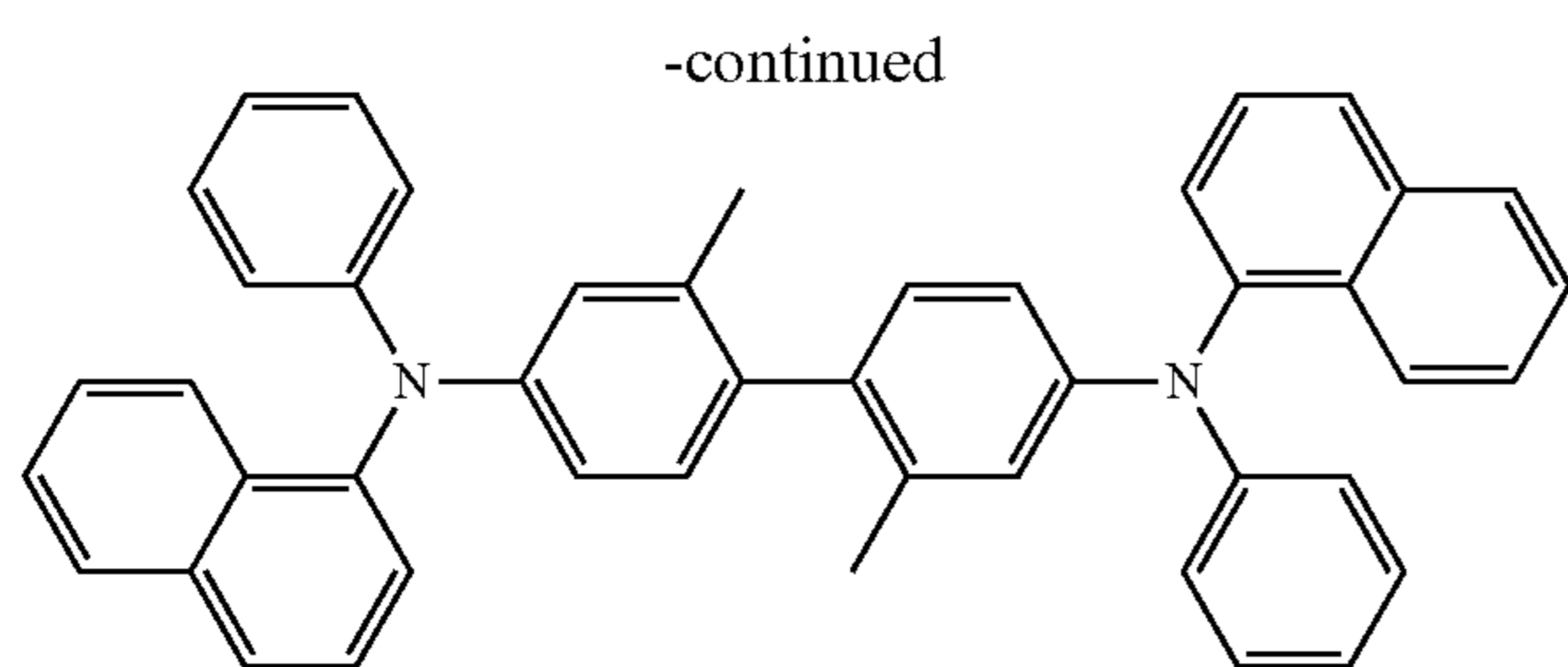
methylated NPB
