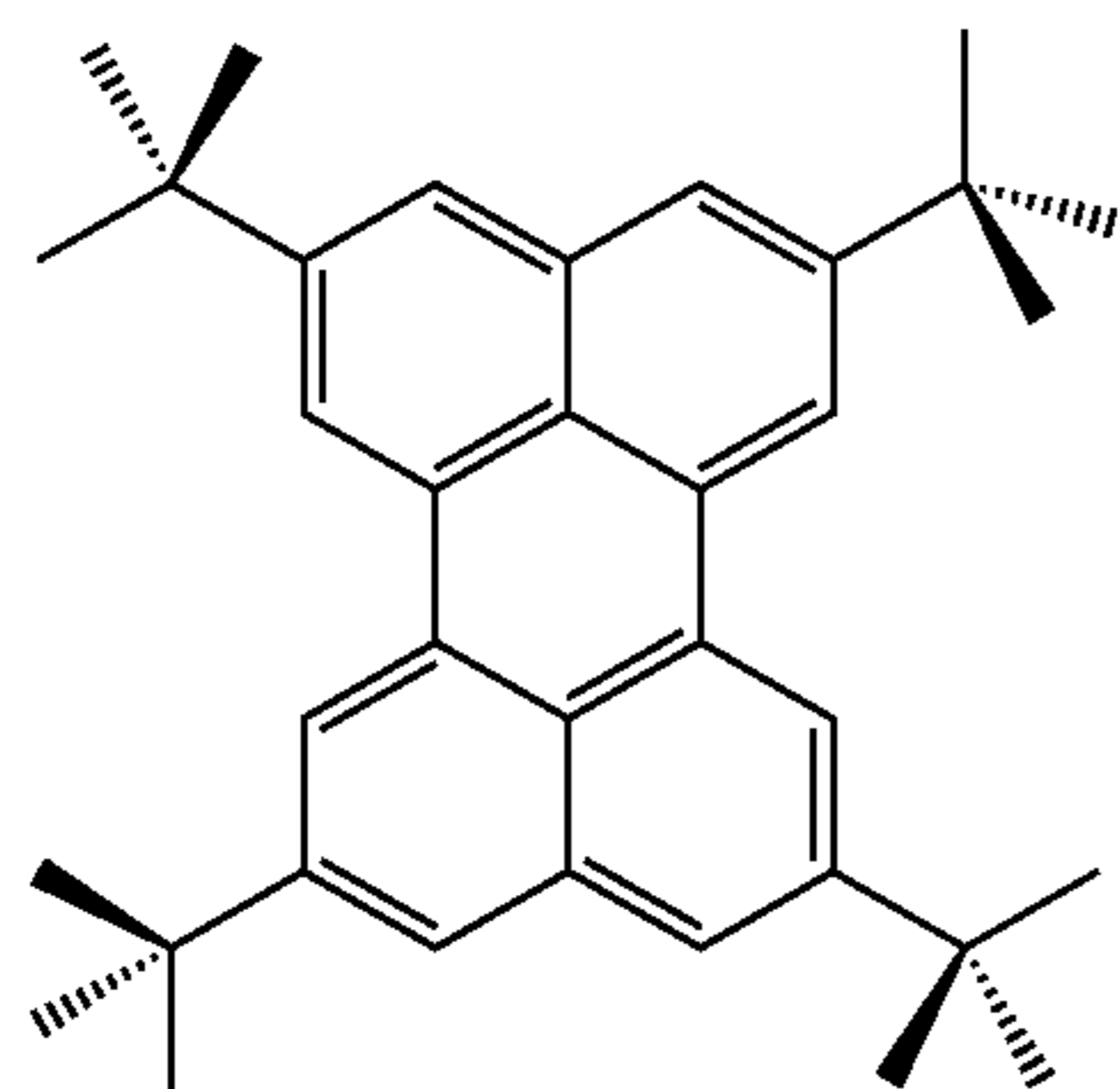
TBPc
