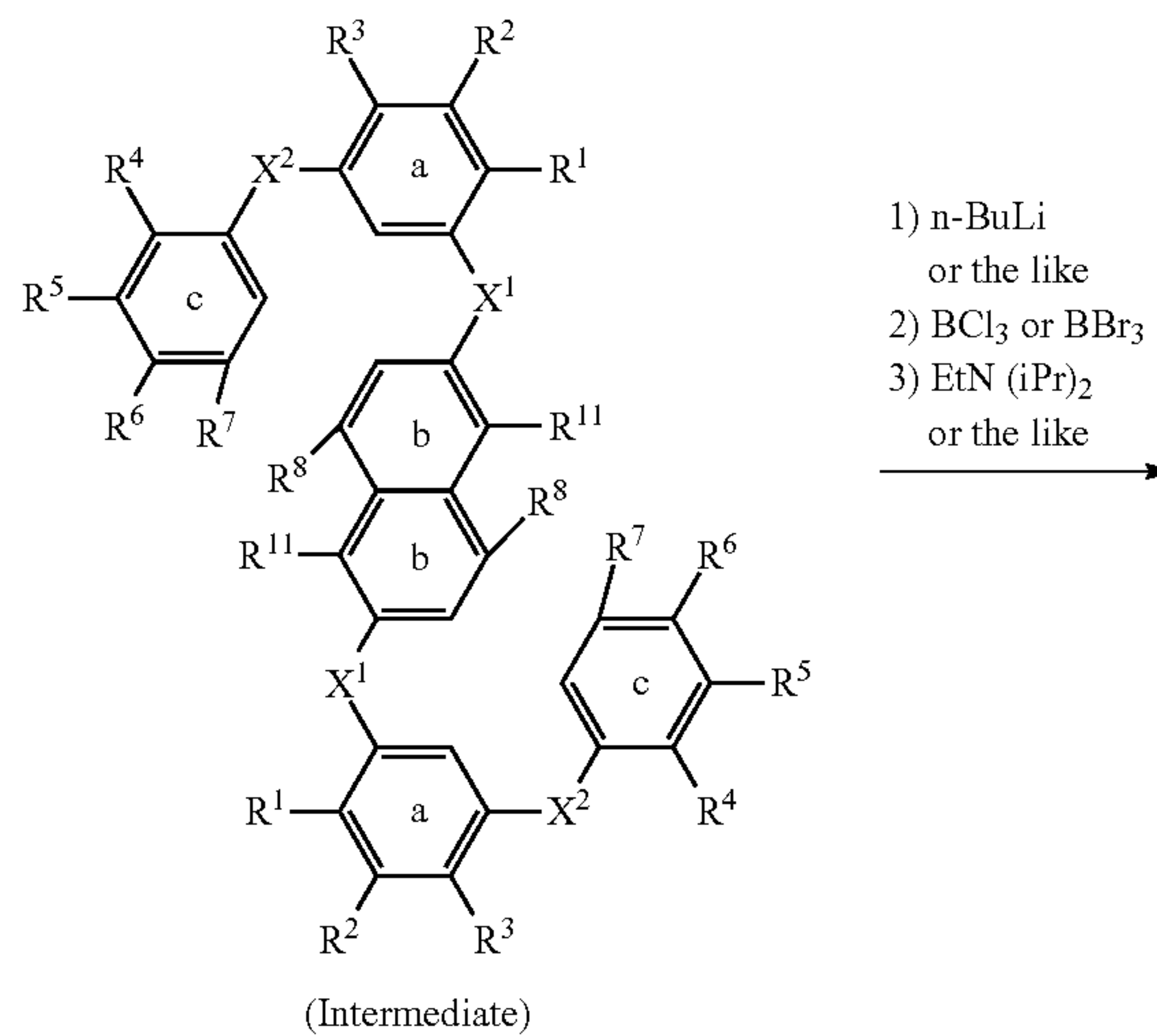
Scheme (5)
