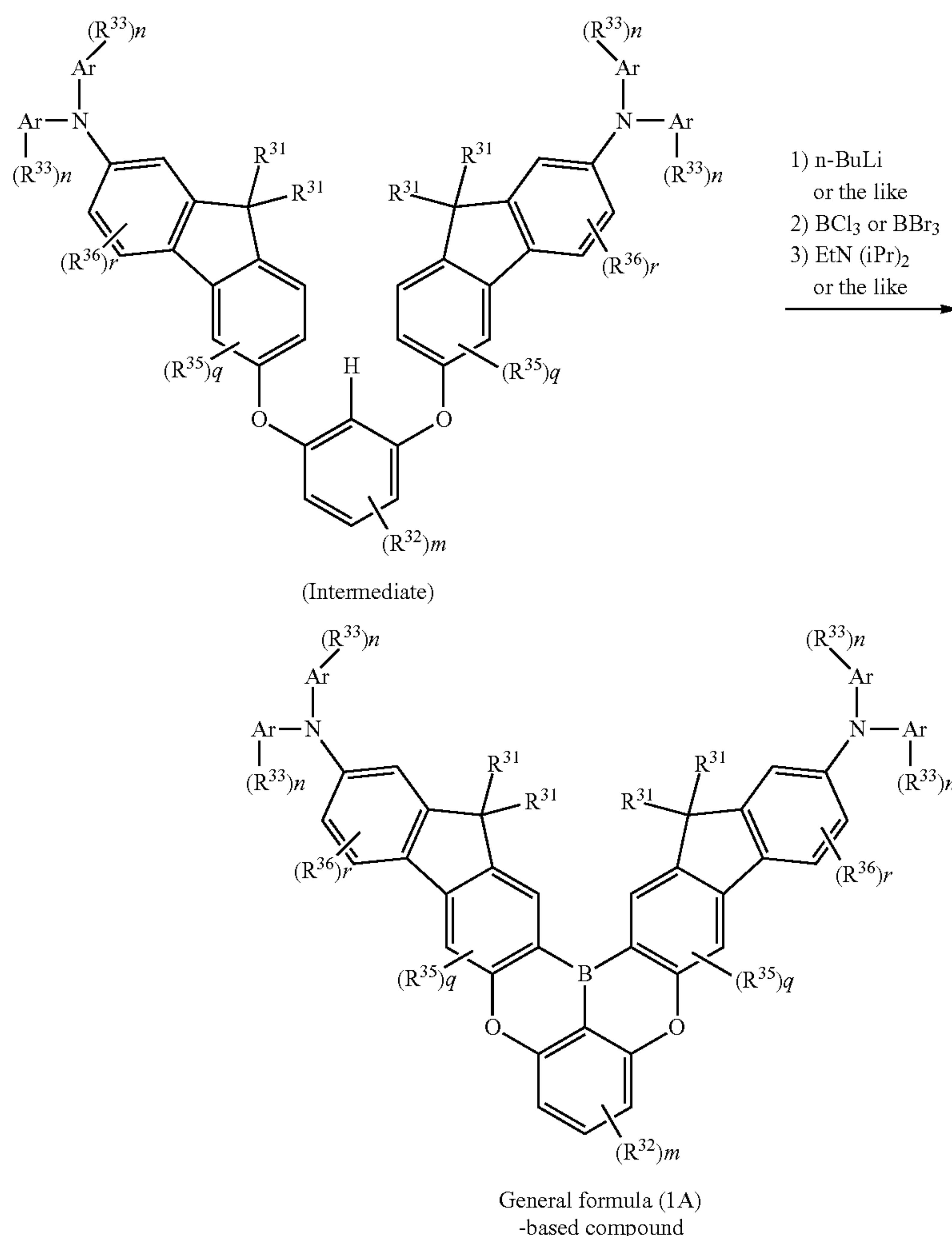
Scheme (1')
