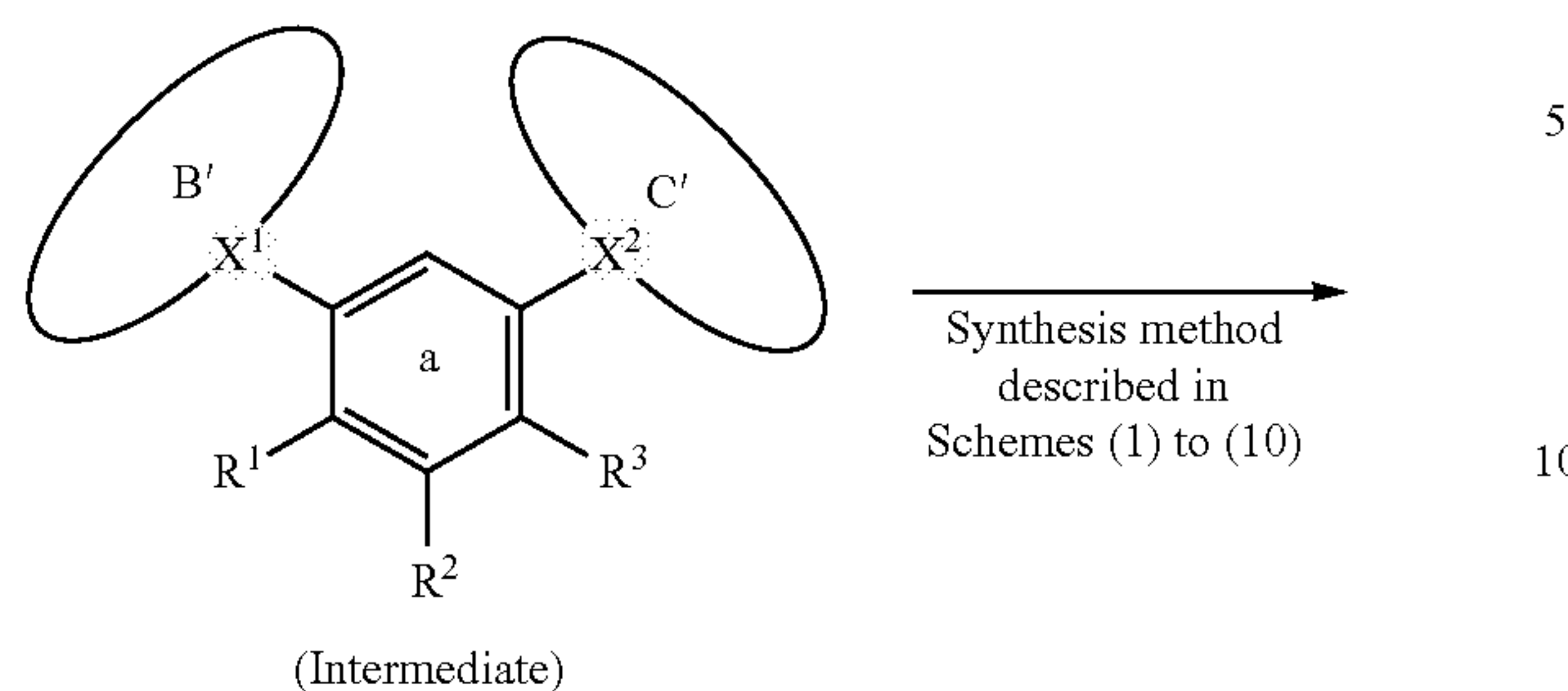
Scheme (13)
