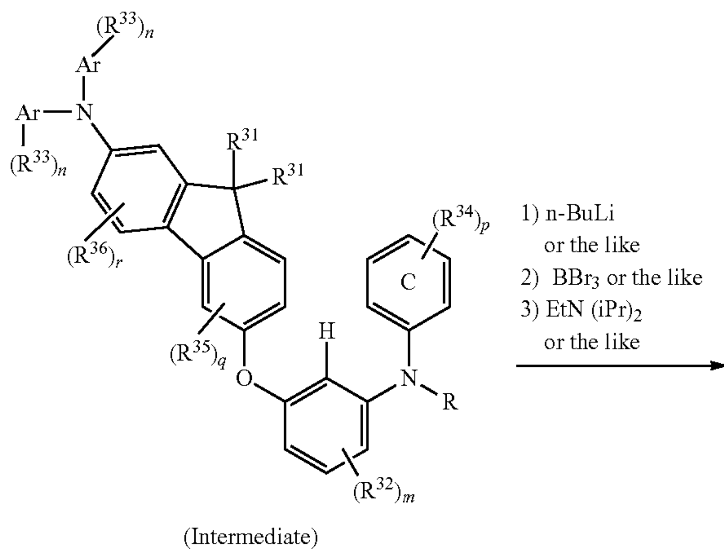
Scheme (6')
