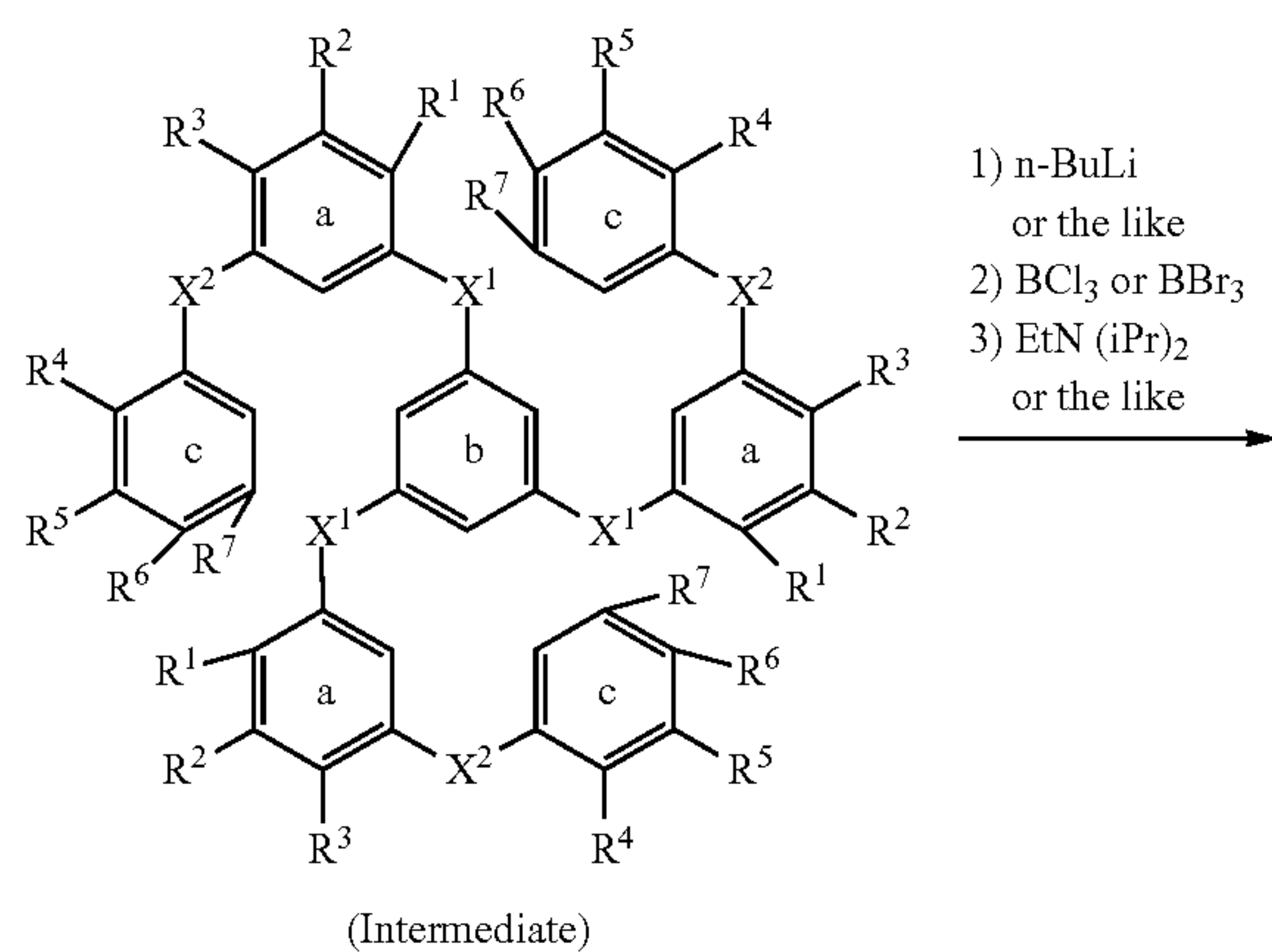
Scheme (4)
