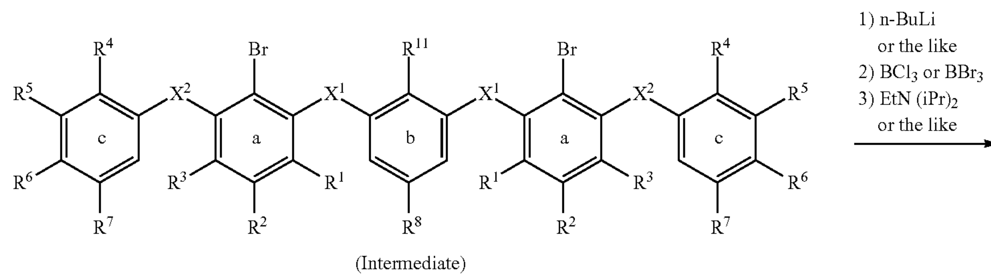
Scheme (9)
