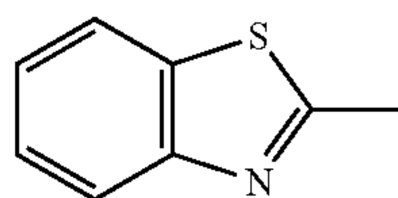
benzothiazole group
