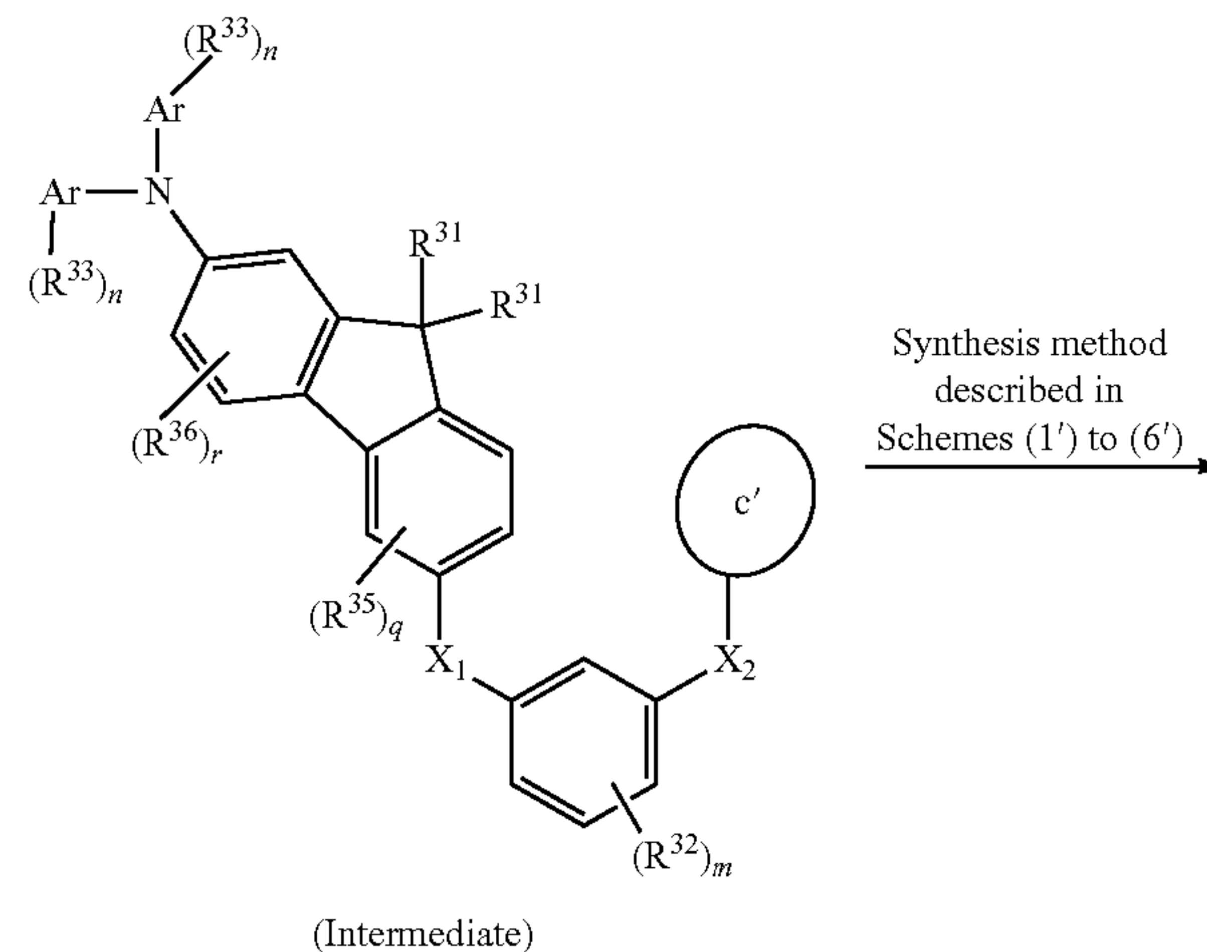
Scheme (7')
