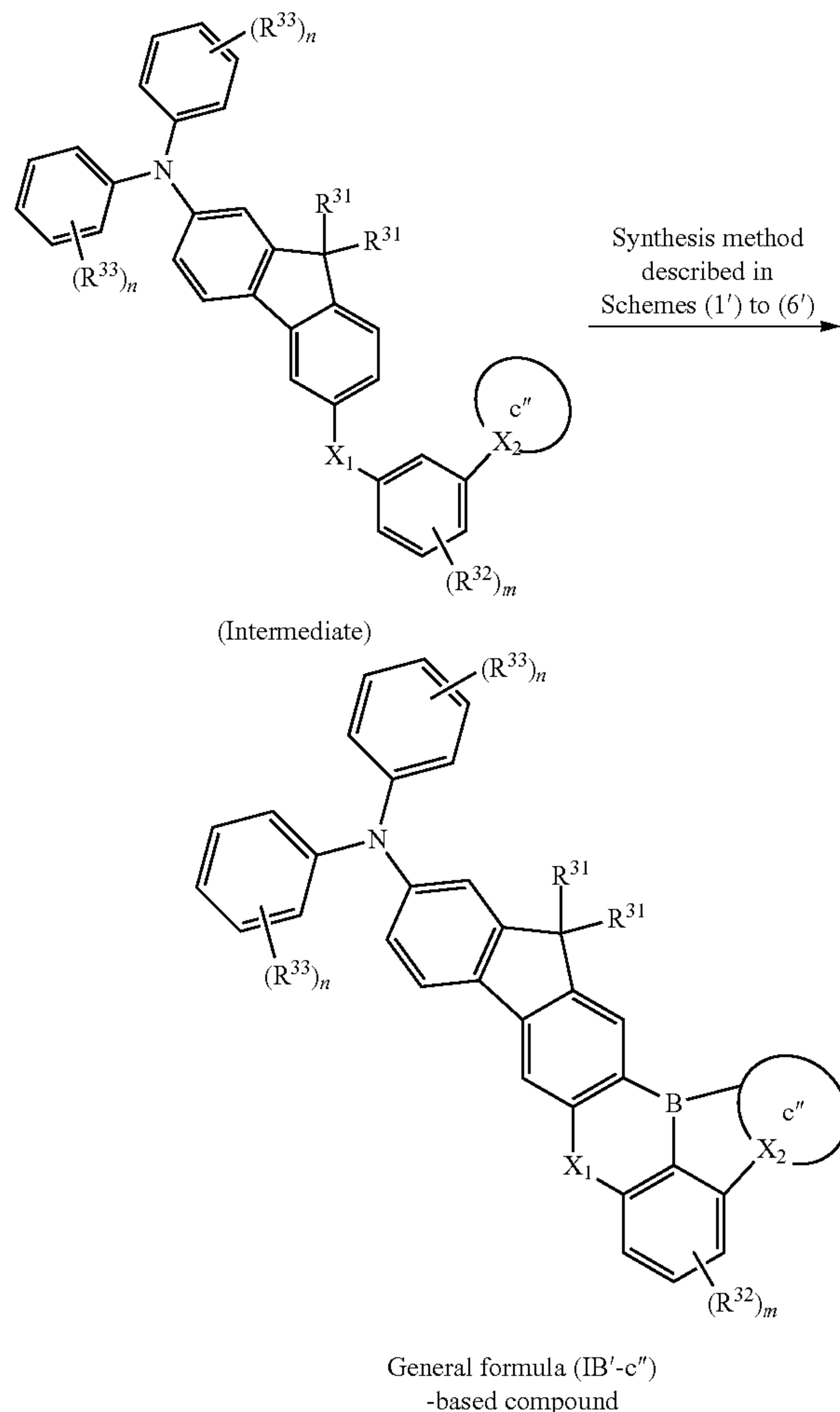
Scheme (10')
