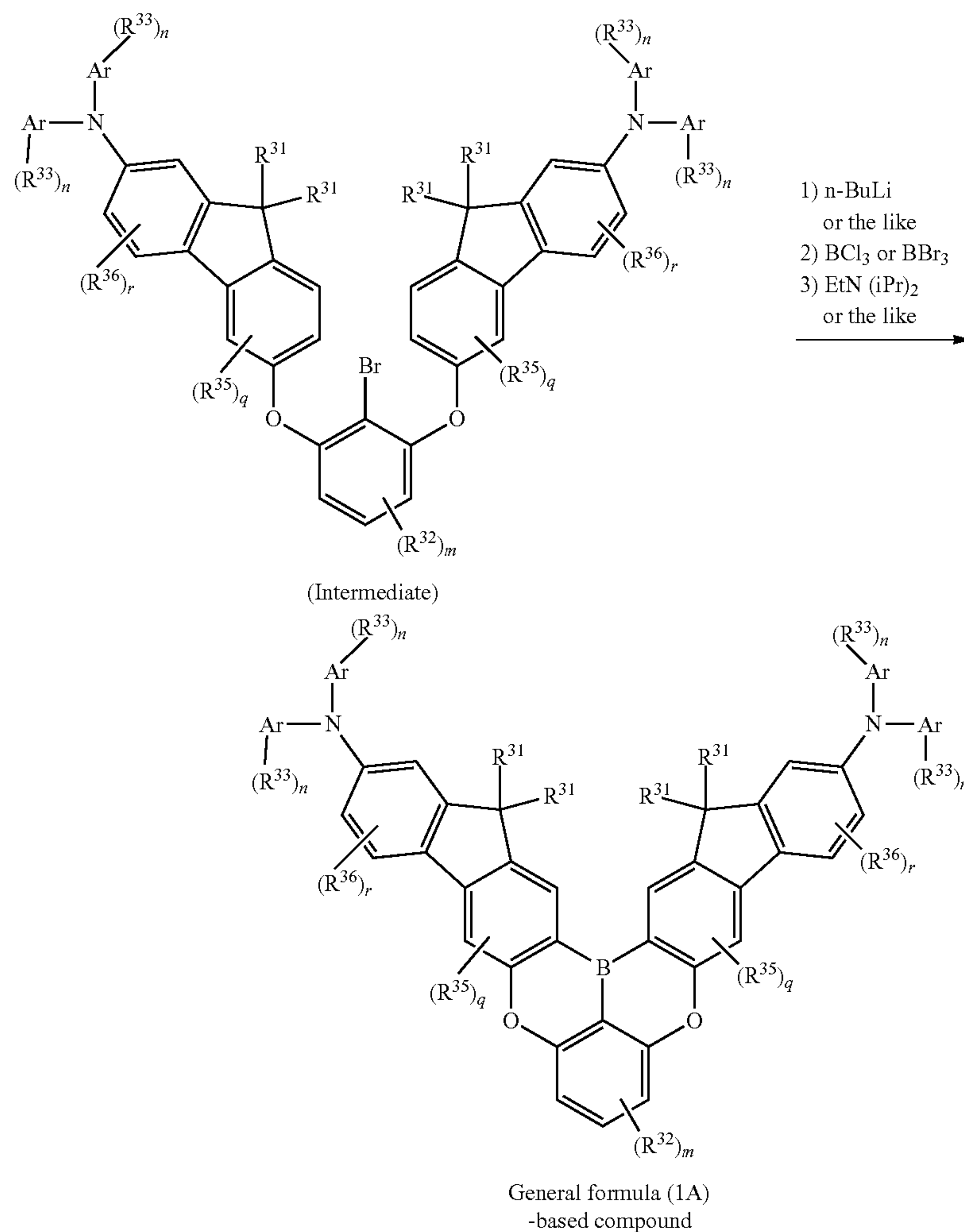
Scheme (3')
