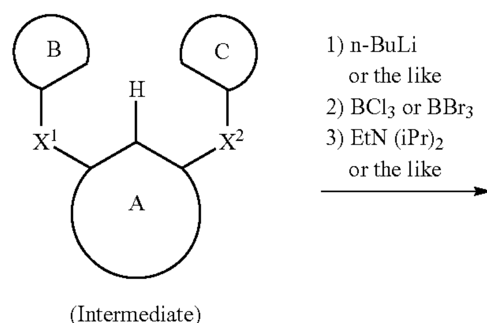
Scheme (1)
