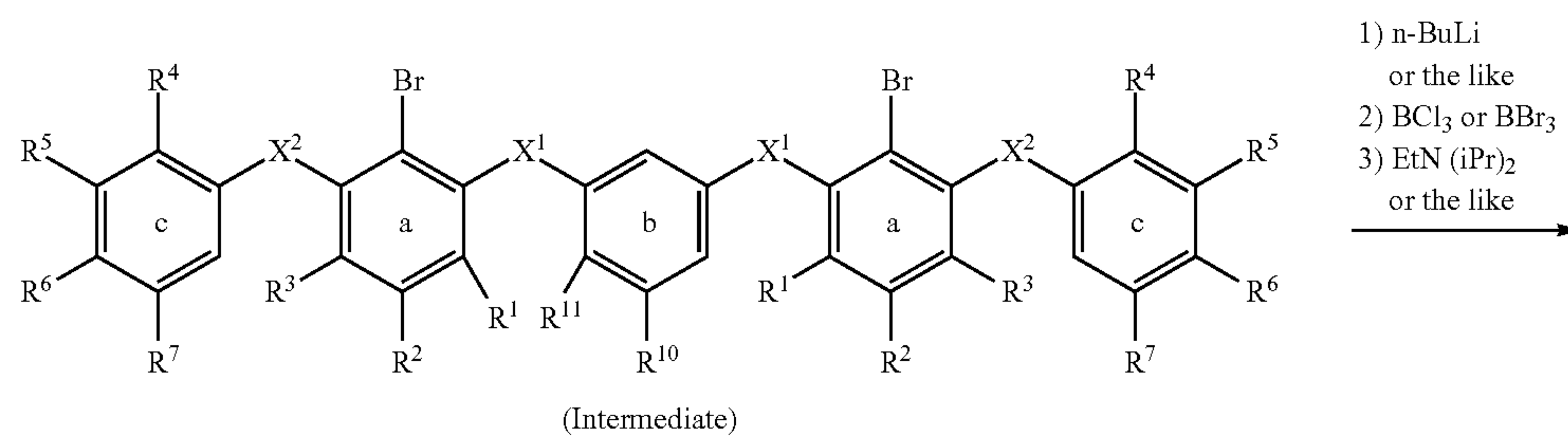
Scheme (9)
