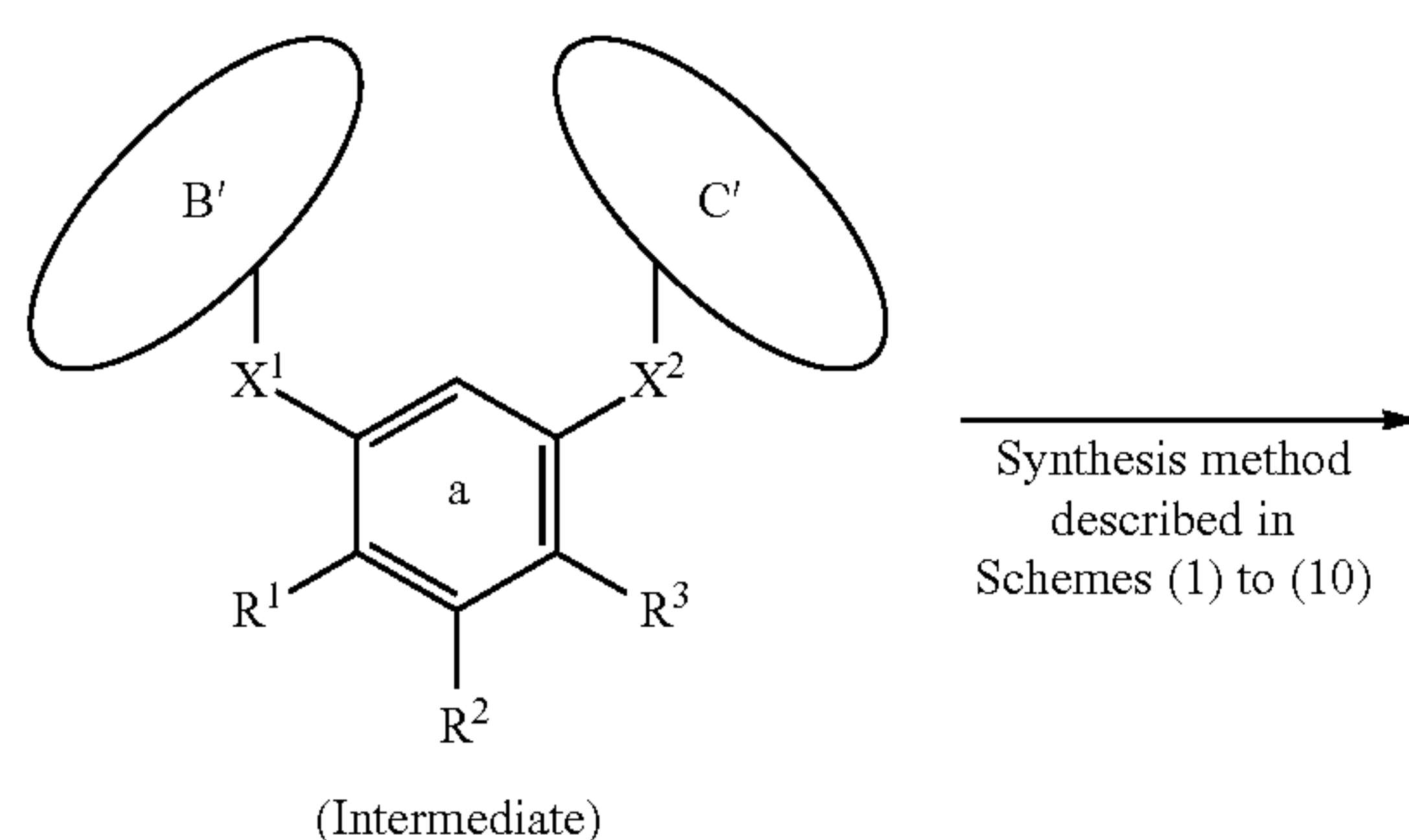
Scheme (11)
