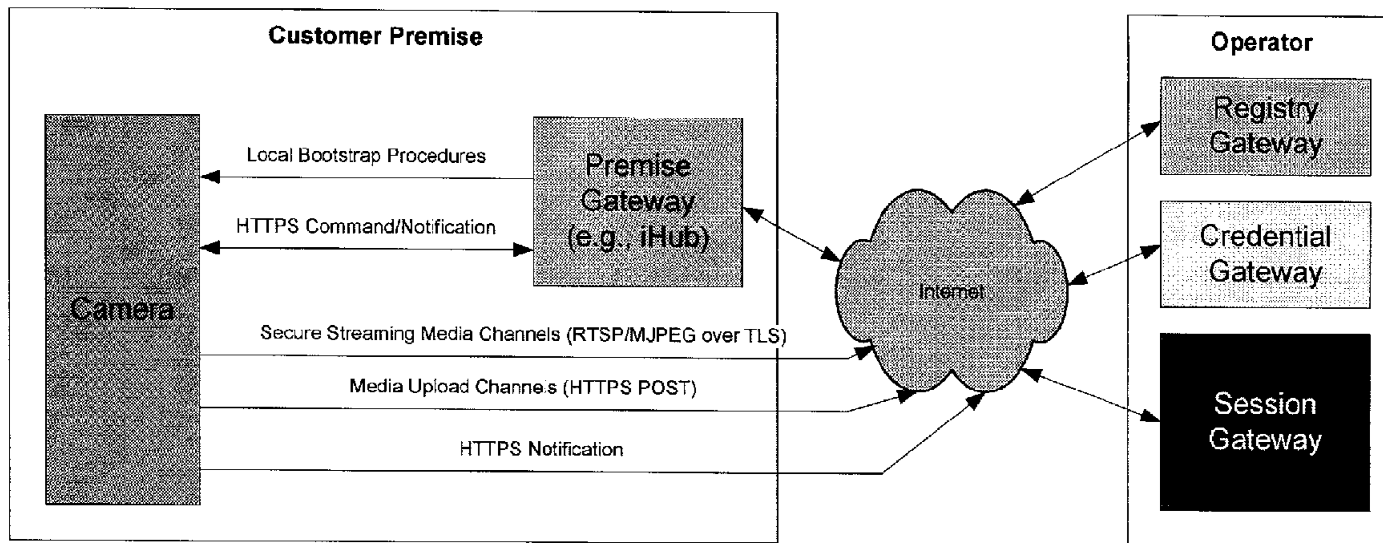
Device with Premises Gateway Deployment Scenario
