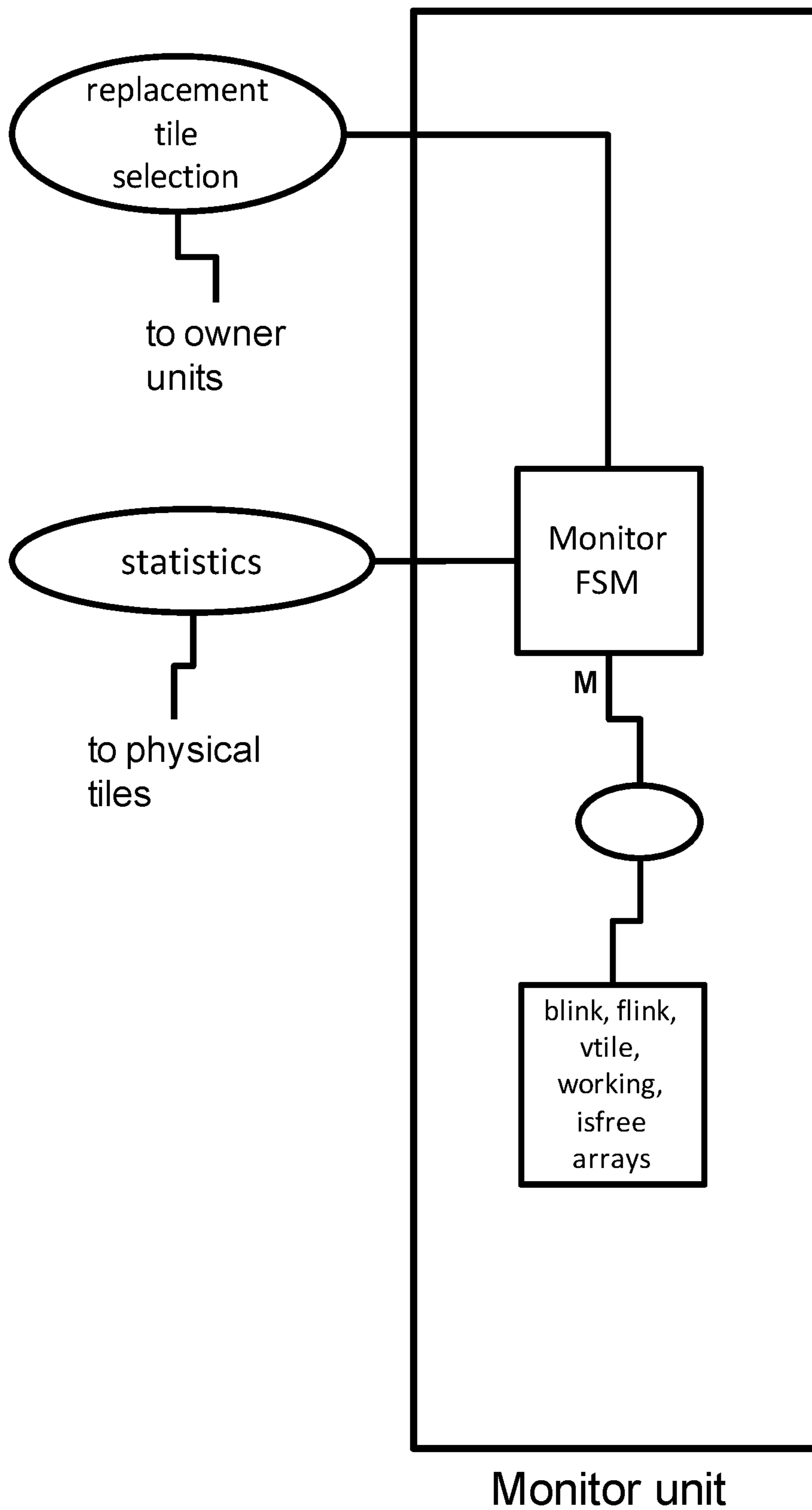
FIG 15 Internal organization of the monitor unit
